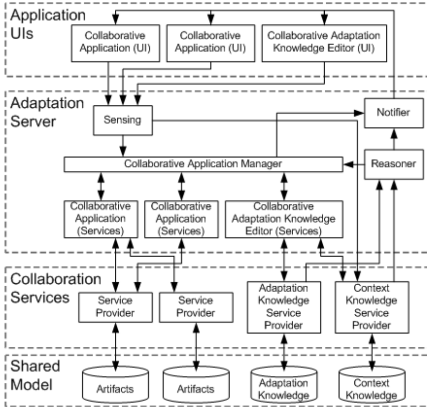
Figure 2 Conceptual Architecture
