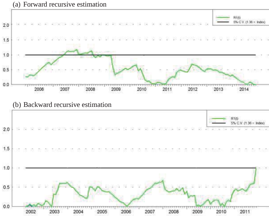
Figure 10: Test for Constancy of the Log-Likelihood, M_t^{10Y}
