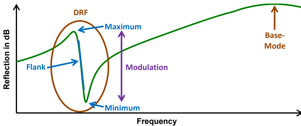
Figure 4-4: General reflection spectrum of the aDSR with resonance feature denotations.
