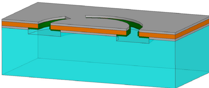
Figure 4-11: Cross-section through a complementary aDSR with undercut on quartz-glass substrate (blue) with gold layer (orange), chrome adhesive and cover layers (gray) and DNA (green) deposited at the bare gold surface. (Layer thicknesses are not true to scale).
