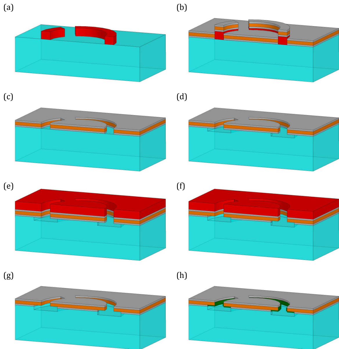
Figure 4-21: Production steps of the biochip depicted at a cross-section (not true to scale) through an aDSR with quartz-glass substrate (blue), chrome (gray), gold (orange), photo resist (red), and DNA sample (green).
