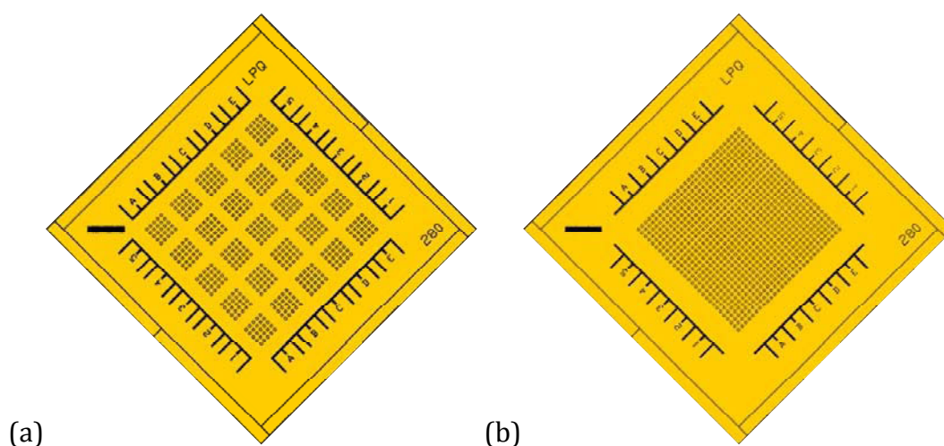
Figure 6-1: Biochip designs with (a) 25 arrays of 5 x 5 resonators and (b) one array of 29 x 29 resonators. Total size is 24 mm x 24 mm. E-field is vertically polarized.
