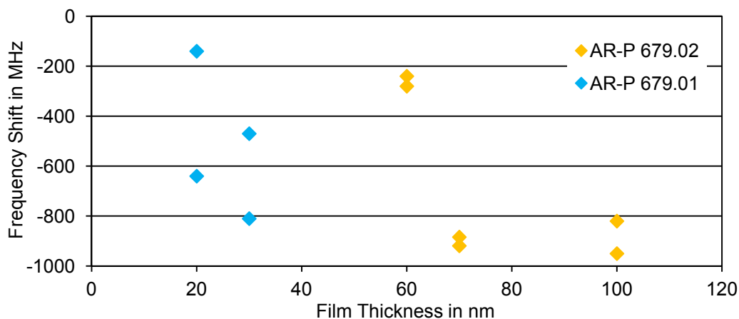
Figure 6-11: Frequency shifts of the biochip's DRF due to PMMA loading, with two measurement spots per chip / film thickness. The resonator apertures are deeper than film thickness, thus resulting in inconsistent shifts but confirming the field concentration in the undercut.
