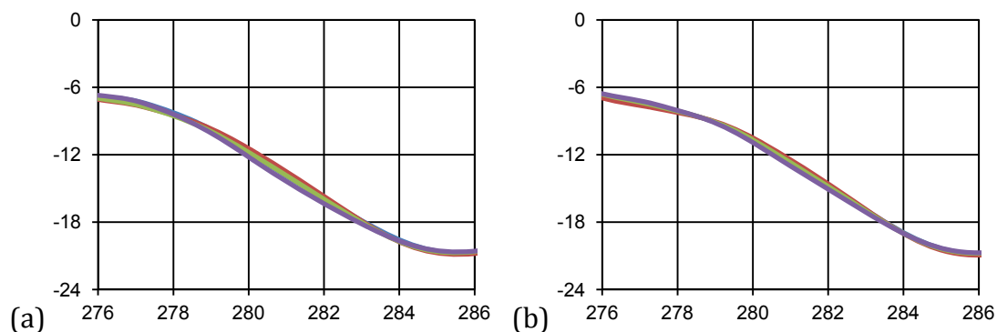
Figure 6-18: Transmission in dB over Frequency in GHz of a measurement of a biochip (a) before and (b) after DNA functionalization process with random sequence “Oligo1/2”. Spots 1 (blue) and 2 (red) are sample spots. Spots 3 (green) and 4 (violet) are references. (Chip „June 2010 series 4 B“)
