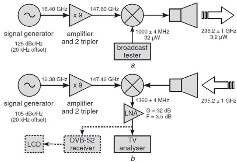
Figure 5-6 (with permission from [Jas10]): a Source and b detector of a 300 GHz digital data transmission test setup for TV broadcast. © [2010] IEEE.
