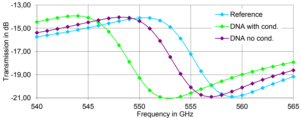
Figure 4-2: Simulated transmission of a complementary aDSR based biochip (blue) with sample material DNA as specified in Table 1, modeled with (green) and without (purple) conductivity.
