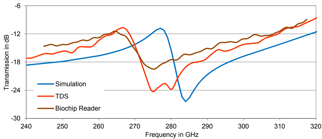
Figure 6-5: Transmission of a complementary aDSR FSS (LP) on silicon substrate. The measurements with the reader (brown) and TDS (red) deviate from the simulation (blue) due to inhomogeneous undercut etching.
