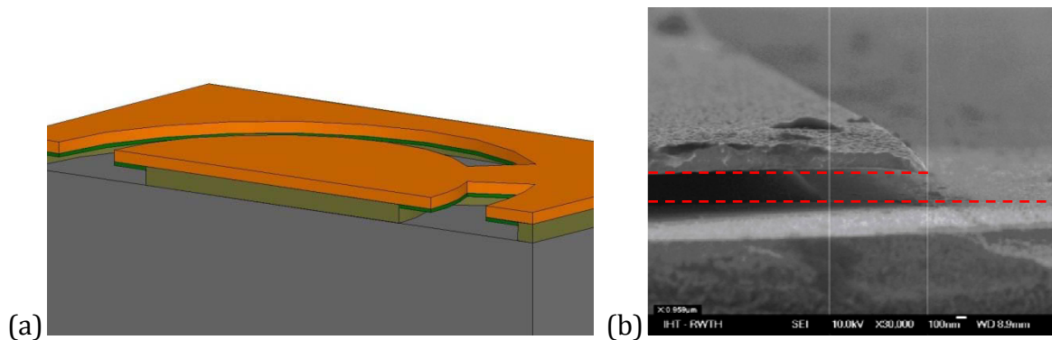
Figure 4-9: (a) [Deb09/this work] Cross-section through a complementary aDSR with undercut on silicon substrate (gray) with oxide layer ( \text{SiO}_2 , brown), metal layer (orange), and sample (green) deposited on the bottom side of the metal. (b) REM picture of the cross-section indicating a 1\ \mu\text{m} wide undercut between the vertical white lines. The red dashed lines identify the material layer interfaces.
