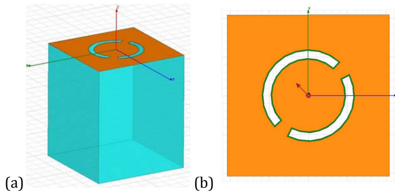
Figure 4-19: HFSS depictions of the aDSR showing (a) a 3D-model of the complementary aDSR in the gold layer (orange) on quartz-glass substrate (blue) and (b) a 2D-image from the bottom side without substrate but with sample (green). The direction of the E-field polarization is depicted in (b) by the red arrow.
