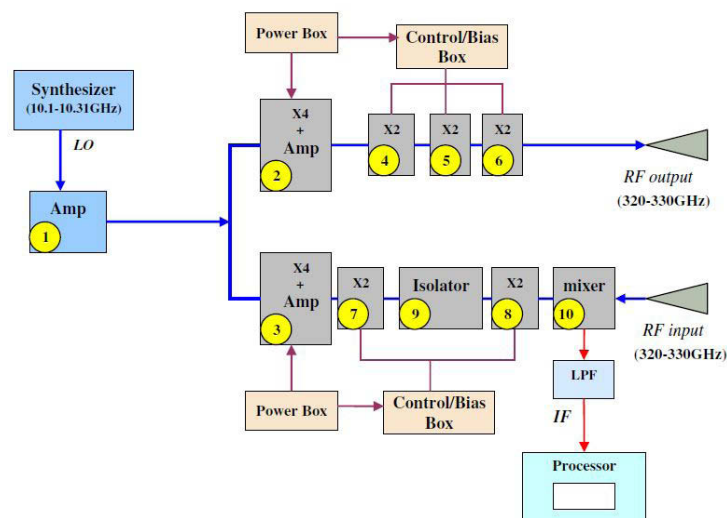
Figure 5-7 (with permission from [Kap10]): 300 GHz imaging radar with one oscillator for source and detector.
