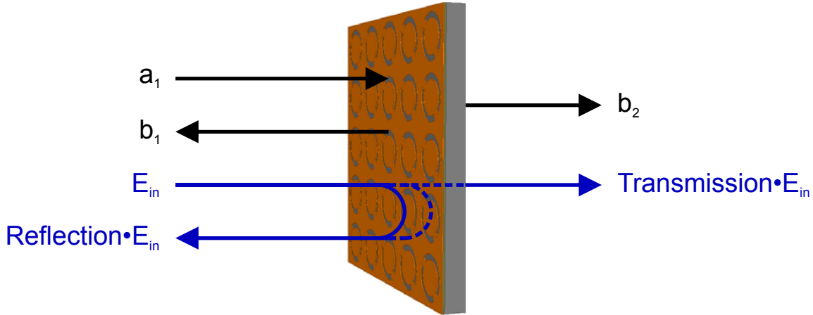
Figure 5-2: Incident ( a_1 ) and outgoing ( b_1 , b_2 ) waves of the biochip and Transmission / Reflection nomenclature for unidirectional forward measurement.
