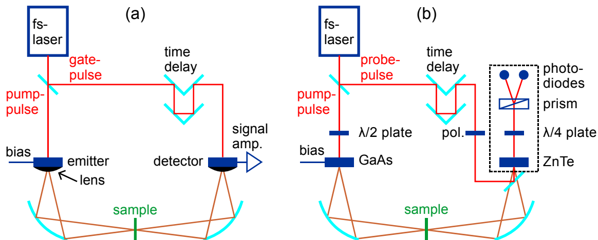
Figure 5-1 (adapted from [Sak05]): Draft of TDS setups with (a) photoconductive antennas and (b) nonlinear crystals as emitter and detector.
