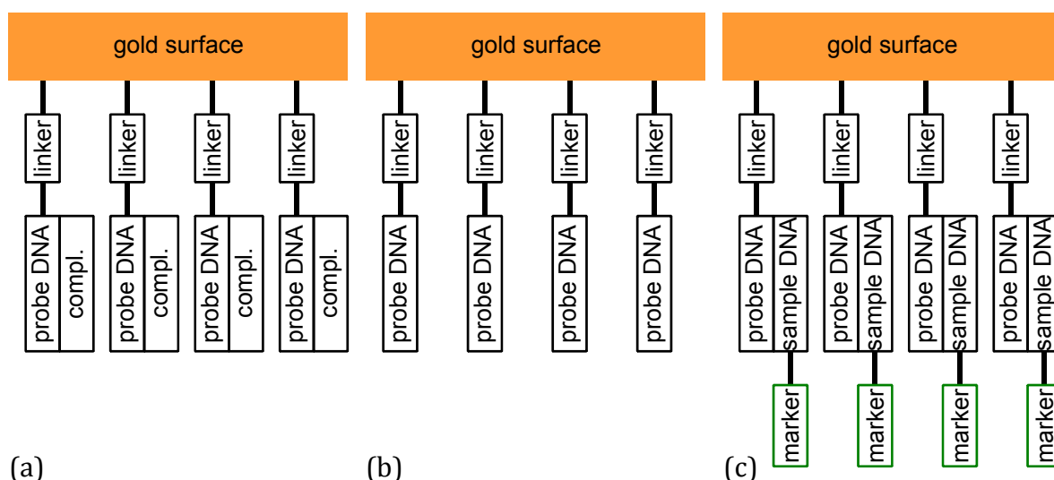
Figure 6-14: Theoretical DNA assembly with (a) immobilized double-stranded molecules linked to the gold surface, (b) single-stranded probe DNA only (functionalized) and (c) hybridized probe and sample strands with fluorescent marker linked to the sample strands.
