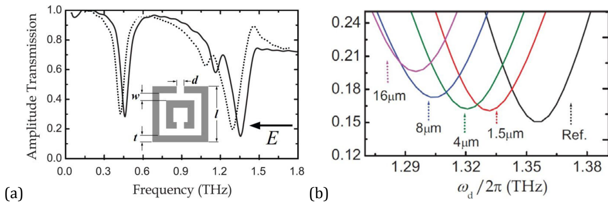
Figure 2-5 (with permission from [OHa08]): (a) Transmission of a metasurface without (solid trace) and with (dotted) 16\text{ }\mu\text{m} photoresist film. (b) Detailed view of the resonance with different film thicknesses.
