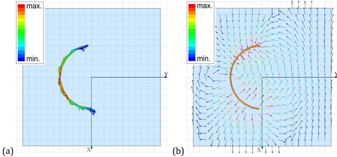
Figure 3-6: Single arc of the aDSR in resonance: (a) surface current vector and (b) electric field vector with a 90^\circ phase difference.
