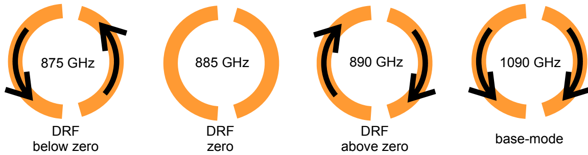
Figure 3-7: Current directions in an aDSR at the maximum (875 GHz), the zero (885 GHz), and the shoulder at the high frequency side (890 GHz) of the dual resonance feature (DRF), and at the base-mode (1090 GHz). (Excitation polarization is from top down.)
