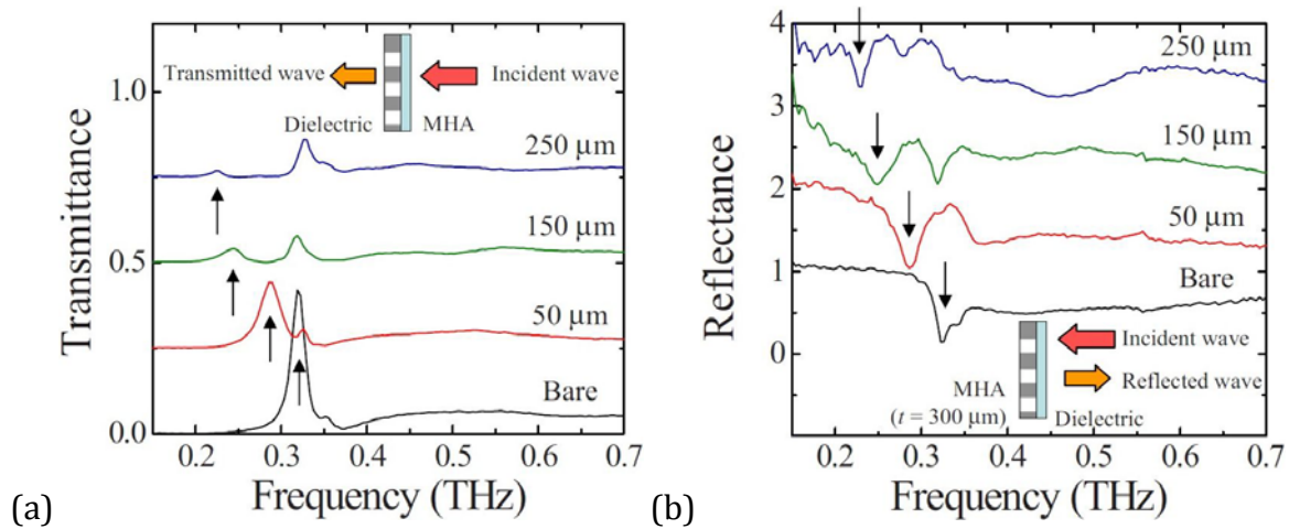
Figure 2-4 (with permission from [Miy10]): (a) Transmittance and (b) reflectance of a metal hole array (MHA) covered with PP-films of different thicknesses. The black arrows point to the MHA resonance.
