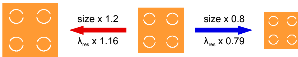
Figure 4-23: Linear rescaling of the FSS shows only little deviation of the measured resonant frequency.
