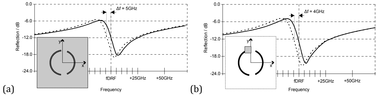
Figure 3-11:[Deb07/this work] Covering (a) the full surface with dielectric material has almost the same effect on the frequency shift as (b) localized functionalization covering only one 64 th of the surface.
