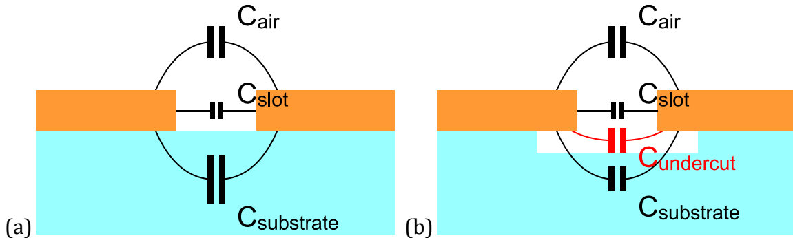
Figure 4-8: Cross-section of the gold FSS (orange) on quartz-glass substrate (blue) with capacitance distribution between arc ends (a) without and (b) with undercut.
