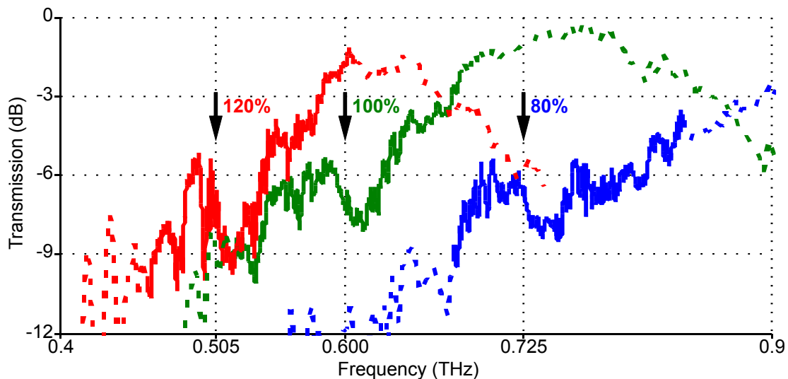
Figure 4-24: TDS measurements of the DRF for different rescaled FSSs on PET-foil with a low S/N below 500 GHz.
