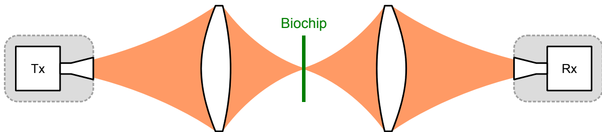
Figure 5-12: Quasi-optical THz-path in 4f-configuration with 2:1 image scale bi-convex lenses.
