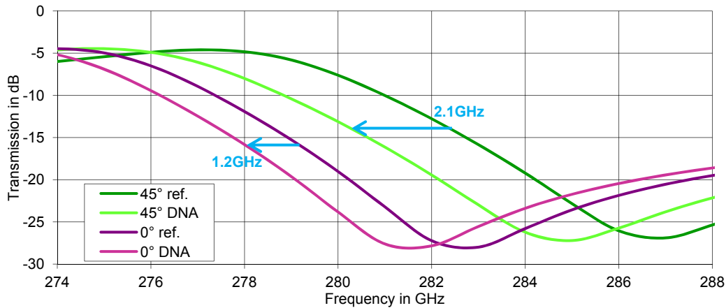
Figure 4-14: DRF of the complementary aDSR FSS with aperture orientation along (purple) and 45^\circ off (green) the grid orientation.
