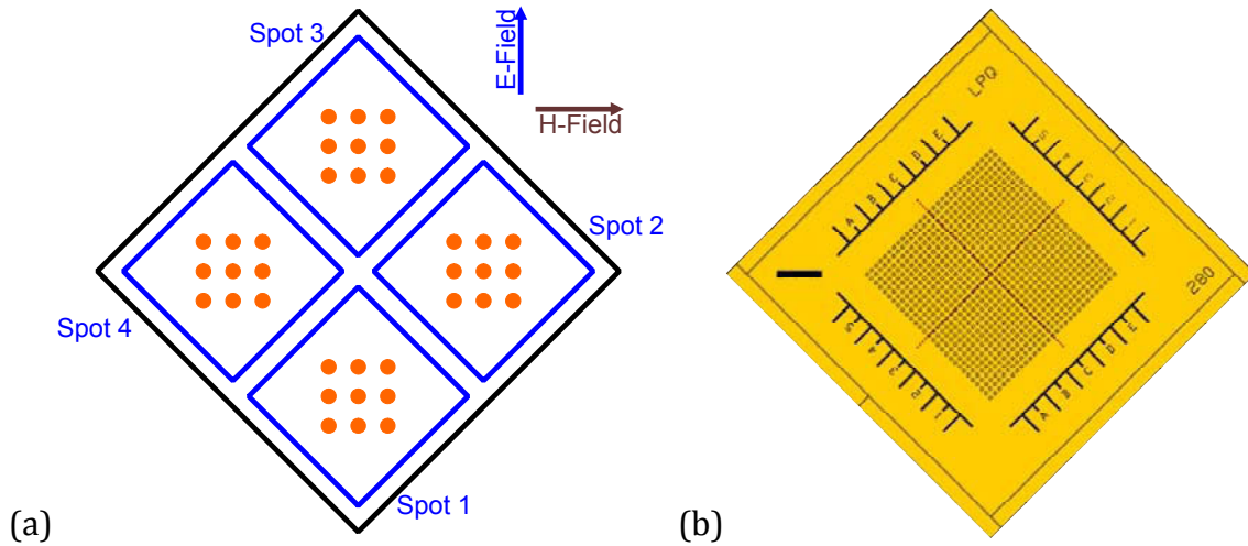
Figure 6-4: Biochip measurement design (a) including 9 measurement focuses (orange dots) per measurement spot (blue square) and (b) corresponding logical division (red lines) of the large array chip.
