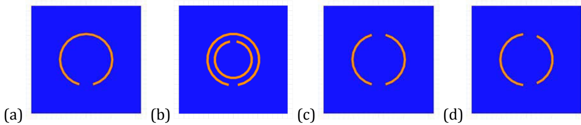
Figure 3-2: Evolution of the split-ring resonator: (a) single split-ring (SRR), (b) concentric double split-ring (dSRR), (c) symmetric double-split ring (DSR), and (d) asymmetric double-split ring (aDSR). II
