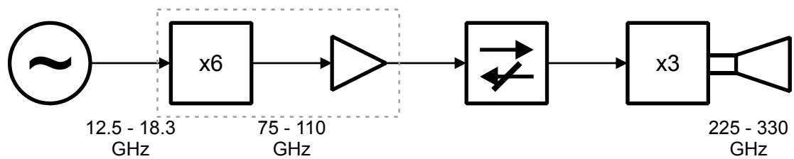
Figure 5-4: Block diagram of the biochip reader THz-source: A local oscillator generates the baseband (Ku) which is converted to the W-band by a sextupler and amplified. After an isolator a tripler generates the mm-band radiation emitted through a horn antenna.
