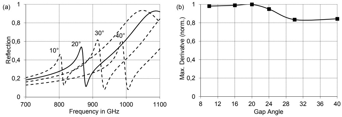
Figure 4-5: Optimization of gap angle d\phi : (a) Reflection DRF and (b) highest steepness of the DRF flank (maximum derivative -\partial R/\partial f ) for different d\phi .
