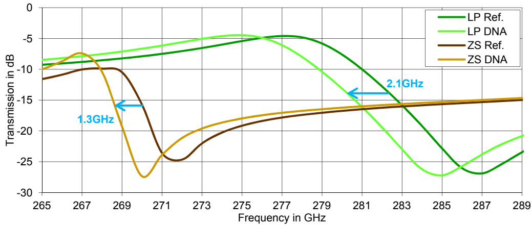
Figure 4-16: DRF of the complementary aDSR FSS with linearly polarized (green) and center-symmetric (brown) arrangement at parallel excitation ( H_{\text{par}} ).
