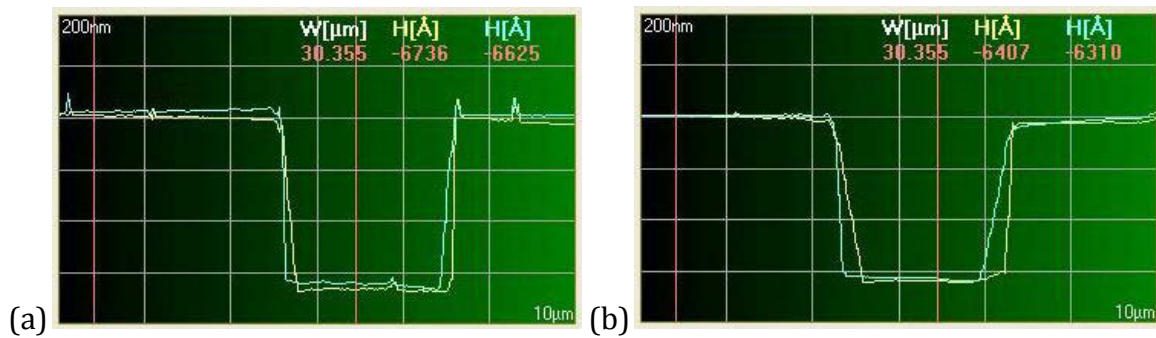
Figure 6-9 (screenshots): AFM measurements of the split-ring topology of (a) a clean chip with an average 668 nm aperture depth and (b) a chip with a 100 nm thin-film of PMMA with an average 636 nm depth.
