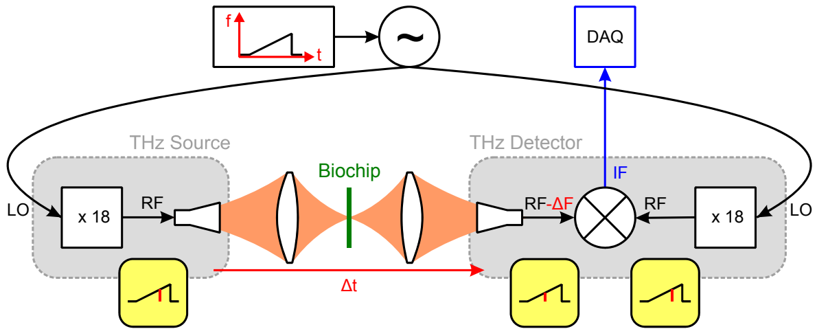
Figure 5-8: Biochip reader scheme: One LO feeds source and detector. The THz-radiation is focused on the biochip by lenses. The insets (yellow) depict the different signal runtimes allowing quasi-heterodyne detection.
