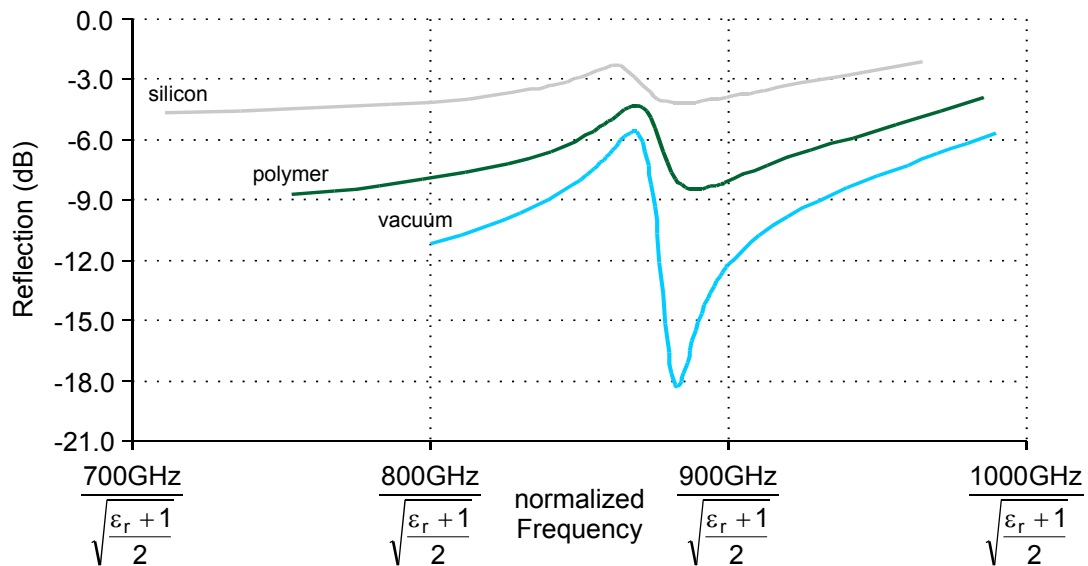
Figure 3-9:[Deb08/this work] Dual resonance feature of an aDSR based FSS on different substrates ( \epsilon_{\text{silicon}} = 11.9 , \epsilon_{\text{polymer}} = 3.2 ). Frequency is divided by the effective refractive index.
