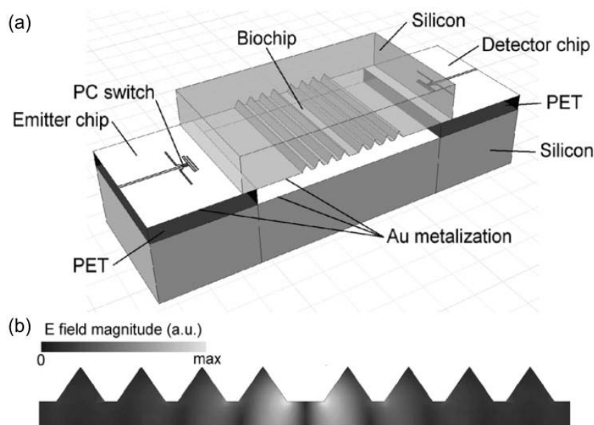
Figure 2-3 (with permission from [Nag06]): (a) Drawing of the modular setup including THz-emitter and -detector and the silicon parallel-plate waveguide (planar bottom-plate and biochip top-plate); (b) E-field distribution inside the waveguide.
