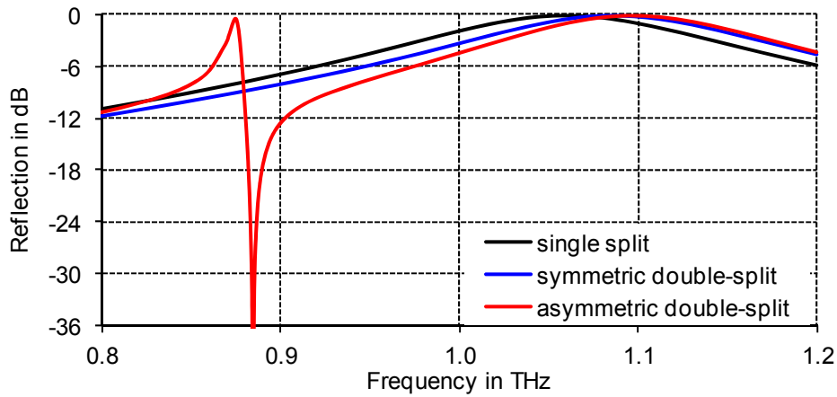
Figure 3-4: Reflection of split-ring resonator based FSSs with different types of split-ring resonators; Base-mode at 1060 GHz / 1090 GHz and dual resonance feature (DRF) at 880 GHz. (HFSS simulation, pec in vacuum)
