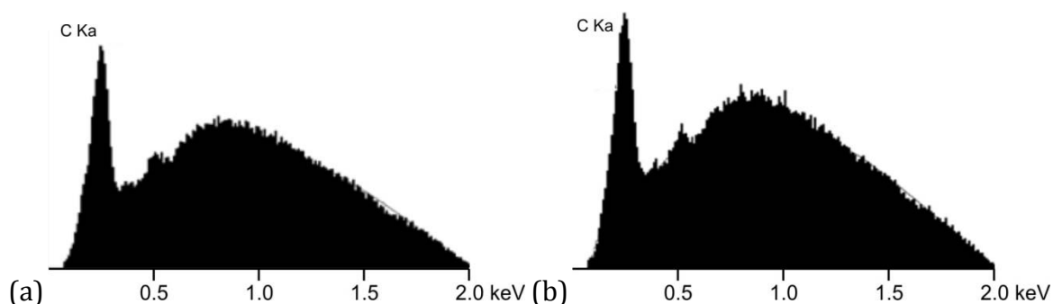
Figure 6-22: EDX spectra of a loaded biochip's (a) reference and (b) sample spot, with almost identical results. (Peaks for Au appear at higher energy levels.)
