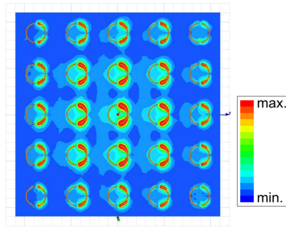
Figure 4-17: E-field distribution on the finite 5 x 5 array (1100 \mu\text{m} square) without substrate by Gaussian Beam excitation at 920 GHz with 500 \mu\text{m} beam waist (FWHM).
