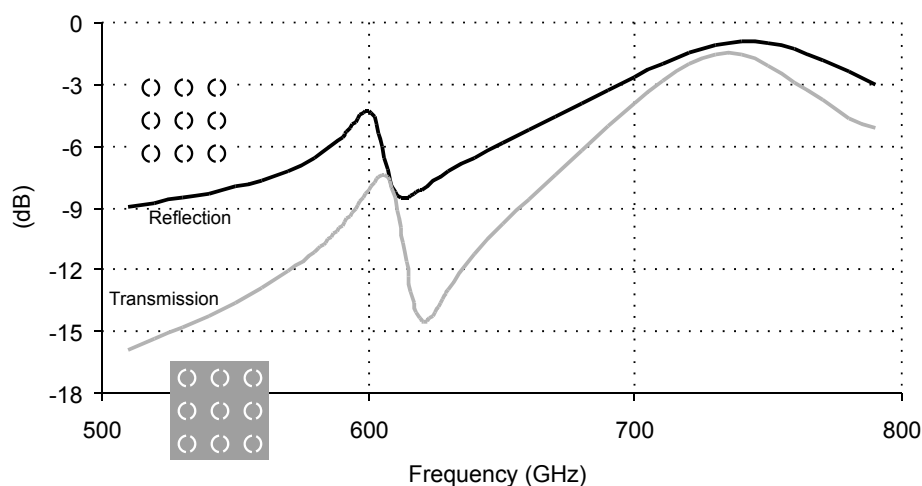
Figure 3-12:[Deb08/this work] Babinet Principle: The reflection spectrum of a FSS and the transmission spectrum of its complementary structure look the same if the polarization orientation of E- and H-field are exchanged. The deviation is due to realistic simulation parameters including finite dimensions, losses, and substrate.
