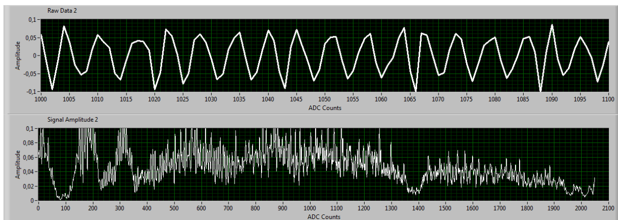
Figure 5-10 (LabView Screenshot): Intermediate frequency IF (upper trace, 100 samples) and system THz frequency response (lower trace, center 2048 samples).
