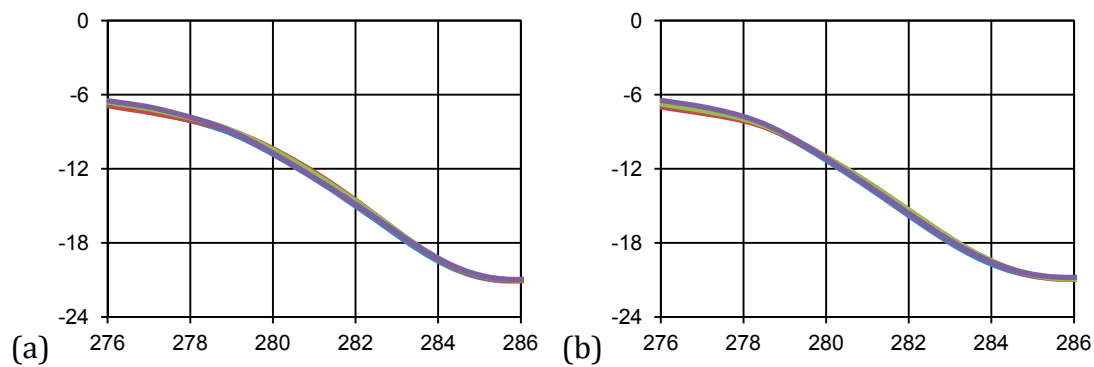
Figure 6-20: Transmission in dB over Frequency in GHz of a measurement of a biochip (a) before and (b) after DNA functionalization process with „MIA“. Spots 1 (blue) and 3 (green) are sample spots. Spots 2 (red) and 4 (violet) are references. (Chip „June 2010 series 4 C“)
