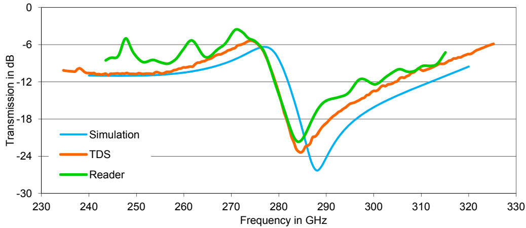
Figure 6-6: Transmission of a complementary aDSR FSS (LP) on quartz-glass substrate. The measurements with the biochip reader (green) and TDS (orange) are in excellent agreement and deviate from the simulation (blue) by less than 3 GHz only.
