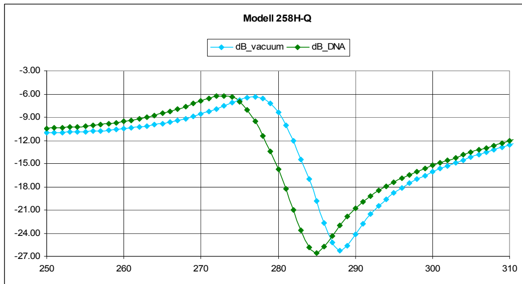
Figure 8-2: The DRF of the 280 GHz LP design shows a frequency shift of 3 GHz upon loading with DNA, corresponding to an amplitude shift of 9 dB at 283 GHz.
