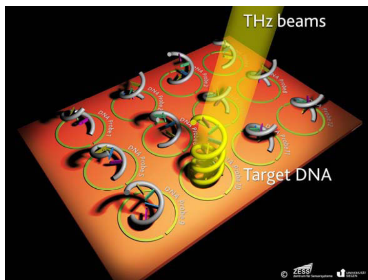
Figure 1-1: Artist's depiction of the biochip with twelve probe resonators (yellow rings), loaded with single-stranded probe DNA molecules (gray with colored nucleotides), and one hybridized probe/target DNA molecule illuminated by a THz-beam (transparent yellow).
