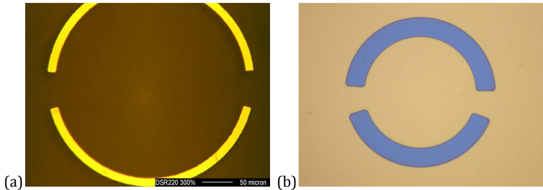
Figure 4-7: Microscopy picture of (a) an aDSR on PET- foil with 150 \mu\text{m} radius and 15 \mu\text{m} width and (b) a complementary aDSR on silicon wafer with 56 \mu\text{m} inner radius and 20 \mu\text{m} width.
