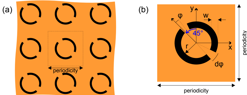
Figure 4-13: (a) Schematic section of the final version of the complementary aDSR FSS and (b) one resonator with denotation including radius r , gap offset angle \phi , gap angle d\phi and arc width w . The design is rotated counter clockwise by 45^\circ compared to the first version (Figure 4-3) and has slightly different parameters. The structures are slits (black) in a gold layer (orange) on quartz-glass.
