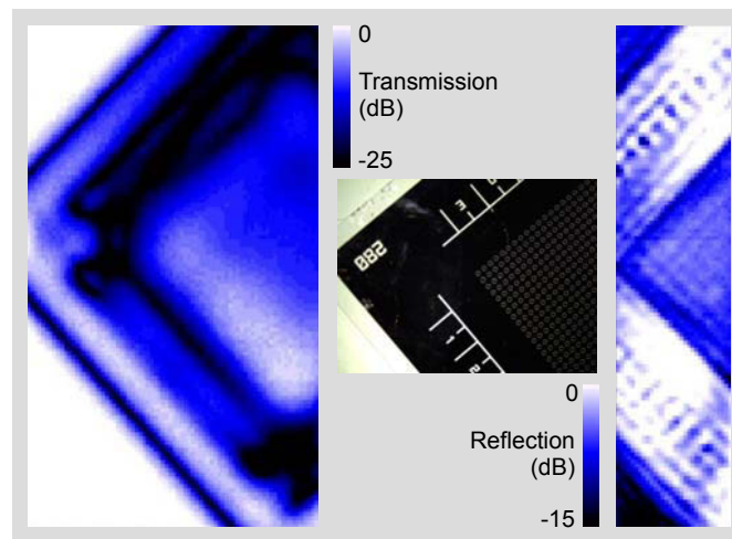
Figure 5-14: Imaging at 275 GHz in 200 \mu\text{m} steps with quasioptical transmission setup (left) and waveguide reflection setup (right); optical photo for comparison (middle), all true to scale.
