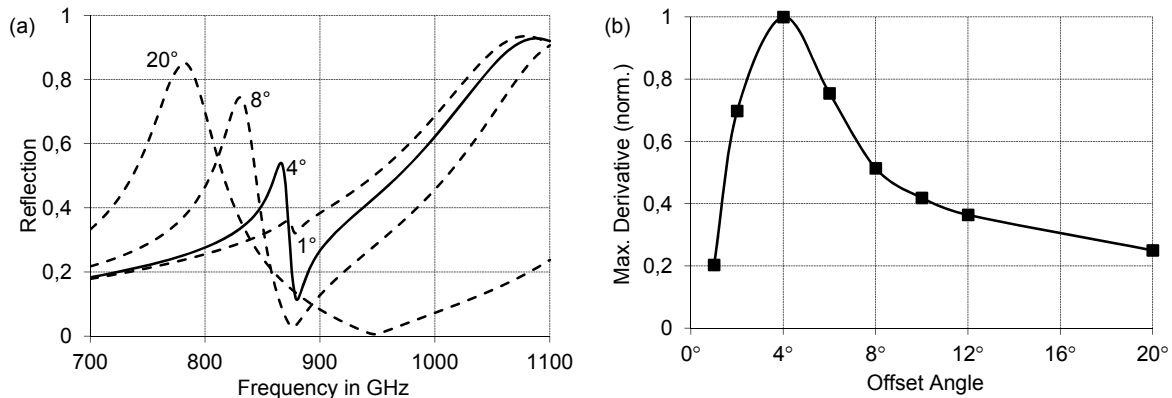
Figure 4-6:[Deb07/this work] Optimization of offset angle \phi : (a) Reflection DRF and (b) highest steepness of the DRF flank (maximum derivative -\partial R/\partial f ) for different \phi .
