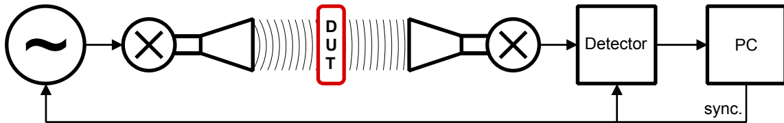
Figure 5-3: Principle of a microwave network analyzer with synchronized signal generator and detector, microwave mixers and horn antennas, and computer for control and analysis; Simplified to transmission ( S_{21} ) measurement of the device under test (DUT).
