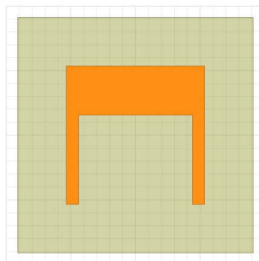
Figure 3-13: Unit cell of a LHM approach at 222 THz ( \lambda = 1350 nm): The SRR has become angular with regard to fabrication capabilities. The SRR side-length is 200 nm.
