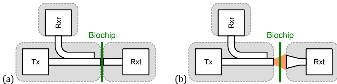
Figure 5-13: Reflection setups with a directional coupler. (a) Waveguide setup: biochip sandwiched between Tx and Rxt waveguide ends without horn antennas. (b) Hybrid setup: biochip in short distance to Tx waveguide end and Rxt with collecting horn antenna.
