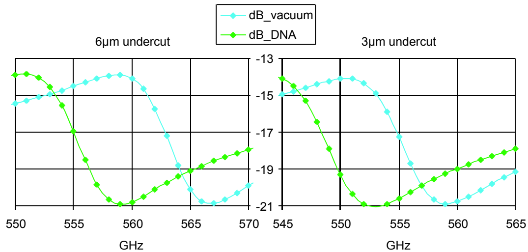
Figure 4-10:[Deb09/this work] Simulated transmission DRF in dB of complementary aDSR biochips (half size: 560 GHz version) on silicon substrate with (green) and without (blue) DNA deposited in the undercut. The frequency shift due to loading of the biochip with a 3 \mu\text{m} wide undercut is almost as large as for the 6 \mu\text{m} undercut.
