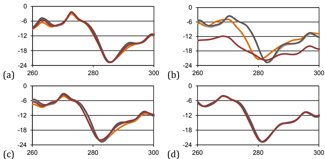
Figure 6-15: Transmission in dB over frequency in GHz of a biochip (a) after cleaning, (b) with salt crust from dried DNA buffer solution, (c) after cleaning from salt, and (d) one day later. Spots 1 (orange) and 4 (red) are loaded, spots 2 and 3 (light and dark gray) are references. The measurements approve chemical resistance to the DNA buffer solution and sensitivity to the salt in the solution and to water.
