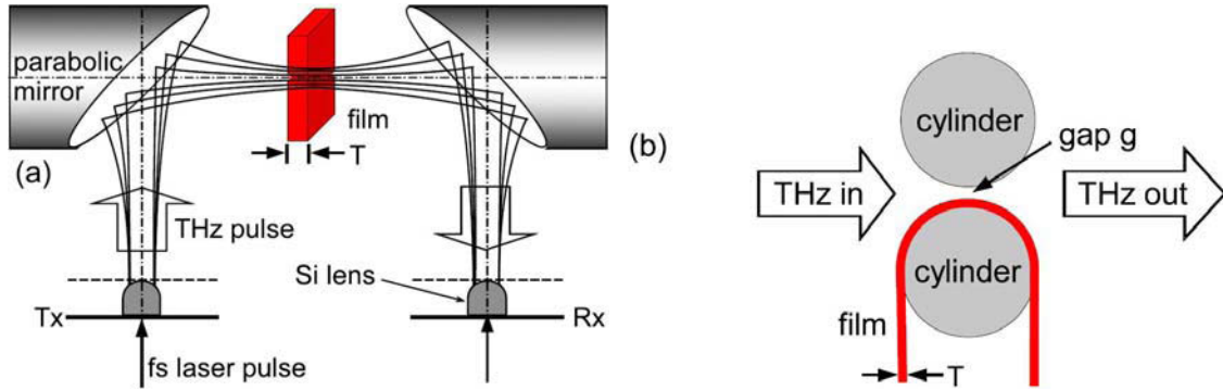
Figure 2-1 (with permission from [The10]): (a) Classical THz-TDS setup: The THz-radiation passes through the sample film one time only in orthogonal direction. (b) Passing through the gap g , more interaction between the film and the THz-radiation occurs.
