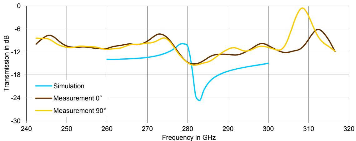
Figure 6-7: Transmission of a complementary aDSR FSS on quartz-glass substrate with center-symmetric (ZS) resonator arrangement. The measurements along and across (dark and light brown) LP-orientation agree very well, but the DRF shape differs strongly from the prediction (blue).
