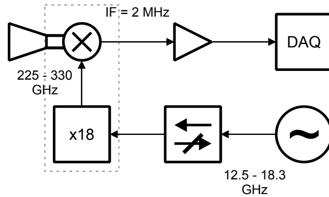
Figure 5-5: Block diagram of the biochip reader THz-detector: The 18 th harmonic of the baseband signal from the local oscillator is mixed with the received THz-radiation. The intermediate frequency (IF) is amplified and digitized. An isolator blocks baseband reflections.
