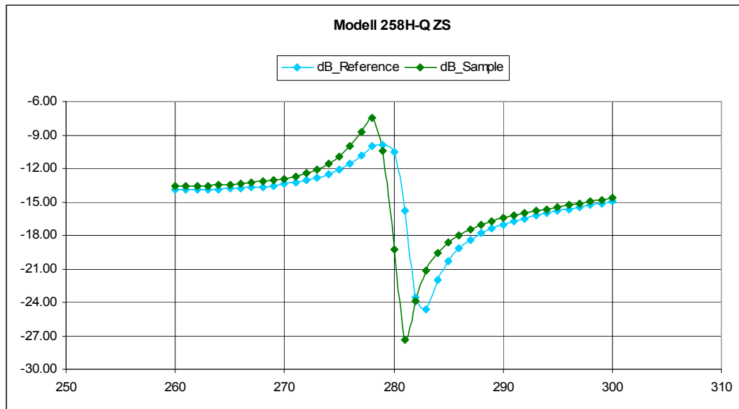
Figure 8-3: The DRF of the 280 GHz LP design shows a frequency shift of 1.5 GHz upon loading with DNA, corresponding to an amplitude shift of 10 dB at 283 GHz.
