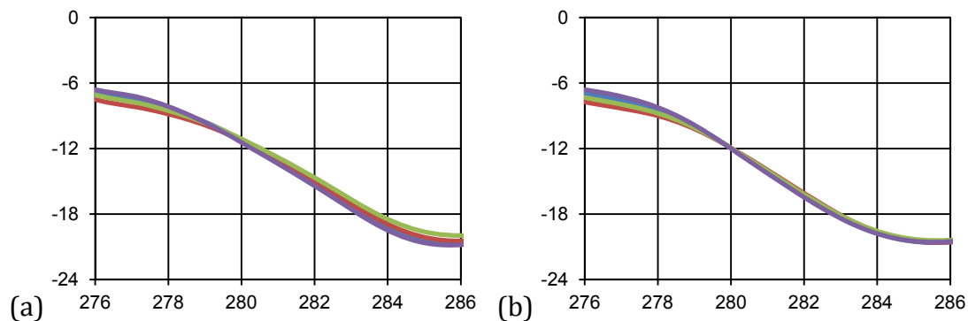
Figure 6-19: Transmission in dB over Frequency in GHz of a measurement of a biochip (a) before and (b) after DNA functionalization process with „Beta-Actin“. Spots 1 (blue) and 3 (green) are sample spots. Spots 2 (red) and 4 (violet) are references. (Chip „June 2010 series 4 A“)
