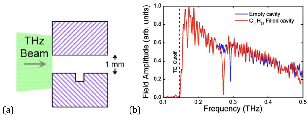
Figure 2-2 (with permission from [Men09]): (a) Sideview of the parallel-plate waveguide sensor with cavity (472 \mu\text{m} width, 412 \mu\text{m} depth) in the lower plate; (b) Frequency response of the sensor with empty and filled cavity (Undecane \text{C}_{11}\text{H}_{24} , n \approx 1.41 ).
