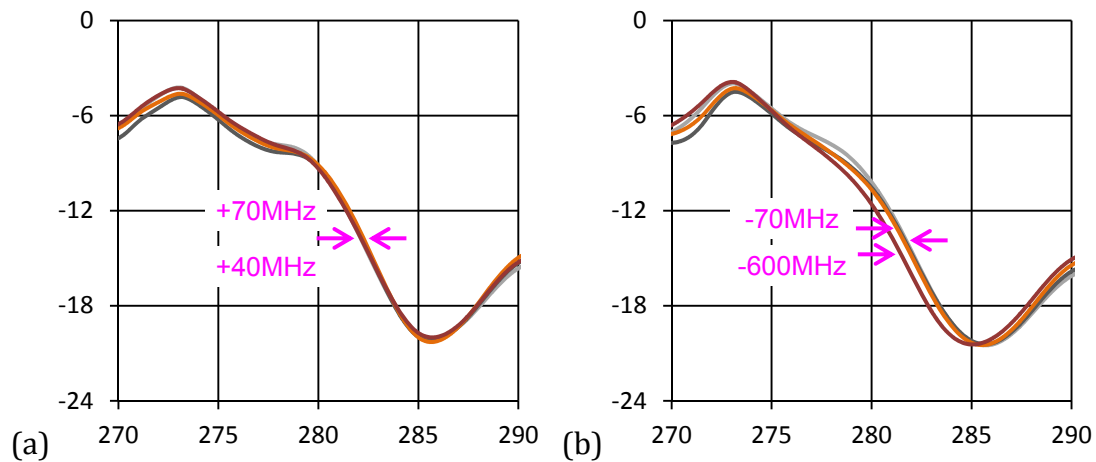
Figure 6-10: Transmission in dB over frequency in GHz of a biochip (a) clean and (b) loaded with a 20 nm thin-film of PMMA. Spots 1 and 2 (light and dark gray) are the references, spots 3 (orange) and 4 (red) are loaded. The frequency shift due to dielectric loading varies over sample spots.
