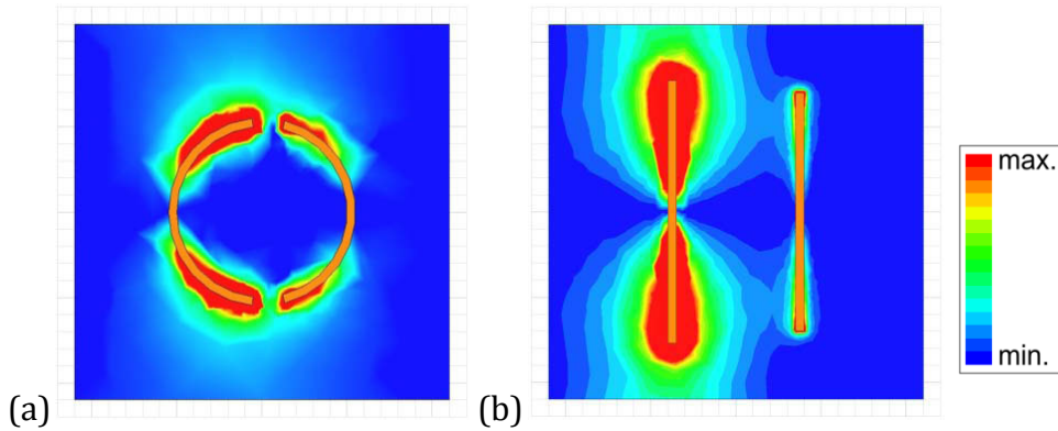
Figure 3-5: E-field magnitude of a FSS element at the maximum of the dual resonance feature of the (a) aDSR and (b) double dipole structure.
