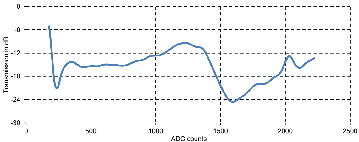
Figure 4-25: Measurement of the 600 GHz biochip with the corresponding reader. The x-axis is scaled in ADC counts, as the frequency could not be calibrated before this experiment.
