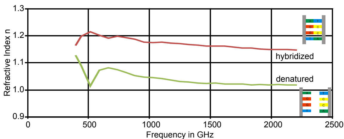
Figure 4-1 (data from [Bru00]): Real part of the refractive index of hybridized (red) and denatured (green) DNA, measured with THz-TDS.
