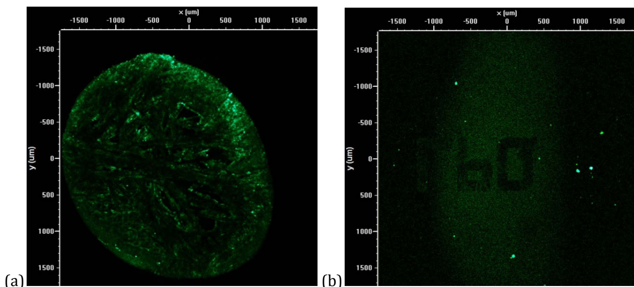
Figure 6-21: Microscope photos of a biochip from the unsuccessful experiments illuminated with 485 nm to excite the fluorescent marker at 514 nm. (a) A drying drop of DNA in solution with brightness from fluorescence at the rim. (b) After purging the chip with DI-water no marker is seen, only some artifacts from dirt particles and the weak illumination.
