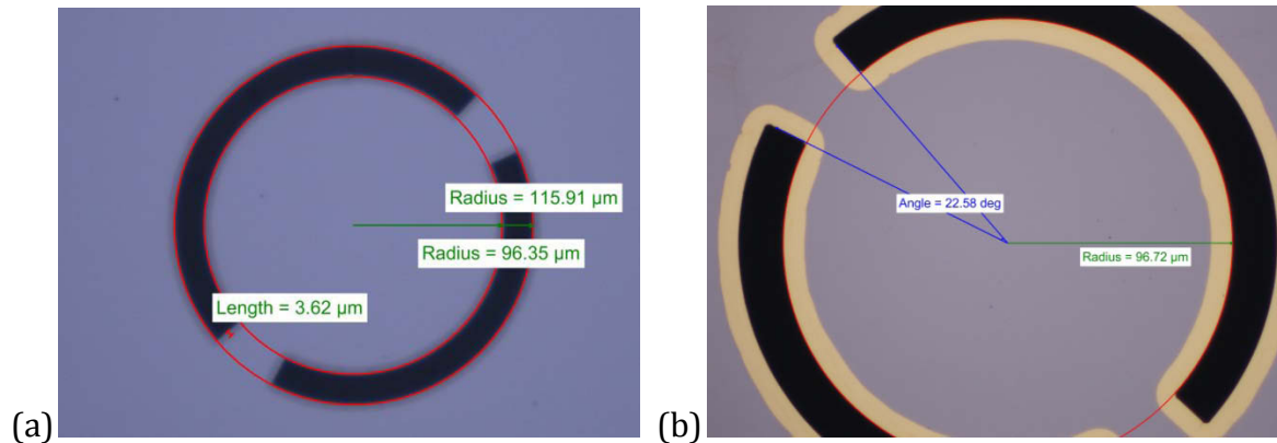
Figure 4-22: Microscope pictures of the bottom-side of an aDSR on quartz-glass with different magnifications. The measured dimensions meet the design comparably good.
