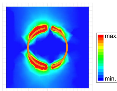
Figure 3-10: The E-Field along an aDSR at maximum reflection (875 GHz) shows a strong concentration of the field at the ends of the long arc.
