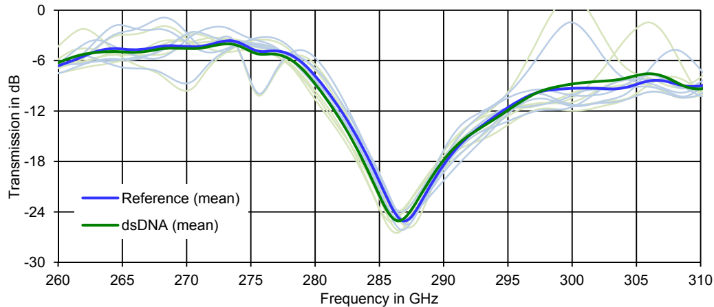
Figure 6-16: Measurements of a biochip with reference spot (blue) and sample spot with DNA loading (green). Individual measurements are in pale, means in strong color.
