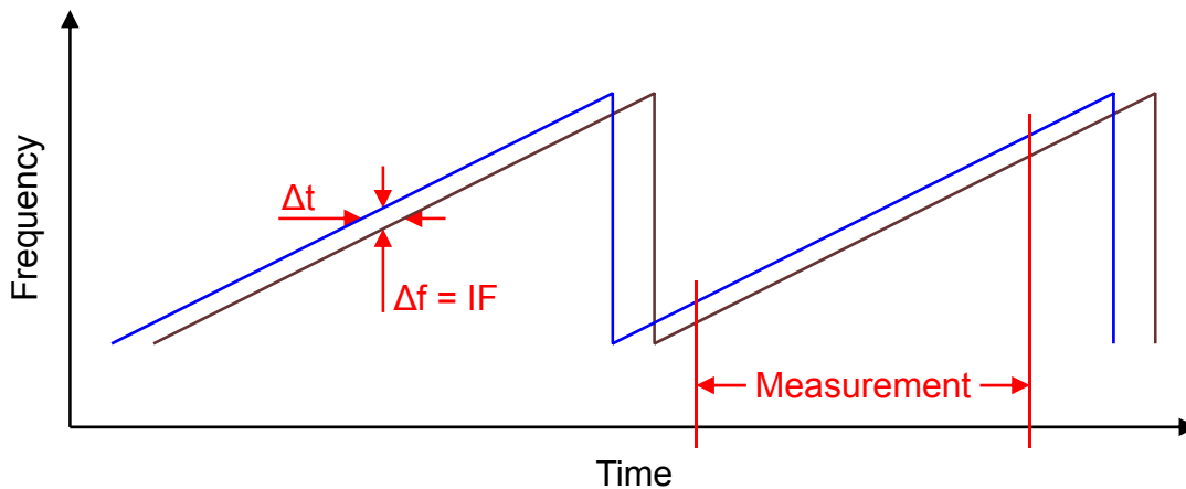
Figure 5-9: THz-frequency ramps at the receiver mixer: The received signal (brown) which travelled the quasi-optical THz-path arrives later than the reference signal (blue). Both ends of each ramp are cut off.
