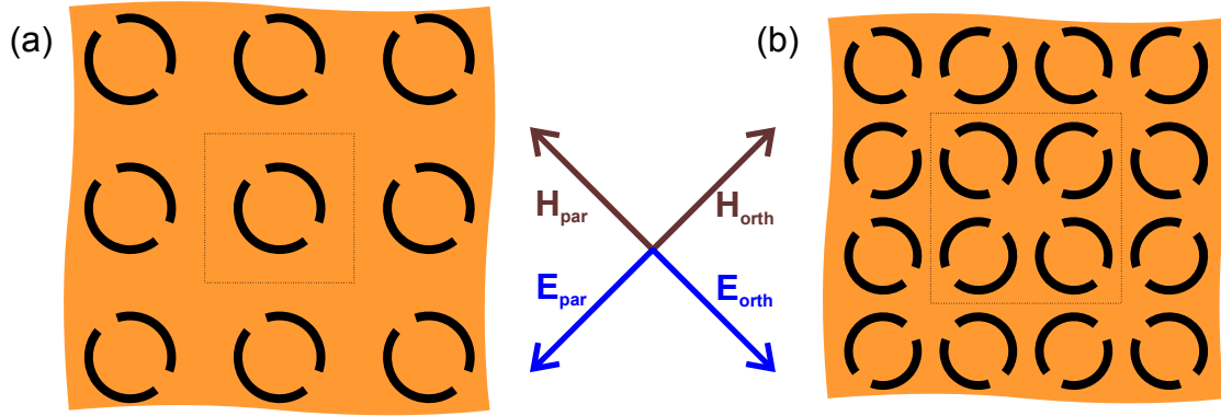
Figure 4-15: (a) Linearly polarized (LP) and (b) center-symmetric (ZS) FSS designs with polarization directions of the incident E- and H-fields (blue / brown arrows).
