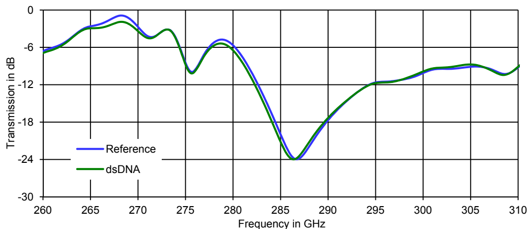
Figure 6-17: Exemplary measurement of a biochip with reference spot (blue) and sample spot with DNA loading (green).
