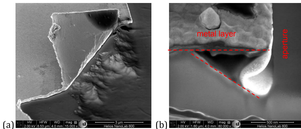
Figure 6-3: SEM-pictures of resonator details showing (a) a rough slope of the undercut sidewall and a part of the metal layer torn and bent, and (b) the cross-section of a resonator side with an almost triangular undercut and an unknown deposition (white) jamming the undercut.
