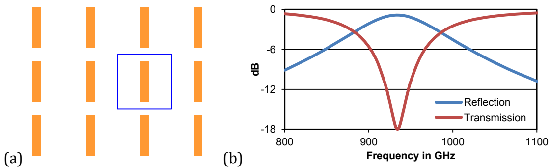
Figure 3-1: (a) FSS with 150\ \mu\text{m} long \lambda/2 -dipoles (orange) with depiction of the unit cell (blue) and (b) corresponding reflection / transmission diagram (orthogonal incidence, E-field polarized along dipoles).
