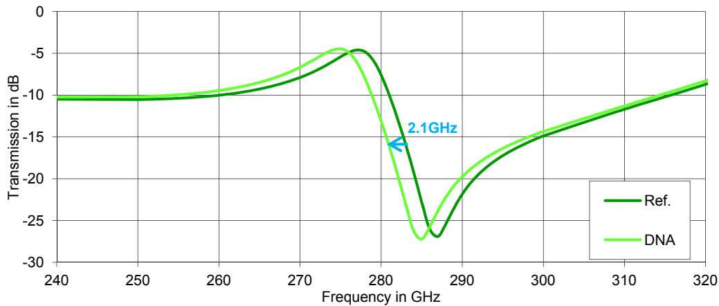
Figure 4-20: Simulated DRF of the complementary aDSR FSS without (dark green) and with (light green) DNA sample.
