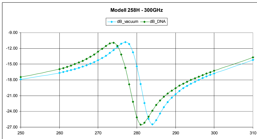
Figure 8-1: The DRF of the 280 GHz LP design shows a frequency shift of 3 GHz upon loading with DNA, corresponding to an amplitude shift of 10 dB at 280 GHz.
