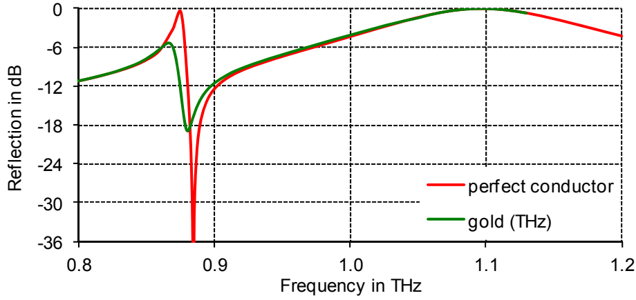
Figure 3-8: Reflection of an aDSR based FSS with the different conductor materials perfect electronic conductor (pec) and gold (with THz-parameters).
