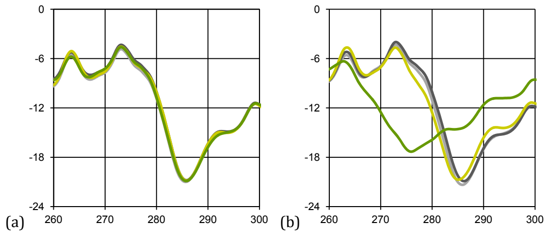
Figure 6-13: Transmission in dB over frequency in GHz of a biochip (a) clean and (b) loaded with thin-films of technical gelatin. Spots 1 and 3 (light and dark gray) are the references, spots 2 and 4 (light and dark green) are covered by a thin and a thick gelatin layer, respectively.
