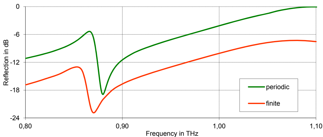
Figure 4-18: Simulated reflection spectrum of the positive aDSR FSS without substrate for the unit cell with periodic boundary conditions (green) and the finite 5 x 5 resonator array with Gaussian Beam excitation.
