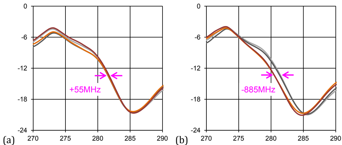
Figure 6-8: Transmission in dB over frequency in GHz of a biochip (a) clean and (b) loaded with a 100 nm thin-film of PMMA. Spots 1 and 2 (light and dark gray) are the references, spots 3 (orange) and 4 (red) are sample spots. The dielectric loading causes a frequency shift of approximately 0.9 GHz.
