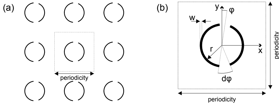
Figure 4-3:[Deb07/this work] (a) Schematic section of the first version of the aDSR FSS and (b) one resonator with denotation including radius r , gap offset angle \phi , gap angle d\phi and arc width w . The structure consists of conductive arcs (black) in vacuum.
