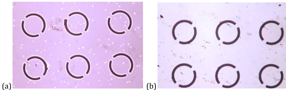
Figure 6-2: Microscope pictures of the biochip, taken from the bottom side, showing the chrome adhesive layer. (a) First set in 2010 after the chrome-etch process, showing defects in the gold layer resembling a starry sky. (b) Third set in 2010 without chrome-etch process.
