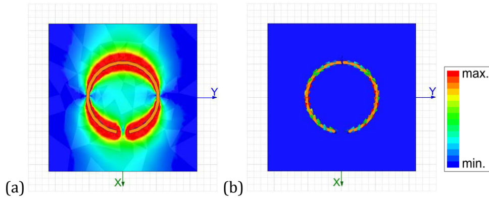
Figure 3-3: (a) E-Field magnitude and (b) surface current vector along the SRR with excitation polarization along X-axis.
