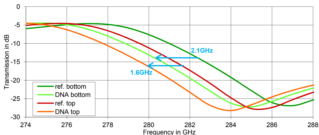
Figure 4-12: Undercut sensitivity: A DNA deposition on the bottom side (light green) of the metal shifts the reference DRF (dark green) 2.1 GHz. An identical deposition on the top side (orange) of the metal shifts the reference DRF (red) 1.6 GHz only. The references deviate due to different FEM meshes for the simulations.
