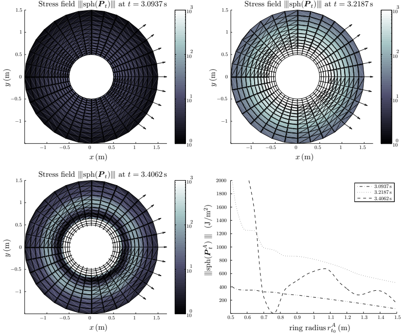
Figure 6.19. Reference configurations pertaining to three time points after the time point t^n = 2.5\text{s} where the time step size is changed from 10ms to 62.5ms. The simulation is done by the mhG(1) method with linear finite elements in time and bilinear finite elements in space. The colour indicates the spectral norm of the spherical part pertaining to the projected first Piola-Kirchhoff stress field in Joule per square meter. The vector arrows at the spatial nodes designate the projected Piola-Kirchhoff heat flux. On the ordinate of the plot in the bottom right corner, the stress norm pertaining to nodes A on a radial line is indicated, which ends at a node on the outside of the ring opposite the uninsulated portion. The corresponding radial positions in the reference configuration at time t_0 = 0 are shown on the abscissa.
