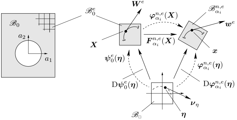
Figure 4.2. The reference configuration \mathcal{B}_0 is partitioned into disjoint sub-domains \mathcal{B}_0^e . A parent domain \mathcal{B}_\square is mapped on each sub-domain in the reference configuration and on the corresponding sub-domain \mathcal{B}_{\alpha_i}^{n,e} in the current configuration.
