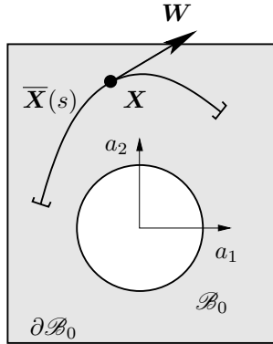
Figure 2.2. A curve \overline{\mathbf{X}}(s) through any point \mathbf{X} in the reference configuration \mathcal{B}_0 and a tangent vector \mathbf{W} \in T_{\mathbf{X}}\mathcal{B}_0 in the corresponding tangent space at this curve.
