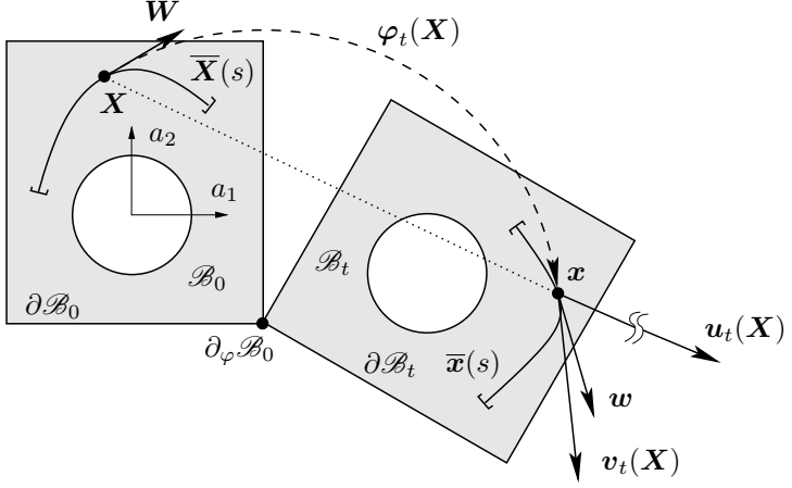
Figure 2.3. The current configuration \mathcal{B}_t with the curve \bar{\mathbf{x}}(s) through the point \mathbf{x} \in \mathcal{B}_t and the corresponding tangent vector \mathbf{w} \in T_{\mathbf{x}}\mathcal{B}_t . Further elements of this tangent space are the deformation velocity \mathbf{v}_t(\mathbf{X}) as tangent vector at the motion \varphi(t) and the displacement vector \mathbf{u}_t(\mathbf{X}) as tangent vector at the displacement curve.
