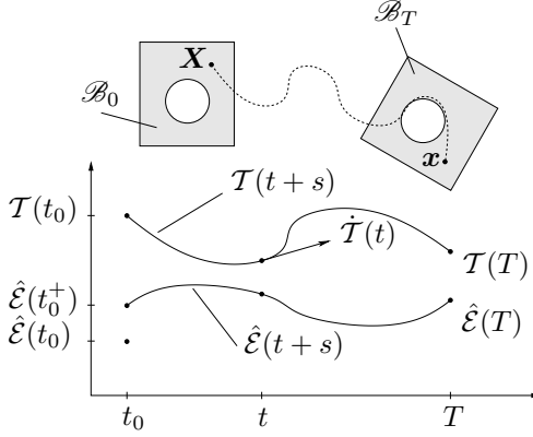
Figure 3.1. The continuous curve T(t+s) connects the kinetic energy T(t_0) of the reference configuration \mathcal{B}_0 with the kinetic energy T(T) of the final configuration \mathcal{B}_T . However, the lower bound of the continuous relative internal energy curve \hat{E}(t+s) does not coincide with the energy \hat{E}(t_0) of the reference configuration.
