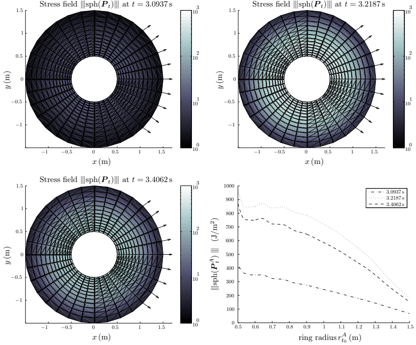
Figure 6.22. The first three plots show reference configurations pertaining to three time points after the change of the time step at time t^n = 2.5 s from the size 10 ms to 62.5 ms. The simulation is done by the ehG(1) method with linear finite elements in time and bilinear finite elements in space. The colour indicates the spectral norm of the spherical part pertaining to the projected first Piola-Kirchhoff stress field in Joule per square meter. The vector arrows at the spatial nodes designate the projected Piola-Kirchhoff heat flux. The plot in the bottom right corner shows the stress norm pertaining to nodes A on a radial line which ends at a node on the outside of the ring opposite the uninsulated portion. The radial positions of these nodes in the reference configuration at time t_0 = 0 are shown on the abscissa.
