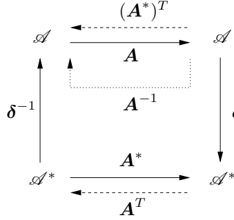
Figure 2.1. A linear mapping \mathbf{A} between two vectors in the ambient space \mathcal{A} possesses an inverse \mathbf{A}^{-1} , and a transpose \mathbf{A}^T as well as a dual mapping \mathbf{A}^* on the dual ambient space \mathcal{A}^* .
