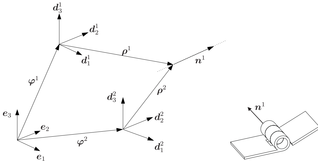
Figure 4.3.: Revolute pair
