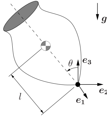
Figure 5.1.: Symmetrical top
