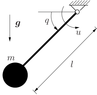
Figure 8.1.: Mathematical pendulum
