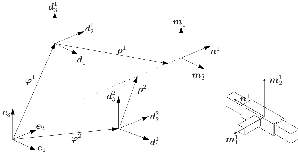
Figure 4.5.: Prismatic pair
