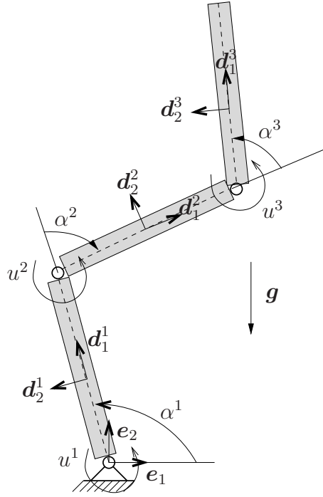
Figure 6.1.: 3-link manipulator
