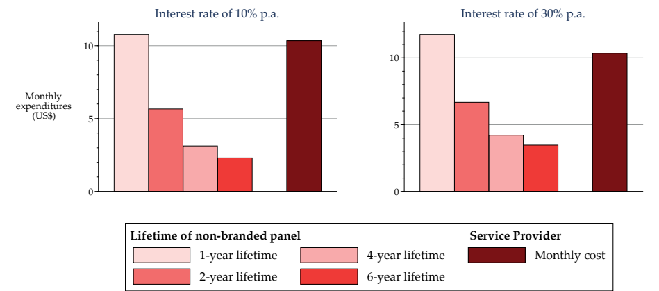
Figure 5: Cost comparison between non-branded and branded SHSs
