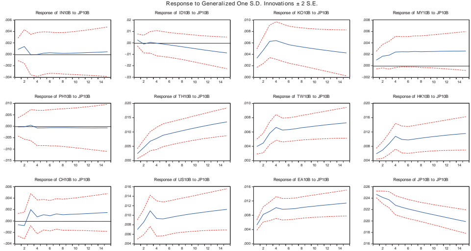
Figure 7: Generalized impulse responses to shocks emanating from Japan
