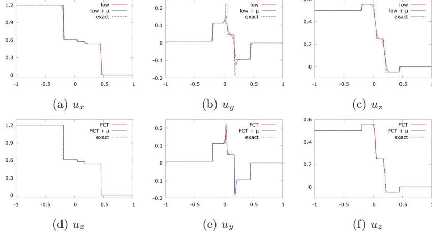
Figure 3: Numerical solutions of the Ryu-Jones problem using the viscosity operator (14) and its scaled version " +\mu " (20) at T_{end} = 0.2 ( h = \frac{1}{512} )
