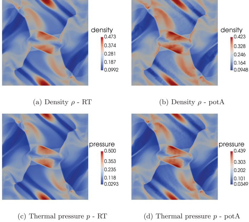
Figure 6: Numerical solutions of the Orszag-Tang vortex problem at T_{end} = 0.5 ( h = \frac{1}{200} ) using different divergence cleaning approaches
