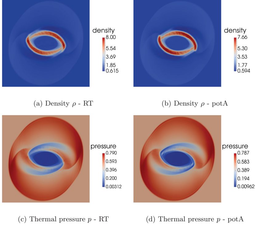
Figure 4: Numerical solutions of the rotor problem at T_{end} = 0.295 ( h = \frac{1}{200} ) using different divergences cleaning approaches
