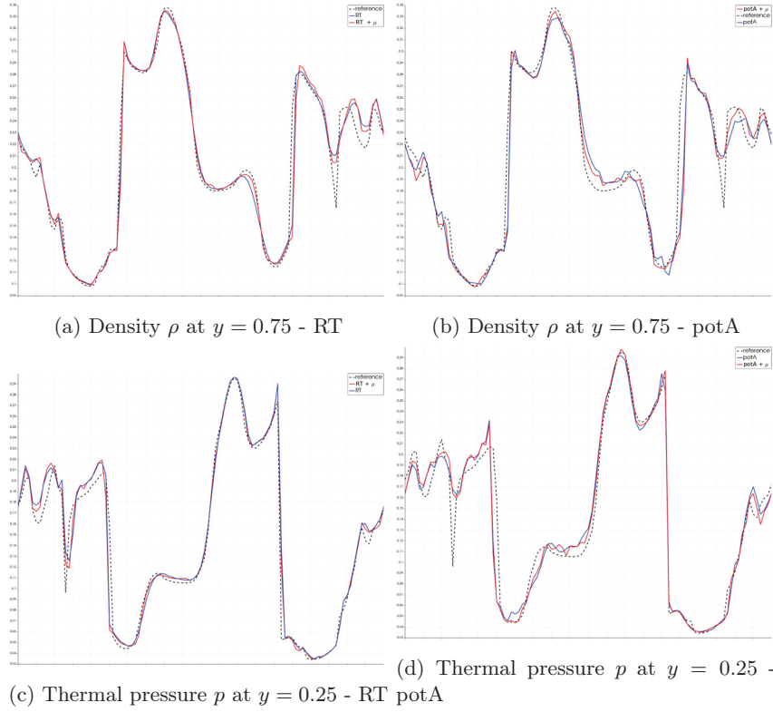
Figure 7: Comparison of the numerical solutions of the Orszag-Tang vortex problem at T_{end} = 0.5 ( h = \frac{1}{200} ) using the viscosity operator (14) and its scaled version "+ \mu " (20)
