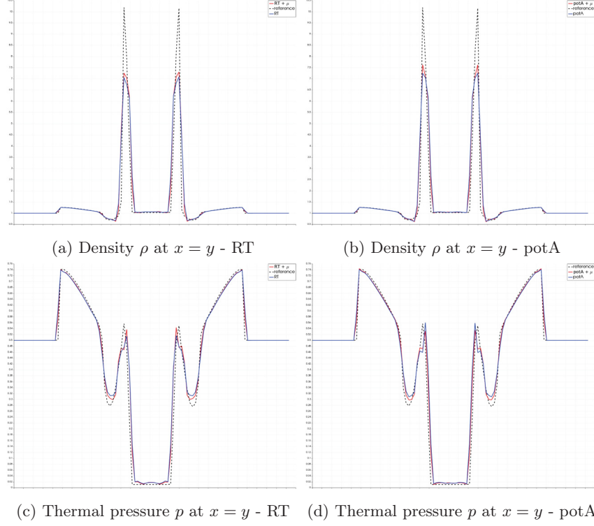
Figure 5: Comparison of the numerical solutions of the rotor problem at T_{end} = 0.295 ( h = \frac{1}{200} ) using the viscosity operator (14) and its scaled version "+ \mu " (20)
