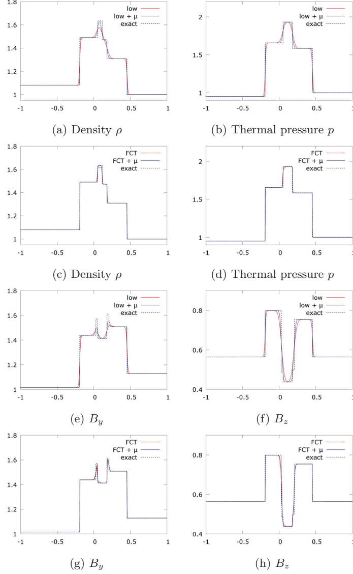
Figure 2: Numerical solutions of the Ryu-Jones problem using the viscosity operator (14) and its scaled version "+μ" (20) at T_{end} = 0.2 ( h = \frac{1}{512} )
