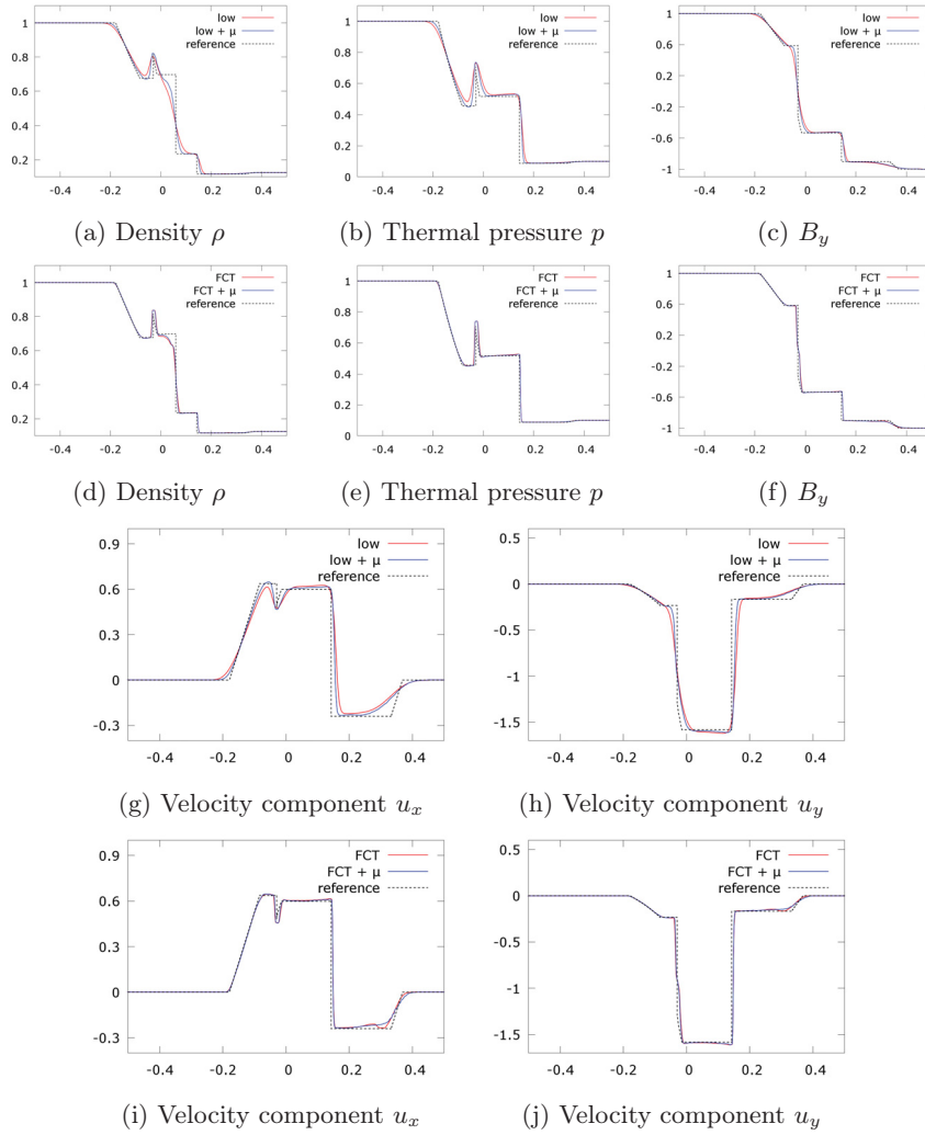
Figure 1: Numerical solutions of the Brio-Wu problem using the viscosity operator (14) and its scaled version "+ \mu " (20) at T_{end} = 0.1 ( h = \frac{1}{512} )
