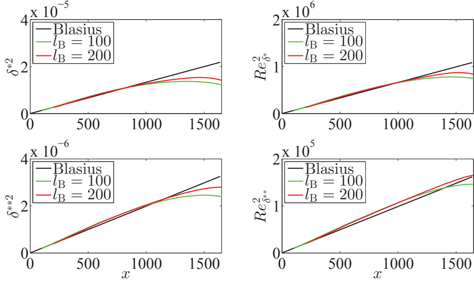
Figure 12: The dependencies on x of squares of the displacement thickness \delta^* and the momentum loss thickness \delta^{**} ( left ). The dependencies on x of corresponding squares of the Reynolds numbers Re_{\delta^*} and Re_{\delta^{**}} ( right ).
