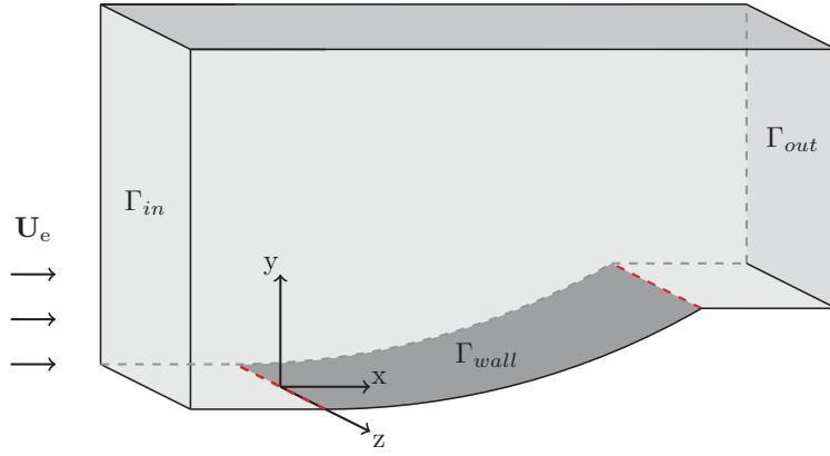
Figure 8: The computational domain with two buffer zones.
