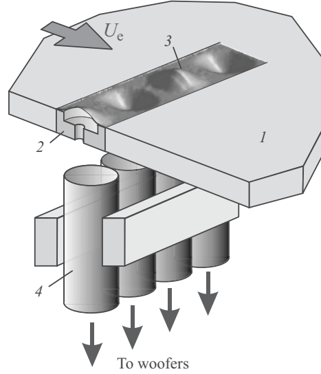
Figure 2: Disturbance source [2]: concave surface (1); insert (2); elastic membranes (3); pneumatic lines (4).
