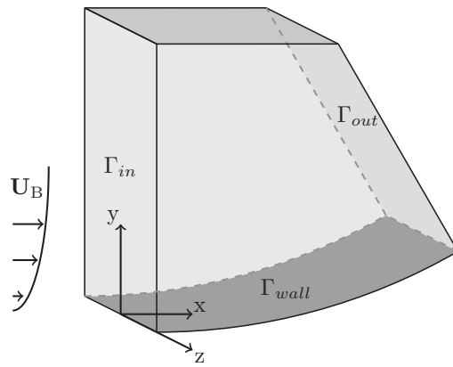
Figure 9: The computational domain without buffer zones.
