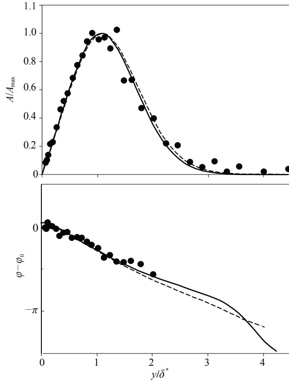
Figure 5: Amplitude ( top ) and phase ( bottom ) profiles obtained experimentally [2] ( \bullet ) for \lambda_z = 12 mm f = 8 Hz at x = 1200 mm in comparison with the results of computations using linear theory of hydrodynamic stability with account for (—) and dropping (---) the terms containing the velocity of the base flow normal to the surface V and streamwise derivatives of the streamwise velocity of the base flow U (see details in [11]).
