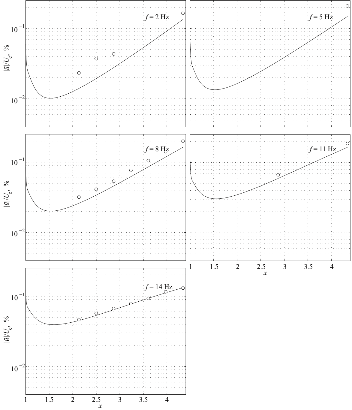
Figure 7: Computed (—) and measured (o) amplification curves for amplitudes of the streamwise disturbance velocity at wall-normal distances corresponding to U/U_e = 0.6 for \lambda_z = 12 mm.
