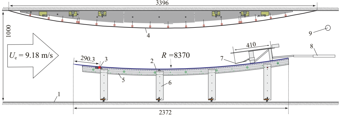
Figure 1: Experimental setup [2]: wall of working part of the wind-tunnel (1); concave plate (2); the insert for disturbance sources (3); adjustable wall bump (4); rigid frame made of fixed-radius ribs (5); supports (6); hot-wire probe with traversing mechanism (7); traversing mechanism handle (8); flow-blockage adjuster (9).
