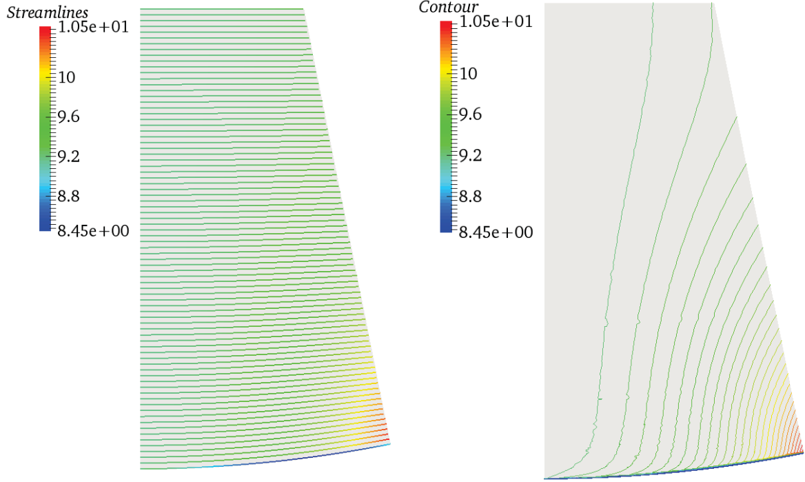
Figure 10: Streamlines ( left ), contour lines ( right ).
