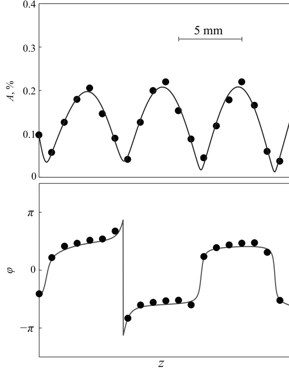
Figure 4: Amplitudes ( top ) and phases ( bottom ) of disturbances in z for \lambda_z = 12 mm and f = 8 Hz at x = 1200 mm): experimental data ( \bullet ) and their approximation by a 10th-order polynomial ( — ) [2].
