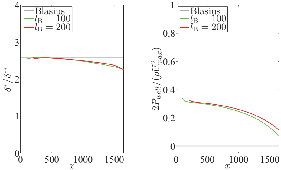
Figure 13: The ratio of the displacement thickness and the momentum loss thickness ( left ). Dimensionless pressure ( right ).
