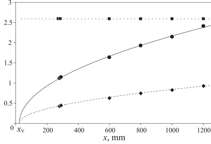
Figure 3: Comparison of integral boundary-layer characteristics. Experimental data [2]: \delta^* , mm (●); \delta^{**} , mm (◆); \delta^*/\delta^{**} (■); numerical data for Blasius boundary layer (—), (---), (···), respectively; the effective origin of the Blasius boundary-layer x_v = 21.6 mm.
