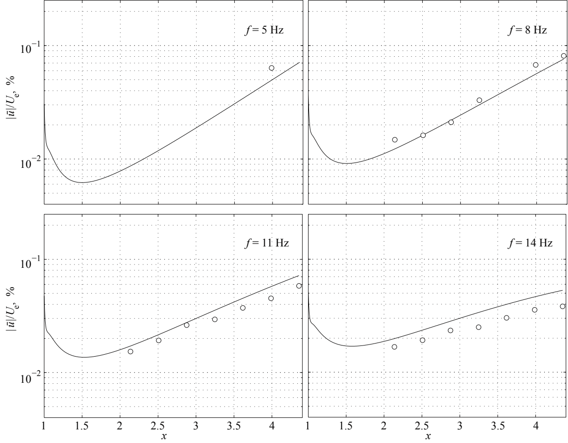
Figure 6: Computed (—) and measured ( \circ ) amplification curves for amplitudes of the streamwise disturbance velocity at wall-normal distances corresponding to U/U_e = 0.6 for \lambda_z = 8 mm.
