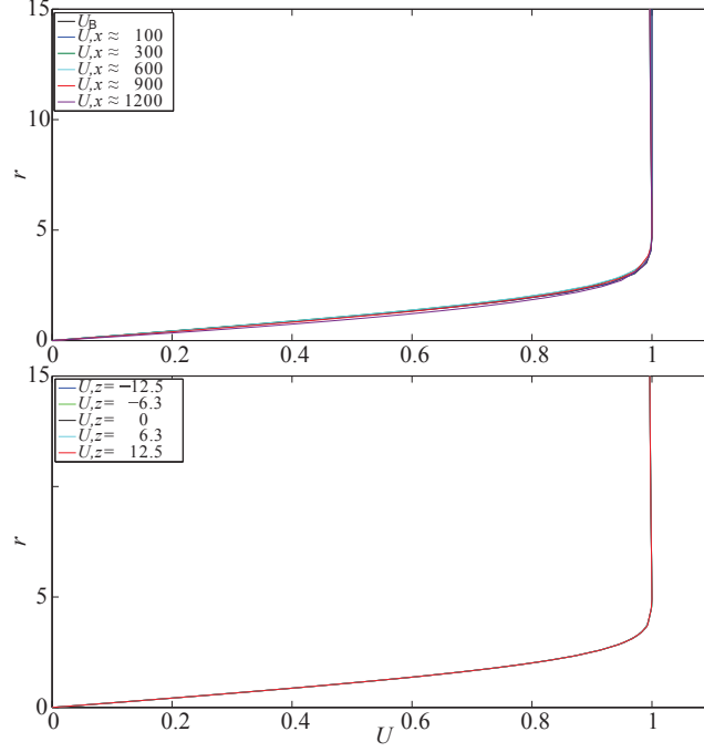
Figure 11: The dependencies of the streamwise component U on r at: different coordinates x , mm for z = 0 ( top ) and x \approx 700 mm and different z , mm ( bottom ).
