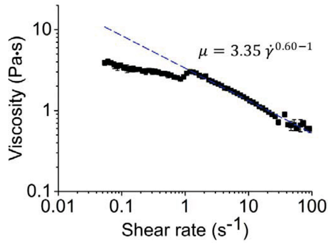
Fig S9. Apparent dynamic viscosity of the shear thinning fluid. Power law model (dotted line) is used to fit the data in the shear rate range of 1~100 s -1 . The error bars represent standard deviations.
