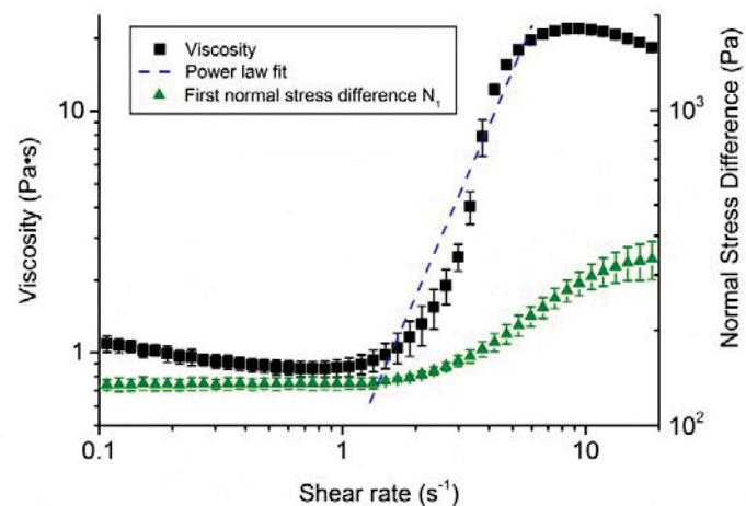
Fig S7. Apparent dynamic viscosity of the shear thickening fluid. Power law model (dotted line) is used to fit the viscosity (black squares) in the shear rate range of 1.5\sim6\text{ s}^{-1} . The change of first normal stress difference N_1 of our shear thickening medium is two orders of magnitude smaller than the Boger fluid used in 8 . Thus, the viscosity change is dominant during the swimming process. The error bars represent standard deviations.
