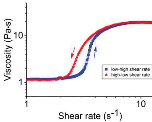
Fig S10. Hysteresis of viscosity of the shear thickening fluid. When the shear rate increases from a low viscosity (blue squares), the transition occurs at a higher critical shear rate, while when the shear rate decreases from a high viscosity (red triangles), the transition takes place at a lower shear rate. The error bars represent standard deviations.
