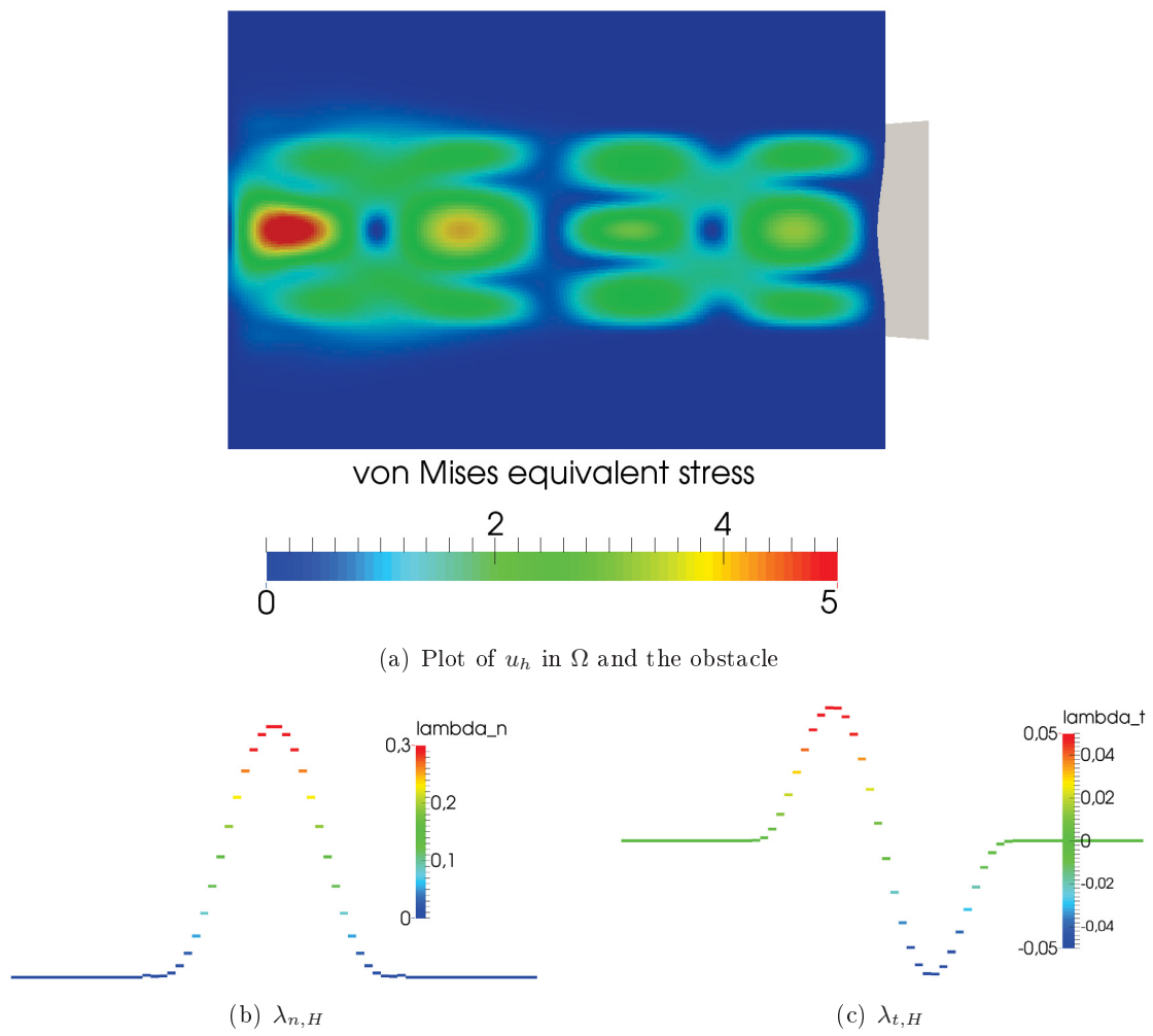
Fig. 4: Numerical solution of the first example for M_\Omega = 24576 and M_C = 64
