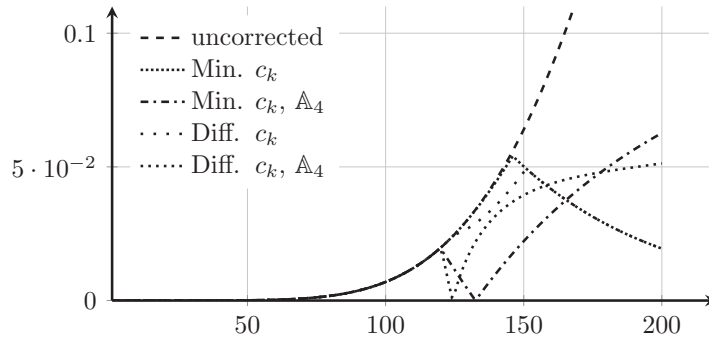
Figure 7: Euclidean error norm of the second order orientation tensor A_2 of the planar elongational flow with a Fourier approximation of order N_p = 6 depending on the time.
