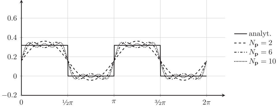
Figure 1: Demonstration of the Gibbs phenomenon for different orders N_p .
