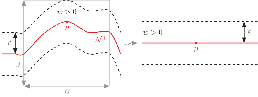
FIG. 5.2. Local rectification of the set \mathcal{N}^+ in two dimensions.
