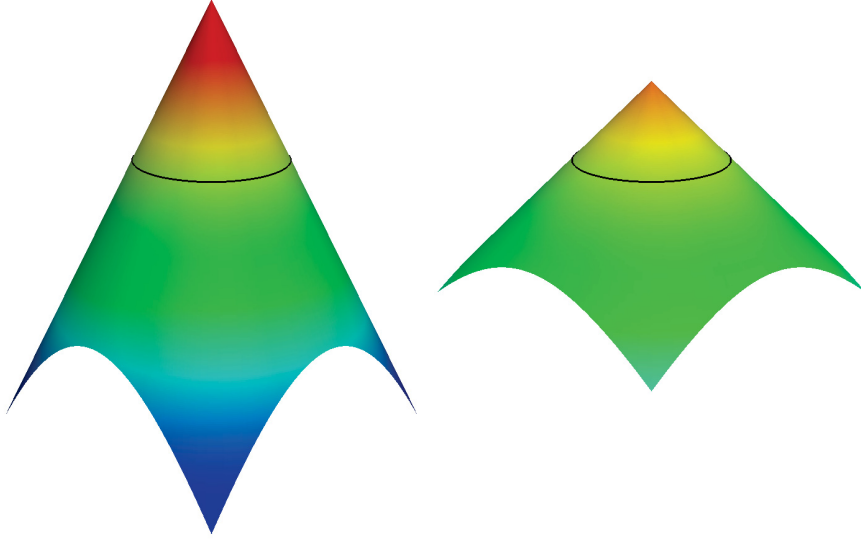
Figure 4. Circular interface: initial condition (left) and the level set function after reinitialization (right)
