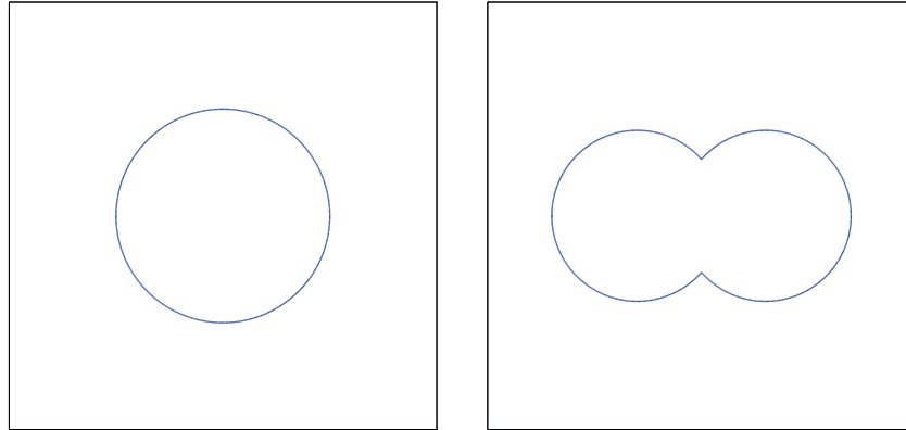
Figure 3. Test case interface shapes
