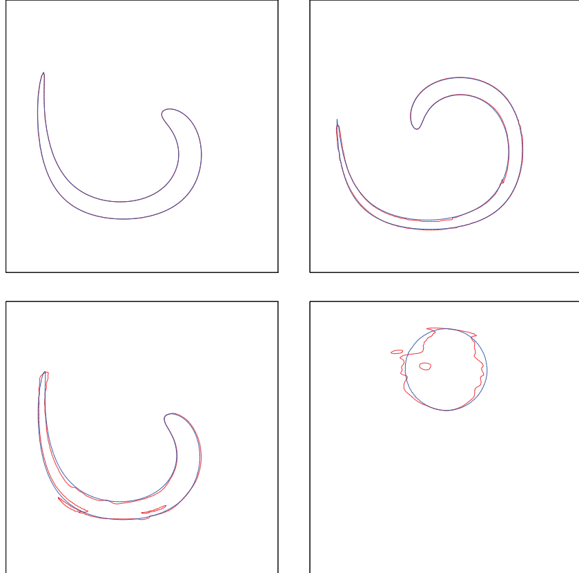
Figure 8. Vortex flow zero level sets for Optimal Control ( \beta = 10^{-1} ) in blue and Convected Reinitialization in red: t = \frac{T}{4} (top left), t = \frac{T}{2} (top right), t = \frac{3T}{4} (bottom left) and t = T (bottom right)
