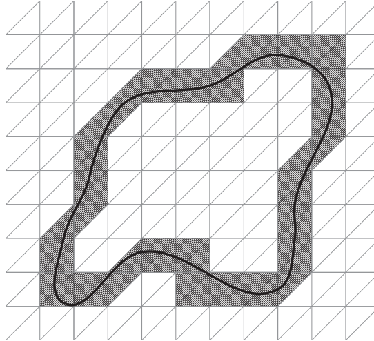
Figure 1. Interface region \Omega_{\text{int}} (shaded)
