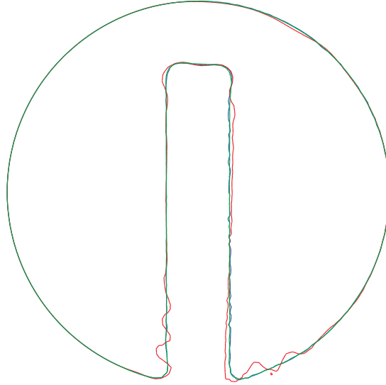
Figure 7. Isocontours of the non-reinitialized approach (green), the Optimal Control approach (blue) and the Convected Reinitialization approach (red)
