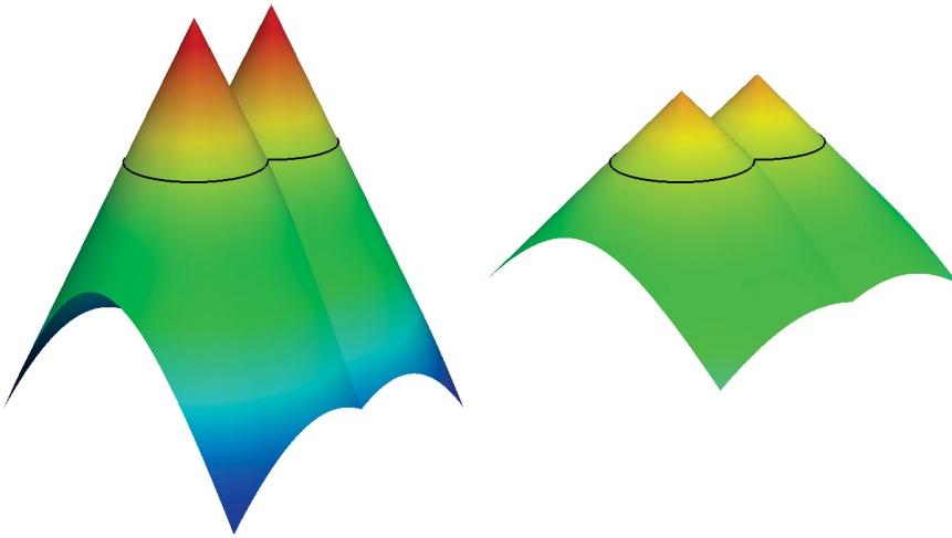
Figure 5. Non-convex overlapping circle interface: initial condition (left) and the level set function after reinitialization (right)
