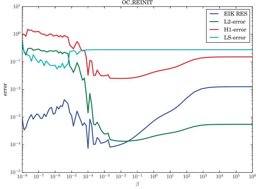
Figure 2. Influence of regularization parameter \beta on the errors of \varphi_h .
