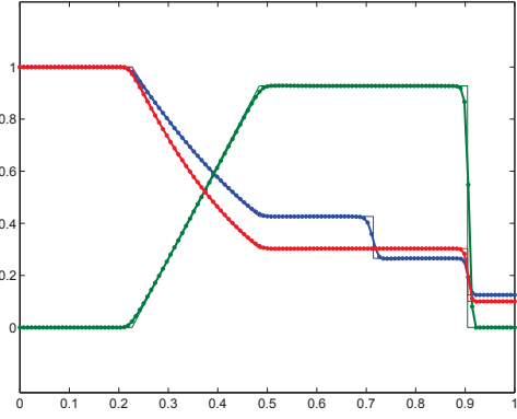
(b) HLL- P_1 -L, E_2^p=9.93\text{e-}5
