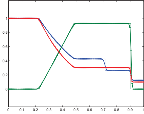
(a) LF- P_1 -L, E_2^p=9.83\text{e-}5
