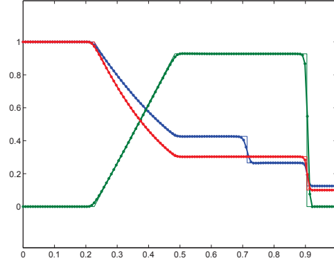
(c) LF- P_1 -Q, E_2^p=9.61\text{e-}5
