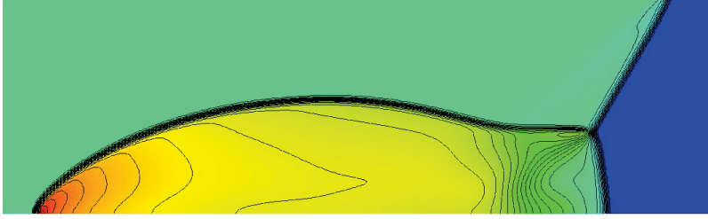
(a) HLL- P_0 , \rho \in [1.4, 20.60]
