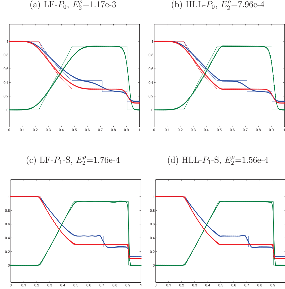
Figure 2: Shock tube problem: P_0 vs. P_1 with segregated limiting of the conserved variables, h = 1/128 , \Delta t = 10^{-3} . Snapshots of the density (blue), velocity (green), and pressure (red) distribution along the line y = 0.5 at t = 0.231 .
