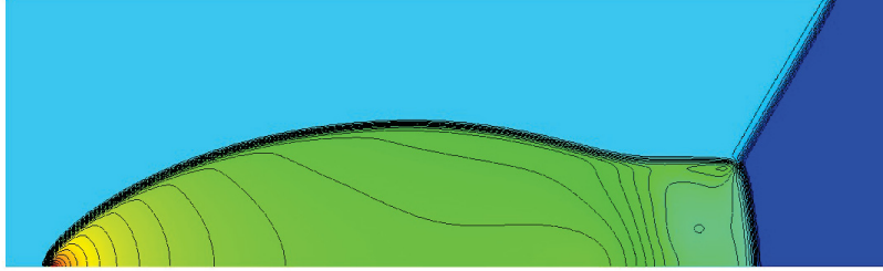
(a) HLL- P_0 , p \in [1.0, 544.41]
