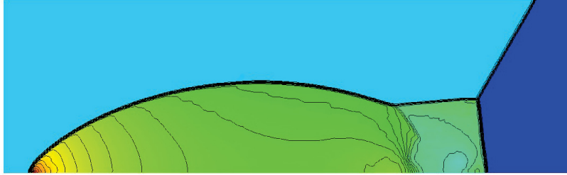
(c) HLL- P_1 -L, p \in [1.0, 543.41]
