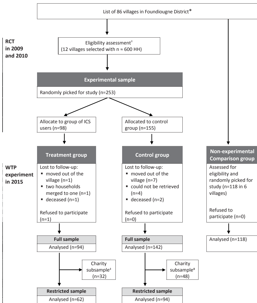
Figure 1: Participant Flow
