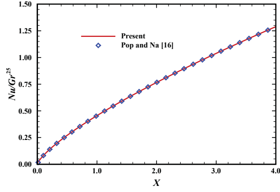
Fig. 2 Nusselt number coefficient for Pr = 0.72 , \phi = 10^\circ , D_\rho = 0.0 , \gamma = 0.0 , \epsilon = 0.0 and n = 0.0 .
