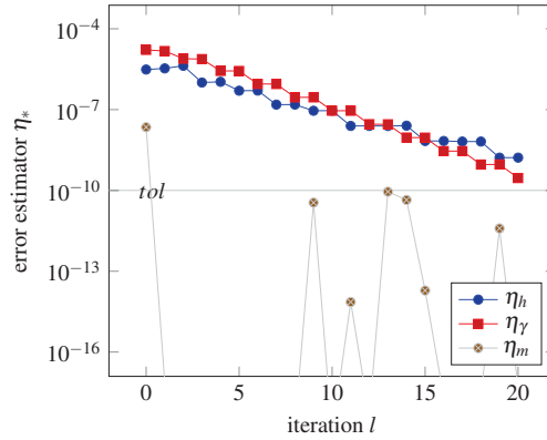
FIGURE 6. Second example: absolute value of the estimator in the l -th iteration
