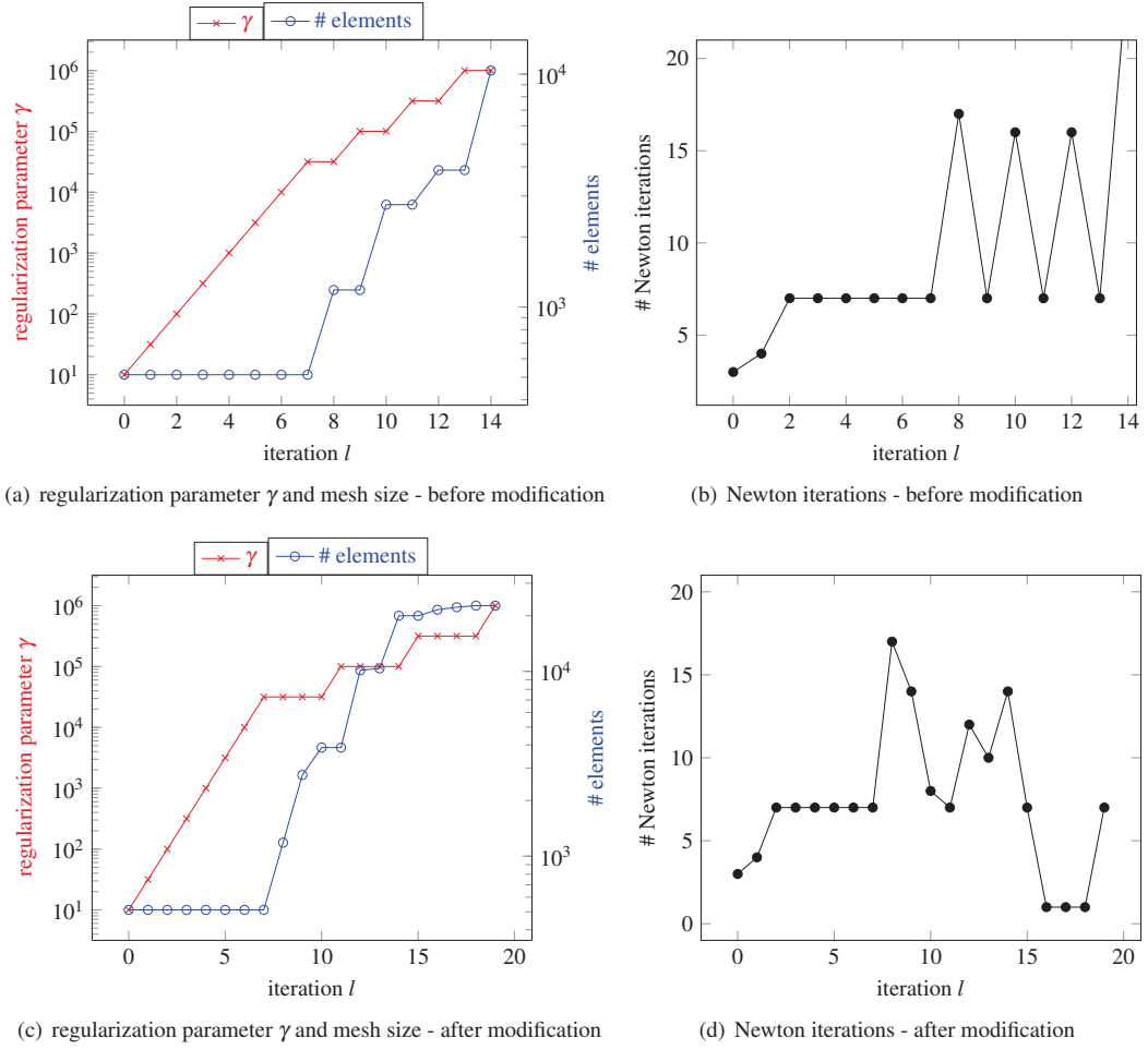
FIGURE 10. Third example: development of simulation parameters and number of Newton iterations per global iteration
