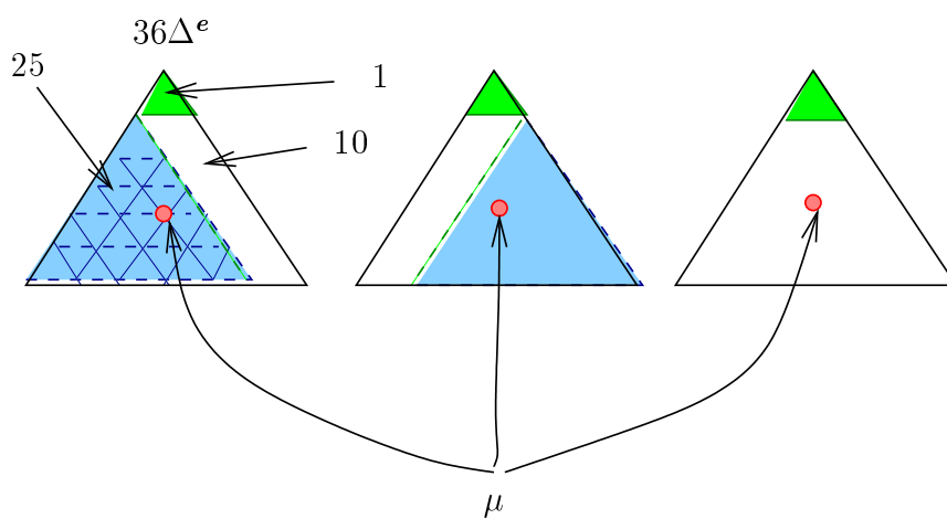
Figure 5.4: Representing the cepheid of Figure 5.3
