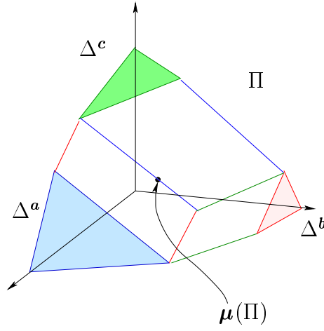
Figure 5.1: The solution for a variant of Figure 5.1
