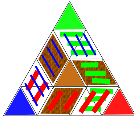
Figure 2.7: Structure of a sum of four prisms
