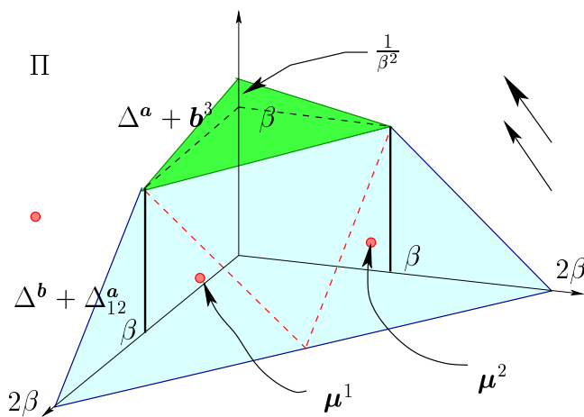
Figure 5.3: The solution for a variant of Figure 2.3
