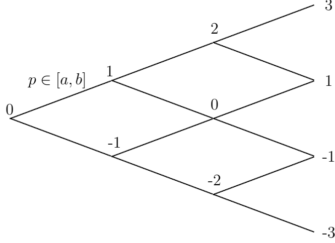
Figure 1: Cox-Ross-Rubinstein Model
