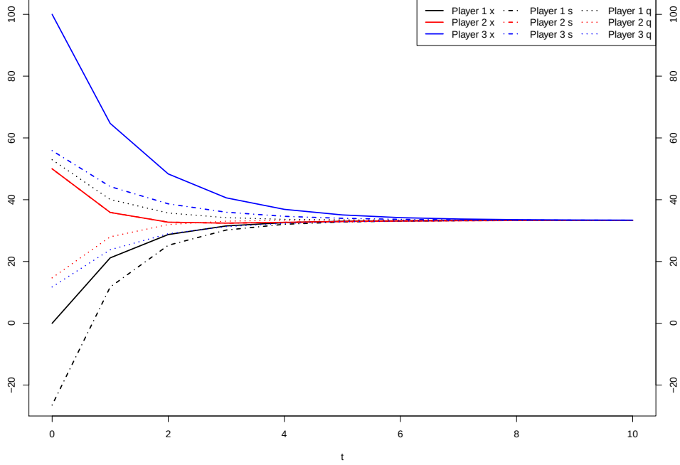
Figure 2: A three-agent example with one honest, one conforming, and one counter-conforming agent.
