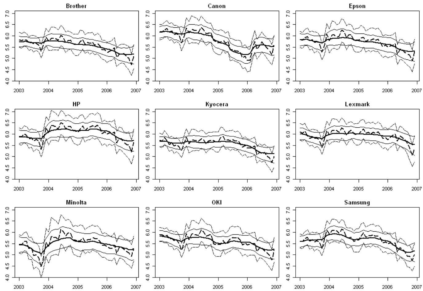
Figure 1: Time series of the period-by-period OLS estimates with pointwise 2\sigma -intervals (broken lines) and the MCMC estimates with 0.95-confidence bands (solid lines) of the brand coefficients
