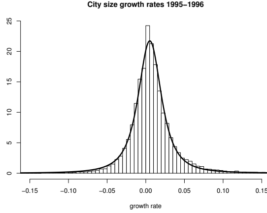
Figure 1: Histogram of the city size growth rates and a fitted t -distribution with two degrees of freedom.
