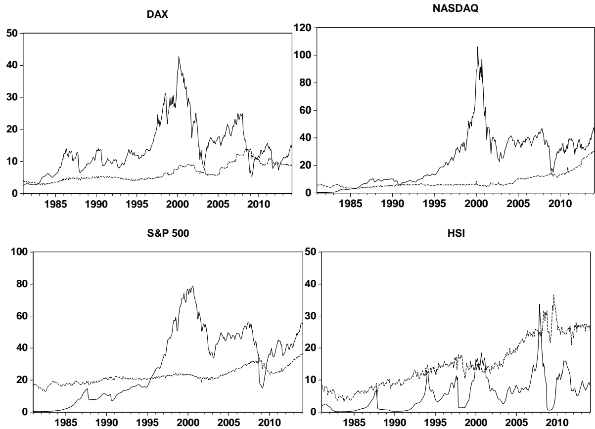
Figure 6. Estimated bubble processes (solid lines) and fundamental processes (dashed lines) of the DAX, NASDAQ, S&P 500 and HSI
