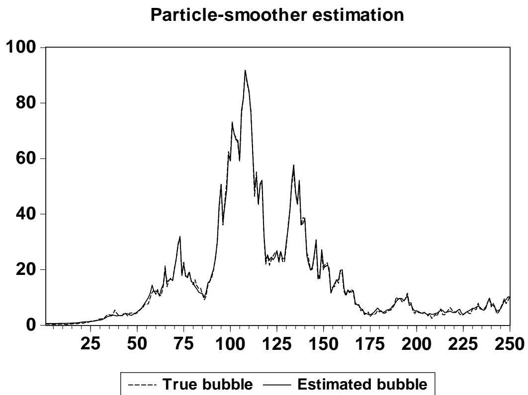
Figure 4. True versus estimated bubble processes
