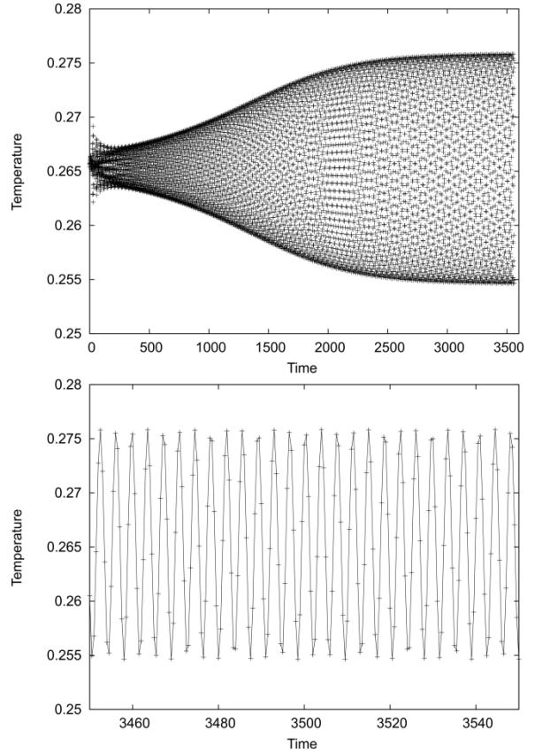
Fig.4. Temperature oscillation at \beta = 0.65 .
