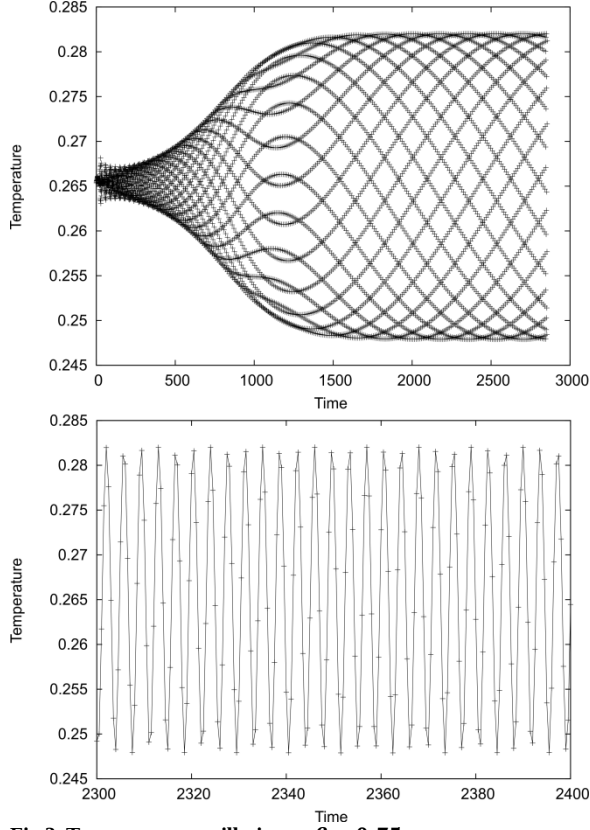
Fig.3. Temperature oscillation at \beta = 0.75 .
