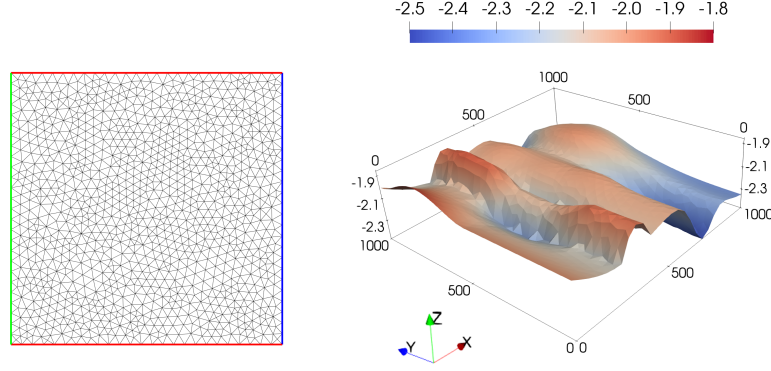
Fig. 1.1: Computational domain and mesh (left), exact bathymetry (right).
