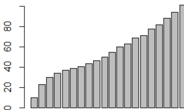
Figure 6. Barplot.
