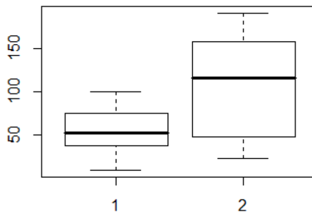
Figure 7. Boxplot.
