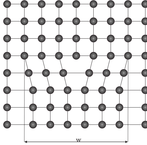
Figure 2.6: Width of dislocation.
