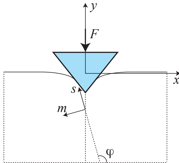
Figure 4.1: Wedge indentation.
