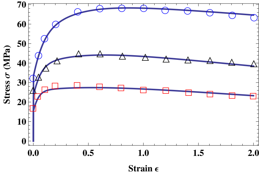
Figure 3.3: Stress-strain curves for aluminum at the highest strain rate \dot{\epsilon} = 25 \text{ s}^{-1} , for temperatures 300 C, 400 C, 500 C shown from top to bottom. The experimental points are taken from Shi et al. (1997a).
