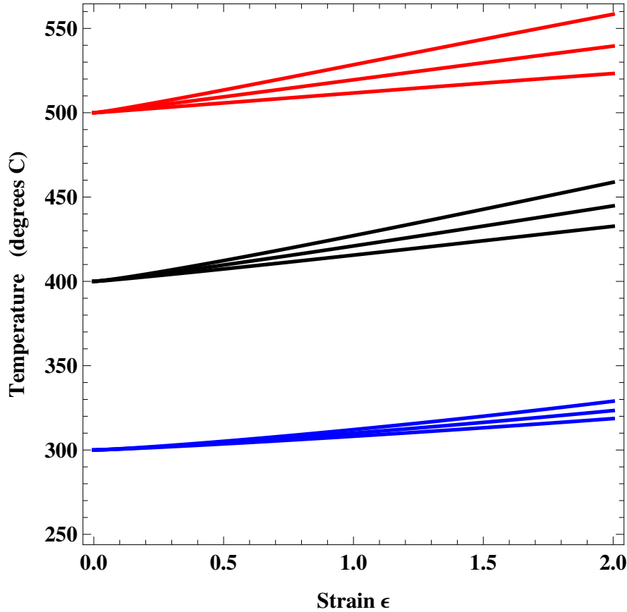
Figure 3.8: Temperature as a function of strain for each of the nine stress-strain tests shown for aluminum in the preceding figures. The initial ambient temperatures are 300 \text{ C} , 400 \text{ C} and 500 \text{ C} (blue, black, and red) as seen on the left axis. Each group of three curves is for strain rates of \dot{\epsilon} = 0.25 \text{ s}^{-1} , 2.5 \text{ s}^{-1} , and 25 \text{ s}^{-1} , from bottom to top.
