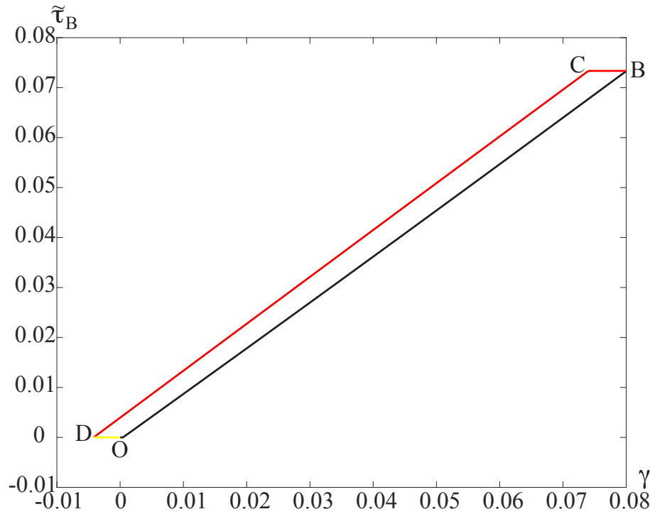
Figure 4.27: The normalized back stress \tilde{\tau}_B near the boundary versus \gamma at the strain rate \dot{Q} = 10^{-13} , for room temperature, and for \gamma^* = 0.08 : (i) loading path (black), (ii) load reversal (red/dark gray), (iii) second load reversal (yellow/light gray).
