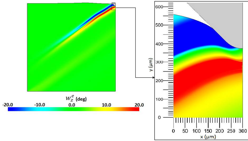
Figure 4.16: Simulated lattice rotation [\frac{1}{2}(v_{,x} - u_{,y}) + \frac{1}{2}\beta] \times 180^\circ/\pi , h = 200\mu\text{m} .
