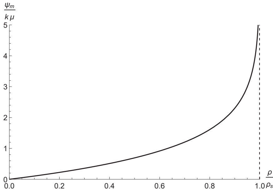
Figure 4.2: Energy density of dislocation network.
