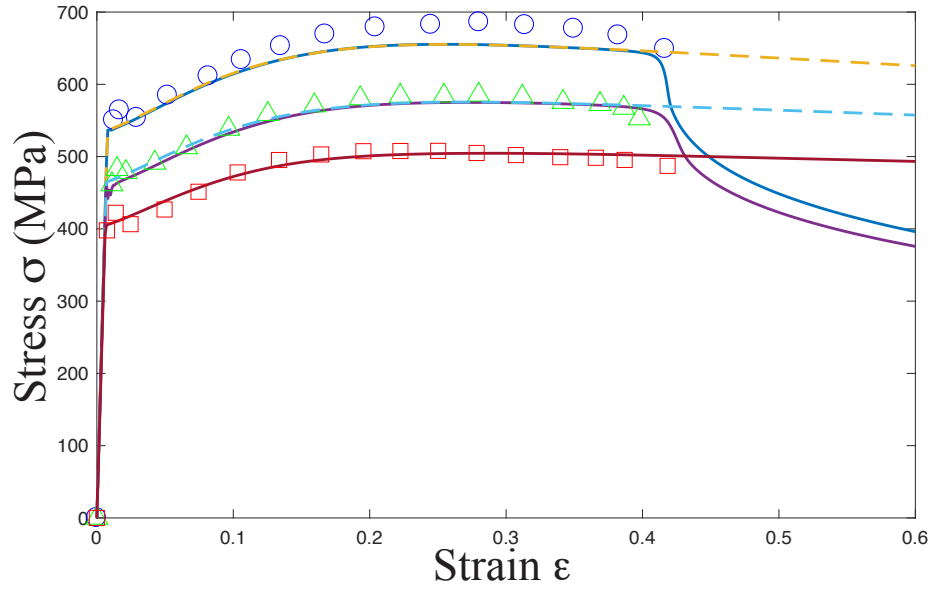
Figure 3.15: Stress-strain curves for steel at the strain rate \dot{\epsilon} = 1000/\text{s} , for temperatures -73^\circ\text{C} , 70^\circ\text{C} , 250^\circ\text{C} shown from top to bottom. The experimental points are taken from Marchand and Duffy (1988).
