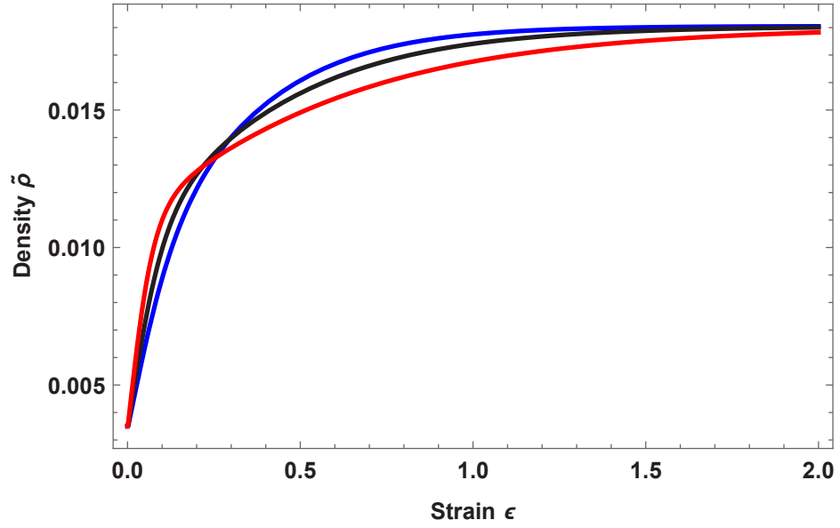
Figure 3.6: Theoretical dislocation density distribution for pure aluminum at the strain rate \dot{\epsilon} = 25 \text{ s}^{-1} , for temperatures 300 C, 400 C, 500 C shown from right to left.
