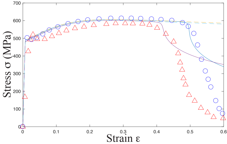
Figure 3.16: Stress-strain curves for steel at the strain rates \dot{\varepsilon} = 3300/\text{s} and \dot{\varepsilon} = 1600/\text{s} shown from top to bottom, for room temperature. The experimental points are taken from Marchand and Duffy (1988).
