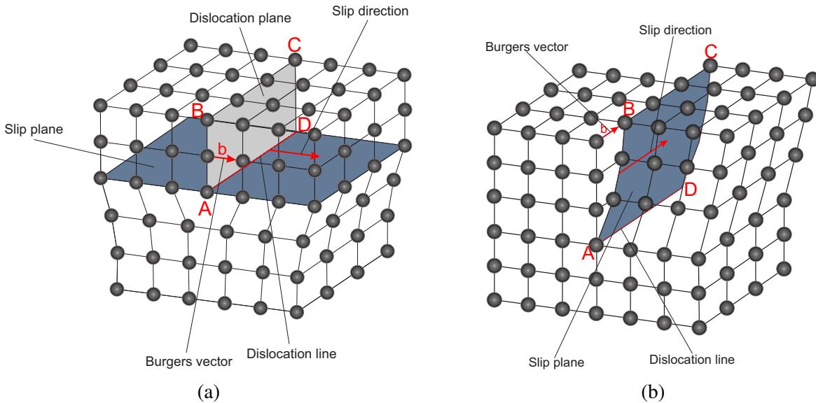
Figure 2.8: Edge and screw dislocation.
