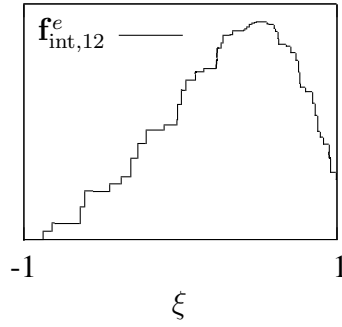
(a) 8 \times 8 standard Gauss-Legendre quadrature.
