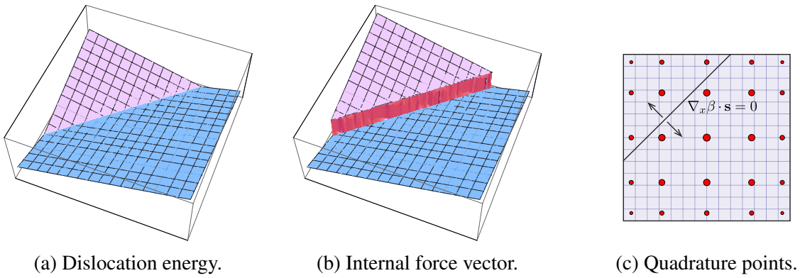
Figure 4.8: Integrands for energy and the element internal force vector.
