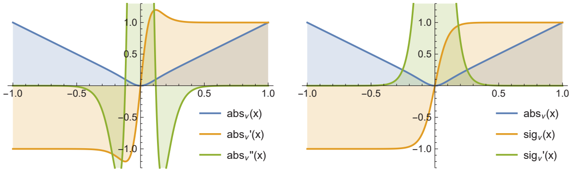
Figure 4.6: Smooth approximations of |x| and its derivatives for \nu = 20 . It can be seen that the consistent derivative in (4.19) on the left hand side has a bump close to x = 0 while the relaxed approximation of the derivative in (4.20) on the right hand side does not expose this behaviour. Furthermore, the second derivative of the relaxed formulation is strictly positive.
