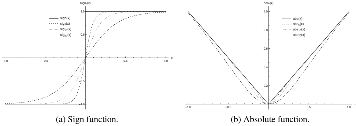
Figure 4.7: Quality of the approximate function for sign and absolute value functions with different \nu .
