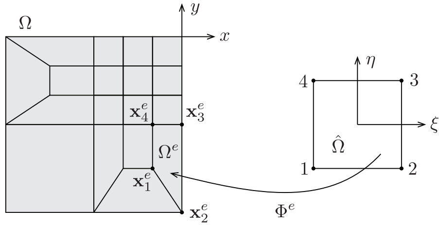
Figure 4.4: Discretization of the domain \Omega into bilinear isoparametric elements \Omega^e , e = 1, \dots, n_e . Each element \Omega^e is obtained by the mapping (4.15) from the square \hat{\Omega} = (-1, 1) \times (-1, 1) in the (\xi, \eta) -plane, with counterclockwise node numbering.
