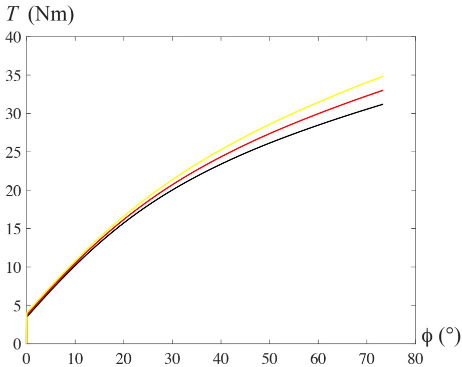
Figure 3.25: The torque-twist curves for the bars twisted at different twist rates and for room temperature: (i) \dot{\phi} = 0.25^\circ/\text{s} (black), (ii) \dot{\phi} = 2.5^\circ/\text{s} (red/dark gray), (iii) \dot{\phi} = 25^\circ/\text{s} (yellow/light gray).
