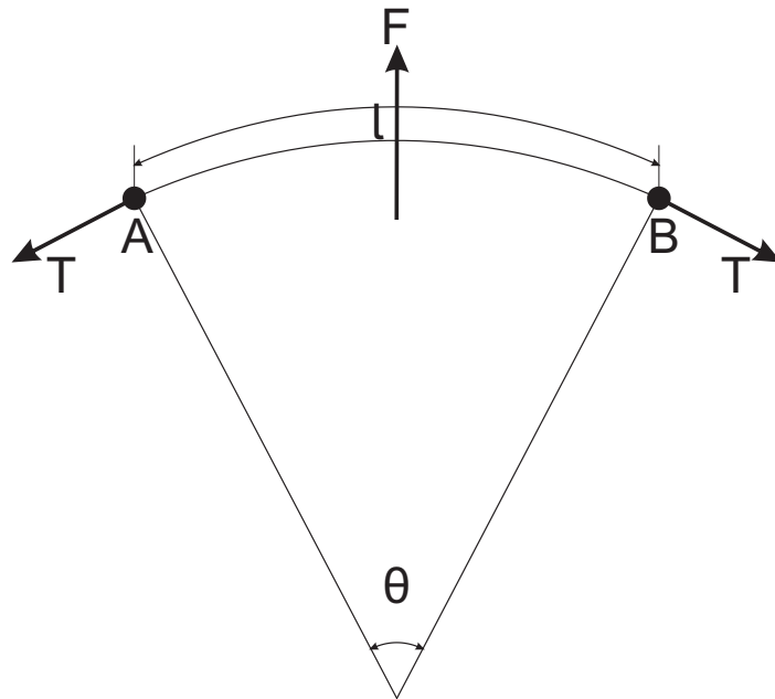
Figure 2.13: Line tension of dislocation.
