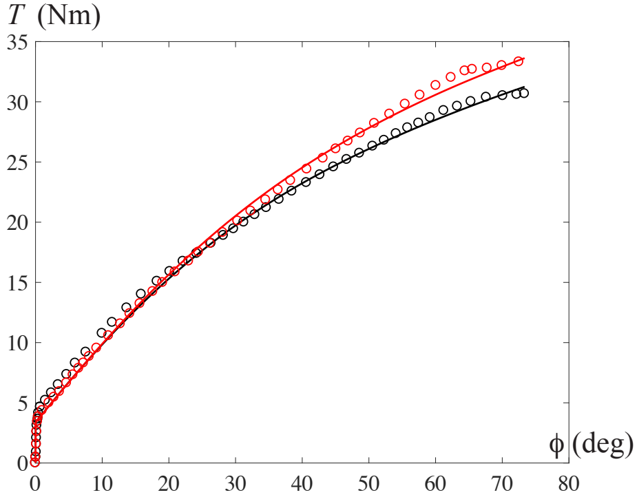
Figure 3.22: The torque-twist curves at the twist rate \dot{\phi} = 0.25^\circ/\text{s} and for room temperature: (i) sample 1: TDT-theory: black curve, experiment Horstemeyer et al. (2002): black circles (ii) sample 2: TDT-theory: red/dark gray curve, experiment Horstemeyer et al. (2002): red/dark gray circles.
