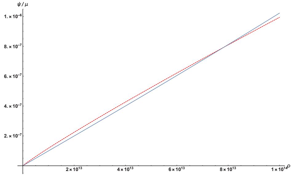
(a) \rho^g \in (0, 10^{14}/\text{m}^2) .
