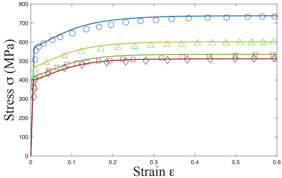
Figure 3.13: Quasi-static stress-strain curves for steel at the strain rate \dot{\epsilon} = 10^{-4}/\text{s} , for temperatures -190^\circ\text{C} , -73^\circ\text{C} , 25^\circ\text{C} , 70^\circ\text{C} shown from top to bottom. The experimental points are taken from Marchand and Duffy (1988).
