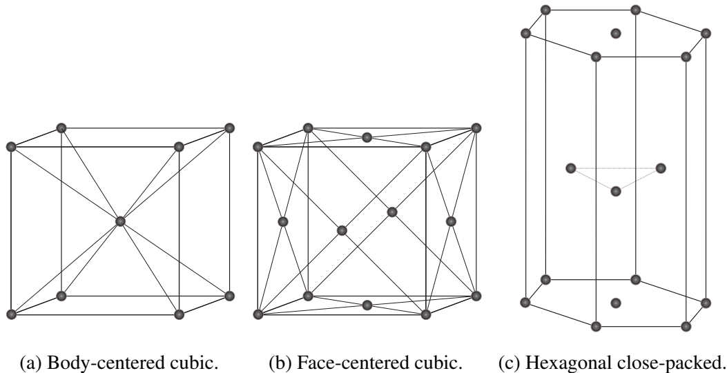
Figure 2.1: Unit cell structure of common metals.
