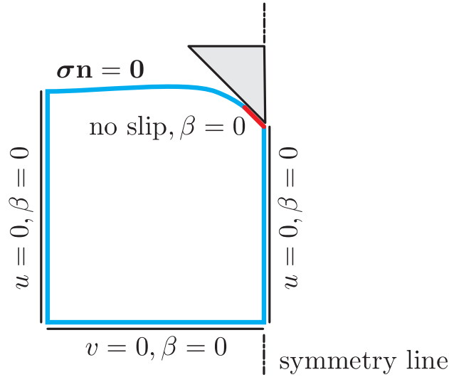
Figure 4.3: Boundary conditions for symmetric left-half.
