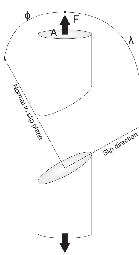
Figure 2.7: Diagram for computing resolved shear stress.
