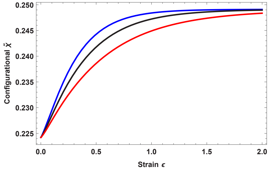
Figure 3.7: Theoretical configurational temperature for pure aluminum at the strain rate \dot{\epsilon} = 25 \text{ s}^{-1} , for temperatures 300 C, 400 C, 500 C shown from left to right.
