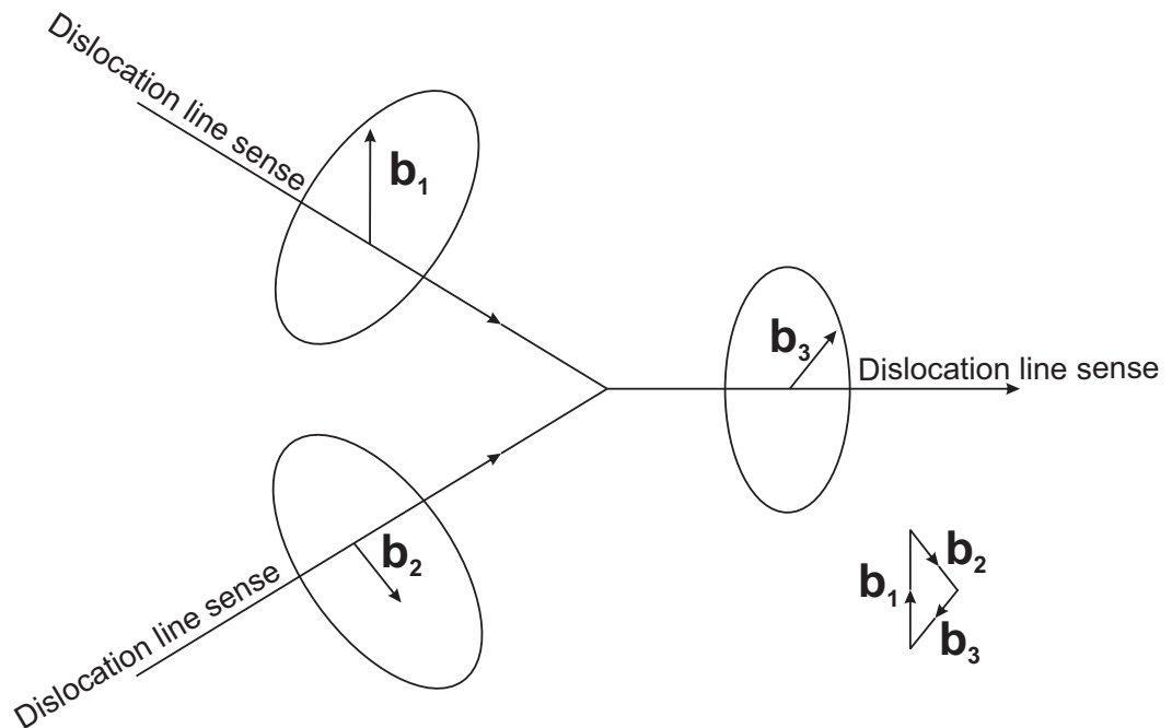
Figure 2.10: Sum of two dislocation lines.
