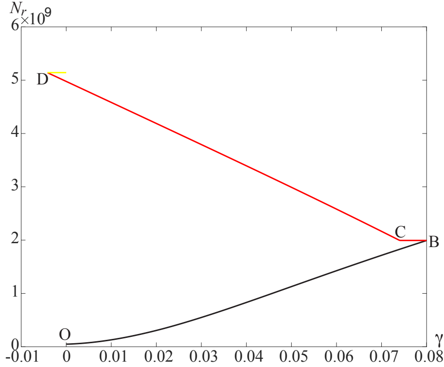
Figure 4.24: N_r versus \gamma at the strain rate \tilde{Q} = 10^{-13} , for room temperature, and for \gamma^* = 0.08 : (i) loading path (black), (ii) load reversal (red/dark gray), (iii) second load reversal (yellow/light gray).
