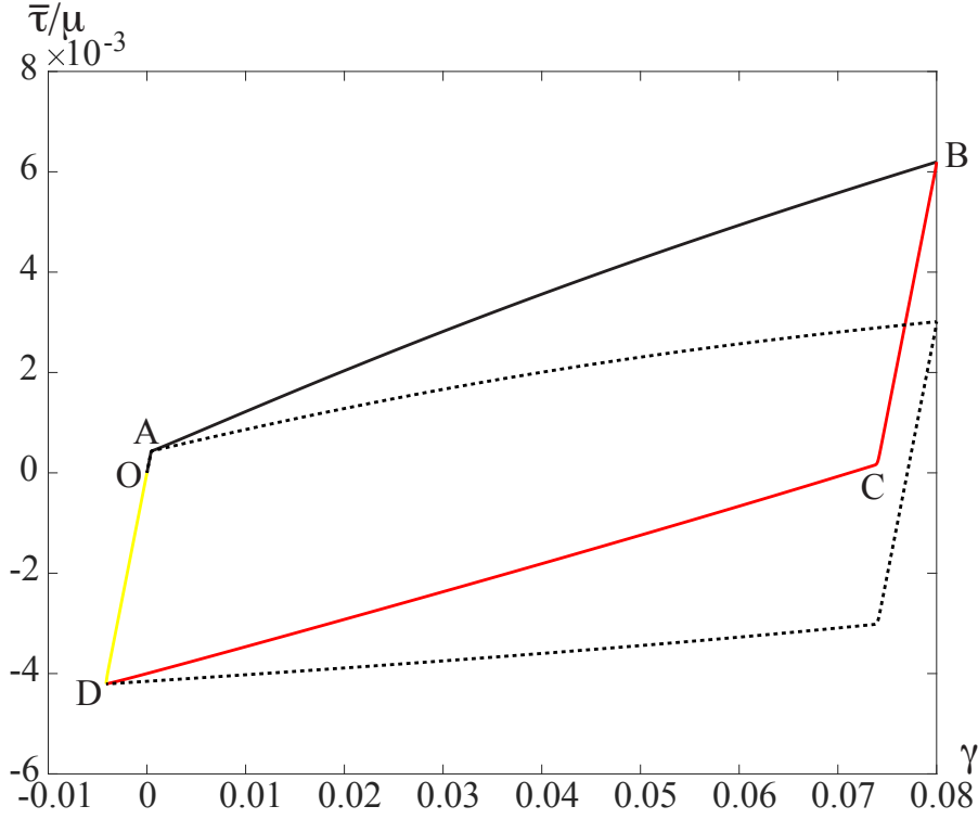
Figure 4.21: Stress-strain curves at the strain rate \tilde{Q} = 10^{-13} , for room temperature, and for \gamma^* = 0.08 : (i) loading path OAB (black), (ii) load reversal BCD (red/dark gray), (iii) second load reversal DO (yellow/light gray), (iv) flow stress versus strain (dashed black curve).
