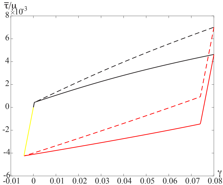
Figure 4.28: The stress-strain curves for specimens with different sizes at the strain rate \tilde{Q} = 10^{-13} , for room temperature, and for \gamma^* = 0.08 : (i) c = 5.1 micron (dashed), (ii) c = 51 micron (bold).
