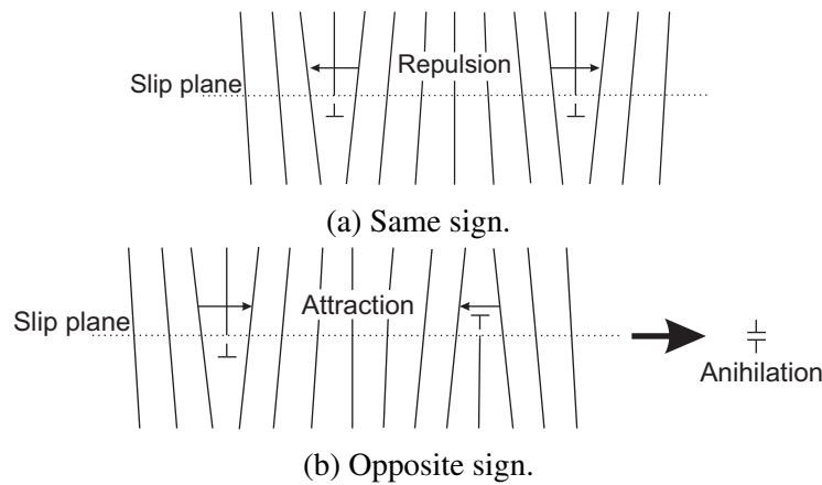
Figure 2.16: Interaction of two straight edge dislocations lying on the same slip planes.
