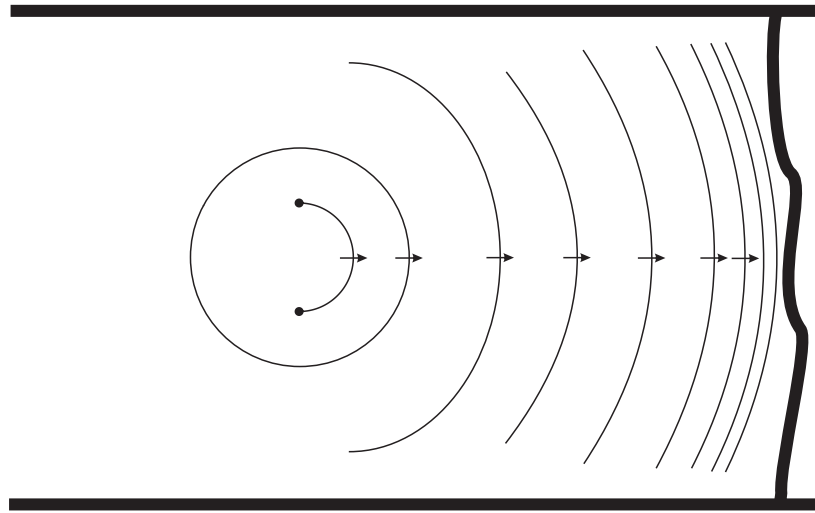
Figure 2.15: From Frank-Read source to dislocation pile-up against grain boundary.
