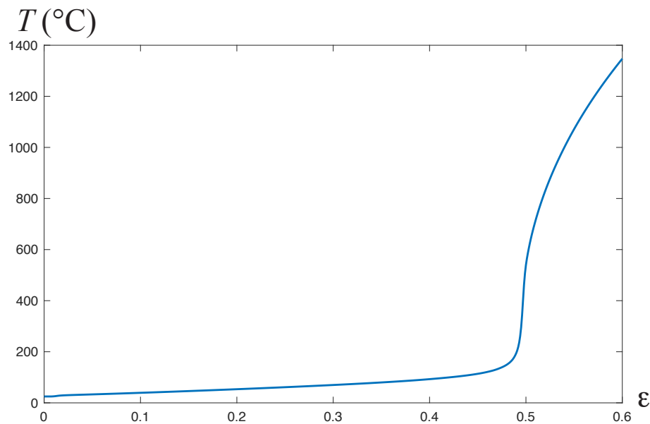
Figure 3.20: Temperature at the center of the shear band ( \tilde{y} = 0 ) for the strain rate \dot{\epsilon} = 3300/\text{s} and room temperature as the function of the strain.
