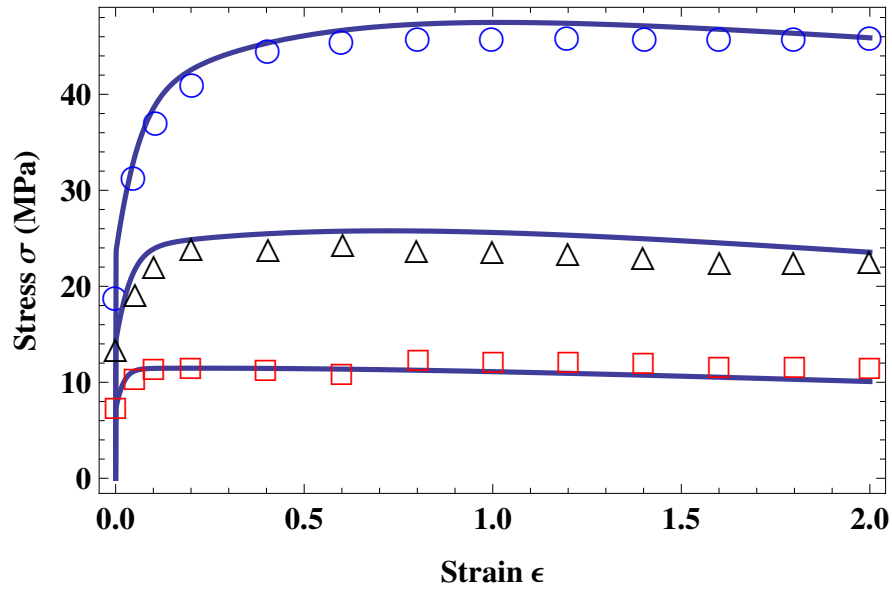
Figure 3.1: Stress-strain curves for aluminum at the small strain rate \dot{\epsilon} = 0.25 \text{ s}^{-1} , for temperatures 300°C, 400°C, 500°C shown from top to bottom. The experimental points are taken from Shi et al. (1997a).
