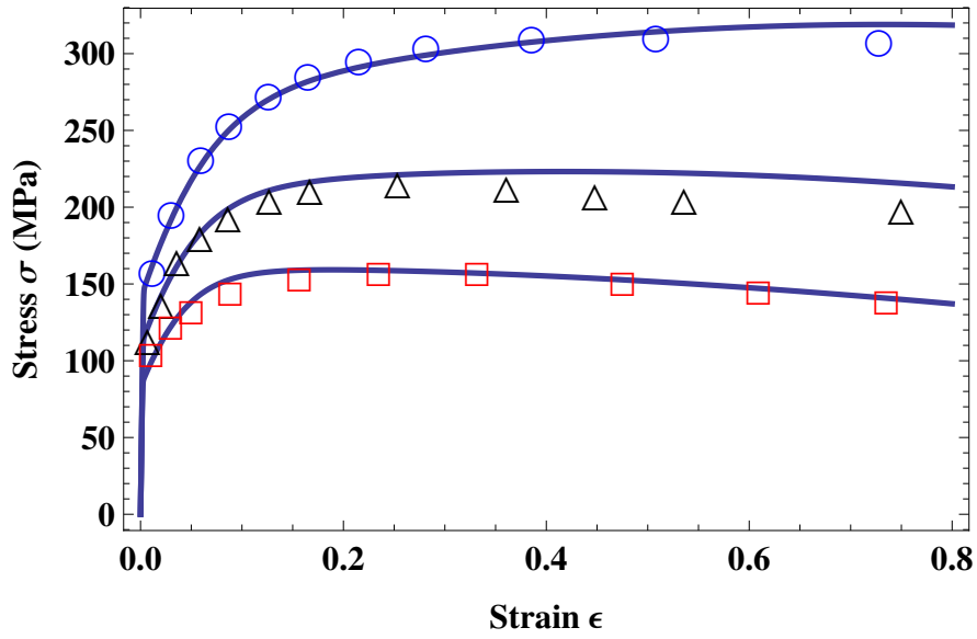
Figure 3.10: Stress-strain curves for steel at the strain rate \dot{\epsilon} = 1.0 \text{ s}^{-1} , for temperatures 850 C, 950 C, 1050 C shown from top to bottom. The experimental points are taken from Abbod et al. (2007).
