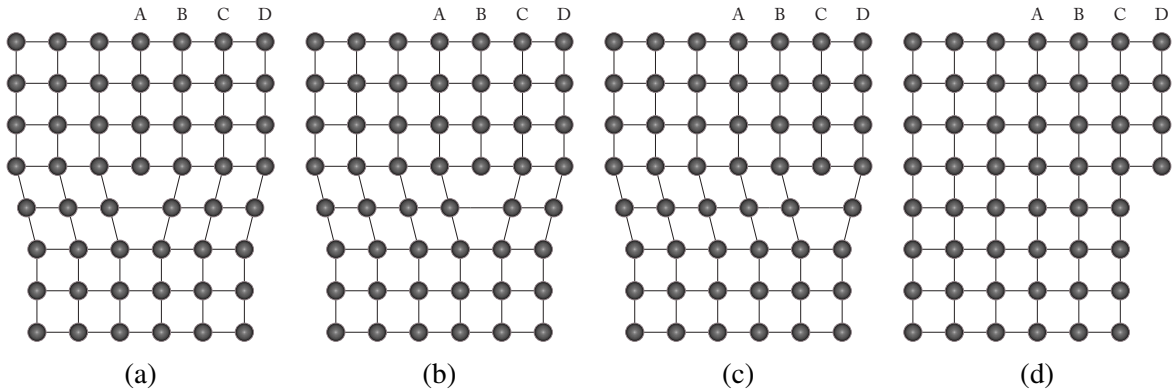
Figure 2.5: Dislocations traveling through the crystal lattice in response to an applied shear stress.
