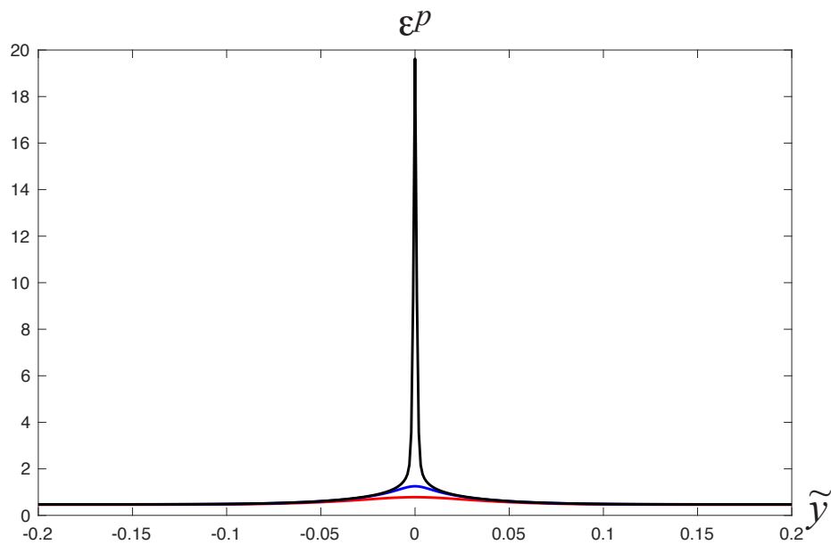
Figure 3.18: Plastic strain distributions for the strain rate \dot{\varepsilon} = 3300/\text{s} and room temperature at the strains \varepsilon = 0.47 (red), \varepsilon = 0.49 (blue), and \varepsilon = 0.51 (black).
