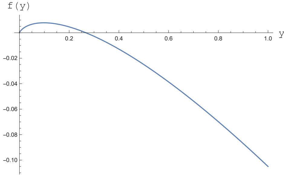
Figure 4.18: Dimensionless energy density f(y) = \psi_m/\mu .
