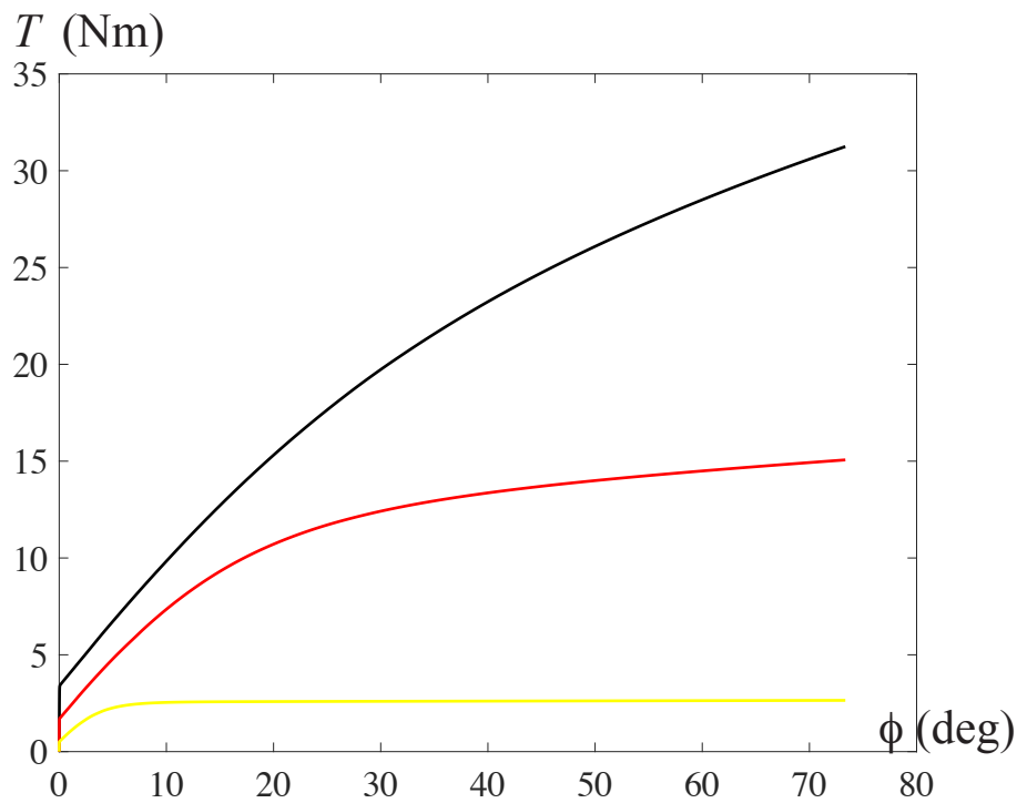
Figure 3.26: (Color online) The torque-twist curves for the bars twisted at the same twist rate \dot{\phi} = 0.25^\circ/\text{s} and for three different ambient temperatures: (i) T = 25^\circ\text{C} (black), (ii) T = 250^\circ\text{C} (red/dark gray), (iii) T = 500^\circ\text{C} (yellow/light gray).
