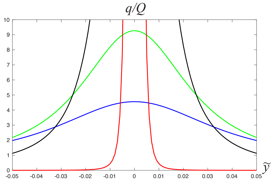
Figure 3.17: Theoretical fractional strain rate distributions for steel for \dot{\varepsilon} = 3300/\text{s} at room temperature: (i) at strain \varepsilon = 0.45 (blue), (ii) at strain \varepsilon = 0.47 (green), (iii) at strain \varepsilon = 0.49 (black), (iv) at strain \varepsilon = 0.497 (red).
