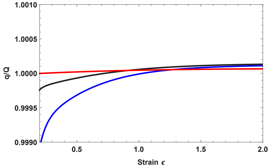
Figure 3.4: Theoretical fractional strain rate distribution for pure aluminum at the strain rate \dot{\epsilon} = 0.25 \text{ s}^{-1} , for temperatures 300 \text{ C} , 400 \text{ C} , 500 \text{ C} shown from bottom to top.
