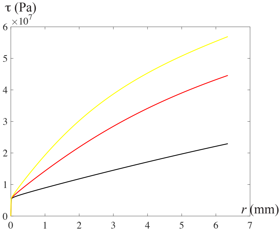
Figure 3.23: Stress distribution \tau(r) at the twist rate \dot{\phi} = 0.25^\circ/\text{s} and for room temperature: (i) \phi = 10^\circ (black), (ii) \phi = 30^\circ (red/dark gray), (iii) \phi = 50^\circ (yellow/light gray).
