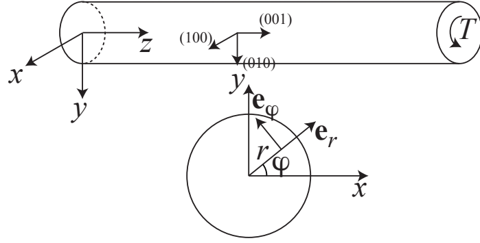
Figure 3.21: Torsion of a single crystal bar.
