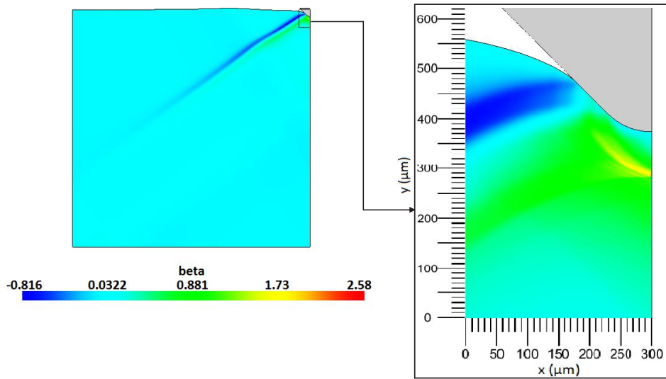
Figure 4.17: Simulated plastic slip, h = 200\mu\text{m} .
