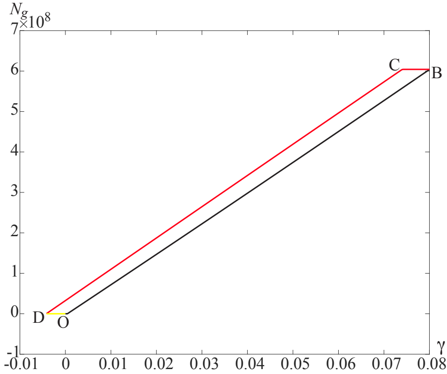
Figure 4.23: N_g versus \gamma at the strain rate \tilde{Q} = 10^{-13} , for room temperature, and for \gamma^* = 0.08 : (i) loading path (black), (ii) load reversal (red/dark gray), (iii) second load reversal (yellow/light gray).
