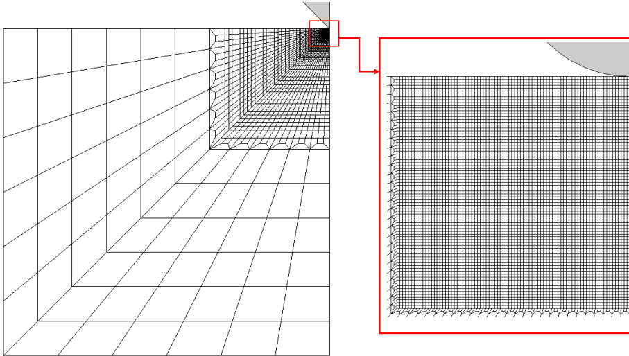
Figure 4.11: Mesh distribution and the zooming near the indenter tip.
