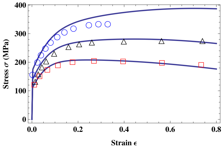
Figure 3.11: Stress-strain curves for steel at the highest strain rate \dot{\epsilon} = 10 \text{ s}^{-1} , for temperatures 850 C, 950 C, 1050 C shown from top to bottom. The experimental points are taken from Abbod et al. (2007).
