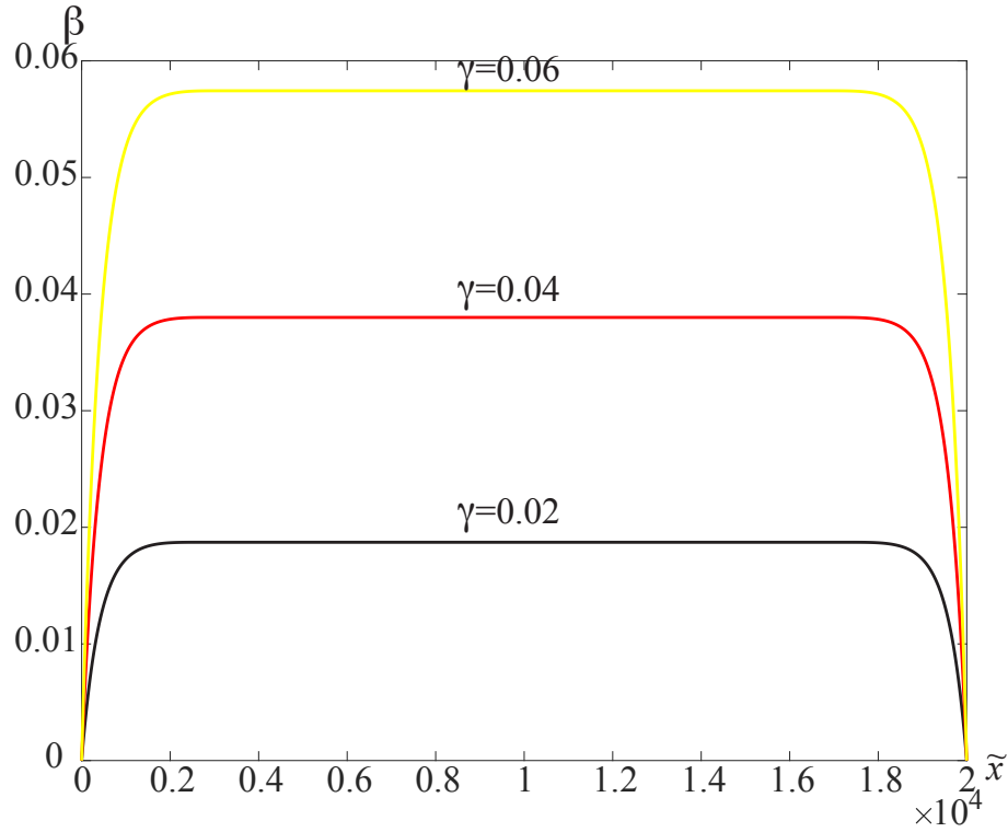
Figure 4.22: Evolution of \beta(\tilde{x}) at the strain rate \tilde{Q} = 10^{-13} and for room temperature during the loading along AB: (i) \gamma = 0.02 (black), (ii) \gamma = 0.04 (red/dark gray), (iii) \gamma = 0.06 (yellow/light gray).
