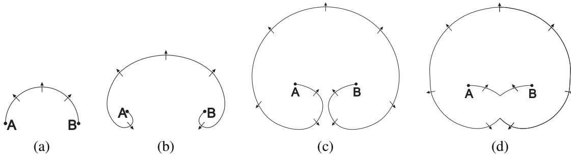
Figure 2.14: Schematic representation of Frank Read source.
