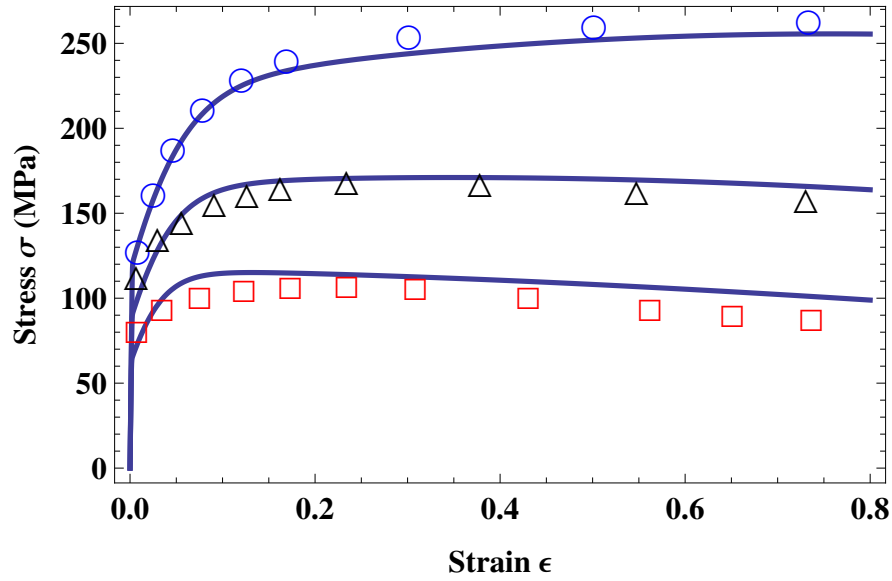
Figure 3.9: Stress-strain curves for steel at the small strain rate \dot{\epsilon} = 0.1 \text{ s}^{-1} , for temperatures 850 \text{ C} , 950 \text{ C} , 1050 \text{ C} shown from top to bottom. The experimental points are taken from Abbod et al. (2007).
