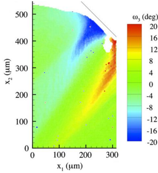
Figure 4.15: Experimental lattice rotation w_z^e from Kysar et al. (2010). Reprinted by permission.
