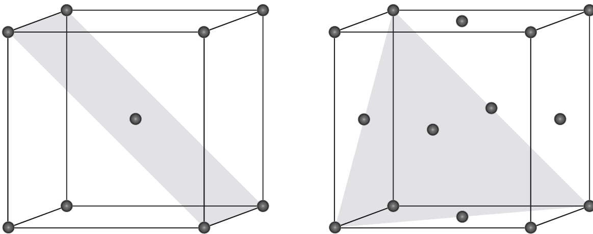
Figure 2.4: Example of most readily slip planes in BCC and FCC unit cells.
