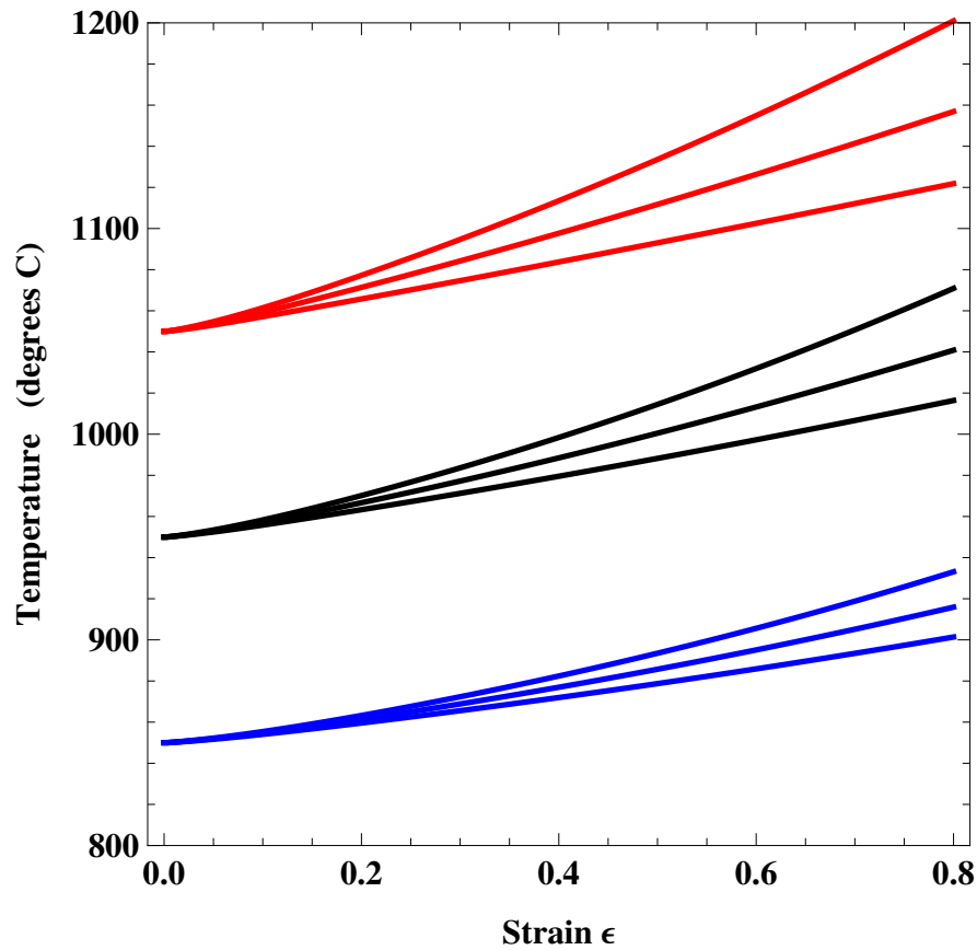
Figure 3.12: Temperature as a function of strain for each of the nine stress-strain tests shown for steel in the preceding figures. The initial ambient temperatures are 850\text{ C} , 950\text{ C} and 1050\text{ C} (blue, black, and red) as seen on the left axis. Each group of three curves is for strain rates of \dot{\epsilon} = 0.10\text{ s}^{-1} , 1.0\text{ s}^{-1} , and 10\text{ s}^{-1} , from bottom to top.
