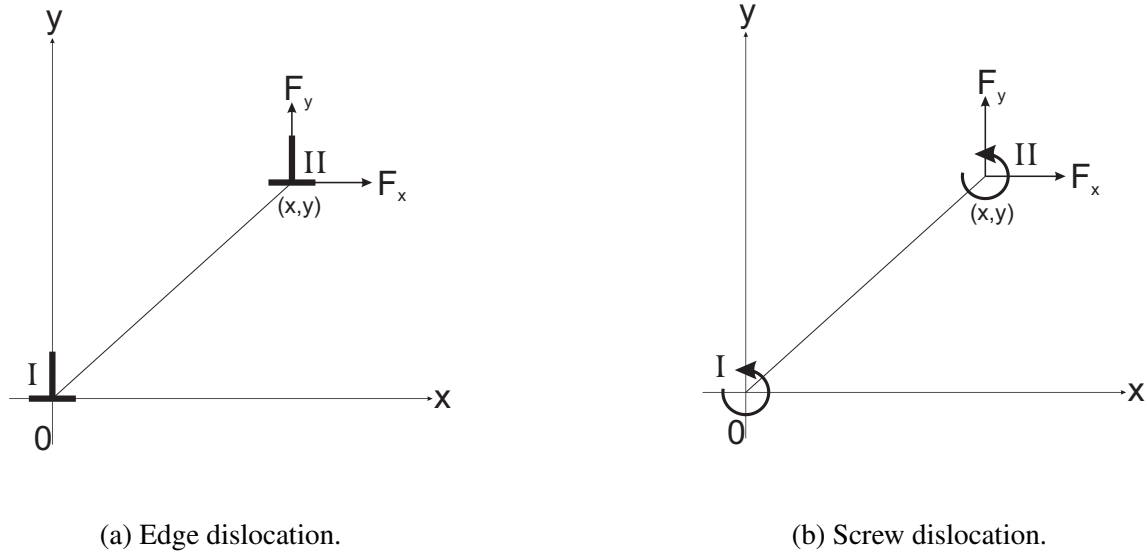
Figure 2.17: Interaction of two straight parallel on different slip planes.
