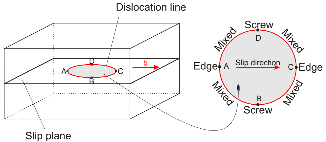
Figure 2.9: Dislocation loop.
