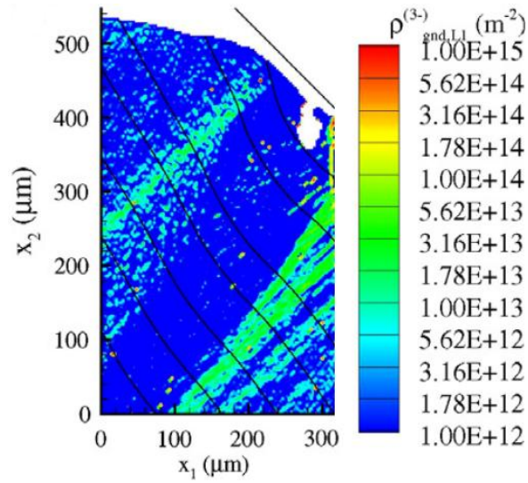
(b) \rho^- , with crystallographic traces tangential to the slip direction, h = 200\mu\text{m} .
