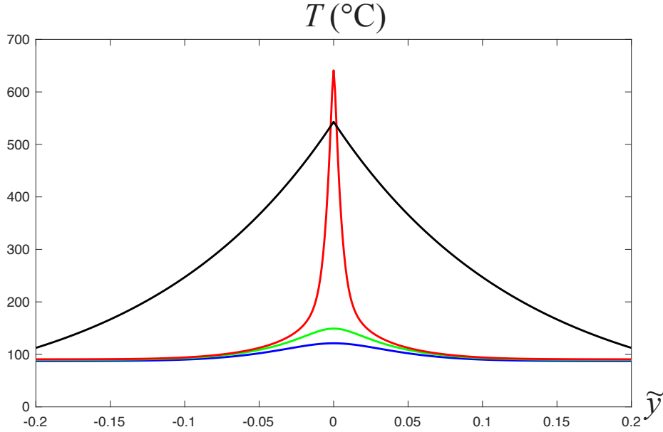
Figure 3.19: Temperature distributions for the strain rate \dot{\varepsilon} = 3300/\text{s} and room temperature at the strains \varepsilon = 0.46 (blue), \varepsilon = 0.48 (green), and \varepsilon = 0.505 (red). The black curve is the empirical law proposed by Marchand and Duffy (1988).
