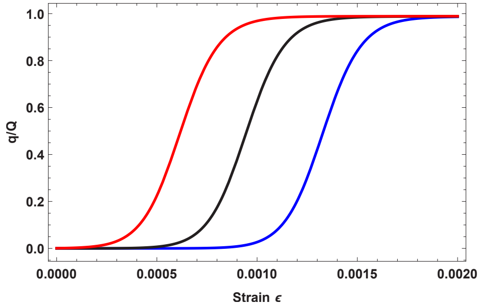
Figure 3.5: Theoretical fractional strain rate distribution across the initial yielding transition for pure aluminum at the strain rate \dot{\epsilon} = 2.5 \text{ s}^{-1} , for temperatures 300 \text{ C} , 400 \text{ C} , 500 \text{ C} shown from right to left.
