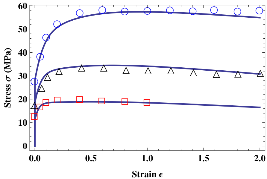
Figure 3.2: Stress-strain curves for aluminum at the strain rate \dot{\epsilon} = 2.5 \text{ s}^{-1} , for temperatures 300°C, 400°C, 500°C shown from top to bottom. The experimental points are taken from Shi et al. (1997a).
