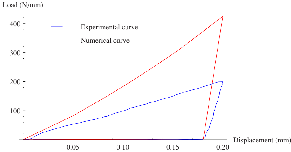
Figure 4.12: Load-displacement curve.
