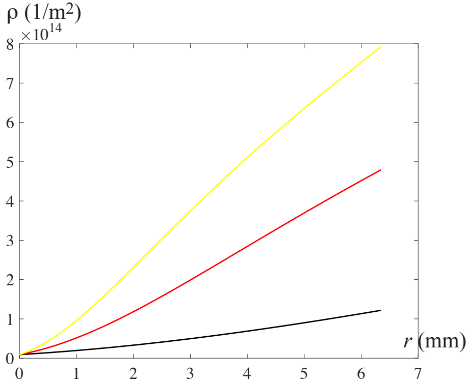
Figure 3.24: Total density of dislocations \rho(r) at the twist rate \dot{\phi} = 0.25^\circ/\text{s} and for room temperature: (i) \phi = 10^\circ (black), (ii) \phi = 30^\circ (red/dark gray), (iii) \phi = 50^\circ (yellow/light gray).
