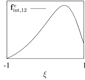
(b) 4 \times 4 quadrature on triangles.
