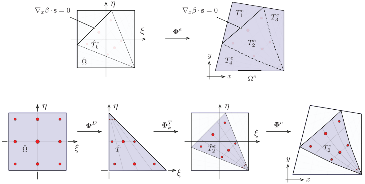
Figure 4.9: Quadrature on triangles, \hat{T} = \{(x, y)^T \in \mathbb{R}^2 \mid x, y > 0, x + y < 1\} .
