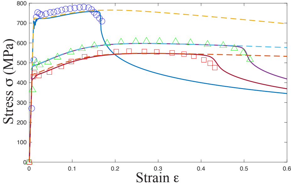
Figure 3.14: Stress-strain curves for steel at the strain rate \dot{\epsilon} = 1000/s , for temperatures -190 °C, 25 °C, 134 °C shown from top to bottom. The experimental points are taken from Marchand and Duffy (1988).
