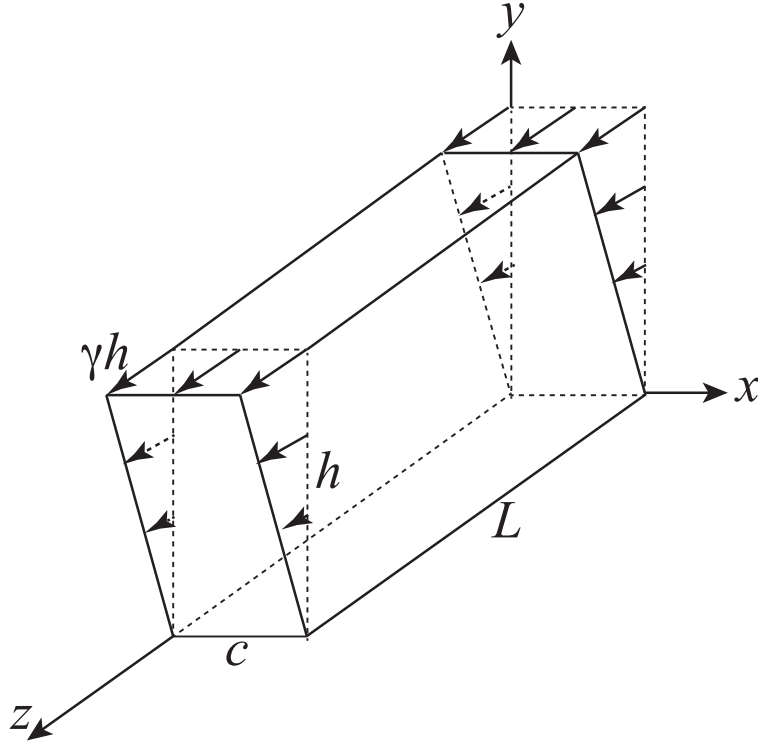
Figure 4.20: Anti-plane constrained shear.
