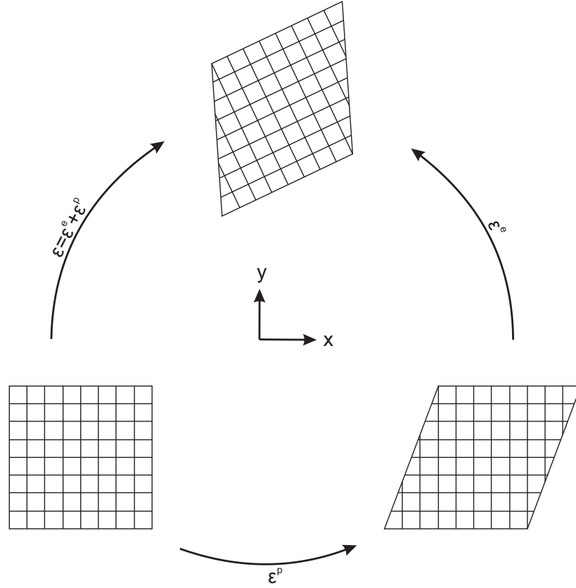
Figure 2.18: Decomposition of total strain.
