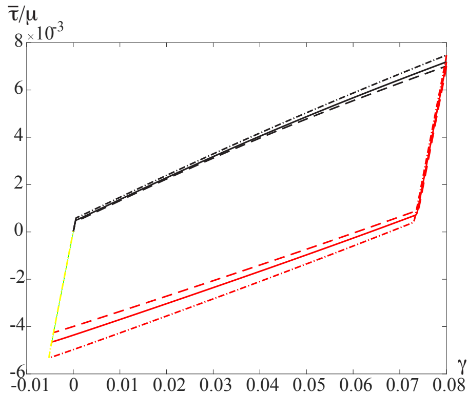
Figure 4.29: The stress-strain curves for the specimen loaded at different strain rates, for room temperature, and for \gamma^* = 0.08 : (i) \tilde{Q} = 10^{-13} (dashed), (ii) \tilde{Q} = 10^{-11} (bold), (iii) \tilde{Q} = 10^{-8} (dashed and dotted).
