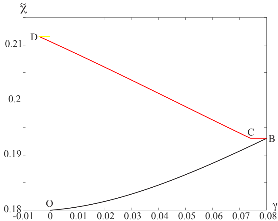
Figure 4.25: \tilde{\chi}(\tilde{c}/2) versus \gamma at the strain rate \tilde{Q} = 10^{-13} , for room temperature, and for \gamma^* = 0.08 : (i) loading path (black), (ii) load reversal (red/dark gray), (iii) second load reversal (yellow/light gray).
