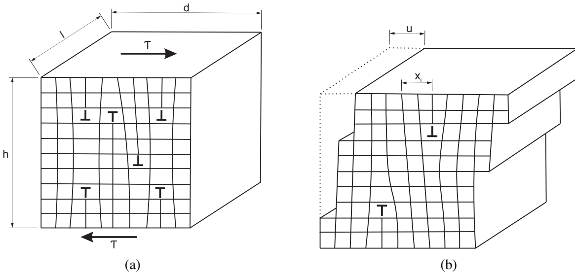
Figure 2.11: Schematic illustration for Orowan relation.
