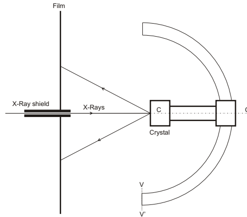
Figure 2.17: Laue back-reflection X-ray method.
