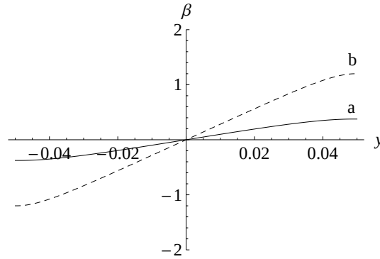
Figure 4.15: Function \beta(y) for M = 0.00015 and a) \varphi = \frac{\pi}{3} , b) \varphi = \frac{\pi}{6} .
