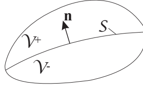
Figure 3.4: Region \mathcal{V} with the discontinuity surface \mathcal{S}
