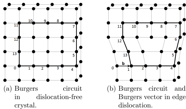
Figure 2.12: Burgers circuit around edge dislocation.
