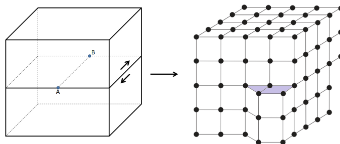
Figure 2.10: Screw dislocation.
