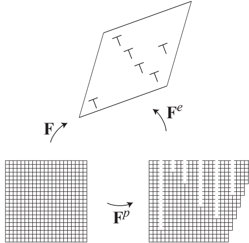
Figure 3.3: Multiplicative decomposition
