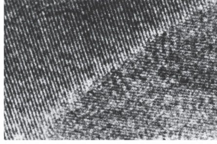
Figure 2.20: HREM micrograph of a typical grain boundary (Valiev [77]). Reprinted by permission.
