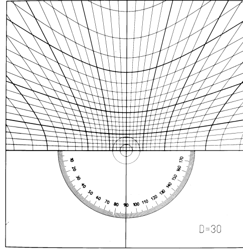
Figure 2.16: Greninger Chart (Hybler [19]). Reprinted by permission.
