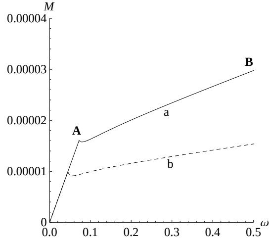
Figure 4.18: Moment-curvature curve for: a) \varphi = \frac{\pi}{3} , b) \varphi = \frac{\pi}{6} .
