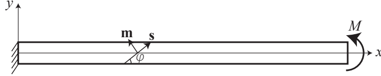
Figure 4.9: Single crystal beam bent by a moment M .
