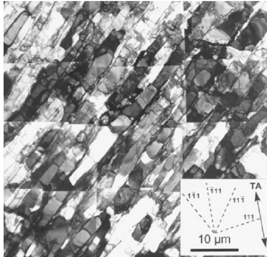
Figure 2.19: Transmission electron micrographs of polycrystalline pure aluminum (Hansen [17]). Reprinted by permission.
