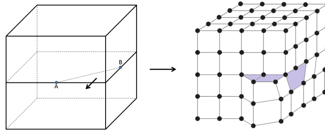
Figure 2.11: Mixed dislocation.
