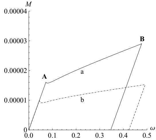
Figure 4.19: Moment-curvature curve during loading and unloading for: a) \varphi = \frac{\pi}{3} , b) \varphi = \frac{\pi}{6} .
