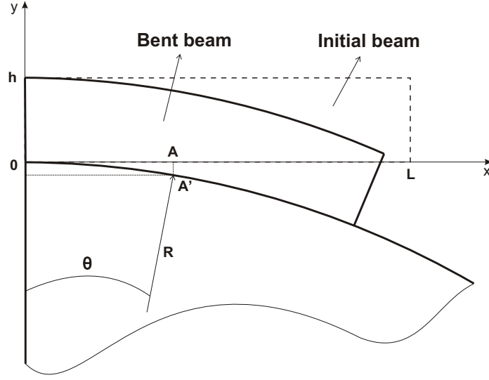
Figure 4.3: The displacements of the bent beam.
