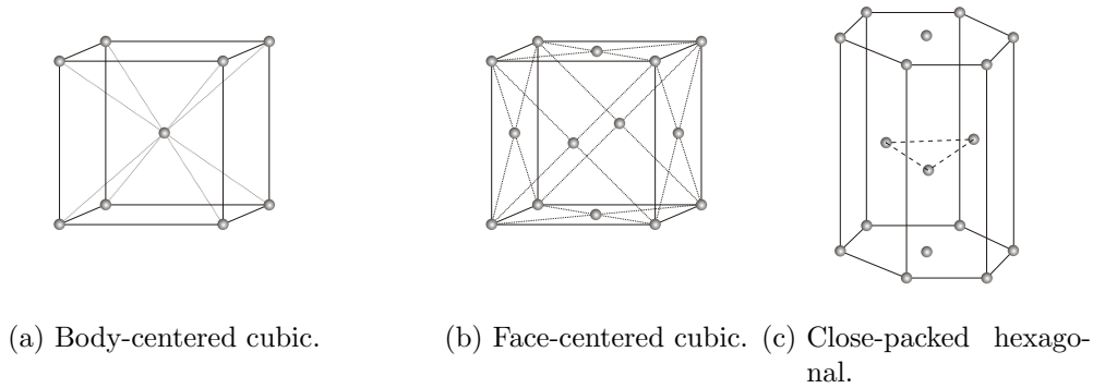
Figure 2.2: Crystal structure.
