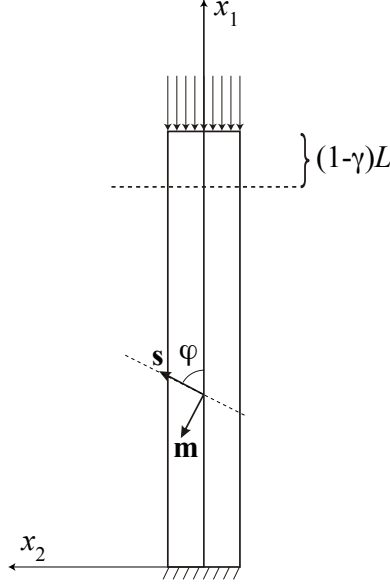
Figure 5.1: Cross section of a single crystal plate under plane strain compression.
