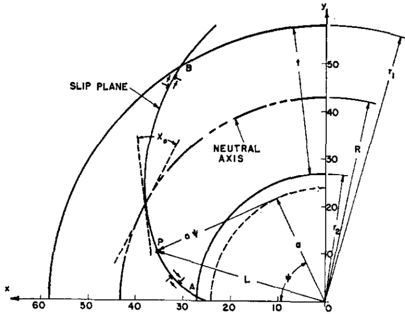
Figure 3.1: Geometry of slip planes in bent specimen (Gilman [16]). Reprinted by permission.
