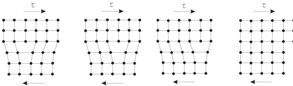
Figure 2.9: Migration of the edge dislocation.
