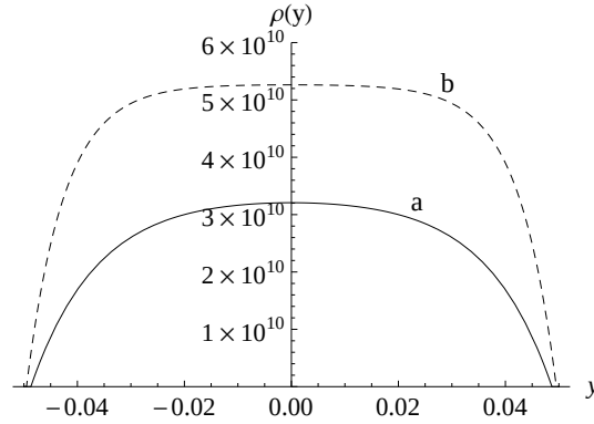
Figure 4.12: Dislocation density for M = 0.00015 and a) \varphi = \frac{\pi}{3} , b) \varphi = \frac{\pi}{6} .
