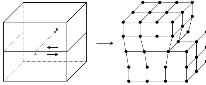
Figure 2.8: Edge dislocation.
