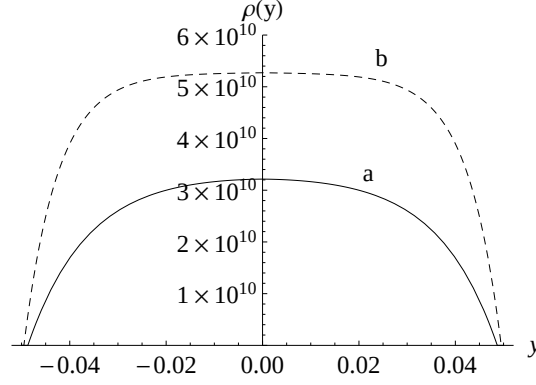
Figure 4.16: Dislocation density for M = 0.00015 and a) \varphi = \frac{\pi}{3} , b) \varphi = \frac{\pi}{6} .
