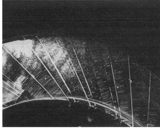
Figure 2.18: View along intersections of slip planes with polygon boundaries in a polygonized zinc crystal (Gilman [16]). Reprinted by permission.
