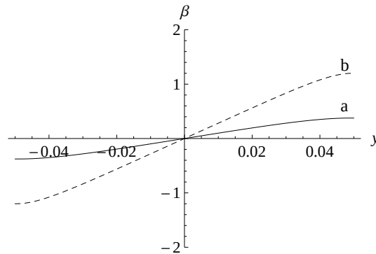
Figure 4.11: Function \beta(y) for M = 0.00015 and a) \varphi = \frac{\pi}{3} , b) \varphi = \frac{\pi}{6} .
