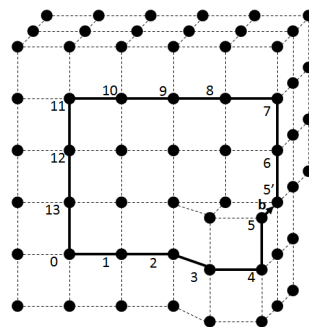
Figure 2.13: Burgers circuit and Burgers vector in screw dislocation.
