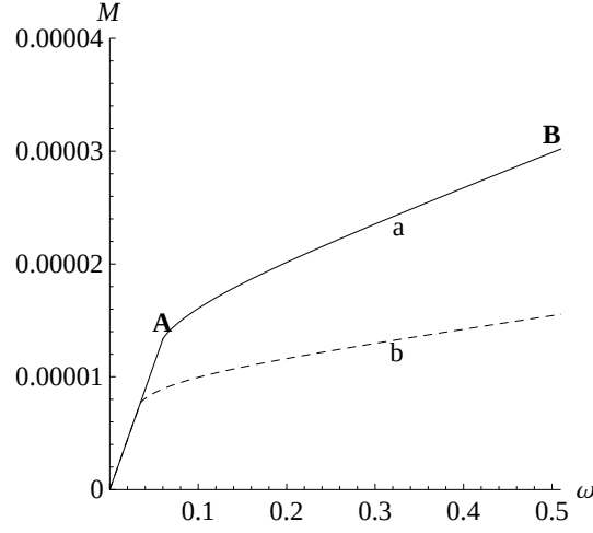
Figure 4.14: Moment-curvature curve for: a) \varphi = \frac{\pi}{3} , b) \varphi = \frac{\pi}{6} .
