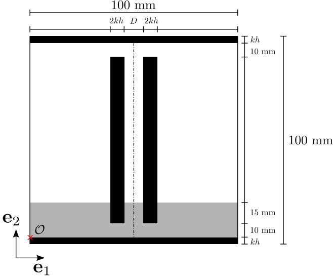
Figure 4.14: Initial simulation configuration for capillary rise between parallel plates. For further details on color coding of bulk phases in schematic, see caption to Fig 4.11.
