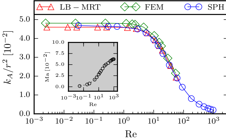
Figure 5.2: Dependence of the non-dimensional apparent permeability on Re as predicted by our SPH calculations compared to reference results for the same pore-space morphology published in Narváez et al. [147]. Non-dimensionalization was performed with respect to the cross-sectional fibre radius r . The inset shows the filter velocity based Mach number.
