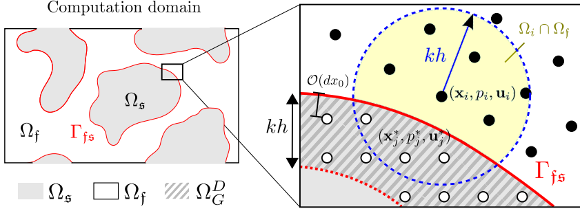
Figure 3.11: Schematic representation of fixed ghost particles (open markers) that populate the ghost domain (shaded region) adjacent to a solid surface (red line). Ghost particles serve as sampling points for fluid particles \mathbf{x}_i \in \Omega_f (closed markers). Fictitious ghost particle properties p_j^* and \mathbf{u}_j^* enforce essential boundary conditions. Upon discretization, the spatial uncertainty with respect to the exact position of the boundary \Gamma_{fs} is of order \mathcal{O}(dx_0) .
