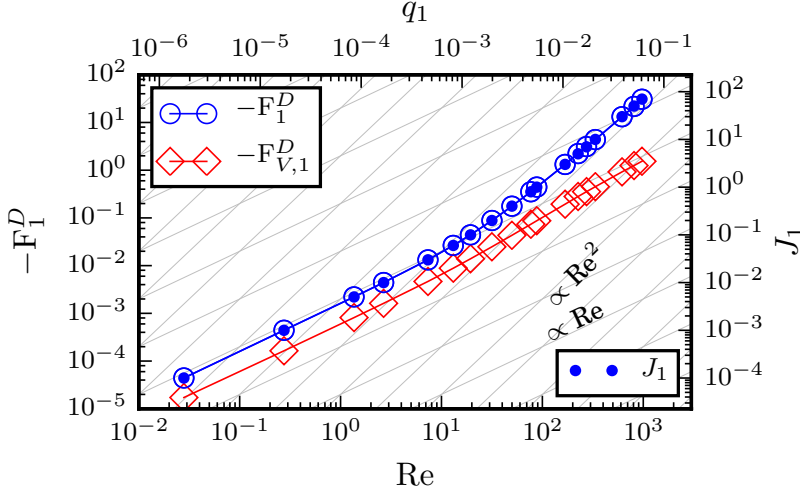
Figure 5.3: Dependence of the total microscopic drag force F_1^D [N], skin friction component F_{V,1}^D [N] and macroscopic external driving force J_1 [N/m 3 ] on Re and the filter velocity q_1 [m/s]. A set of curves scaling either with Re or Re^2 are plotted to indicate scaling properties of F_1^D and J_1 .
