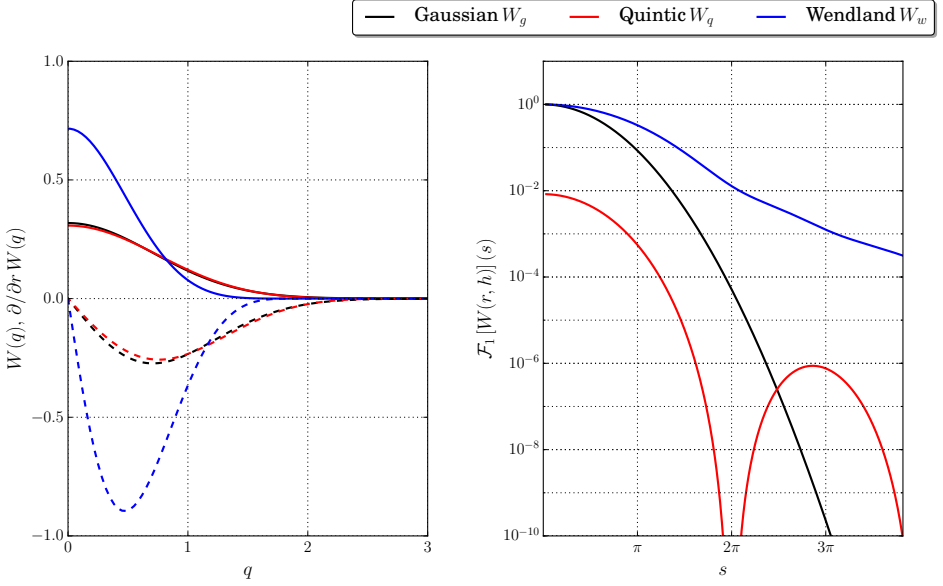
Figure 3.2: One-dimensional kernel functions W(q) with smoothing lengths set to unity h = 1 (left, Solid lines), their derivatives \partial/\partial r W(q) (left, Dashed lines) and respective one-dimensional Fourier transforms \mathcal{F}_1[W(r, h)](s) (right).
