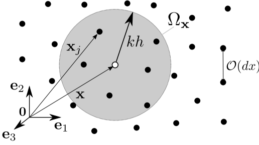
Figure 3.1: Schematic of the nodal integration scheme covering the compact support domain \Omega_{\mathbf{x}} of focal point \mathbf{x} .
