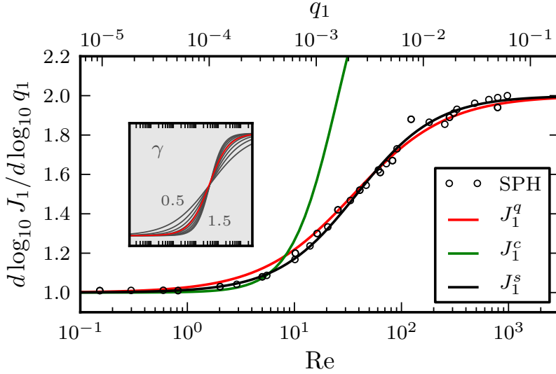
Figure 5.7: The dependence of the apparent exponent d \log_{10} J_1 / d \log_{10} q_1 on Re and the filter velocity q_1 . The red curve is derived using the best fitting Forchheimer Eq. (5.2). The green curve is derived using the best fitting cubic transition Eq. (5.3), with the fitting target being restricted to a maximum Re = 10 . The black curve is our postulated phenomenological logistic filtration law. Inset shows the dependence of the logistic curve on \gamma with the derived Forchheimer function (red) added for reference. Inset axes correlate exactly to the outer axes.
