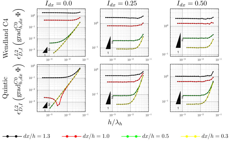
Figure 3.8: Empirical study of L^2 error convergence of the discrete, zeroth order complete gradient operator \text{grad}_{h,dx}^{C0} \Phi in two dimensional space as a function of non-dimensional smoothing length h/\lambda_h , numerical length scale ratio dx/h , grid point perturbation factor I_{dx} and kernel functions W_w and W_q .
