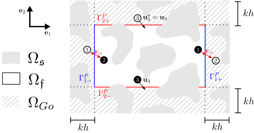
Figure 3.9: Schematic representation of periodic boundary conditions applied to a rectangular domain in two dimensions using the minimum image convention. The outer ghost domain \Omega_{Go} , the width of which is equal to the compact support radius kh , is populated with replicating ghost particles (open markers) that are replications of fluid points located in \Omega (closed markers).
