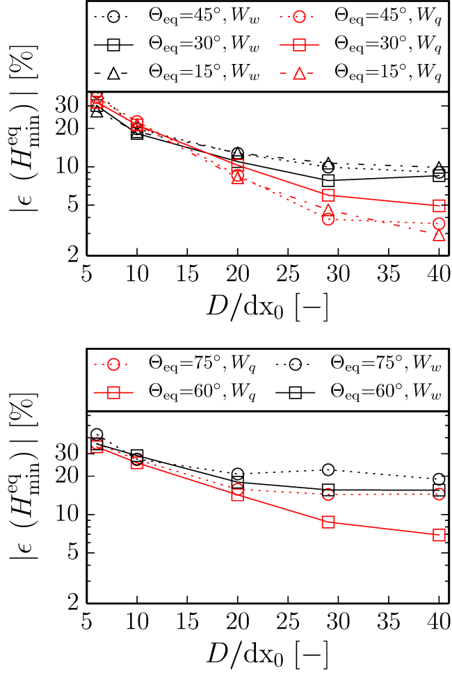
Figure 4.17: Absolute values of relative errors in numerical estimates of H_{\min}^{\text{eq}} as a function of resolution D/dx_0 .
