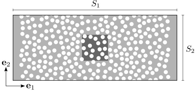
Figure 5.1: Computational domain proposed by Narváez et al. [147]. The domain is periodic in both \mathbf{e}_1 and \mathbf{e}_2 direction and the domain dimensions satisfy S_2 = 0.4 S_1 . The external force is applied in \mathbf{e}_1 direction. The fiber count equals 266. The centered dark gray area corresponds to the subdomain for which streamlines are shown in Fig. 5.4. Integration points are initially set up on a Cartesian lattice with 1280 and 512 points in \mathbf{e}_1 and \mathbf{e}_2 direction, respectively.
