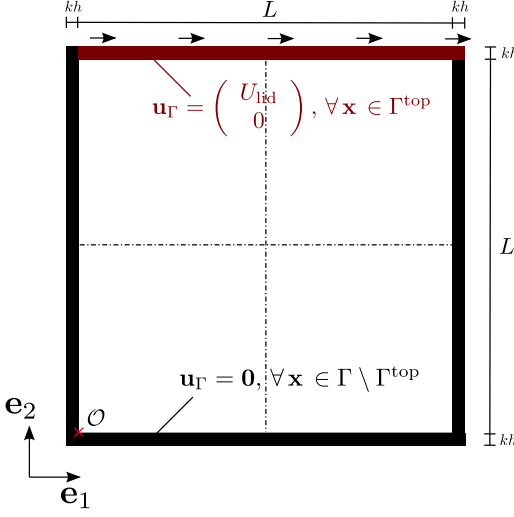
Figure 4.3: Simulation configuration for lid-driven square cavity flow. Flow within the fluid region, represented by the white area, is driven by the prescribed velocity \mathbf{u}_\Gamma = U_{\text{lid}}\mathbf{e}_1 of the upper boundary \Gamma^{\text{top}} , which is referred to as lid. The remaining boundaries \Gamma \setminus \Gamma^{\text{top}} remain impermeable and static. No-slip conditions apply to all boundaries of the fluid region. For further details on notation, see caption to Fig 4.1.
