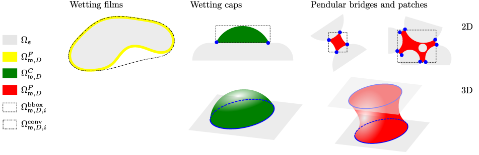
Figure 6.16: Schematic diagram of the proposed classification of hydraulically reservoir-disconnected wetting phase clusters into wetting films \Omega_{w,D}^F (yellow), wetting caps \Omega_{w,D}^C (green) and pendular clusters \Omega_{w,D}^P (red). Blue markers indicate contact points (2D) whereas blue lines indicate contact lines (3D). Minimum bounding box \Omega_{w,D,i}^{bbox} (dashed line) and convex hull \Omega_{w,D,i}^{conv} (dash-dot line) serve to identify cluster set membership.
