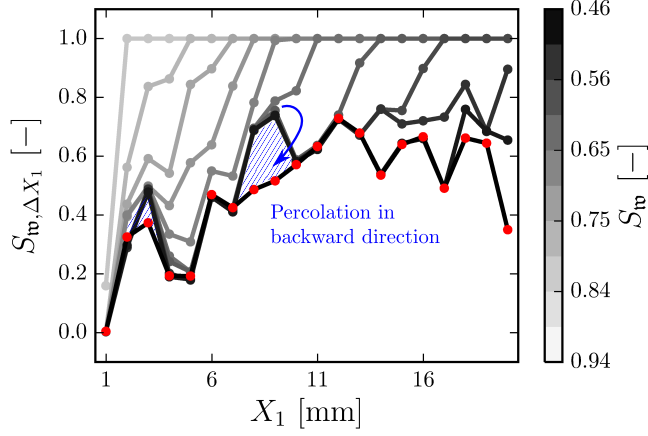
Figure 6.7: Evolution of saturation profiles in direction of \mathbf{e}_1 for microstructure A at Ca = 10^{-5} and M = 10^0 . Width of vertical slices \Delta X_1 = L_W/20 . Red markers indicate residual saturation profile at breakthrough.
