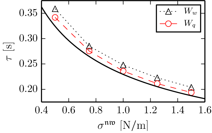
Figure 4.19: Numerical estimates of the period of oscillation as a function of interfacial tension \sigma^{nw} . Solid line represents theoretical prediction according to Eq. (4.11).
