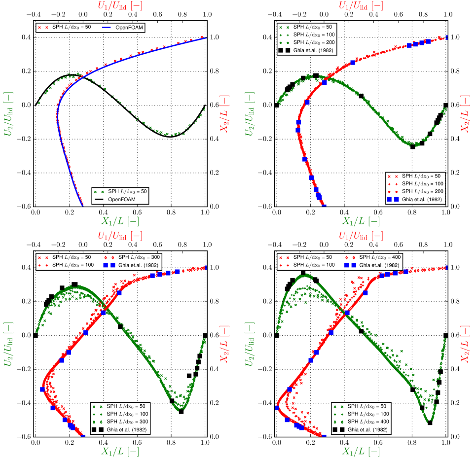
Figure 4.5: Normalized velocity profiles U_1(X_1/L = 0.5, X_2/L) (Red markers and blue lines) and U_2(X_1/L, X_2/L = 0.5) (Green markers and black lines) along vertical and horizontal symmetry lines of the square cavity, respectively, for Re = 1, 100, 400, 1000 (from top-left to bottom-right). Cross markers represent velocity components of SPH particles that are located within the narrow region \pm dx_0 from the central symmetry lines. Numerical reference results have been adopted from Ghia et al. [76] ( Re = 100, 400, 1000 , square markers) or computed using OpenFOAM [206] ( Re = 1 , solid lines). Numerical resolutions for SPH computations are given in terms of the ratio L/dx_0 .
