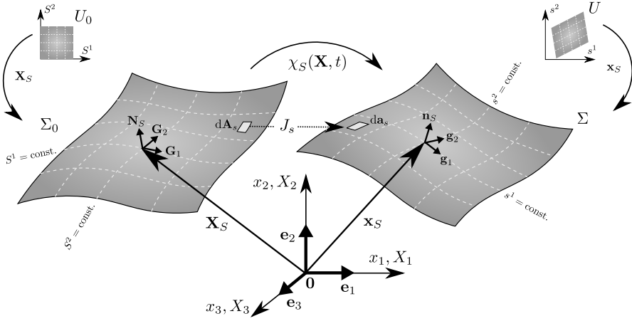
Figure 2.3: Schematic representation of motion of a surface through three-dimensional space, its reference and current configurations as well as the concept of mapping. The oriented differential surface area element of the reference configuration d\mathbf{A}_S = \mathbf{N}_S \cdot [d\mathbf{G}_1 \times d\mathbf{G}_2] , whereas in the current configuration d\mathbf{a}_s = \mathbf{n}_s \cdot [d\mathbf{g}_1 \times d\mathbf{g}_2] . Moreover, d\mathbf{A}_S = \|\mathbf{dG}_1 \times \mathbf{dG}_2\| dS^1 dS^2 and d\mathbf{a}_s = \|\mathbf{dg}_1 \times \mathbf{dg}_2\| ds^1 ds^2
