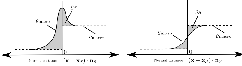
Figure 2.7: Schematic mass density concentration profiles plotted in direction of the normal \mathbf{n}_S for a multi-phase system with non-negligible concentration of surfactants (left) and a system with negligible interface-excess mass density (right).
