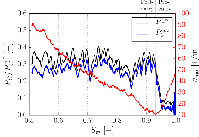
Figure 6.5: Normalized P_C(S_w) and a_{wn}(S_w) for primary drainage in microstructure C at Ca = 10^{-5} and M = 10^0 . Capillary pressures are normalized using the reference capillary pressure P_C^{\text{ref}} .
