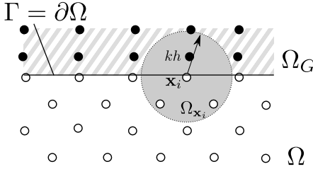
Figure 3.6: Schematic of the ghost particle approach whereby the set of sampling points is extended by spatially fixed ghost particles (closed markers) that are elements of the ghost domain \Omega_G .
