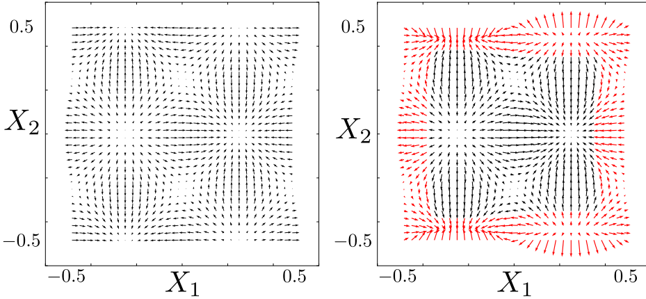
Figure 3.7: Analytic evaluation of the gradient field \text{grad } \Phi (left) and discrete reproducing approximation \text{grad}_{h,dx} \Phi (right) for \Phi = \sin(2\pi X_1) \cos(2\pi X_2) within the bounded domain \Omega = \{\mathbf{x} \in \mathbb{R}^2 \mid -0.5 \leq X_2, X_1 \leq 0.5\} . Red arrows highlight boundary particles that are prone to boundary inconsistency errors.
