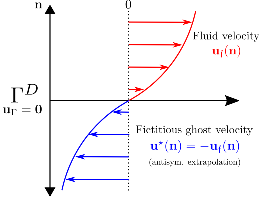
Figure 3.10: Schematic of fictitious velocity field (blue line) that is prescribed to ghost particles plotted in direction \mathbf{n} normal to the Dirichlet boundary. Fictitious velocities exhibit antisymmetry with respect to the fluid velocity field (red line) about the plane of symmetry \Gamma^D . Accounting for viscous momentum exchange between ghost particles and fluid particles subsequently reproduces the no-slip condition.
