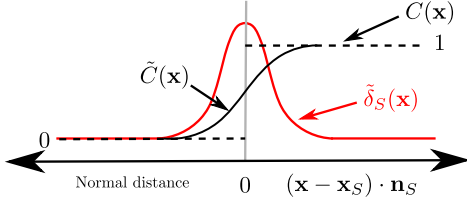
Figure 2.8: Schematic representation of the phase indicator field C(\mathbf{x}) , its smooth approximation \tilde{C}(\mathbf{x}) and modified surface Dirac distribution \tilde{\delta}_S(\mathbf{x}) .
