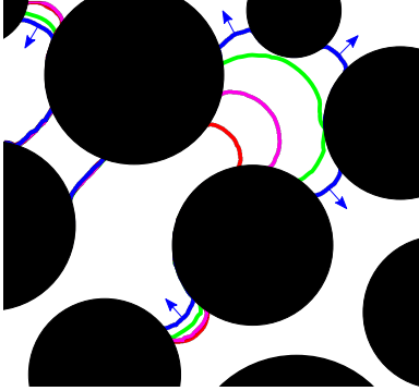
Figure 6.4: Evolution of \Gamma_{\text{wn}} during a Haines jump as observed in a subdomain of microstructure B having size 4.5 \text{ mm} \times 4.5 \text{ mm} for \text{Ca} = 10^{-5} and \text{M} = 10^{-1} . Arrows indicate direction of interfacial velocity. Menisci are initially located in pore-throats (Red contours) whereas an additional pore-body is observed to be drained post-event (Blue contours). Retraction of menisci from adjacent pore-throats suggests cooperative pore-filling. Despite it is not connected to the advancing finger, a pore-throat meniscus located near the upper edge of the plot retracts as well. Meanwhile, the trapped wetting cluster observed in the upper left-hand corner remains static. Time increment between superimposed contour plots amounts to 0.45 s. Plot was generated by linearly interpolating unstructured SPH particle data of phase indicator field C^{\text{wn}} to points of a regular grid using matplotlib.mlab.griddata and subsequently plotting contour lines C^{\text{wn}} = 0.5 .
