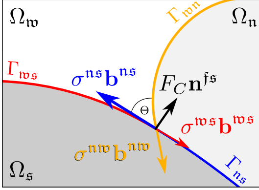
Figure 2.10: Schematic representation of concurrent forces comprised of boundary curve tractions \sigma^{\alpha\beta} \mathbf{b}^{\alpha\beta} and contact line constraining force F_C \mathbf{n}^{fs} acting on common point of contact line that is constrained to the solid-fluid interface.
