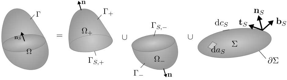
Figure 2.4: Schematic representation of a material domain \Omega comprised of two bulk phases \Omega_+ and \Omega_- with outer unit normal \mathbf{n} and a surface \Sigma representing an internal interface. The surface \Sigma is bounded by the boundary curve \partial\Sigma with unit tangent vector \mathbf{t}_S and unit vector \mathbf{b}_S = \mathbf{n}_S \times \mathbf{t}_S perpendicular to \partial\Sigma .
