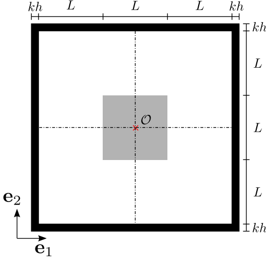
Figure 4.7: Simulation configuration for fully immersed liquid droplet. Black, white and gray areas correspond to fictitious solid phase \Omega_s , wetting phase \Omega_w and non-wetting phase \Omega_n , respectively. For further details on notation, see caption to Fig 4.1.
