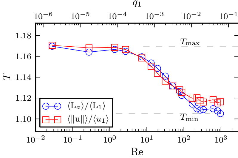
Figure 5.5: Dependence of the hydraulic tortuosity T on Re and the filter velocity q_1 . Upper bound estimate of the hydraulic tortuosity following Duda et al. [60] are marked red.
