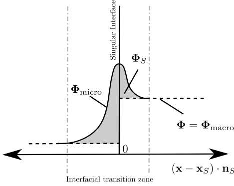
Figure 2.5: Schematic of a microscopic, continuous density field \Phi_{\text{micro}} and a macroscopic, discontinuous representation \Phi_{\text{macro}} in the vicinity of an interface plotted in direction of the normal \mathbf{n}_S according to Edwards et al. [63, see Fig. (3.6-3)]. In continuum models, the integral of the shaded region, termed interface-excess density \Phi_S , is assigned to a singular interface.
