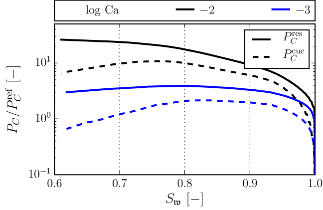
Figure 6.10: Normalized P_C^{\text{cuc}}(S_w) (dashed lines) and P_C^{\text{res}}(S_w) (solid lines) for primary drainage in microstructure C at M = 10^{-1} and various capillary numbers \text{Ca} (color coded).
