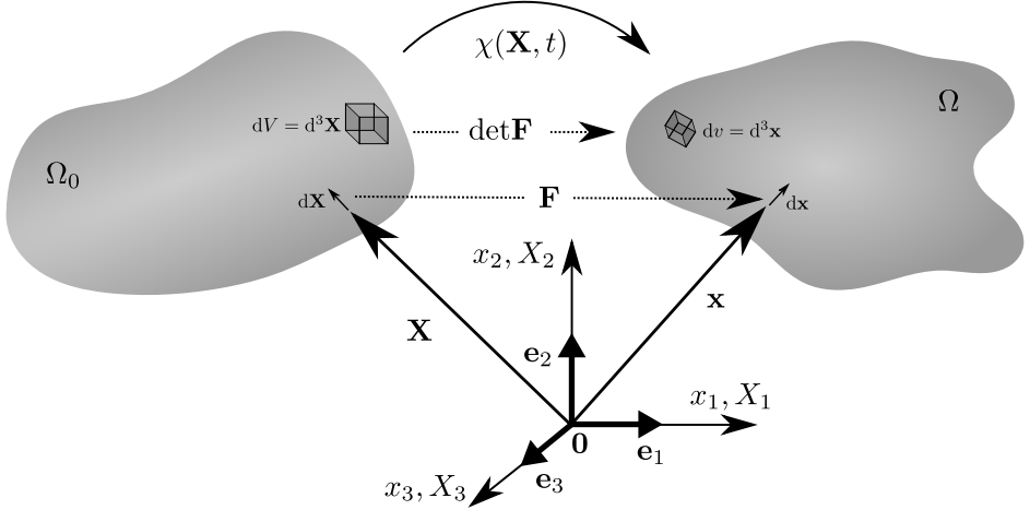
Figure 2.1: Schematic representation of motion of a material body, its reference and current configurations as well as the concept of mapping.
