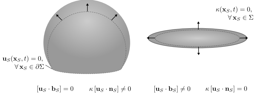
Figure 2.6: Interpretation of flux terms occurring in the transport theorem for surfaces. For the deformation mode depicted on the LHS, the boundary curve integral in Eq. (2.45) vanishes. For the deformation mode depicted on the RHS, the second surface integral in Eq. (2.45) vanishes.
