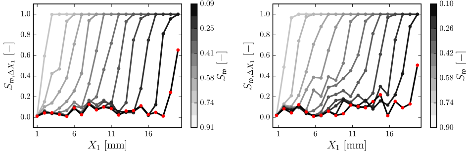
Figure 6.12: Evolution of saturation profiles in direction of \mathbf{e}_1 for microstructure A (left) and C (right) at \text{Ca} = 10^{-2} and M = 10^1 . Among the set of tested microstructures, microstructure A exhibits the narrowest fiber diameter distribution and microstructure C the widest. Width of vertical slices \Delta X_1 = L_W/20 . Red markers indicate residual saturation profile at breakthrough.
