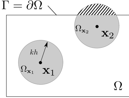
Figure 3.5: Schematic of truncation of the compact kernel support domain \Omega_{\mathbf{x}} by the computation domain boundary \Gamma leading to boundary inconsistency errors.
