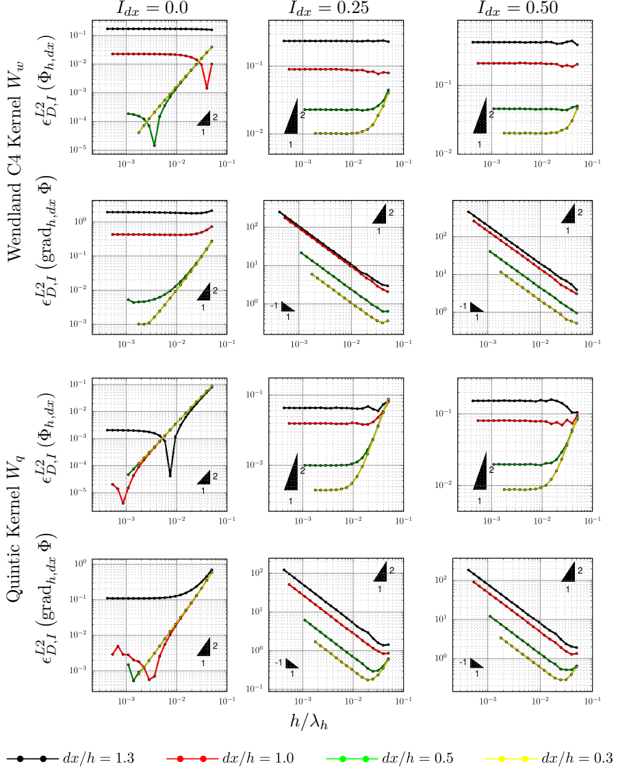
Figure 3.4: Empirical study of L^2 error convergence of the discrete reproducing approximations \Phi_{h,dx} and \text{grad}_{h,dx}\Phi in two dimensional space as a function of non-dimensional smoothing length h/\lambda_h , numerical length scale ratio dx/h , grid point perturbation factor I_{dx} and kernel functions W_w and W_q .
