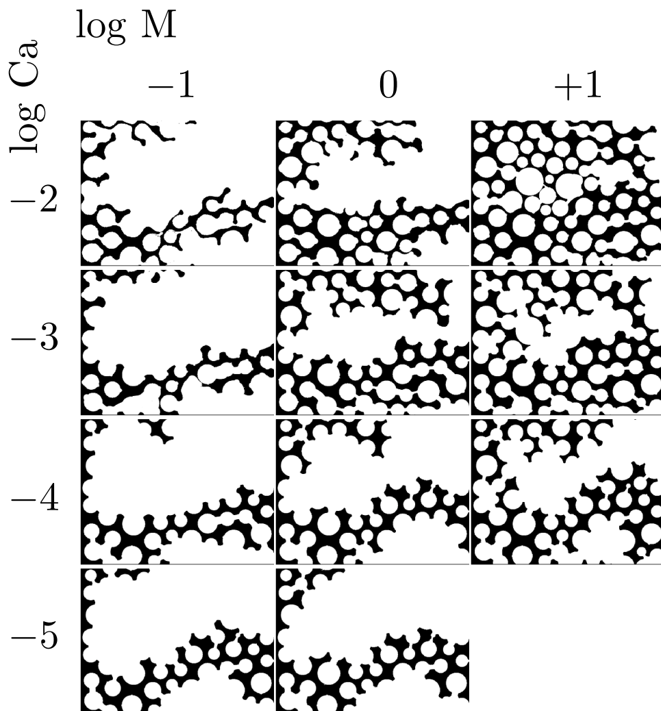
Figure 6.3: Non-wetting phase distribution at breakthrough for microstructure C. Domain \Omega_n is colored black whereas both \Omega_s and \Omega_w are colored white.
