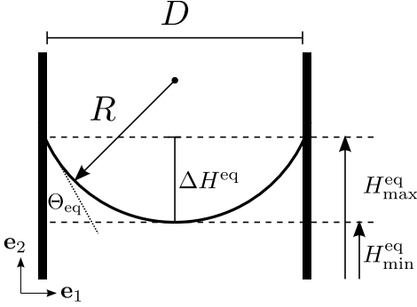
Figure 4.15: Schematic diagram of a meniscus located between two parallel plates that are separated by a narrow gap width D , introducing minimum and maximum capillary rise heights H_{\min} and H_{\max} , respectively. H_{\min} and H_{\max} are measured with respect to the reference height H_{\text{ref}} of the reservoir.
