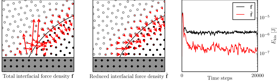
Figure 2.11: Close-up of equilibrium SPH solutions of a wetting fluid droplet on a planar solid substrate. Open circle, filled circle and filled diamond markers represent the SPH particle positions of the non-wetting phase, wetting phase and solid phase, respectively. Lengths and directions of the arrows represent the magnitude and direction of the interfacial force density field, respectively. (left) Solution using the total interfacial force density \mathbf{f} following Eq. (2.94). (middle) Solution using the reduced interfacial force density \tilde{\mathbf{f}} following Eq. (2.93). (right) Evolution of total kinetic energy over the number of time steps.
