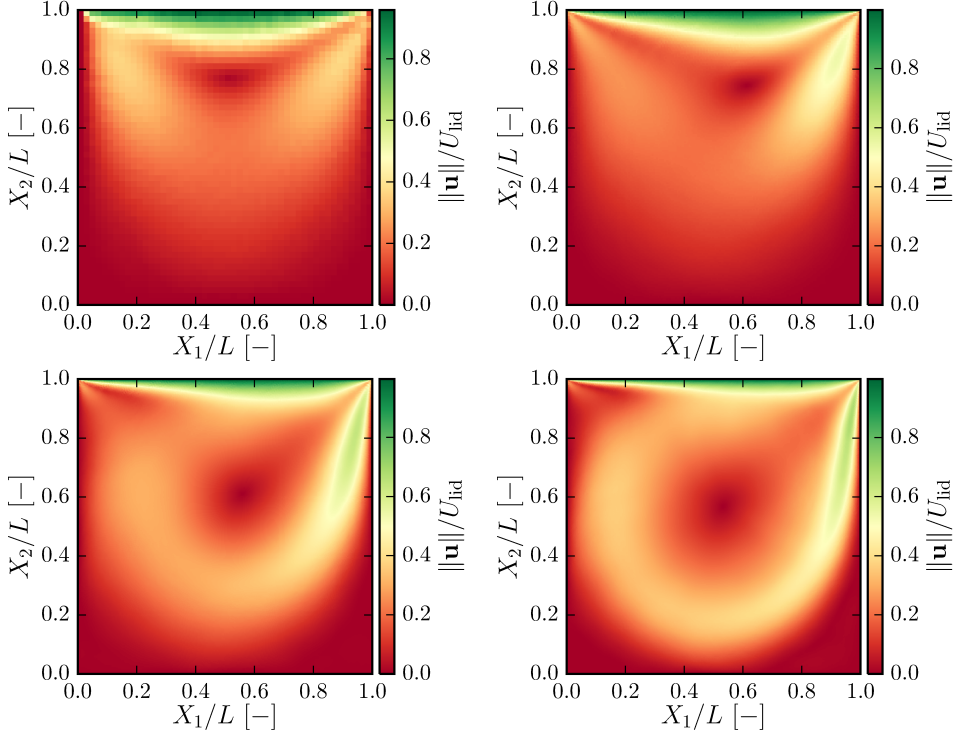
Figure 4.4: Normalized velocity magnitudes during lid-driven square cavity flow for \text{Re} = 1, 100, 400, 1000 (from top-left to bottom-right). Plot was generated by linearly interpolating unstructured SPH particle data of particle velocities to points of a regular grid using matplotlib.mlab.griddata and subsequently plotting the scalar field of normalized fluid velocity magnitudes.
