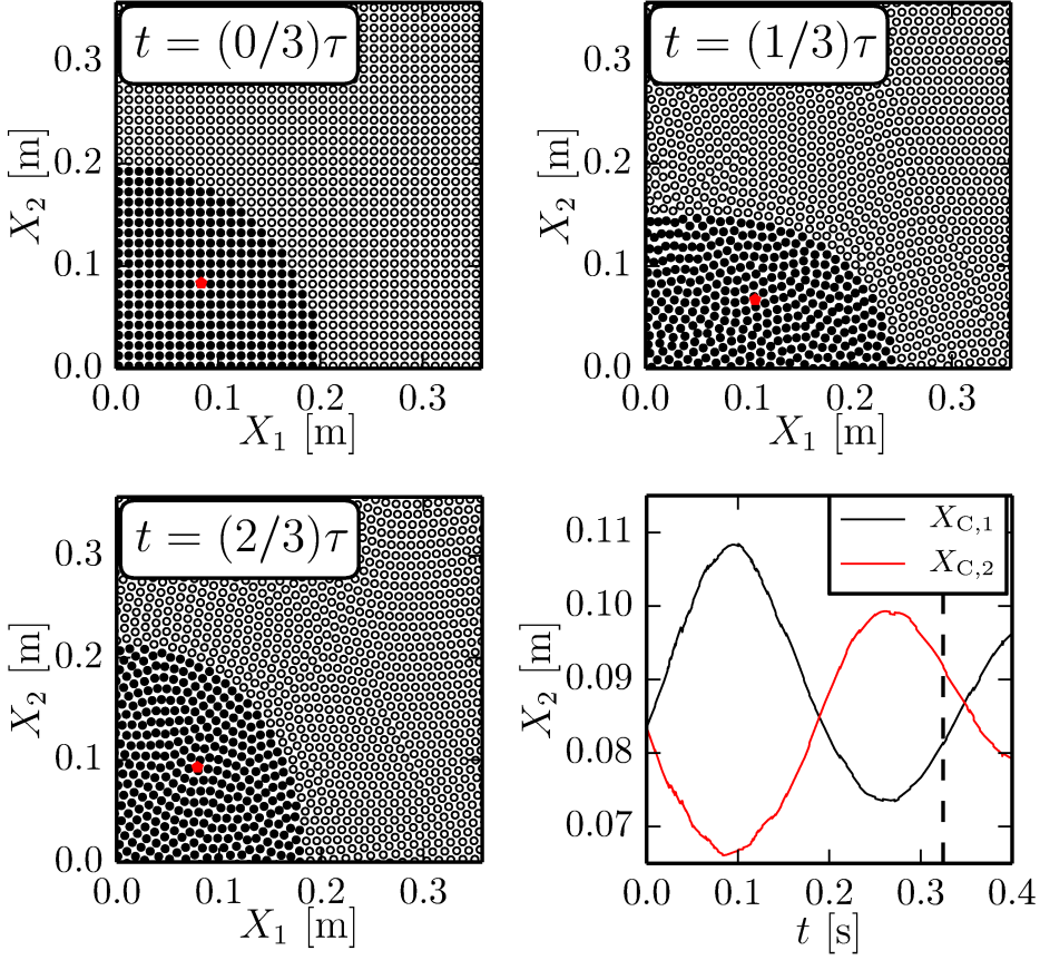
Figure 4.20: Close-up plots of particle positions indicating the mode of oscillation in the upper right-hand quarter X_1 > 0, X_2 > 0 at times t = 0.0 , t = \tau/3 and t = 2\tau/3 for \sigma^{\text{wn}} = 0.5 N/m and W = W_w . Filled and open markers represent particles of the droplet and surrounding medium, respectively, while the red markers indicate the center-of-mass position of the upper right-hand quarter of the droplet. Plot in bottom-right corner shows corresponding center-of-mass coordinates ( X_{C,1}, X_{C,2} ) as a function of time, where the vertical dashed line indicates the predicted value of \tau according to Eq. (4.11).
