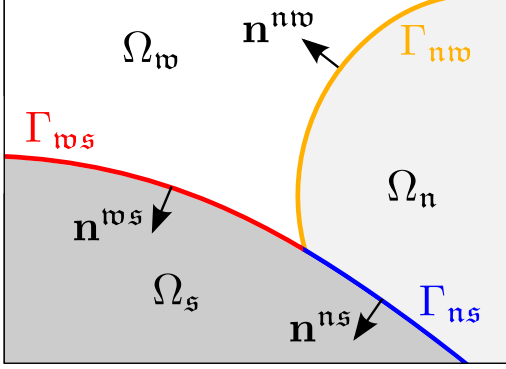
Figure 2.9: Schematic diagram introducing the notation for bulk phases, interfaces \Gamma_{\alpha\beta} and interfacial unit normals \mathbf{n}^{\alpha\beta} with respect to a three-phase system as encountered during multi-phase flow in porous media. The indicator \alpha\beta \in \{\text{nw}, \text{ns}, \text{ws}\} , whereas \mathfrak{s} denotes the bulk solid phase and \mathfrak{n} and \mathfrak{w} denote bulk fluid phases.
