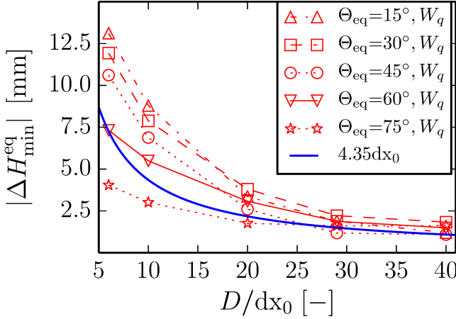
Figure 4.18: Absolute values of the absolute errors in numerical estimates of H_{\min}^{\text{eq}} as a function of resolution D/dx_0 , where results for W = W_w are omitted for the sake of clarity. Solid blue line represents the compact support size of the quintic kernel kh = 4.35 dx_0 . The absolute error is defined to be \Delta(\bullet) = (\bullet)_{\text{exact}} - (\bullet)_{\text{est.}} , where (\bullet)_{\text{exact}} and (\bullet)_{\text{est.}} represent exact solution and numerical estimate, respectively.
