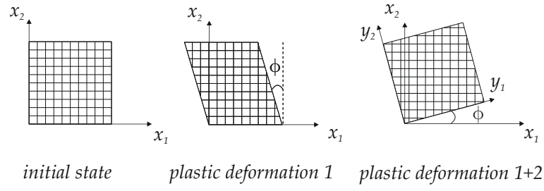
Figure 3.16.: Gedankenexperiment
