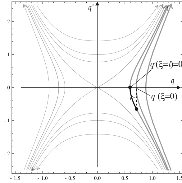
Figure 5.5.: Phase portrait.
