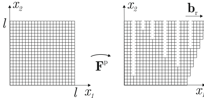
Figure 5.2.: Plastically deformed crystal including dislocations, reprinted by permission from [59]
