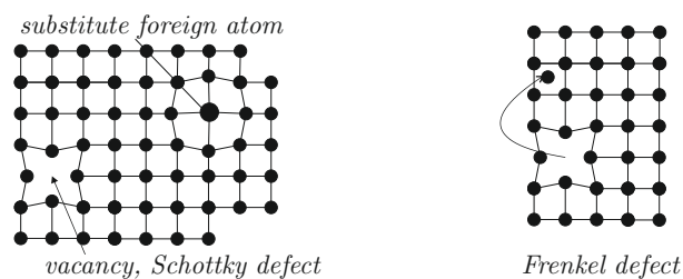
Figure 3.5.: Zerodimensional effects
