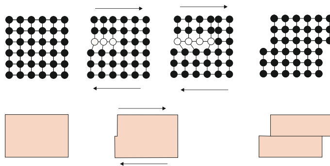
Figure 3.7.: Movement of dislocation causes plastic slip
