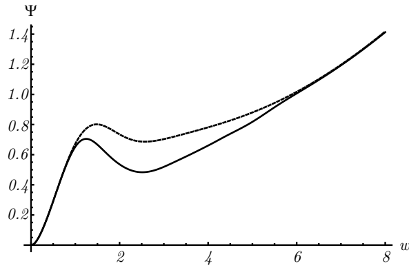
Figure 4.22.: Comparison of relaxed and unrelaxed energy
