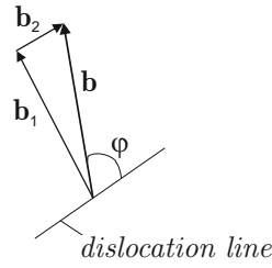
Figure 3.13.: Mixed Burgers vector
