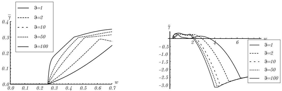
Figure 4.30.: Zoom in and total view of total amount of plastic slip for a shear test under several pseudo-velocities.
