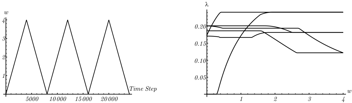
Figure 4.74.: Three load cycle of tension-compression and corresponding evolution of volume fraction of domain two.
