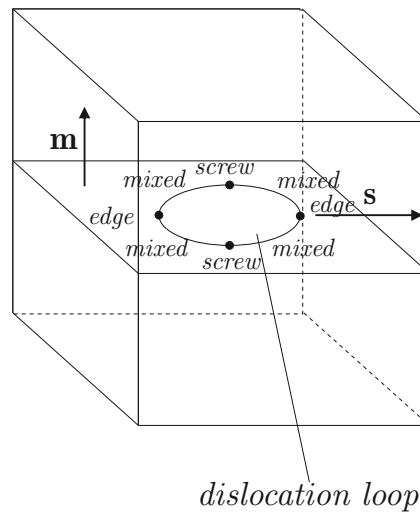
Figure 3.12.: Dislocation loop
