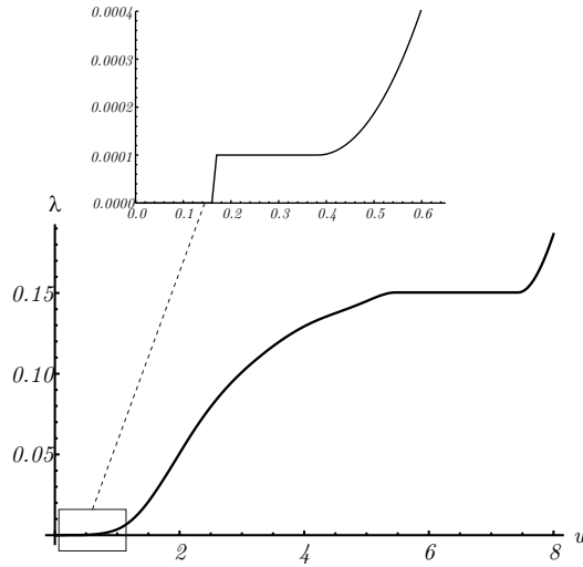
Figure 4.18.: Volume fraction of the second domain for a tension-compression test
