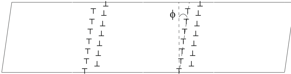
Figure 5.25.: Dislocation arrays in deformed crystal, reprinted by permission from [60].
