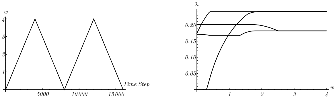
Figure 4.70.: Two load cycles of tension-compression and corresponding evolution of volume fraction of domain two.
