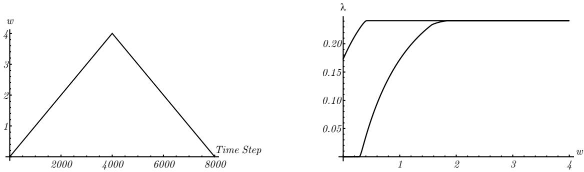
Figure 4.66.: One load cycle of tension-compression and corresponding evolution of volume fraction of domain two.
