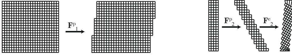
Figure 5.23.: The sequences of deformations in both phases, reprinted by permission from [60].
