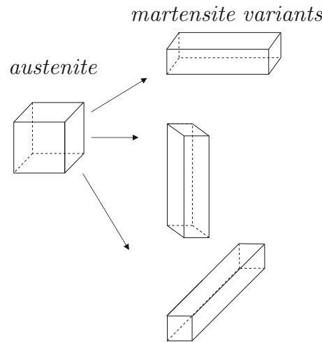
Figure 3.20.: Tetragonal martensite variants.
