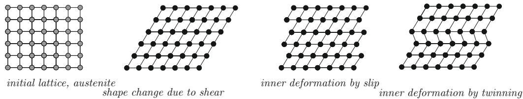
Figure 3.21.: Martensitic transformation
