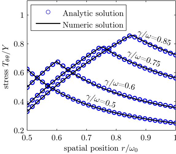
Figure 6.9: Distribution of the circumferential stress component T_{\theta\theta} in case of different loading conditions for the numerical and the analytical approach.
