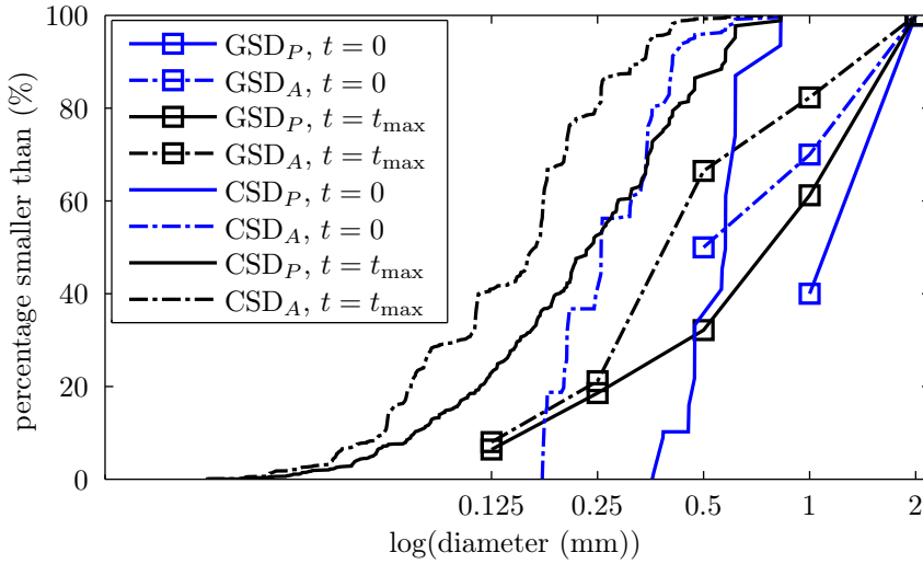
Figure 5.12: Evolution of the morphology, here described by the GSD and CSD, induced by infiltration of a suspension in two different points of the domain in Figure 5.11.
