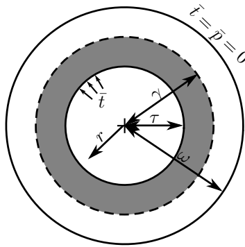
Figure 6.7: Boundary Value Problem (expansion of a cylindrical tube) to compare the numerical approach with an analytical solution in case of ideal plastic yield function using Tresca criterion.
