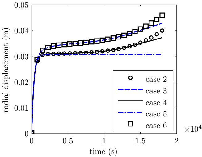
Figure 6.12: Distribution of the displacement of the porous skeleton at a point on the interface of the grout and solid domain for different cases defined in Table 6.3.
