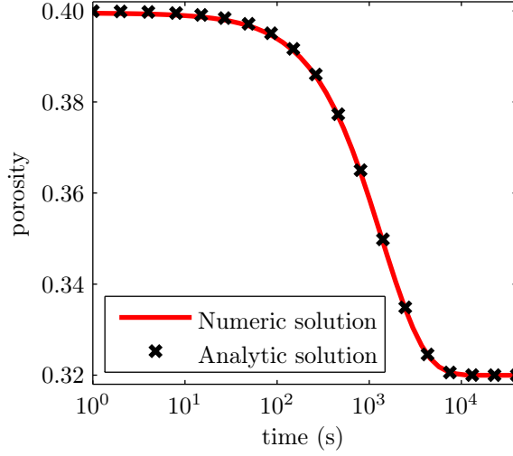
Figure 6.6: Numerical and analytical solution for the time depended evolution of porosity of the 0-dim infiltration approach.
