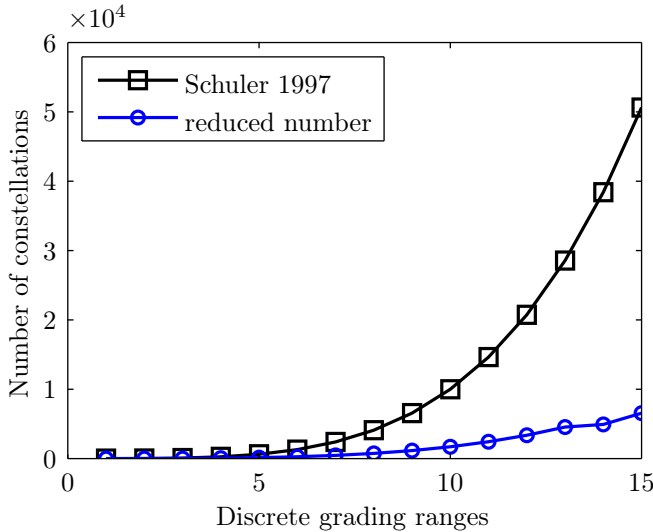
Figure 5.2: Comparison of all possible constellations resulting from permutation of f fractions (cf. Schuler [75]) with the number of physical unique constellations.
