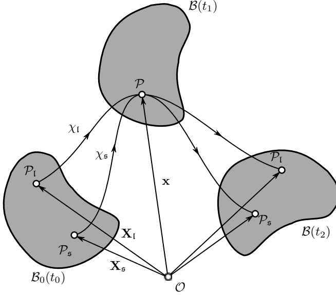
Figure 3.1: Kinematics of a two-phase mixture \alpha = \{s, l\} , with time t_0 < t_1 < t_2 . The motion of each constituent \varphi^\alpha is described by an individual motion function \chi_\alpha , with \mathcal{P}_\alpha depicting the spatial position of the constituent \varphi^\alpha within the body of the mixture \mathcal{B} .
