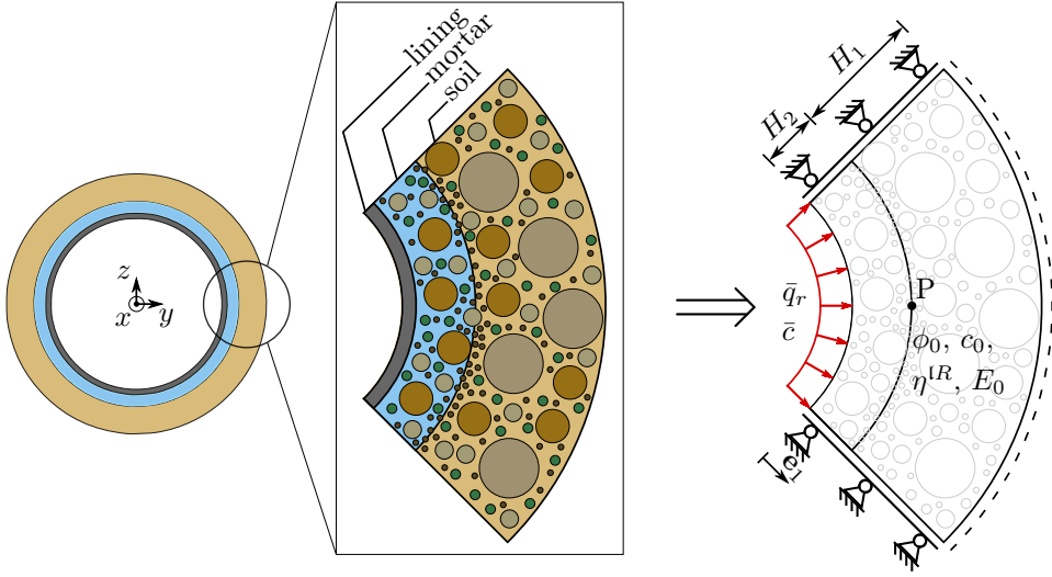
Figure 6.10: From the application (left) to a numerical IBVP (right). Homogenization and boundary conditions for the IBVP.
