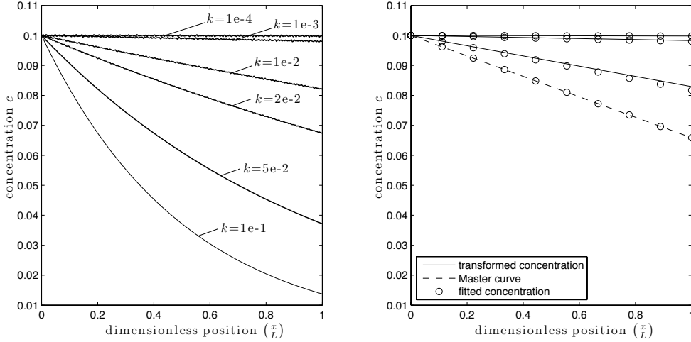
Figure 4.4: Distribution of the concentration c_{eq} at equilibrium, left: calculated concentration distribution, right: fitted and transformed concentration distribution.
