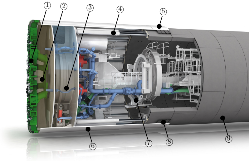
Figure 2.1: Longitudinal section of a Mix-shield TBM, with: ①: cutter head, ②: excavation chamber, ③: pressure chamber, ④: hydraulic jacks, ⑤: tail skin, ⑥: shield, ⑦: tubbing erector, ⑧: brush sealing, ⑨: tunnel lining. ( Copyright: www.herrenknecht.com )
