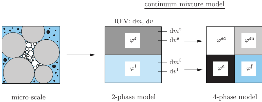
Figure 4.1: Microscale and RVE of a fully-saturated soil and the corresponding four-phase continuum model, from [71, 82].
