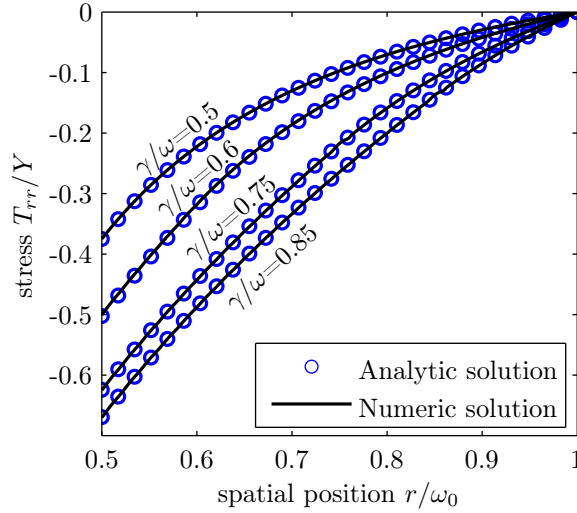
Figure 6.8: Distribution of the radial stress component T_{rr} in case of different loading conditions for the numerical and the analytical approach.
