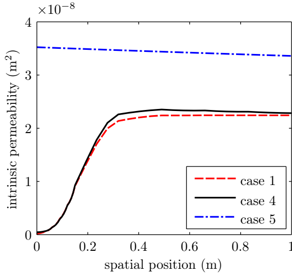
Figure 6.11: Distribution of the intrinsic permeability for the last time step of the simulation along the \mathbf{e}_1 direction, cf. Figure 6.10. The definition of the corresponding cases is given in Table 6.3.
