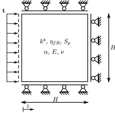
Figure 6.3: Illustration of the 1-dim IBVP and used boundary and initial conditions.
