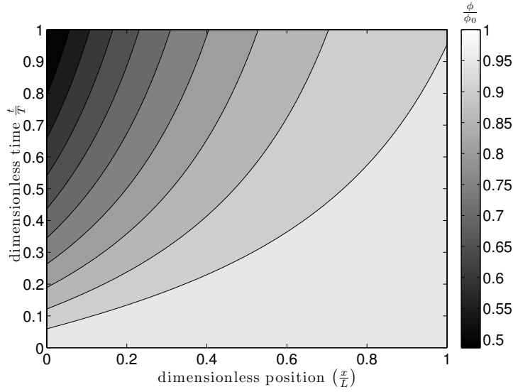
Figure 4.3: Contour plot describing the evolution of the porosity in space and time in the domain.
