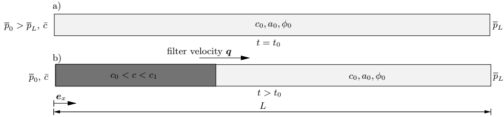
Figure 4.2: Infiltration process: a) initial and boundary conditions for the investigated domain; b) illustration of the concentration profile for t > t_0 .
