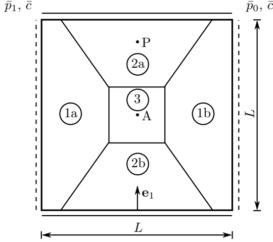
Figure 5.11: Visualization of the computed 2-dim IBVP.
