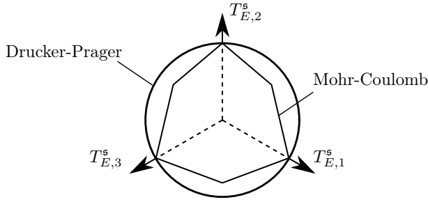
Figure 3.2: Yield surface according to Mohr-Coulomb and Drucker-Prager criterion, illustrated in the plane created by the principal-extra stresses T_{E,1}^s, T_{E,2}^s, T_{E,3}^s (adapted from [108]).
