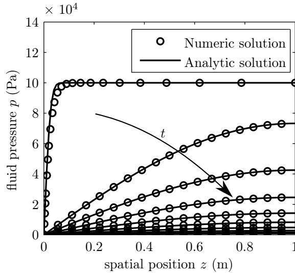
Figure 6.4: Comparison of the analytical and the numerical solution of Terzaghi's consolidation problem. The results of the pressure distribution of both approaches is plotted for the same times. The time step is determined based on the consolidation time \Delta t = 0.1 \times t_{\max} .
