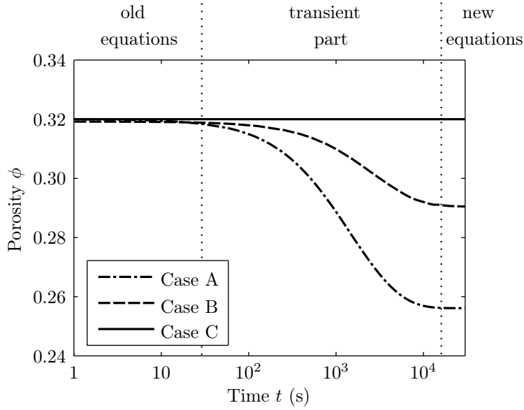
Figure 5.9: Evolution of porosity due to different micro structures. the description of the single cases is given in Figure 5.8.
