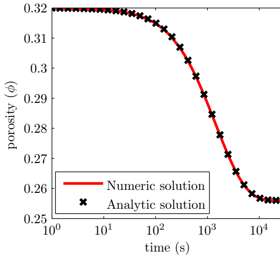
Figure 5.6: Comparison of the numerical and analytical solution for a 0-dim infiltration IBVP.
