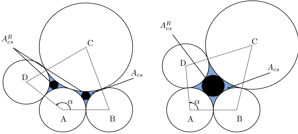
Figure 5.1: Visualization of two possible pore constrictions, the area of a pore constriction A_{cs} (blue), and the area of an effective pore constriction A_{cs}^R (black). Left: densest pore constellation. Right: loosest pore constellation.
