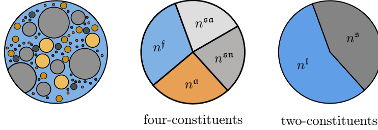
Figure 6.2: Fully saturated RVE representing a soil material (left), its homogenization within the TPM, according to Steeb [82], as a four-constituent approach, with \alpha = \{\mathbf{sa}, \mathbf{sn}, \mathbf{a}, \mathbf{f}\} (middle), and the two-constituent approach, with \beta = \{\mathbf{l}, \mathbf{s}\} (right).
