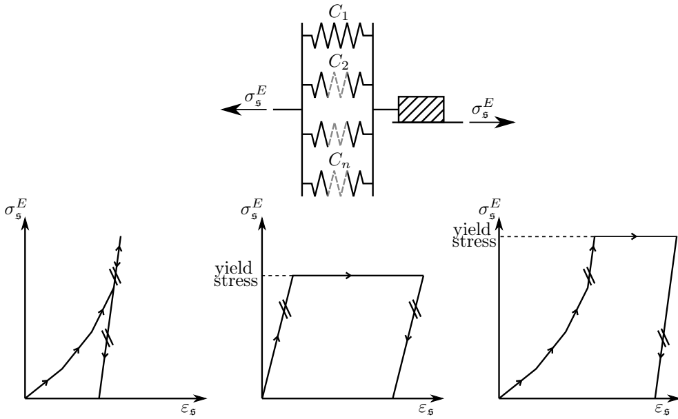
Figure 6.1: Details of numerical implementation of plastic behaviour of the solid skeleton and its stiffening due to infiltration. Upper part: rheological model capturing stiffening and plasticity simultaneously. The stiffening behaviour is represented by in parallel connected spring elements and the plastic deformation by the friction element. Lower part: stress-strain curves of a stiffening (left), plastic solid material (middle), and the superposition of both effects (right).
