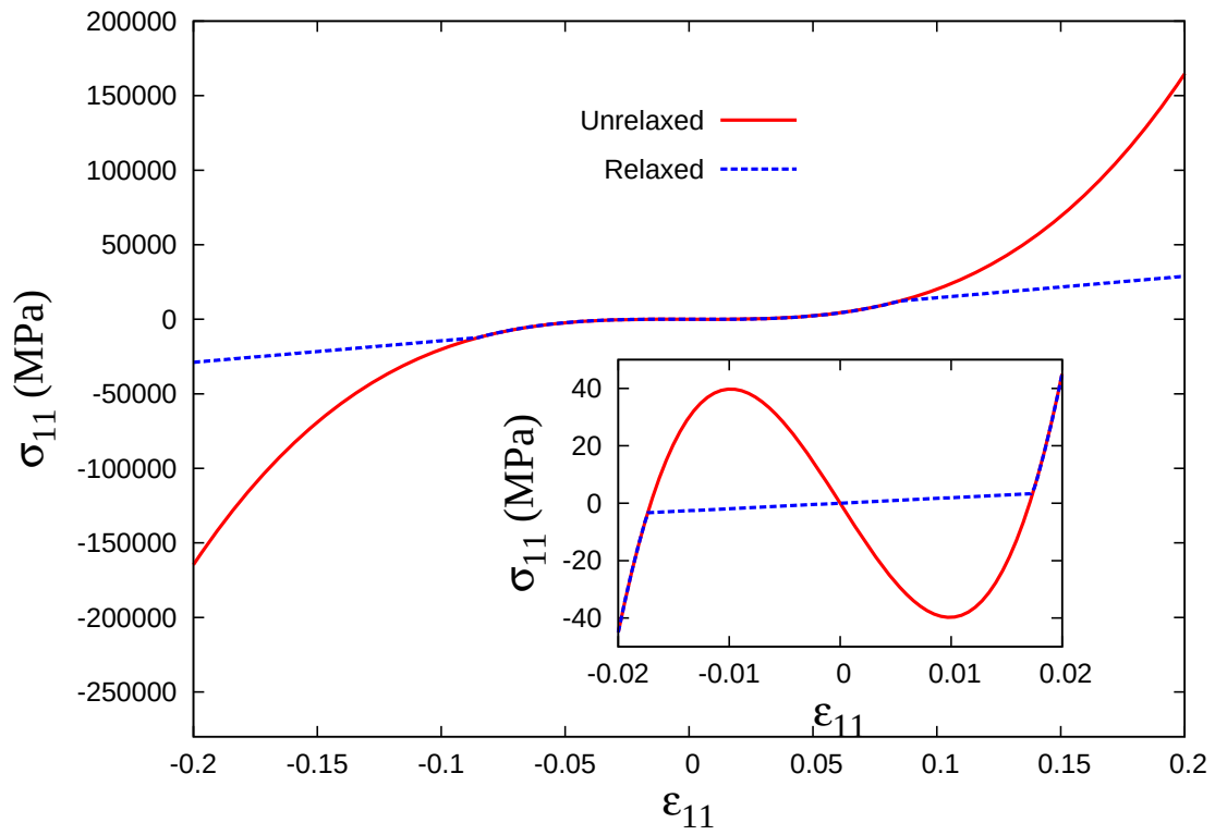
Figure 3.13.: Relaxed and unrelaxed stress-strain curves in tension-compression test.
