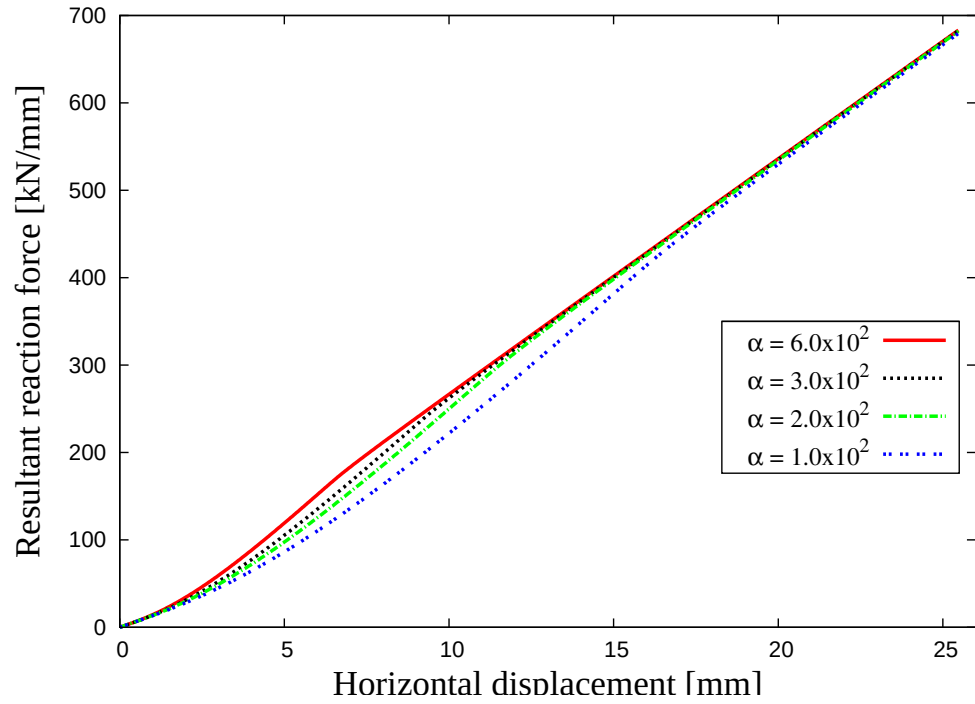
Figure 5.7.: Load-displacement curves obtained from different simulations performed with varying the values of the material parameter \alpha .
