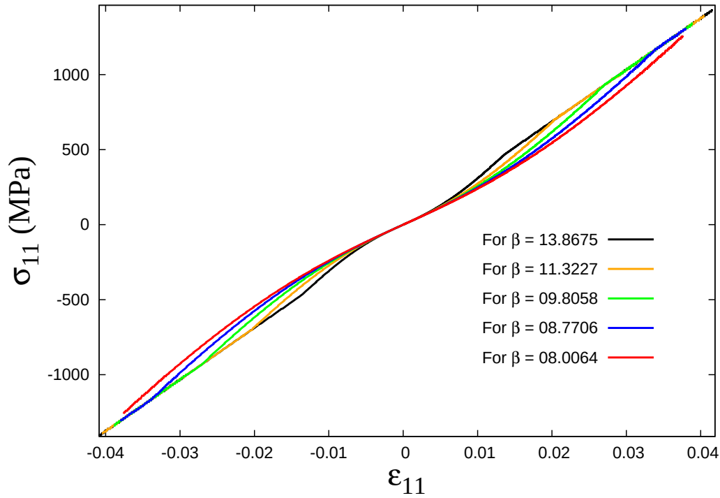
Figure 5.10.: Stress-strain response of the notched plate with a central hole subjected to tension with varying particle size.
