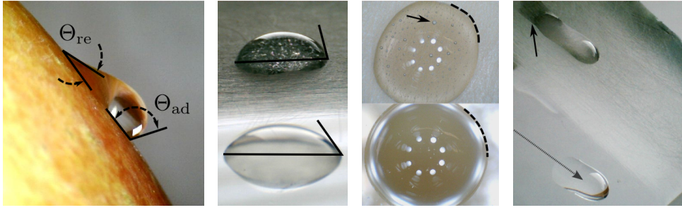
a) Receding and advancing contact angle b) Different contact angles c) Trapped air and distorted circular shape on a rough surface d) Rough surface requires a steeper slope for moving and causes a water film
