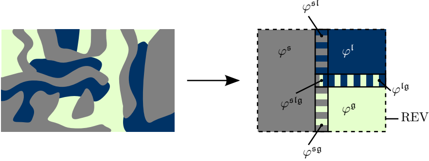
Figure 5.1: Schematic visualization of the modeling concept for a macroscopic, partially saturated system.
