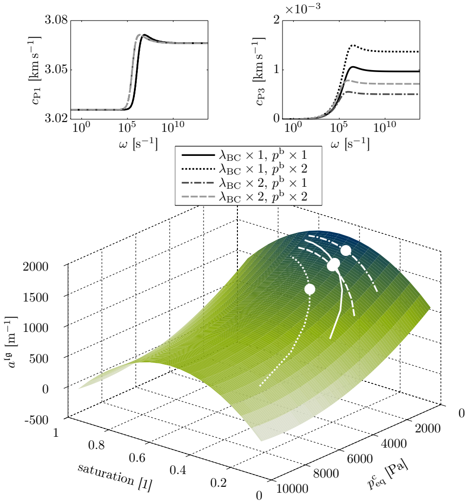
Figure 6.7: P1- and P3-wave phase velocities for different p_{eq}^c - s^l paths realized by different Brooks & Corey parameters (top). The paths are indicated at the a^{lg} - p_{eq}^c - s^l surface of the pore network model in [102] (bottom).
