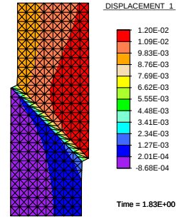
f. Mixed-CST element.
