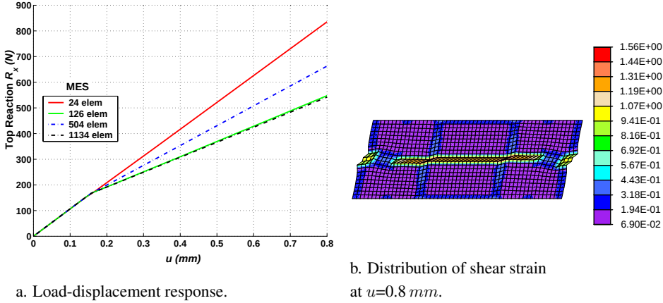
Figure 7.8.: Model based on the assumption of D = A^2 \mathcal{I} and m.n = 0 : Localization within shear test by use of MES element (the mixed enhanced strain method).
