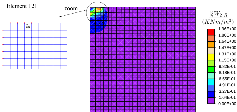
b. Distribution of relaxed energy at the first Gauss point at v = 0.1556 \text{ m} .
