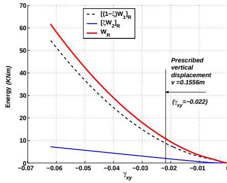
a. Relaxed energy-shear strain at the first Gauss point of the element 121.
