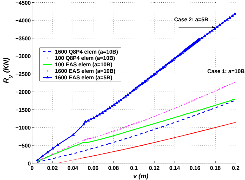
Figure 9.2.: Load-displacement response.
