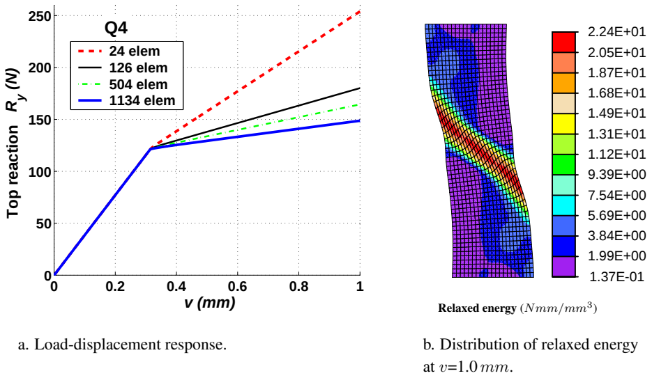
Figure 7.12.: Model based on the assumption of \mathbf{D} = A^2 \mathbf{I} and \mathbf{m.n} = 0 : Localization in tension by use of Q4 element (the displacement method).
