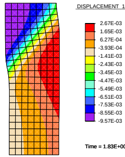
e. Mixed-Q4 element.
