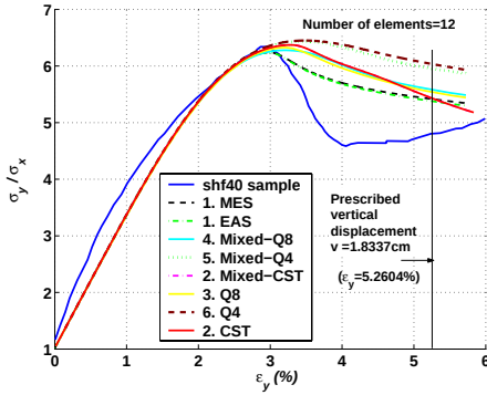
a. Stress-strain curve.
