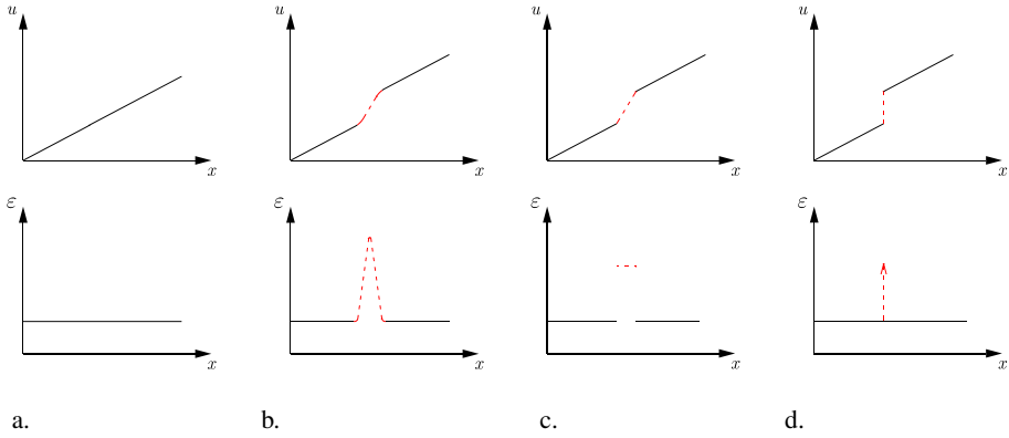
Figure 2.6.: Kinematics description with (a) and (b) no discontinuity, (c) two weak discontinuities, (d) one strong discontinuity in one-dimensional problem.
