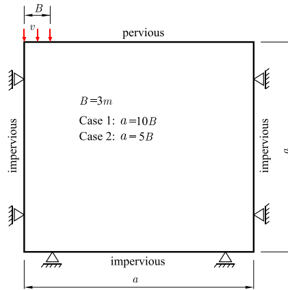
Figure 9.1.: Saturated soil foundation problem: Geometry and boundary conditions.
