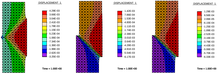
a. Tolerance = 1.E-6, 1.E-8 and 1.E-10, respectively.
