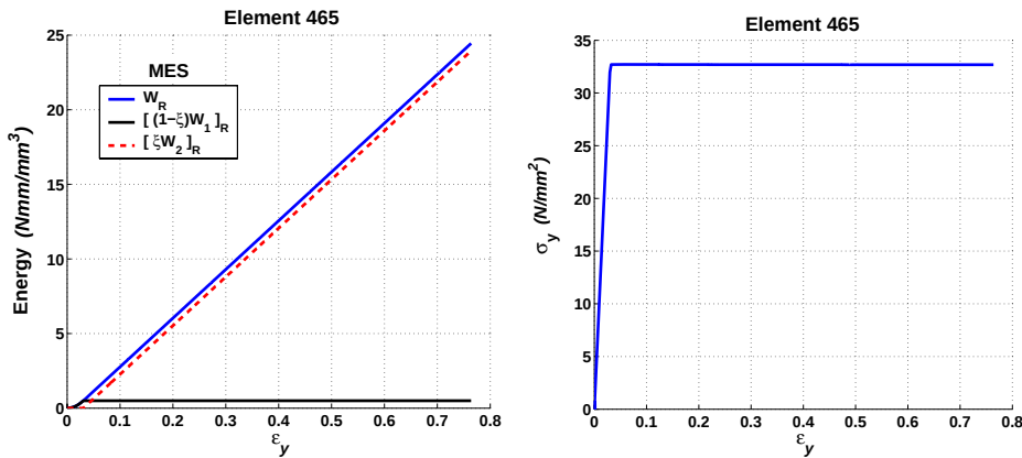
Figure 7.23.: Model based on the assumption of D = \mathcal{C} : Relaxed energy and relaxed normal stress \sigma_y by use of MES element (the mixed enhanced strain method) at the first Gauss point of the element 465.
