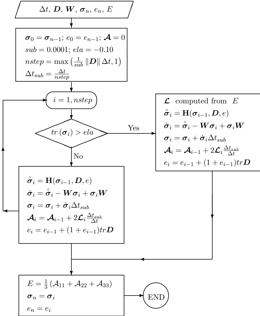
Figure 4.1.: Flow chart of the time integration scheme with the sub-time stepping algorithm proposed by Nübel et al. , 1998[83].
