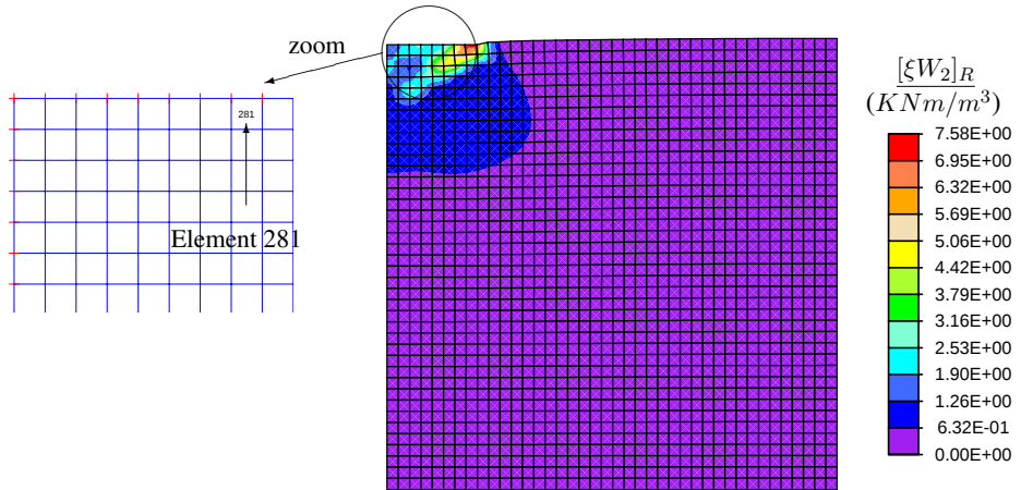
b. Distribution of relaxed energy at the first Gauss point at v = 0.1556 m .
