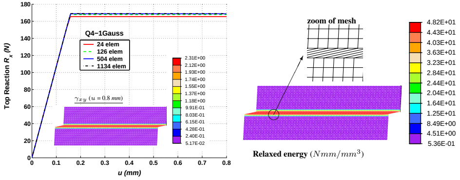
a. Load-displacement response and distribution of shear stress at u=0.8 mm.
