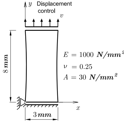
Figure 7.11.: Localization in tension. Geometry and boundary conditions.
