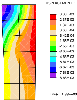
d. Mixed-Q8 element.
