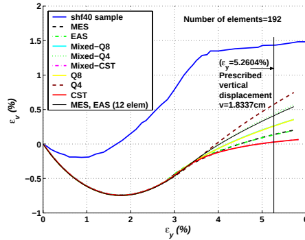
b. Volumetric strain-axial strain.
