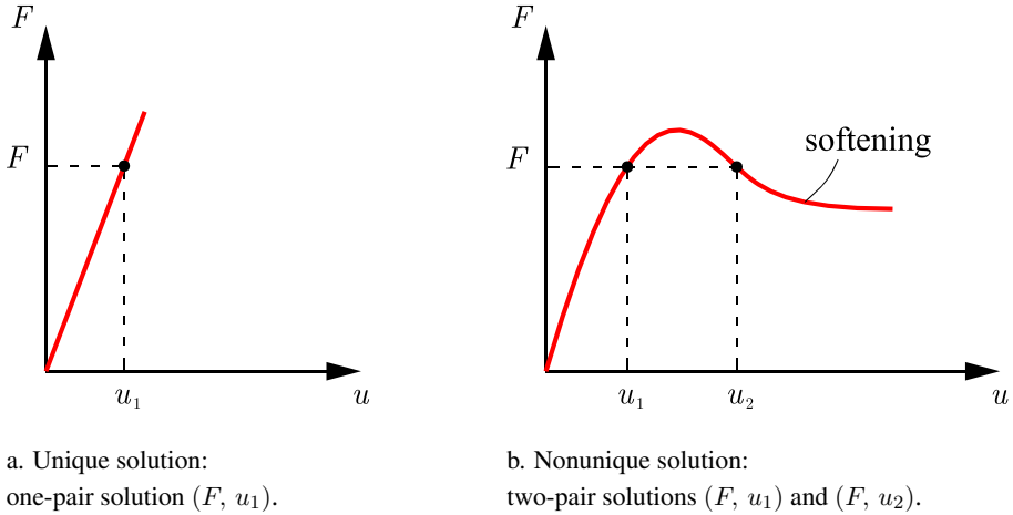
Figure 2.7.: Uniqueness and nonuniqueness.
