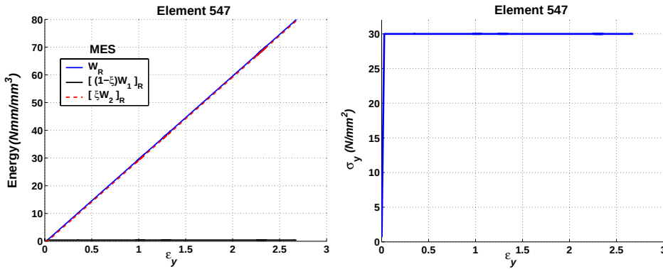
Figure 7.20.: Model based on the assumption of D = A^2\mathcal{I} and -1 \leq m.n \leq 1 : Relaxed energy and relaxed normal stress \sigma_y by use of MES element (the mixed enhanced strain method) at the first Gauss point of the element 547.
