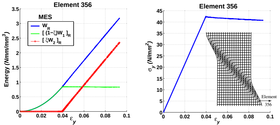
Figure 7.16.: Model based on the assumption of \mathbf{D} = A^2 \mathbf{I} and \mathbf{m} \cdot \mathbf{n} = 0 : Relaxed energy and relaxed normal stress \sigma_y by use of MES element (the mixed enhanced strain method) at the first Gauss point of the element 356.
