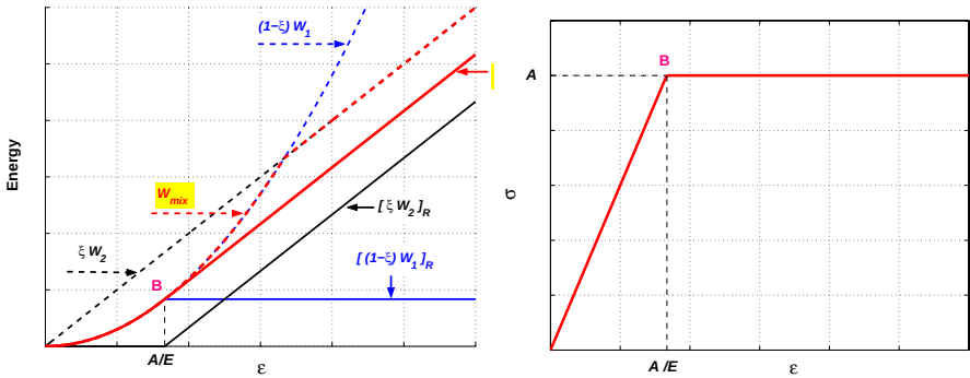
Figure 7.4.: Relaxed energy and stress in one-dimensional problem.
