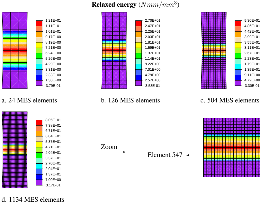
Figure 7.19.: Model based on the assumption of D = A^2\mathcal{I} and -1 \leq m.n \leq 1 : Localization within tension test by use of MES element(the mixed enhanced strain method). Comparison of the different finite element meshes: Distribution of relaxed energy at v = 1.0\text{ mm} .
