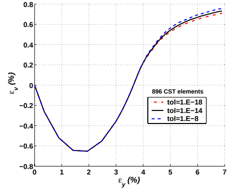
b. Volumetric strain-axial strain.
