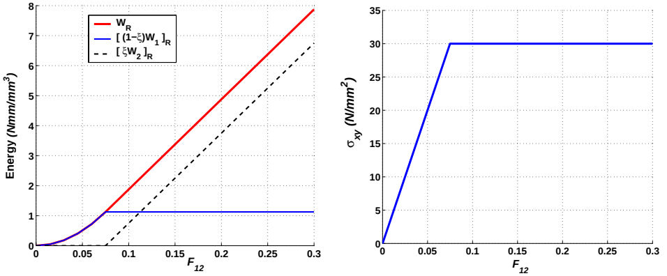
Figure 8.2.: Incompressible Neo-Hookean model: Relaxed energy and relaxed shear stress
