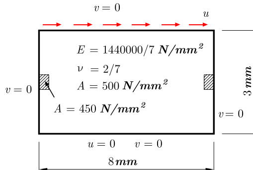
Figure 8.3.: Localization within shear test. Geometry and boundary conditions.
