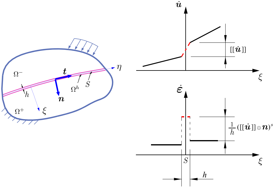
Figure 6.1.: Regularized strong discontinuity [87]
