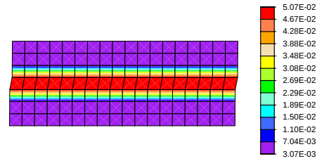
b. 126 Q4 and Mixed-Q4 elements
