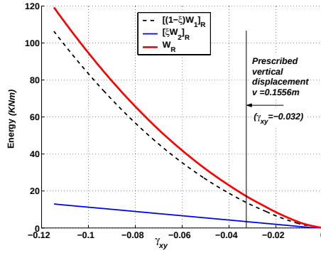
a. Relaxed energy-shear strain at the first Gauss point of the element 121.
