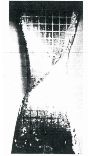
Figure 2.5.: Localized shearing and the inception of shear failure during uniaxial tension of a single crystal of pure copper ( Lisiecki et al., 1982 [3, 69]).
