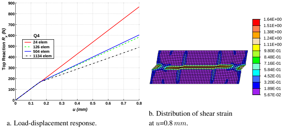
Figure 7.9.: Model based on the assumption of D = A^2 \mathcal{I} and m.n = 0 : Localization within shear test by use of Q4 element (the displacement method with full quadrature).
