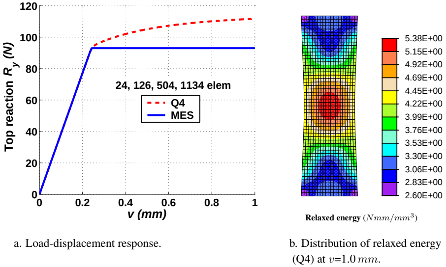
Figure 7.21.: Model based on the assumption of \mathcal{D} = \mathcal{C} : Localization in tension by use of MES element (the mixed enhanced strain method) and Q4 element (the displacement method).
