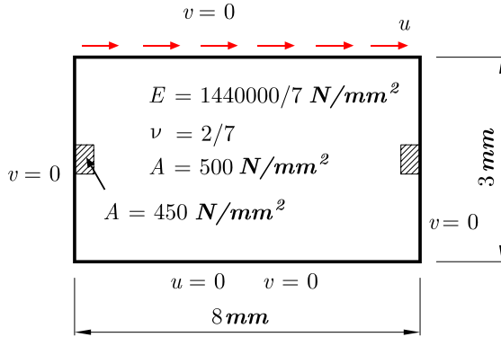
Figure 7.7.: Localization within shear test. Geometry and boundary conditions.
