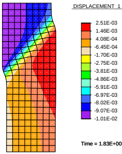
d. Mixed-Q8 element.
