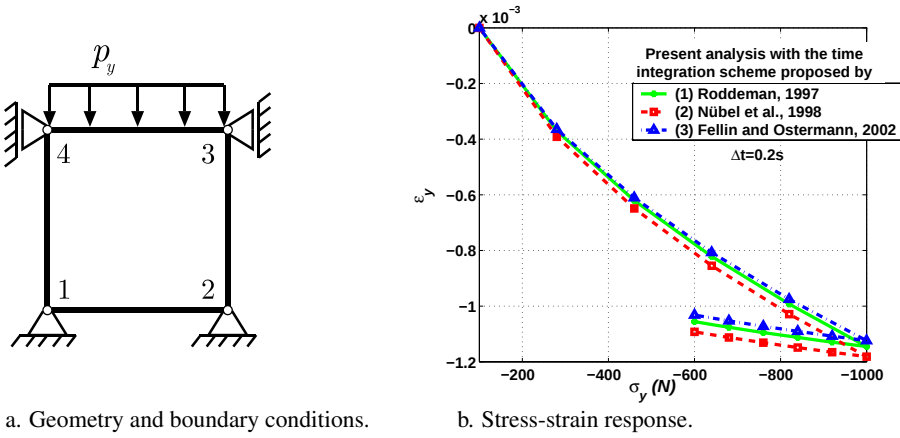
Figure 5.1.: Example 1: One-dimensional compression test.
