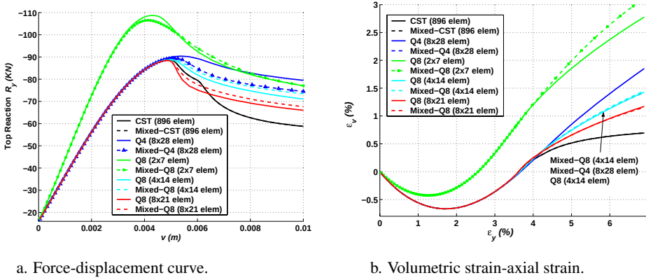
Figure 5.12.: Example 5: Biaxial test.
