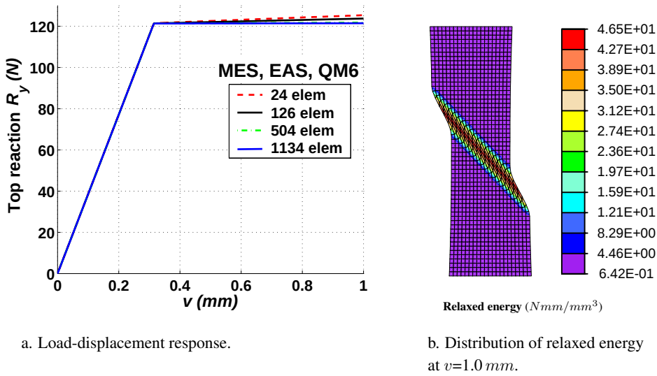
Figure 7.13.: Model based on the assumption of D = A^2\mathcal{I} and m.n = 0 : Localization in tension by use of MES element (the mixed enhanced strain method), EAS element (the enhanced assumed strain method) and QM6 element (the incompatible mode method).
