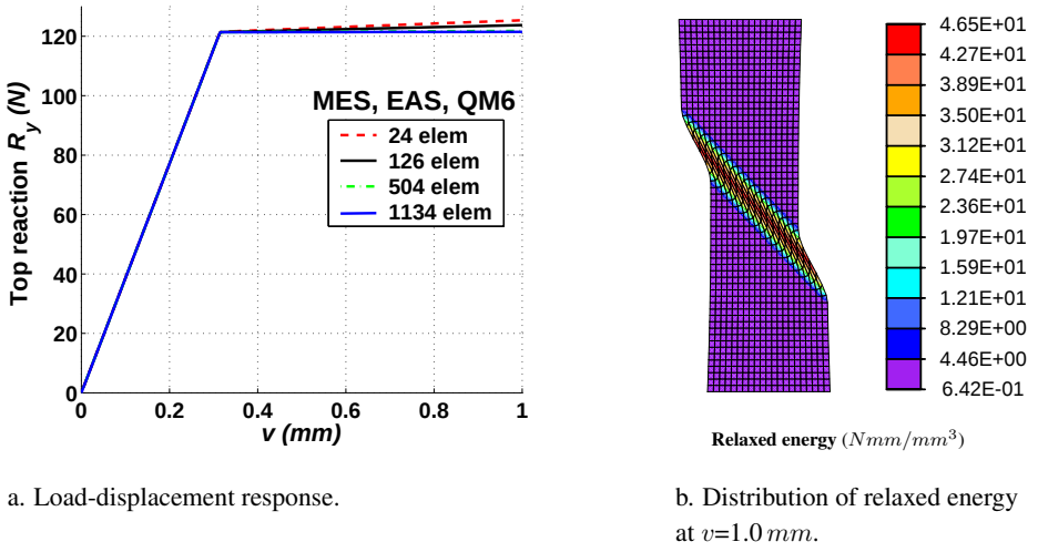
Figure 7.15.: Model based on the assumption of \mathbf{D} = A^2 \mathbf{I} and \mathbf{m} \cdot \mathbf{n} = 0 : Localization in tension by use of MES element (the mixed enhanced strain method), EAS element (the enhanced assumed strain method) and QM6 element (the incompatible mode method).
