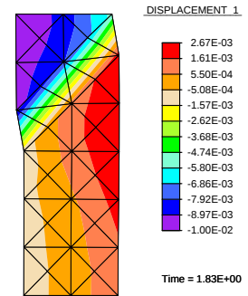
f. Mixed-CST element.
