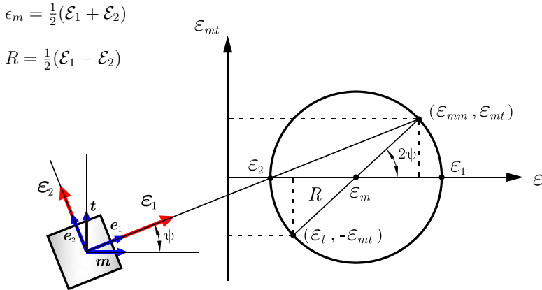
Figure 7.6.: Mohr strain circle.
