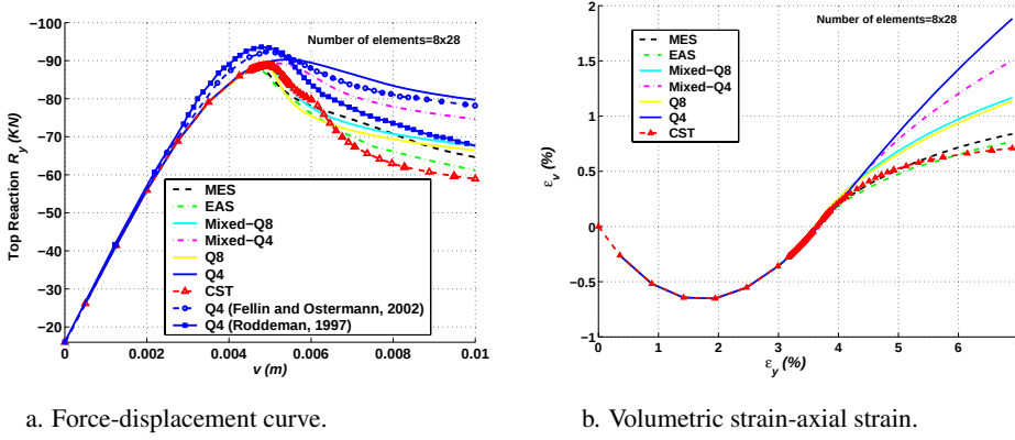
Figure 5.11.: Example 5: Biaxial test (8x28 elements).
