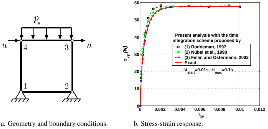
Figure 5.3.: Example 3: Simple shear test.
