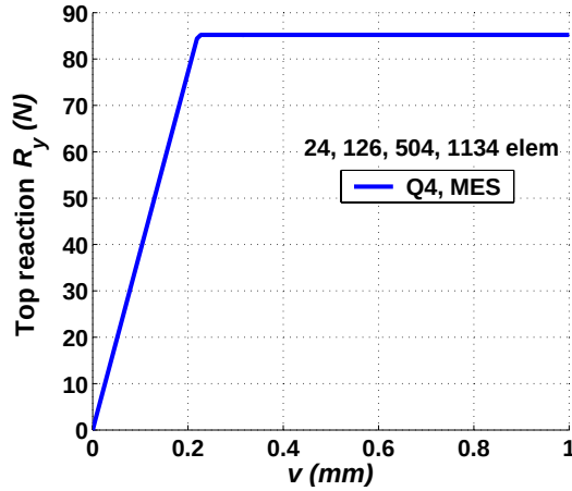
Figure 7.18.: Model based on the assumption of \mathcal{D} = A^2\mathcal{I} and -1 \leq \mathbf{m}.\mathbf{n} \leq 1 : Localization in tension by use of MES element (the mixed enhanced strain method) and Q4 element (the displacement method): Load-displacement response.
