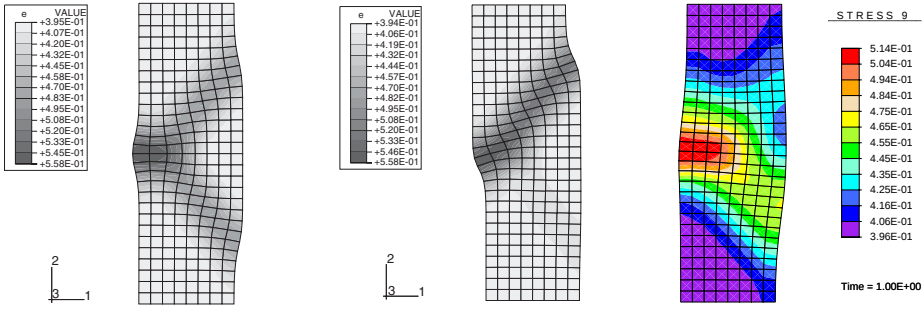
a. Q4 elem ( Fellin and Ostermann, 2002[34] ). b. Q4 elem ( Roddeman, 1997[34] ).
