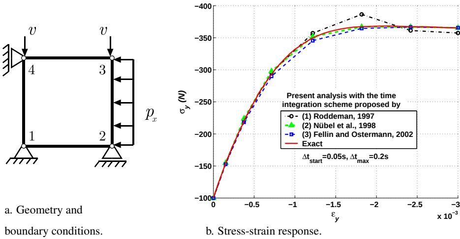
Figure 5.2.: Example 2: Biaxial test.
