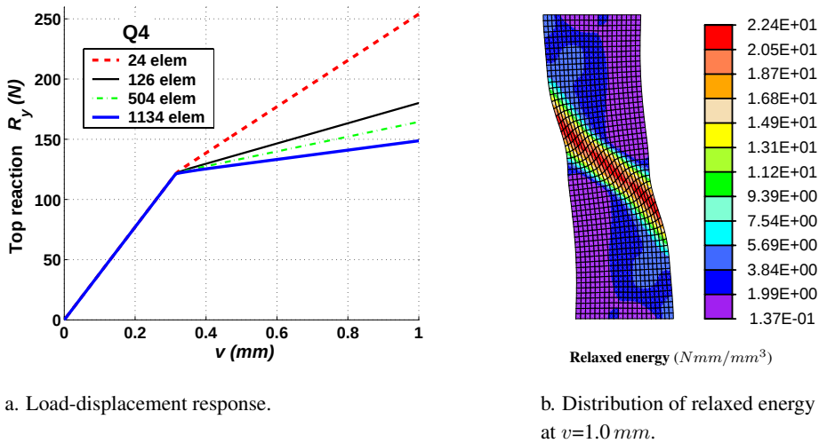
Figure 7.14.: Model based on the assumption of D = A^2\mathcal{I} and m.n = 0 : Localization in tension by use of Q4 element (the displacement method).
