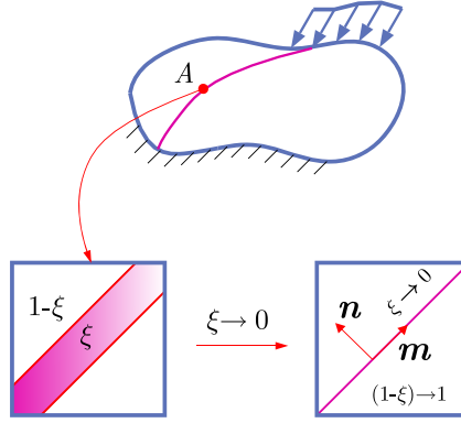
Figure 7.2.: Shear band is treated as the micro-shearing of a rank-one laminate.
