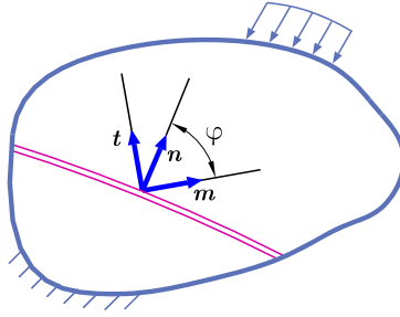
Figure 7.5.: Orientation of the shear band.
