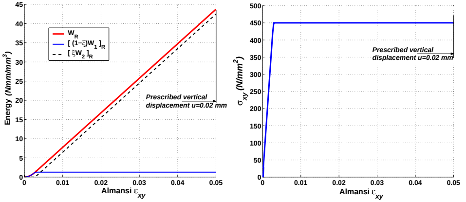
Figure 8.5.: Compressible Neo-Hookean model: Localization within shear test by use of Q4 element (the displacement method) and Mixed-Q4 element (the three-field mixed formulation): Relaxed energy and shear stress in weak elements at the first Gauss point.
