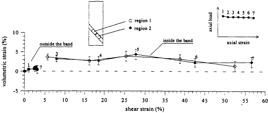
Figure 2.3.: Stereophotogrammetry-based volumetric versus shear strains [35].
