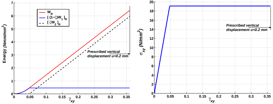
c. Relaxed energy and relaxed shear stress at the weak elements
