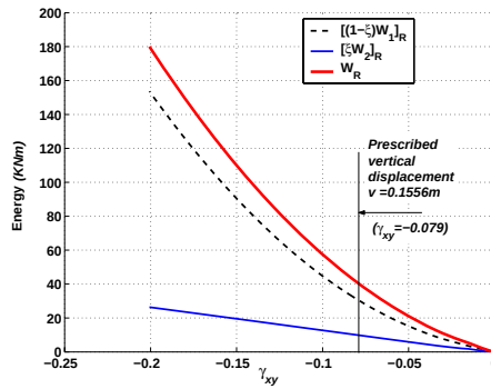
a. Relaxed energy-shear strain at the first Gauss point of the element 281.
