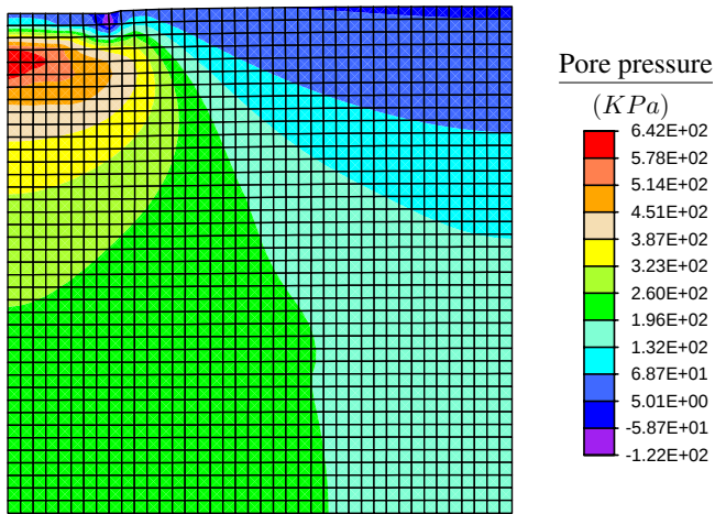
Figure 9.6.: Case 2 ( a = 5B ): Soil foundation problem by use of 1600 EAS elements (The enhanced assumed strain method with four-node displacement and seven enhanced modes for pressure interpolations): Distribution of pore pressure at the first Gauss point at v = 0.1556 m .
