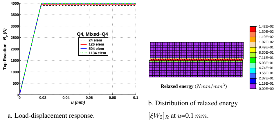
Figure 8.4.: Compressible Neo-Hookean model: Localization within shear test by use of Q4 element (the displacement method) and Mixed-Q4 element (the three-field mixed formulation).
