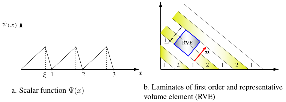
Figure 7.1.: Laminates as special fluctuation fields \varphi [39].
