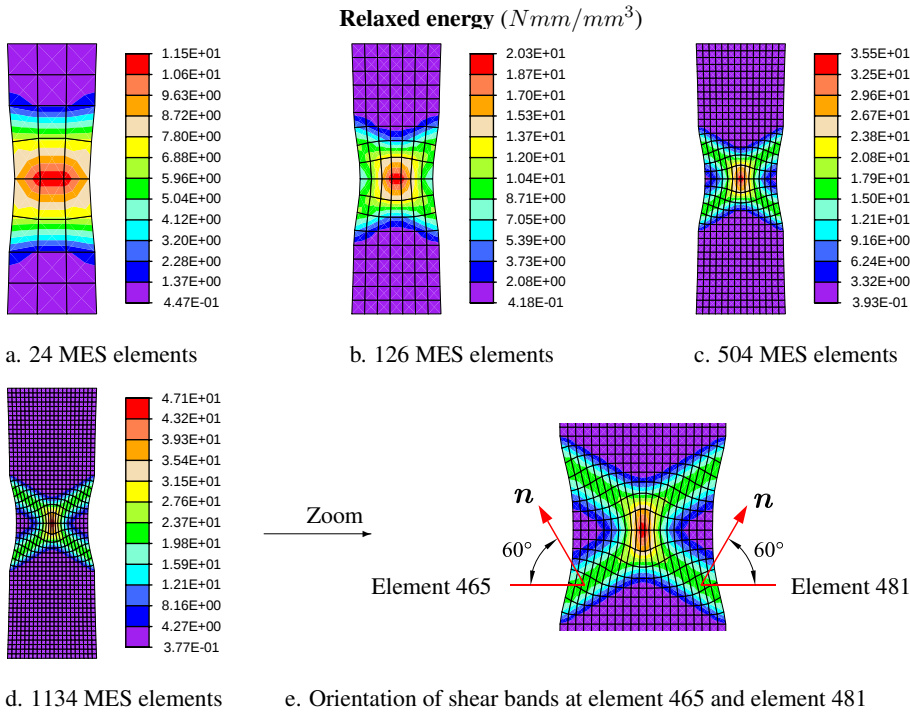
Figure 7.22.: Model based on the assumption of D = \mathcal{C} : Localization within tension test by use of MES element (the mixed enhanced strain method). Comparison of the different finite element meshes: Distribution of relaxed energy at v = 1.0\text{ mm} .
