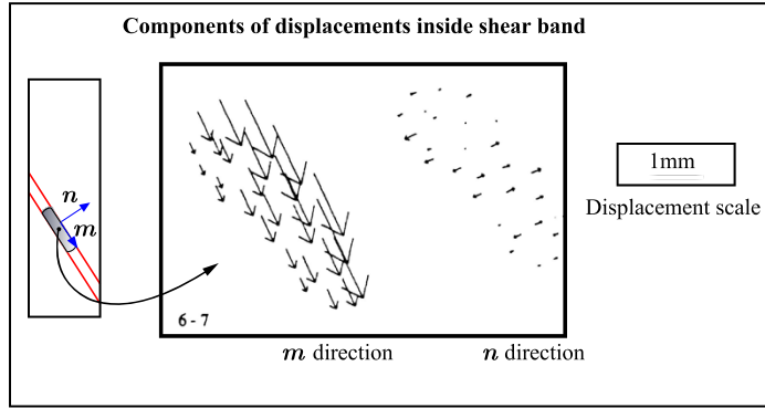
Figure 2.4.: Components of displacement inside the shear band [35].
