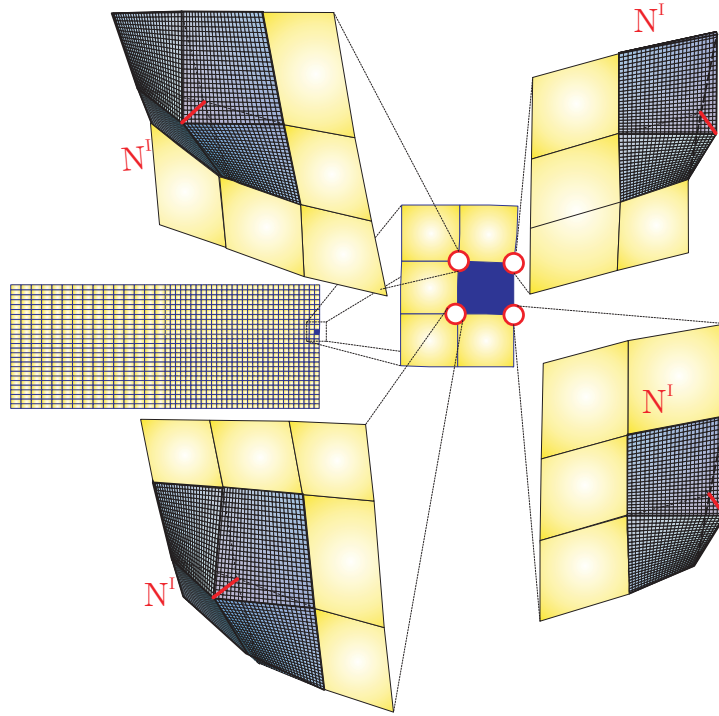
Figure 7.2.: Finite element basis functions on the element on the crack tip
