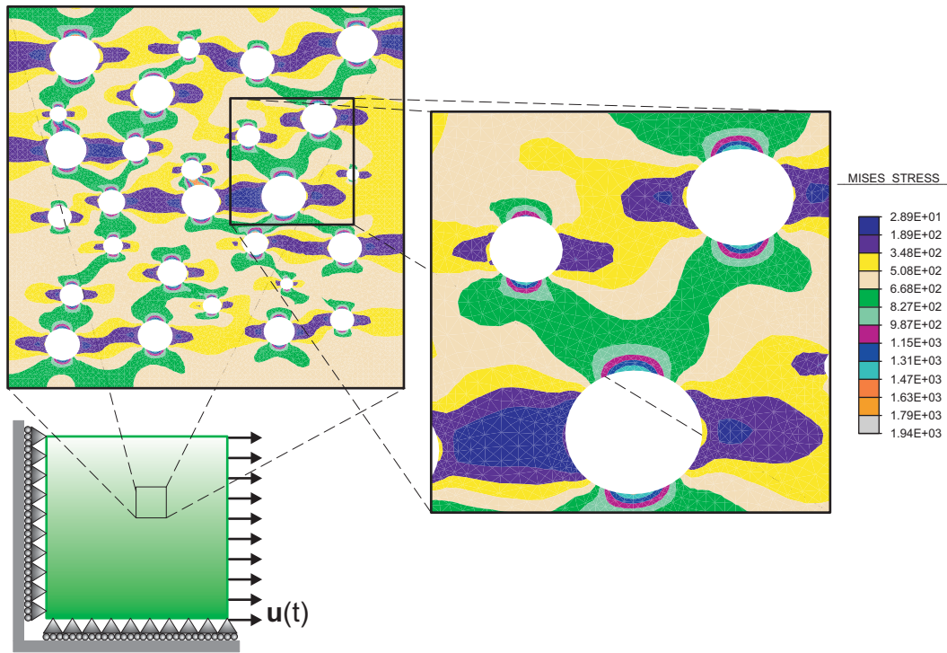
Figure 3.3.: Influence of microdefects on microscale stress
