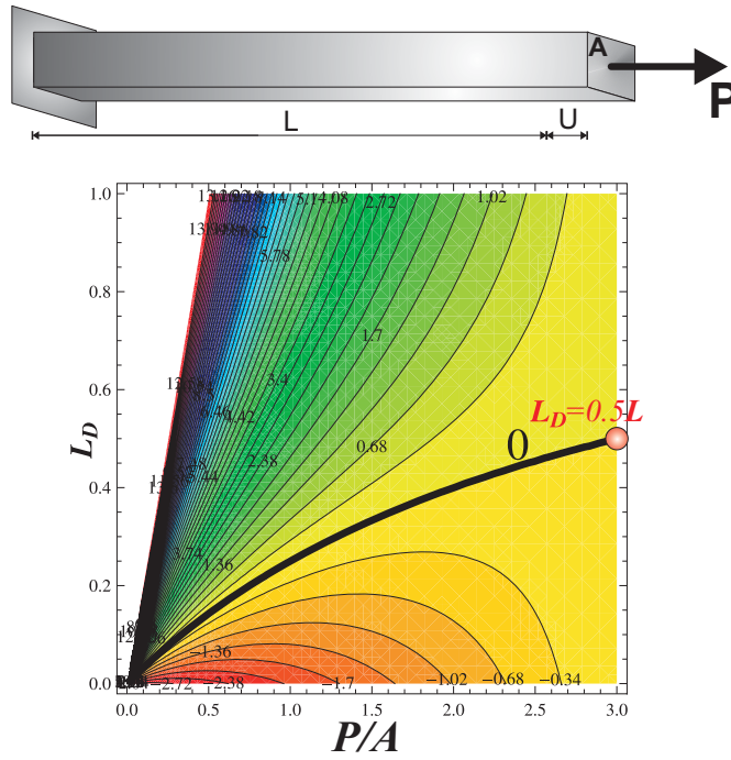
Figure 3.6.: Post-peak displacement of the end of the specimen scaled with the elasticity modulus ( E\bar{U} ) in dependence on the length of the damaged zone
