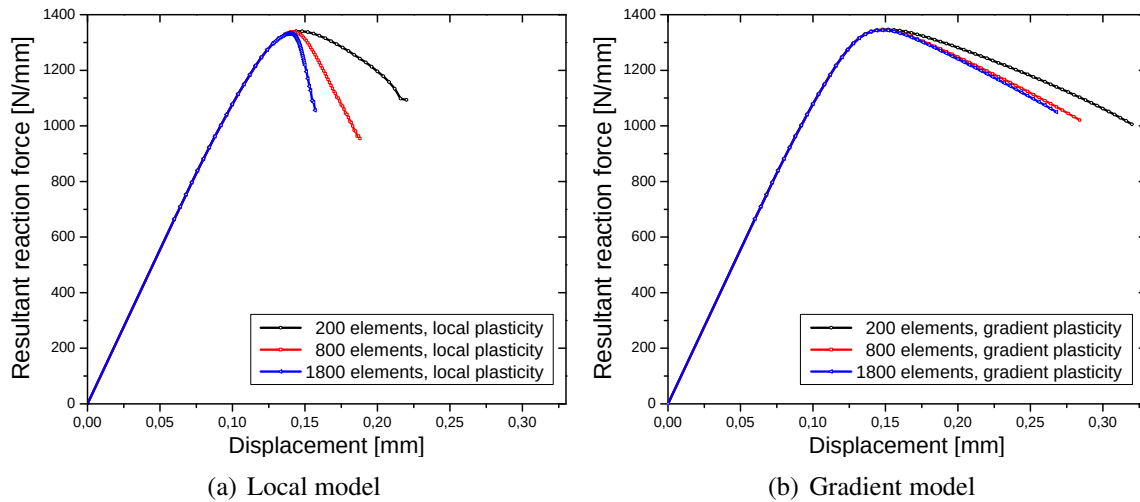
Figure 7.14.: Load-displacement diagrams for the brick-with-a-hole problem using plastic model I
