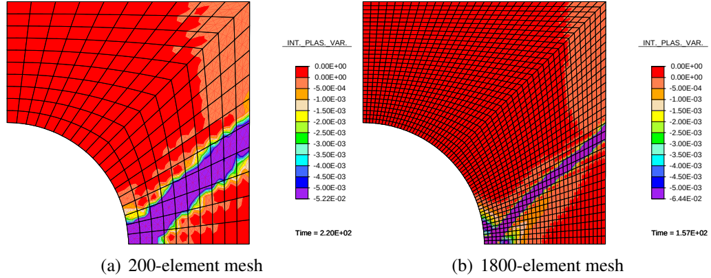
Figure 7.15.: Distribution of the plastic softening variable for the brick-with-a-hole problem at the last converging loading increment using local plastic model I
