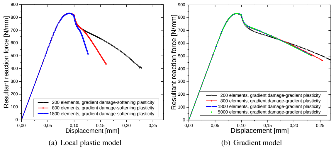
Figure 7.22.: Load-displacement diagrams for the the brick-with-a-hole problem using gradient enhanced damage-plastic model I for the negative plastic hardening parameter K_H < 0 (plastic softening)
