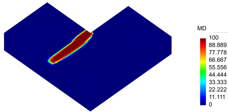
(a) Material Damage on 2300-element mesh
