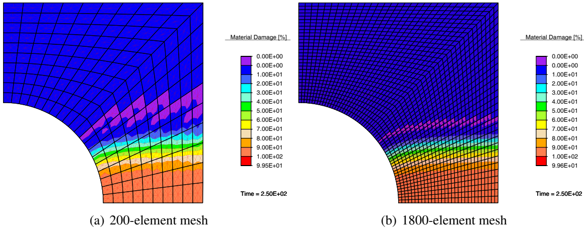
Figure 7.7.: Distribution of the Material Damage for the brick-with-a-hole problem at the end of the test using gradient enhanced damage model I
