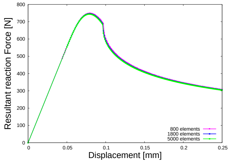
(a) Load-displacement diagrams for the brick with a hole problem using gradient enhanced damage model II
