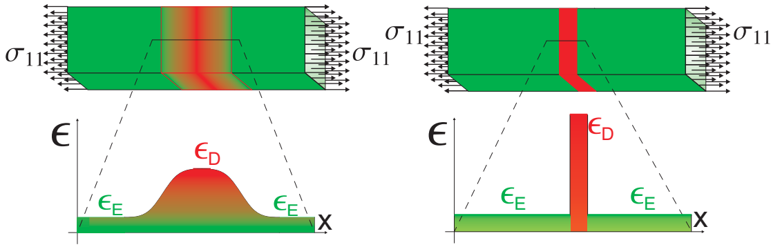
Figure 3.8.: Strain distribution in regularized continuum (left) and crack band (fracture energy) models (right)
