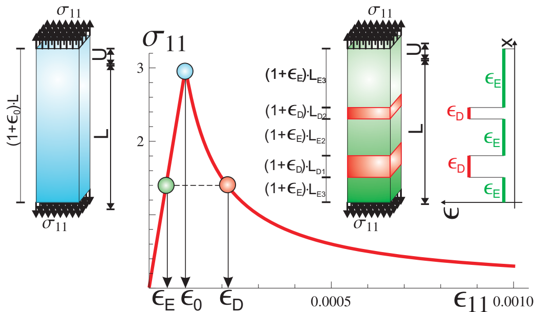
(b) Stress-strain curves resulting from the material model, development of damage zones in the specimen and corresponding strain distribution
