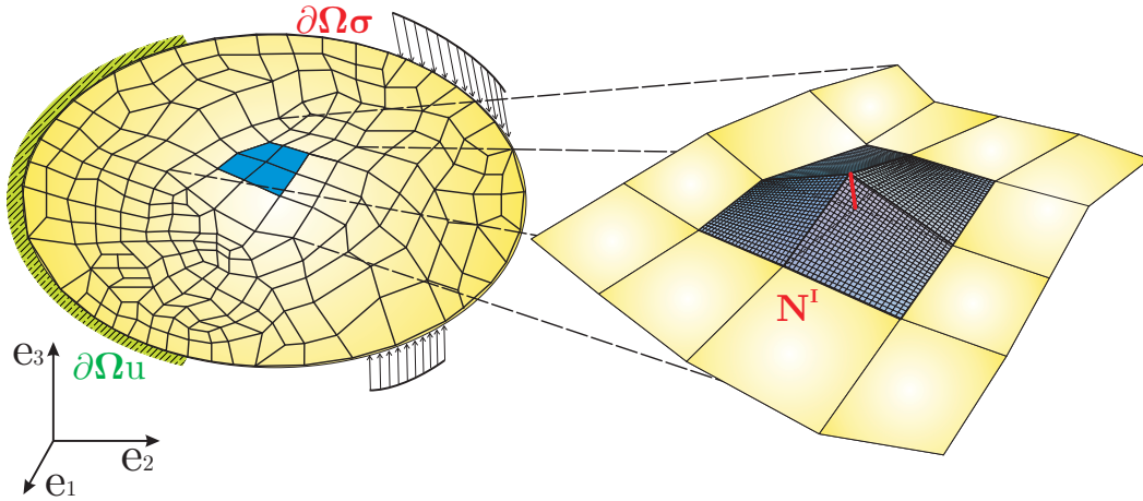
Figure 6.1.: Finite element discretization of domain and a typical basis function in a two-dimensional case
