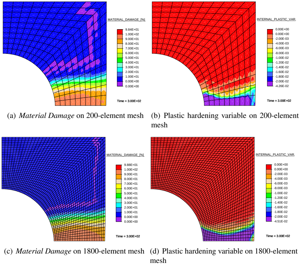
Figure 7.21.: Distribution of internal variables for the brick-with-a-hole problem at the end of the test using gradient enhanced damage model I combined with the local plastic model I
