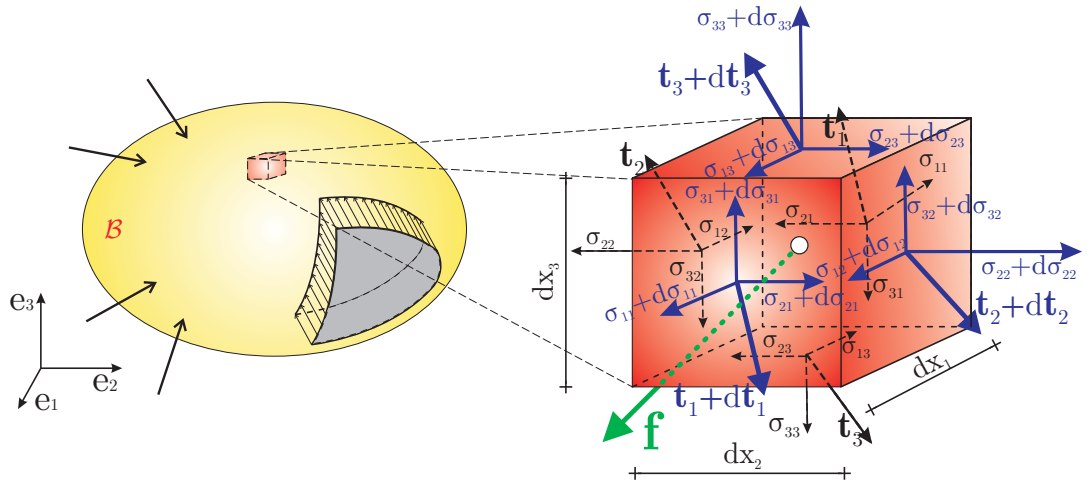
Figure 2.9.: Representation of infinitesimal equilibrium conditions
