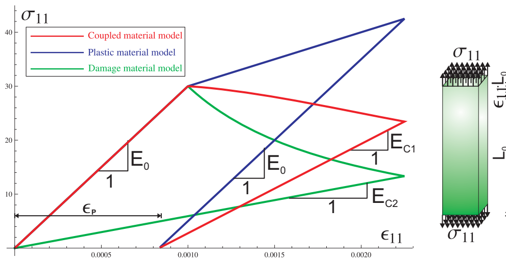
Figure 3.4.: Loading-unloading stress-strain curves of damage, plastic and coupled models
