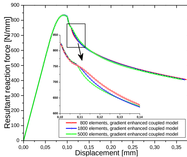
Figure 7.25.: Load-displacement diagrams for the the brick-with-a-hole problem using gradient enhanced coupled damage-plastic model II
