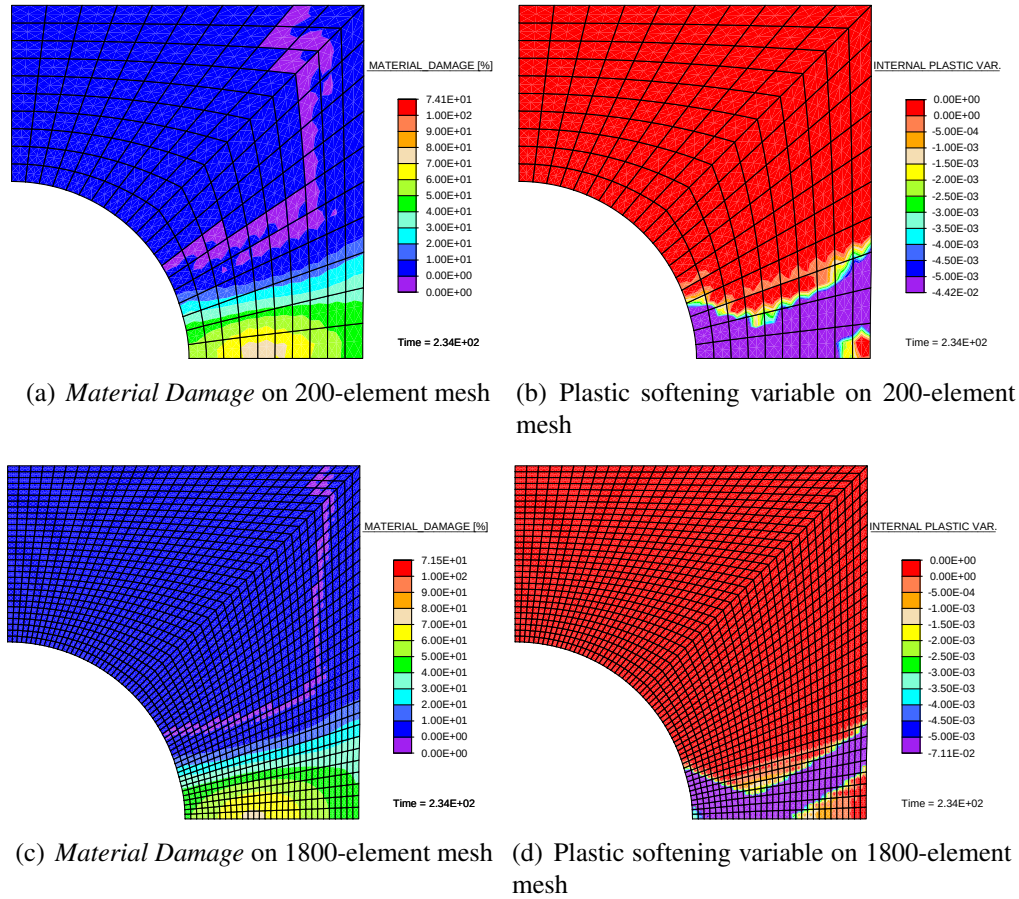
Figure 7.24.: Distribution of internal variables for the brick-with-a-hole problem at the end of the test using gradient enhanced coupled damage-plastic model I
