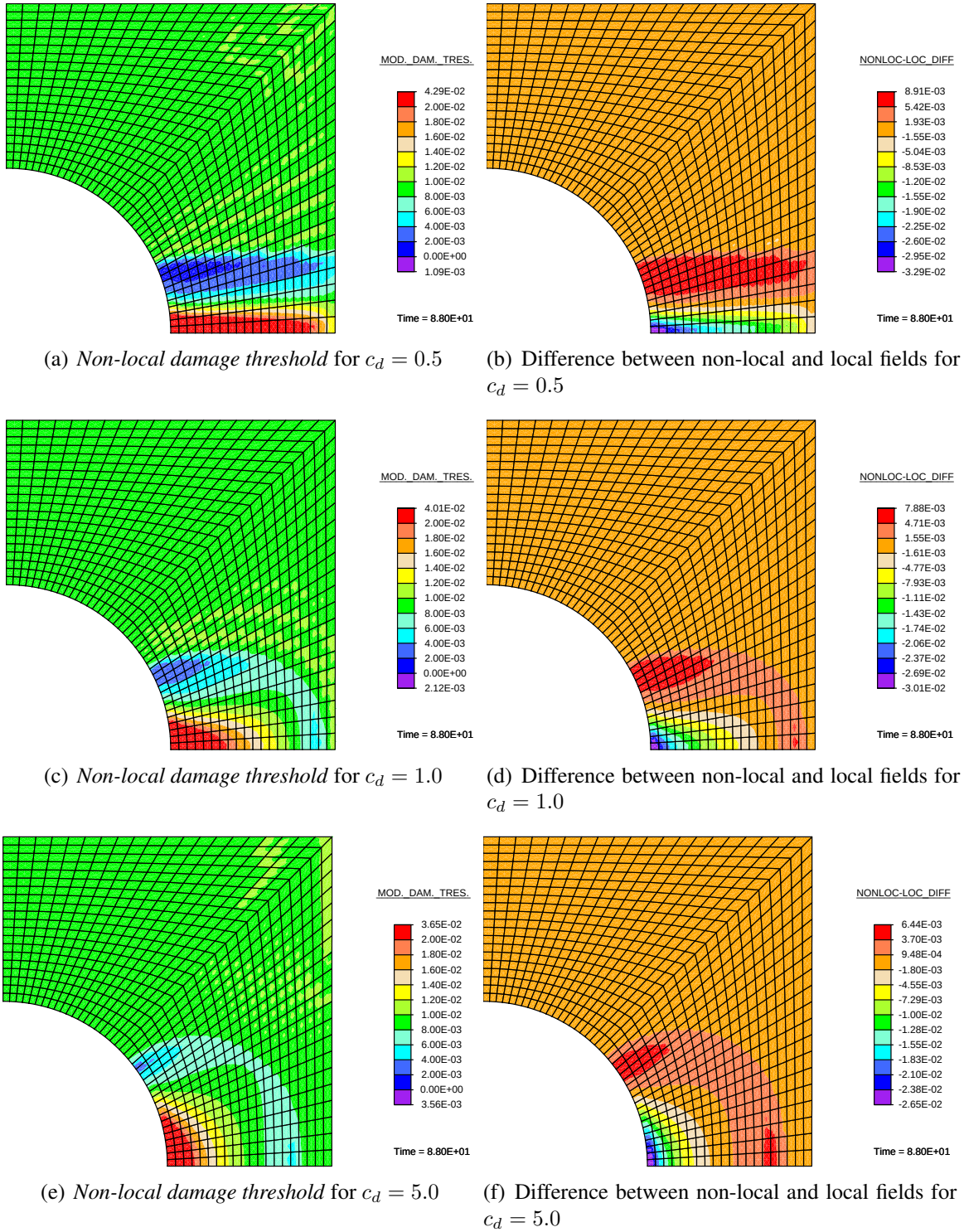
Figure 7.9.: Distribution of the selected problem quantities for the brick-with-a-hole problem on the 800-element mesh at the test stage denoted in the Figure 7.8(a) for \beta_d = 1.0
