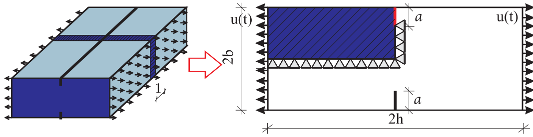
Figure 7.1.: Geometry of the pre-cracked brick test
