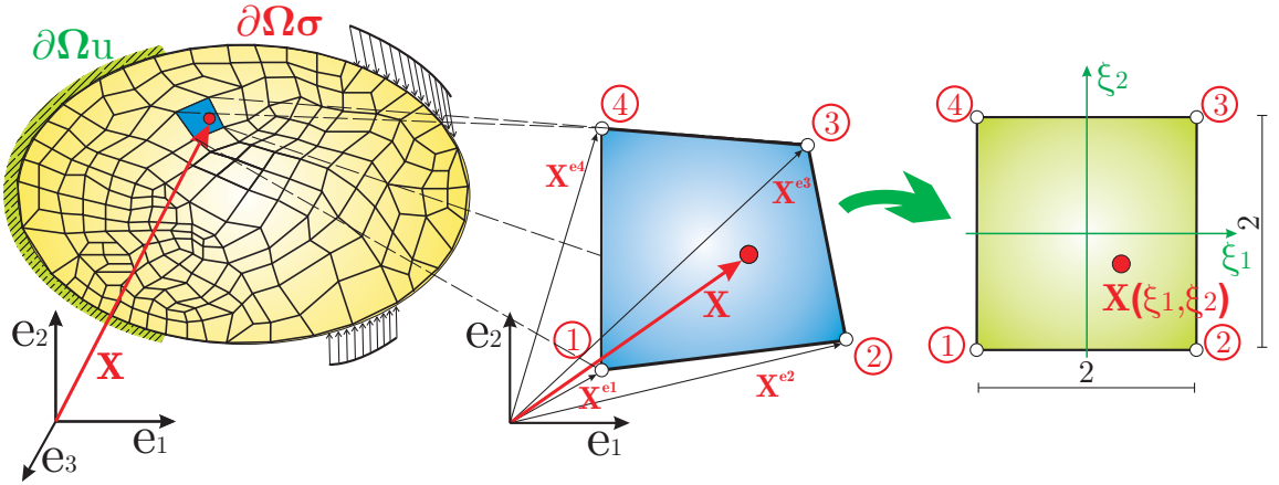
Figure 6.2.: Example of a two-dimensional mapping of an element
