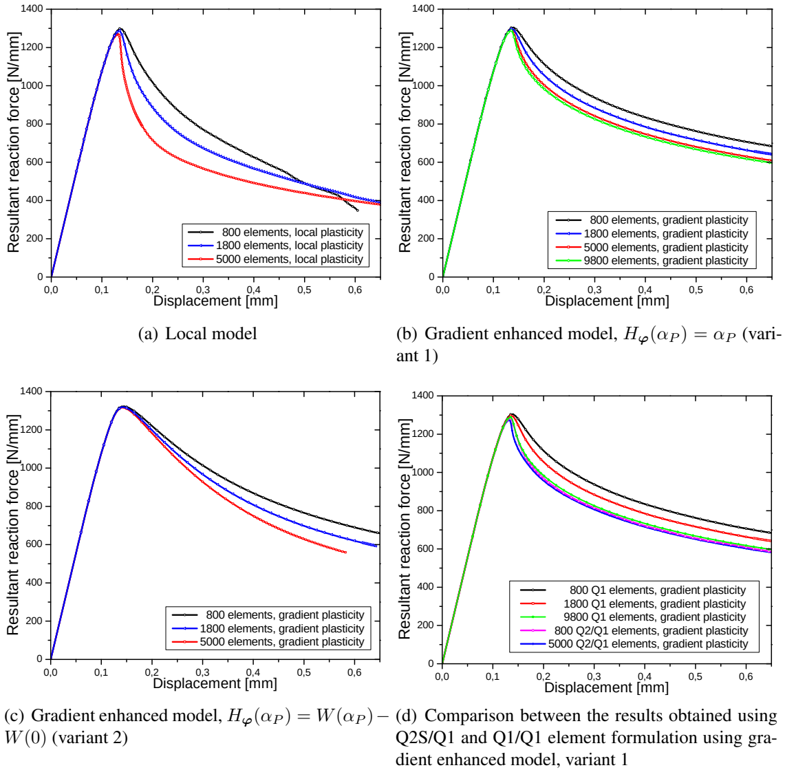
Figure 7.17.: Load-displacement diagrams for the the brick-with-a-hole problem using gradient enhanced plastic model II
