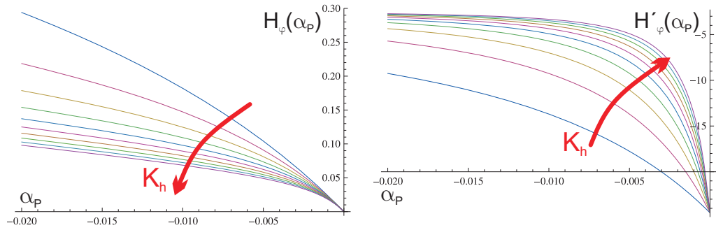
Figure 5.4.: Potential function H_\varphi(\alpha_P) and its derivatives based on the plastic potential W_2(\alpha_P) . The red arrow shows the direction in which the parameter K_H increases.
