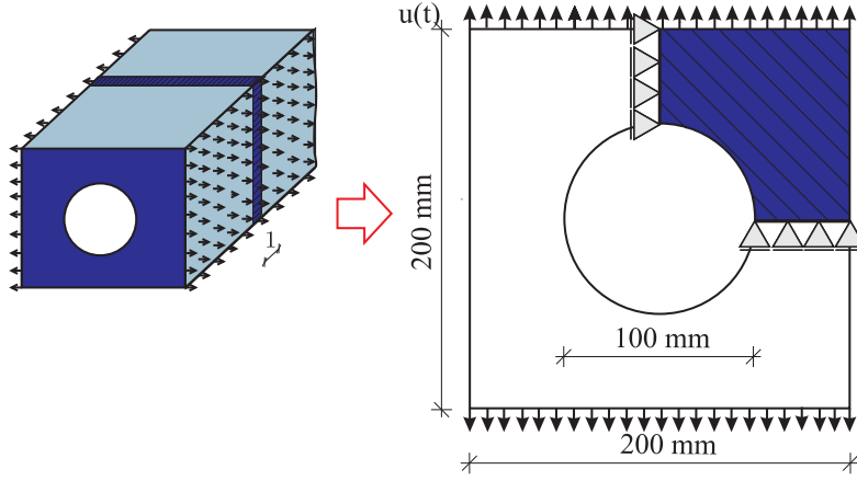
Figure 7.5.: Geometry of the brick-with-a-hole test
