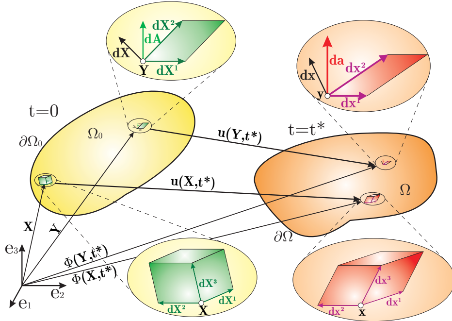
Figure 2.3.: Deformation of infinitesimal volume dV and surface dS elements
