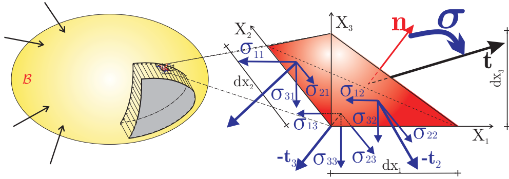
Figure 2.8.: Equilibrium of infinitesimal tetrahedron
