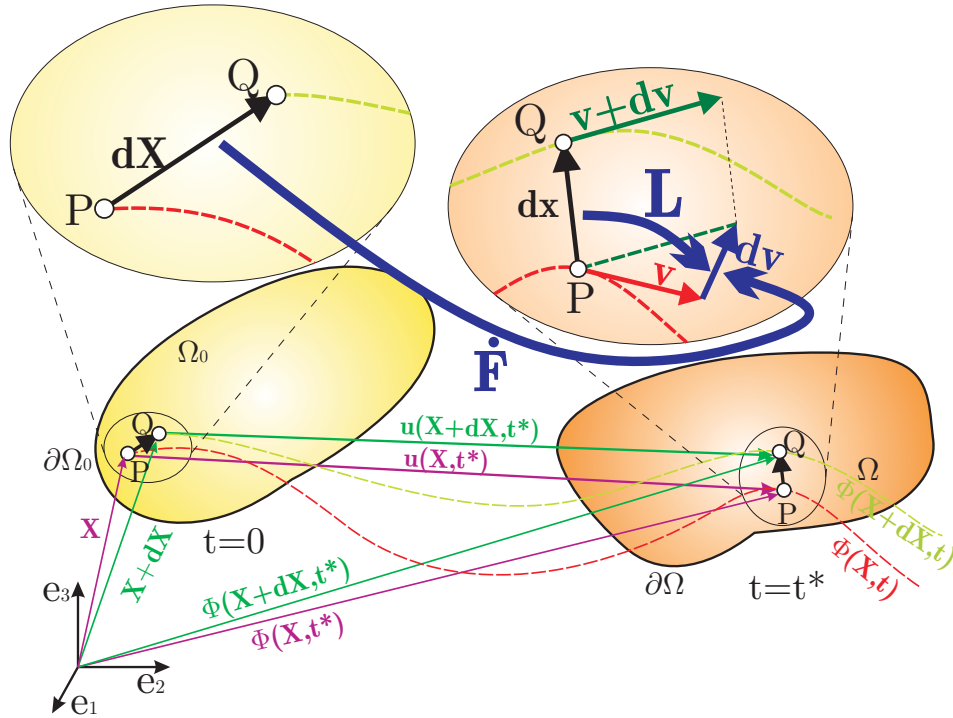
Figure 2.6.: Infinitesimal line elements in reference and current configuration
