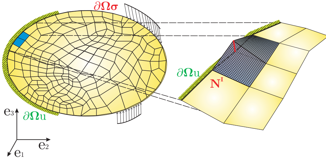
Figure 6.3.: Finite element basis function on the Dirichlet boundary in a two-dimensional case
