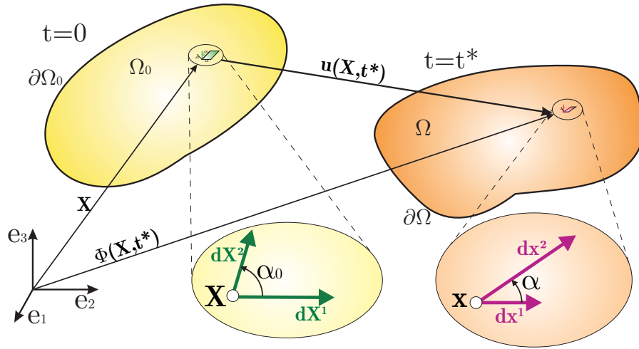
Figure 2.5.: Infinitesimal line elements in reference and current configuration
