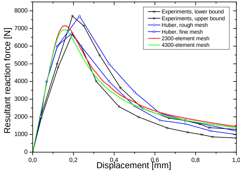
Figure 7.12.: Load-displacement diagrams for the L-panel problem using gradient enhanced damage model II
