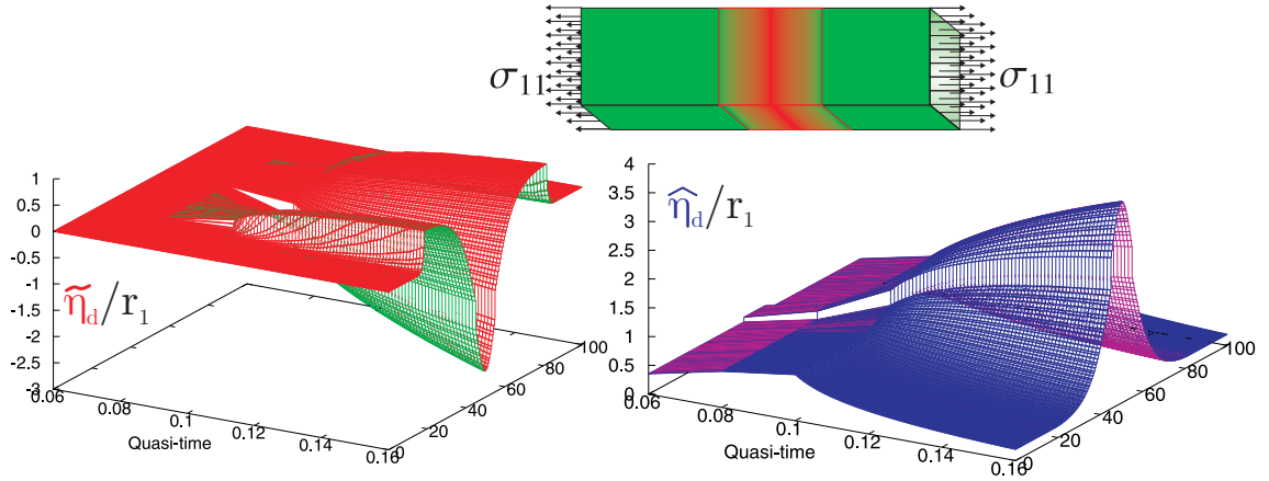
Figure 5.1.: Evolution of a distribution of local ( \hat{\eta}_d ) and interaction ( \tilde{\eta}_d ) part of the micromechanical driving force normalized with the damage threshold r_1
