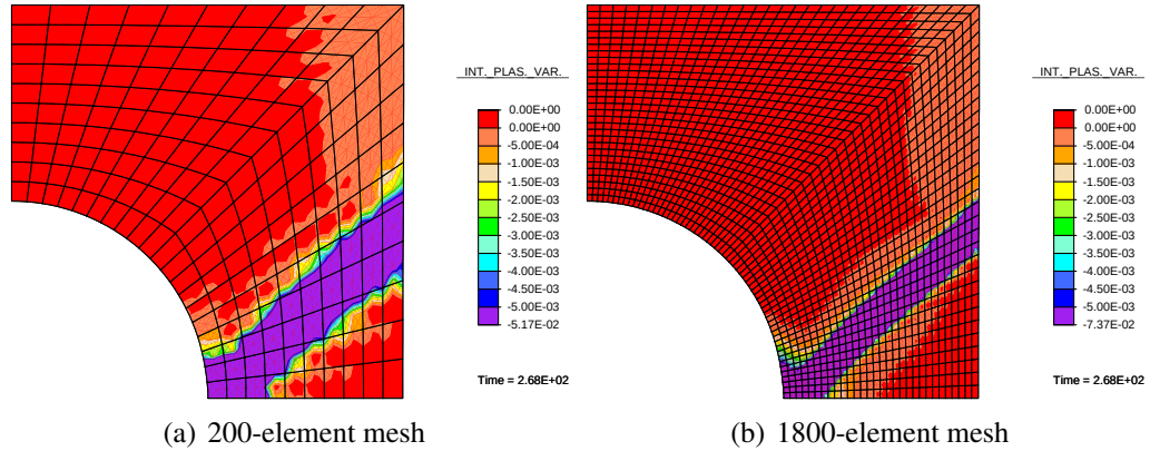
Figure 7.16.: Distribution of the plastic softening variable for the brick-with-a-hole problem at the end of the test using gradient enhanced plastic model I
