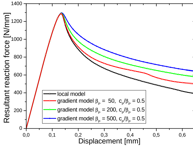
Figure 7.19.: Influence of the change in the parameter \beta_P on the load-displacement diagrams for the brick-with-a-hole problem for the fixed ratio c_P/\beta_P = 0.5 utilizing plastic model II
