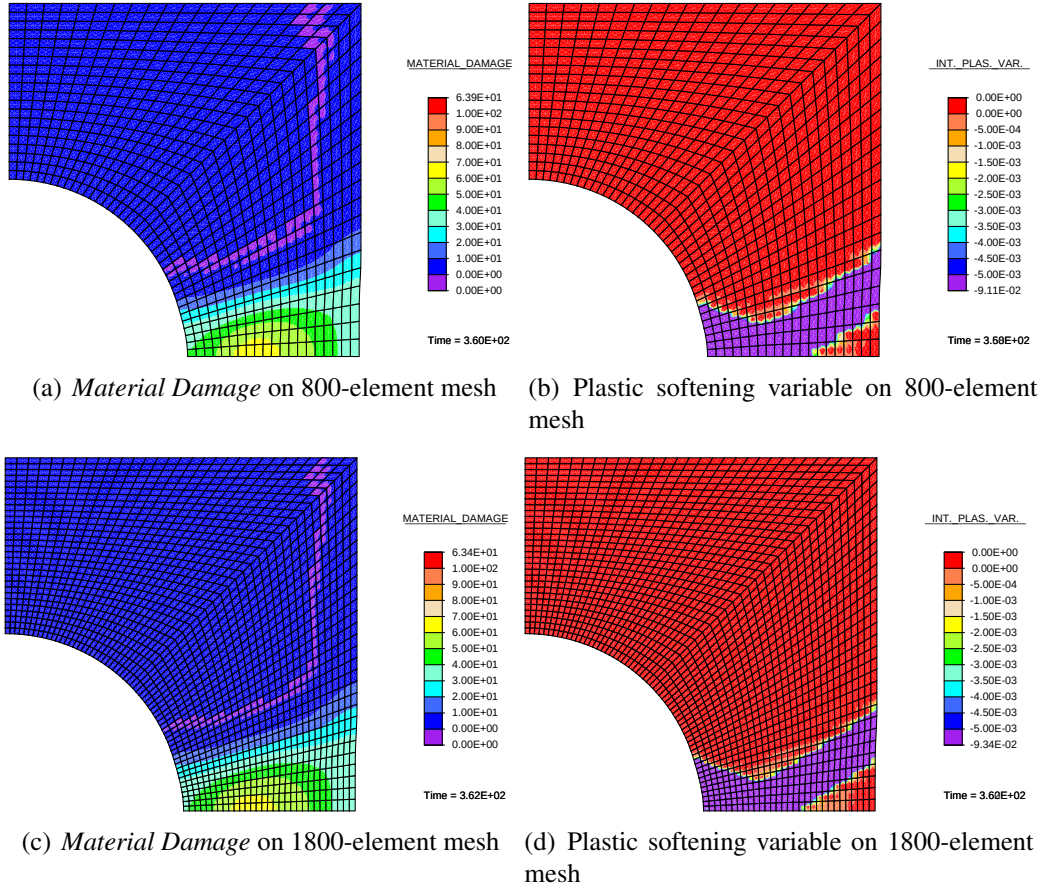
Figure 7.26.: Distribution of the selected calculation results for the brick-with-a-hole problem at the end of the test using gradient enhanced coupled damage-plastic model II
