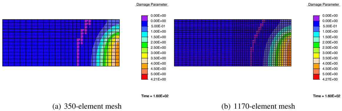
Figure 7.4.: Distribution of the damage parameter for the cracked brick problem at the end of the test using gradient enhanced damage model I
