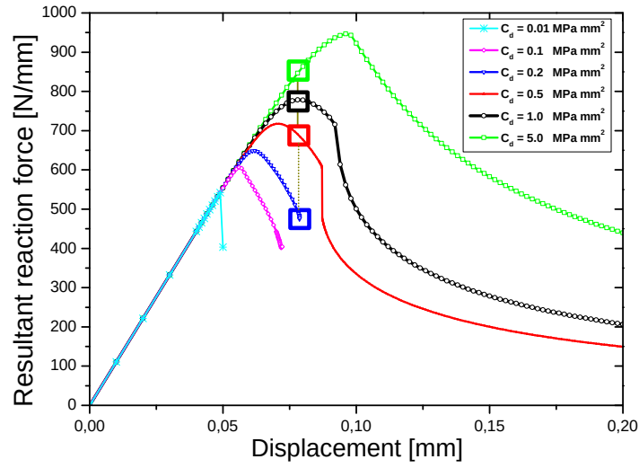
(a) Load-displacement diagrams
