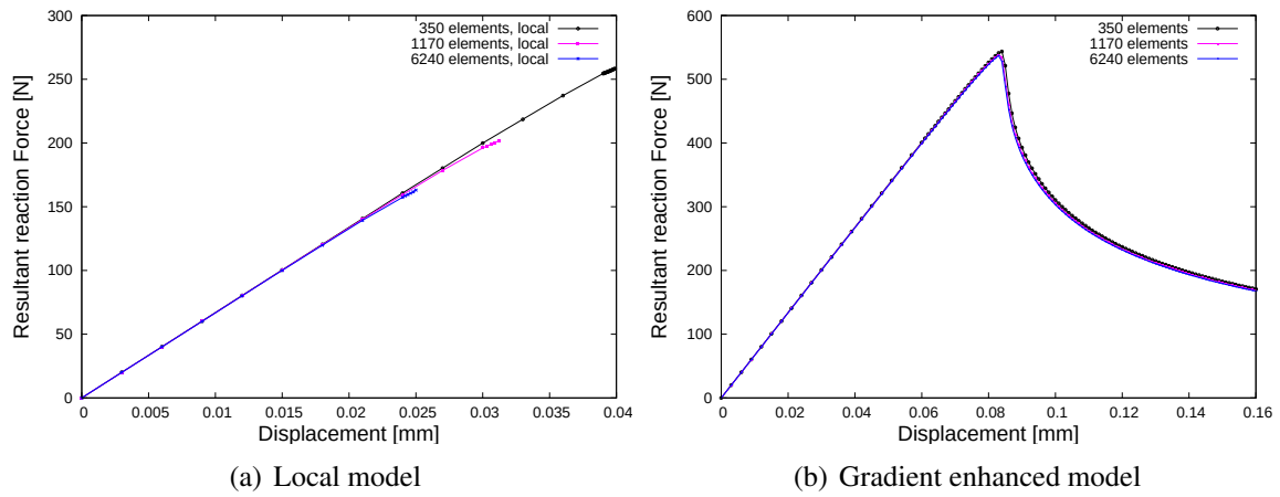
Figure 7.3.: Load-displacement diagrams for the cracked brick problem using local and gradient enhanced damage model I
