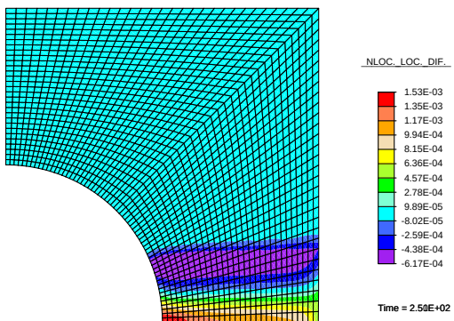
(d) Difference between non-local and local field on 1800-element mesh
