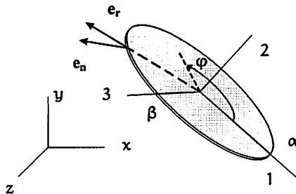
Figure 5.5: elliptical crack and local coordinates
