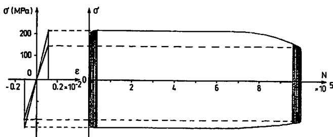
Figure 1.14: cyclic tension-compression test for high cycle fatigue of A316 stainless steel
