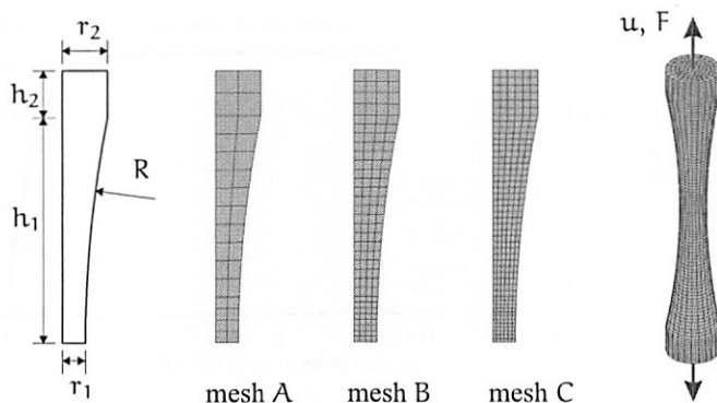
Figure 5.13: specimen geometry and different mesh patterns
