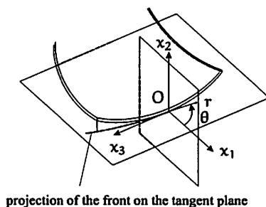
Figure 1.11: arbitrarily shaped crack
