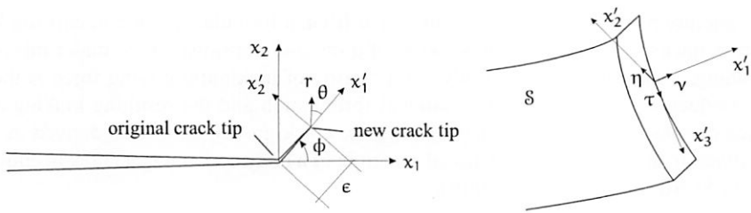
Figure 3.1: crack extension and new crack coordinates
