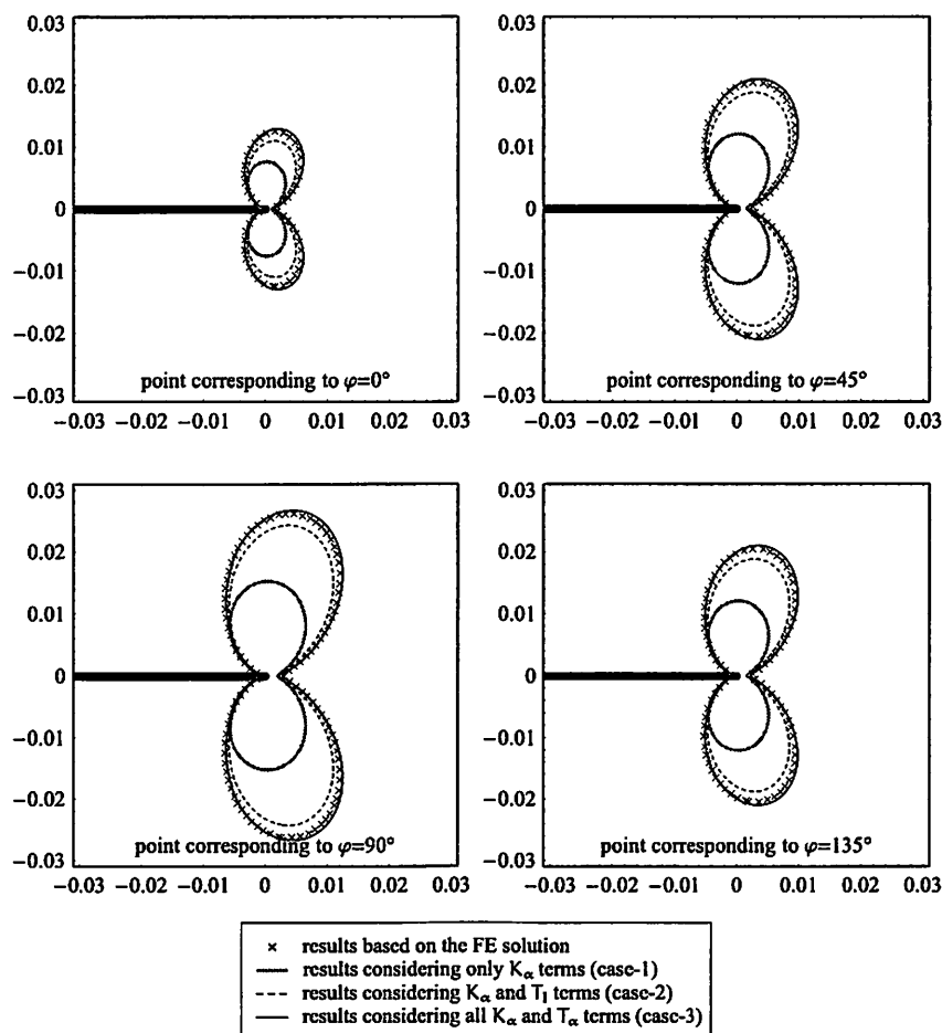
Figure 2.12: elliptical crack with \gamma_x = \gamma_y = 0^\circ , normalized plastic zone \frac{\tau_p}{\alpha}
