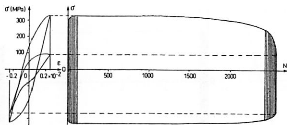
Figure 1.13: cyclic tension-compression test for low cycle fatigue of A316L stainless steel
