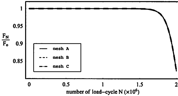
Figure 5.14: load-cycle curves for different mesh patterns
