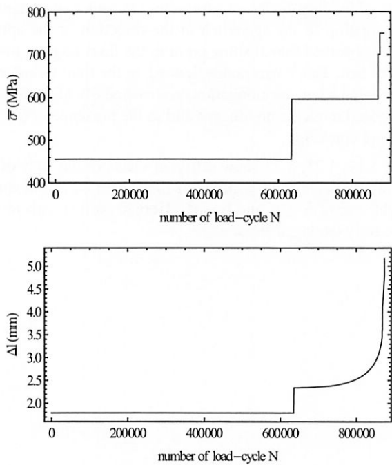
Figure 5.16: experiment 1: stress-cycle and elongation-cycle curves
