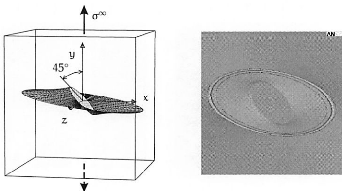
Figure 3.14: growth of the circular crack with \gamma_z = 45^\circ and \gamma_x = \gamma_y = 0^\circ
