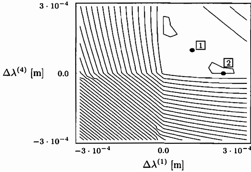
Figure 4.4: 2D contour plot of the potential \mathcal{I}_h as a function of \Delta\lambda^{(1)} and \Delta\lambda^{(4)}
