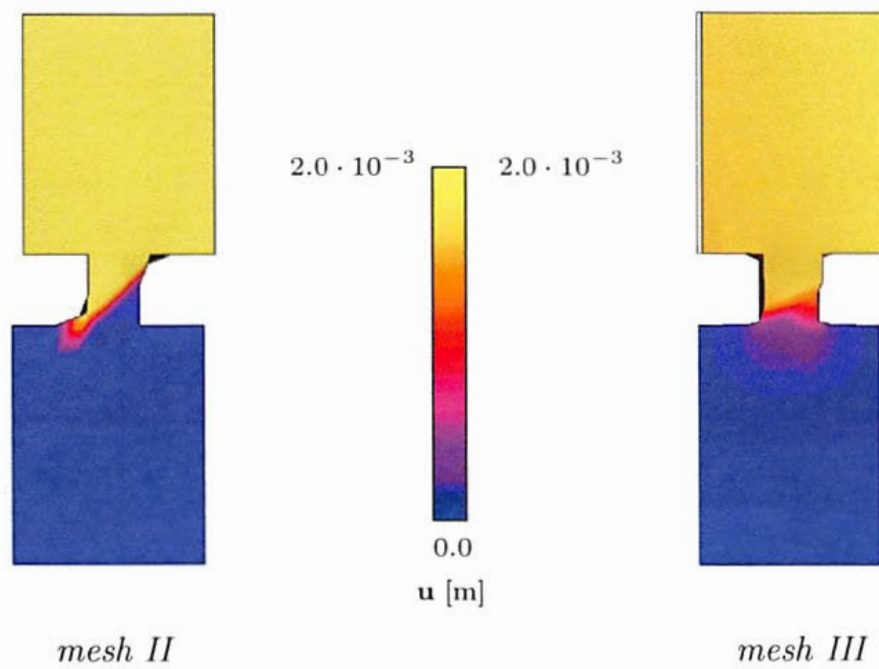
Figure 5.12: Deformed shape (magnification factor 100) and the scalar plot of the total displacement for meshes II and III
