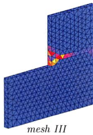
Figure 5.18: Distribution of the internal variable \alpha_{max} for meshes mesh I , II and III
