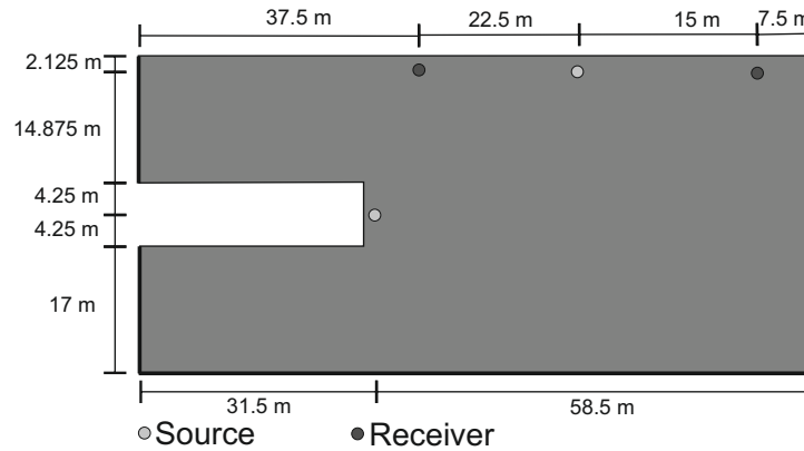
Figure 8.16: Source/receiver setup
