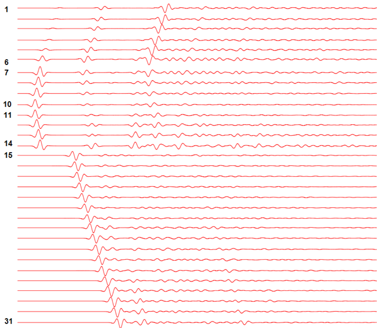
Figure 8.19: Wavefields at the receivers, source s_1 (scenario 1)
