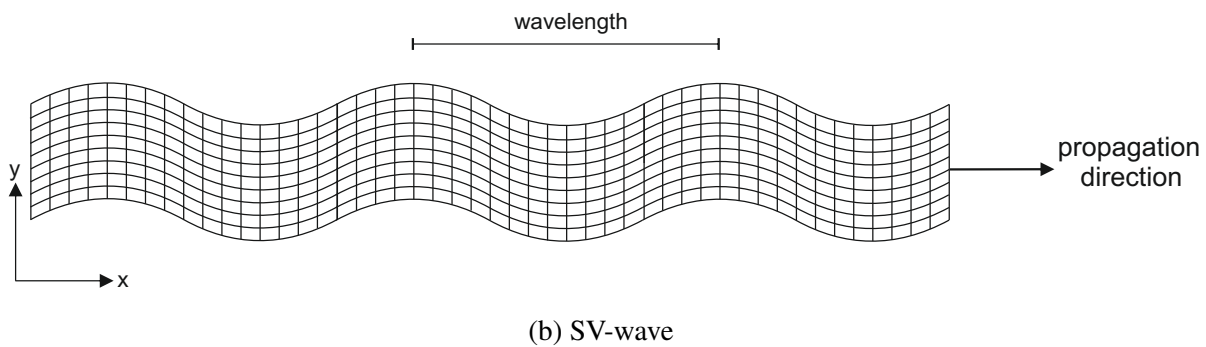
Figure 2.2: Body waves
