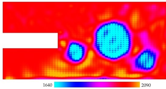
(d) #4, vel. field with polynomials of deg. 6
