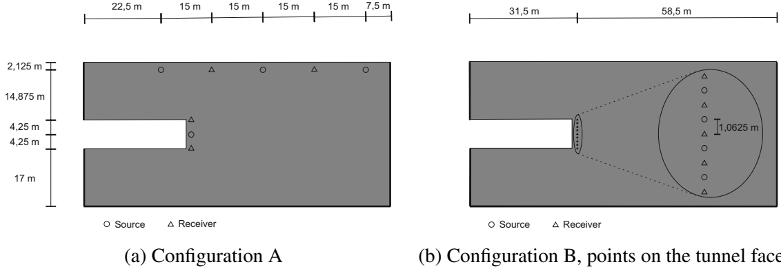
Figure 8.2: Source/receiver configurations
