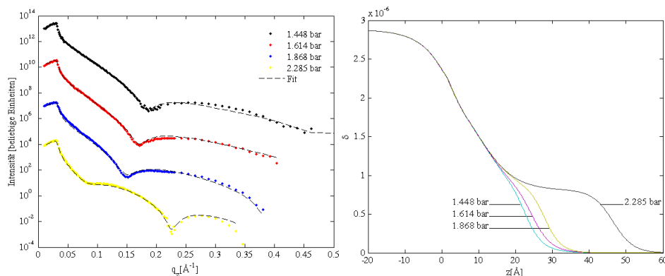
Figure 1a: Reflectivities of Isobutane films adsorbed on Silicon at different pressures.
