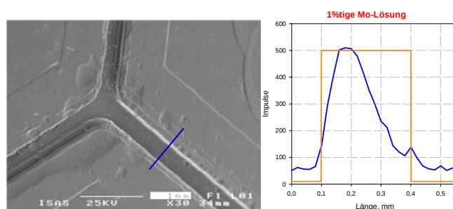
Fig. 5. A SEM micrograph of a micro channel on a PMMA substrate is shown. The elemental distribution over the blue line is represented in the right graph.
