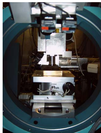
Fig. 1: Experimental set-up at DELTA.
