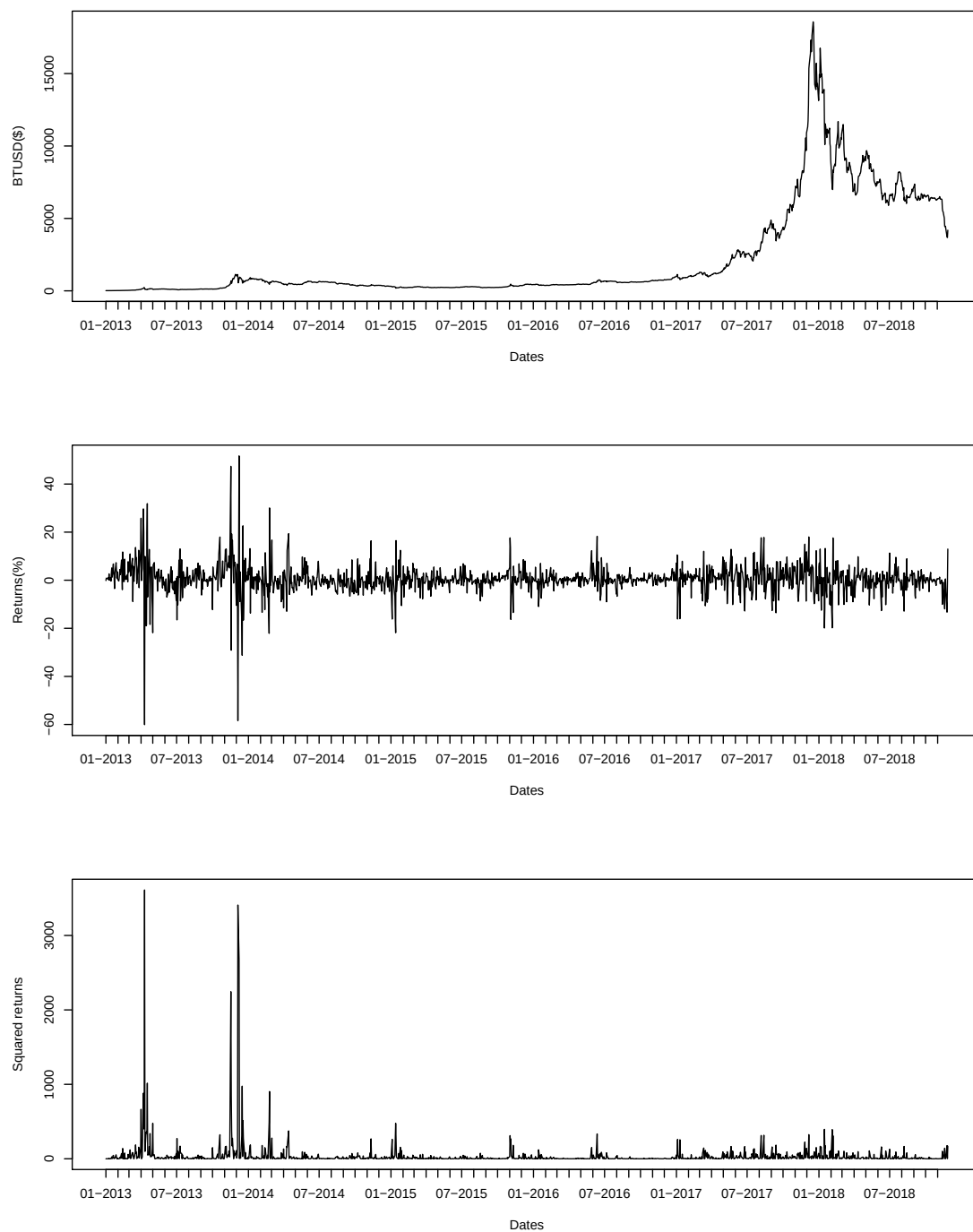
Figure 1: Plot of bitcoin USD exchange rates, the returns and squared returns
