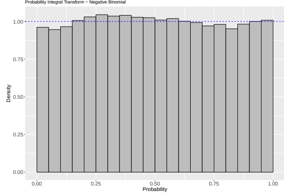
Figure 8: Non-randomized PIT histogram for a conditional Negative Binomial distribution
