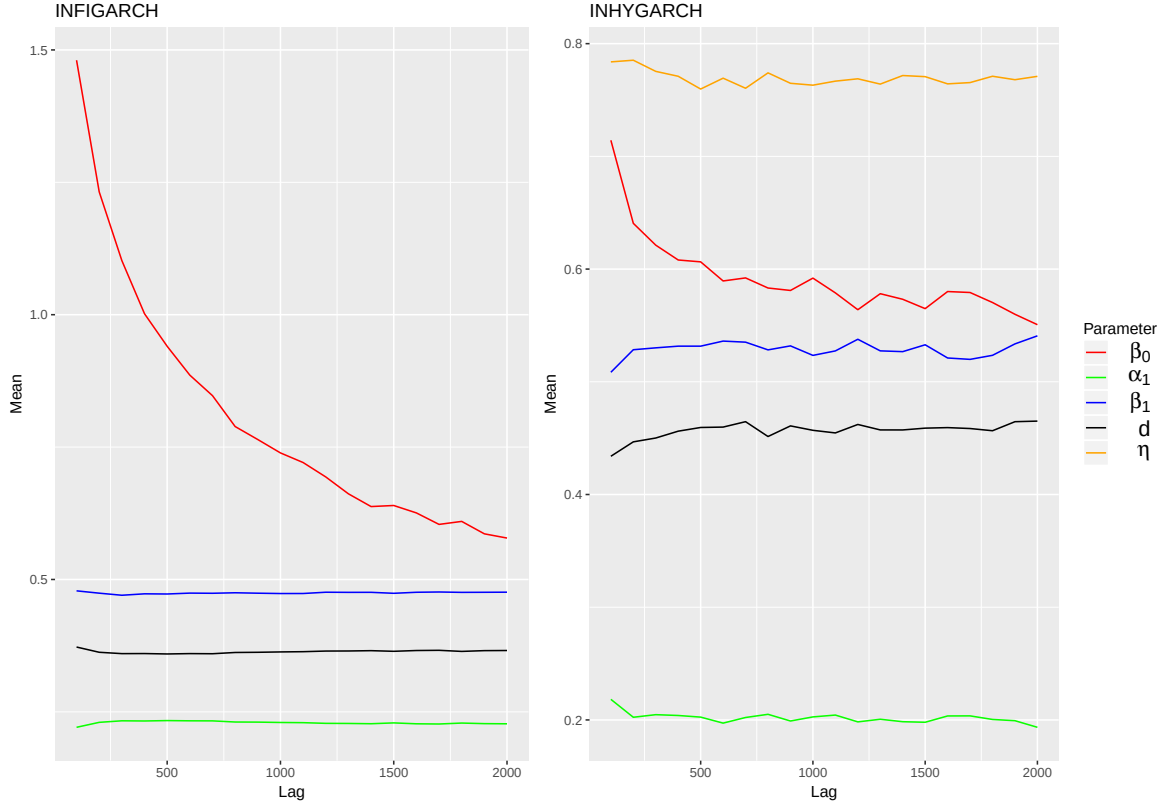
Figure 2: Impact of lag order R on the expectation of the estimators.
