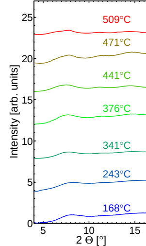
Figure 2: X-ray diffraction pattern for annealed GeO samples are found to be amorphous up to temperatures of 500°C.
