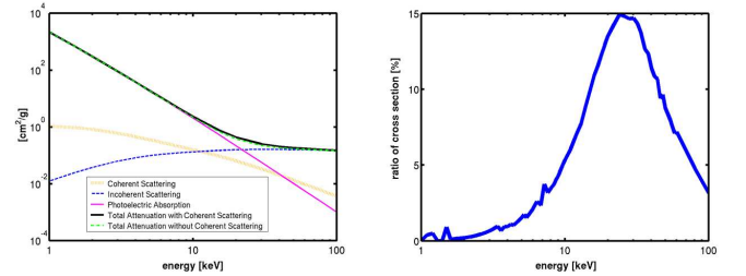
FIG. 2: (Left) X-Ray interaction cross section of carbon as a function of energy [7]. (Right) Assuming that scattering from biological thin films at solid-liquid interfaces is dominated by C and H 2 O, the according ratio of coherent and incoherent cross sections is shown as a function of energy [7].
