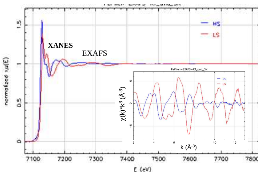
Figure 1: XAFS and k^3 -weighted EXAFS spectra of Fe(Phen) 2 (NCS) 2 before (HS) and after (LS) cooling, at the Fe K-edge
