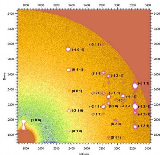
Figure 1 Two-dimensional GISAXS pattern for 100nm PDI8CN2 on Si substrate, measured by grazing incidence angle using image plate detector.
