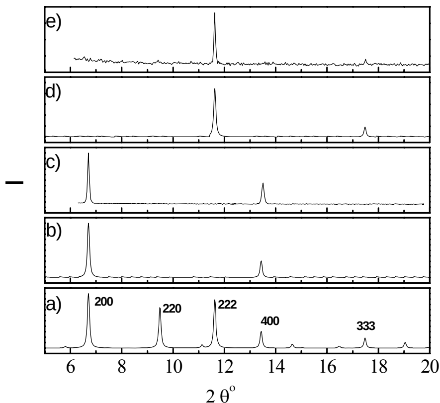
Figure 1. Out-of-plane XRD data for a \text{Cu}_3\text{BTC}_2 \cdot x\text{H}_2\text{O} MOF a) Bulk, b) growth on a MHDA SAM (Simulation), c) experimental growth on MHDA SAM (experimental), d) growth on MUD SAM (Simulation), e) grown on MUD SAM (experimental).
