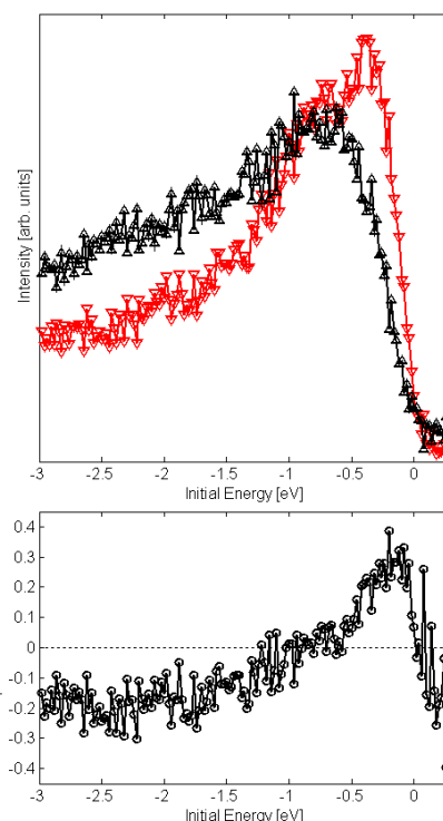
Fig 3. Spin-polarized and spin-polarization spectra of 12ML Co on Cu(100) at h\nu = 54.3 eV. Sherman (asymmetry) function 0.25. Total acquisition time 28 minutes.
