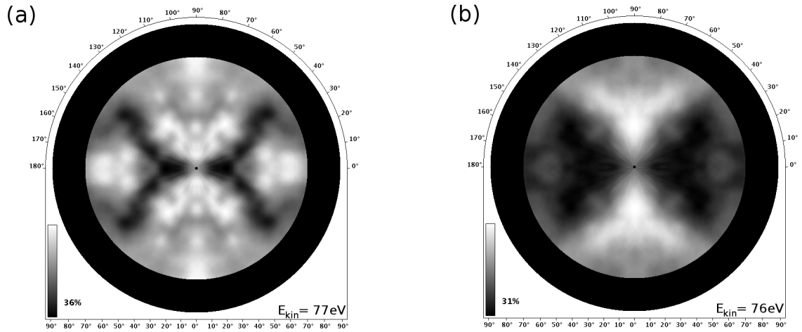
Figure 2: Experimental XPD-pattern of an oxidized Si(110)-surface: Si 2p-signal of the bulk-component (a); Si 2p-signal of the Si 1+ -component (b).
