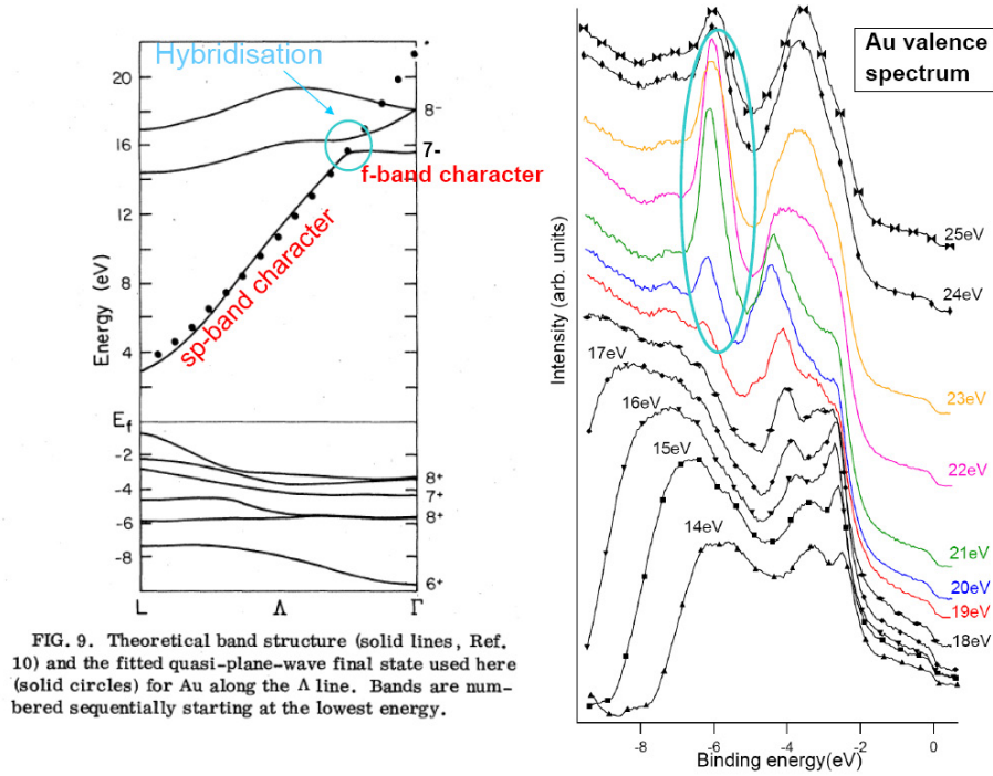
Figure 2: Left: Theoretical band structure of Au (attached from [2]). Right: Au valence spectra measured at DELTA.
