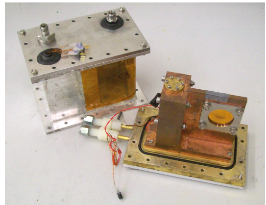
Figure 1: Sample cell with embedded magnetic stirrer.
