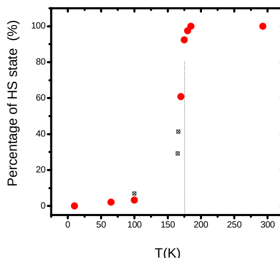
Figure 3: Percentage of HS state \text{Fe(Phen)}_2(\text{NCS})_2 as a function of temperature after linear recombination analysis of the XANES spectra.
