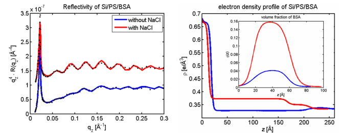
FIG. 4: (Left) XRR data (dotted) and refinements (solid lines) for the adsorption of BSA at the hydrophobic polystyrene-water interface in the presence and absence of NaCl (1 mM) [3]. (Right) Corresponding electron density profiles [3]. To visualize details of the adsorbed layers, the volume fraction profiles are displayed in the inset.
