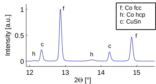
Figure 1: XRD pattern of an industrial workpiece.
