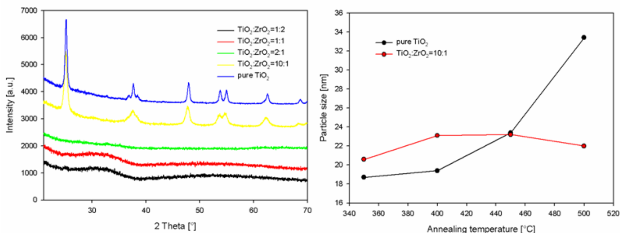
Fig. 2: a) Diffraction patterns of the composite samples after annealing at 500^\circ\text{C} for four hours. b) Particle sizes in dependence of the annealing temperature for the two crystallised samples as determined from XRD analysis.
