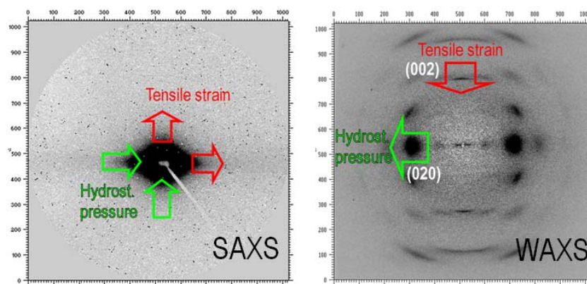
Fig. 3: Comparison of the effects of (hydrostatic) pressure and axis (tensile) strain applied to silk fibers and the resulting changes in the SAXS and WAXS scattering patterns. Left: The red and green arrows indicate how the SAXS scattering pattern grows and shrinks due to tensile stress and hydrostatic pressure, respectively. Right: The red and green arrows indicate the shifts of the (002) and (020) reflections as the fiber is exposed to tensile stress and undirected hydrostatic pressure, respectively.
