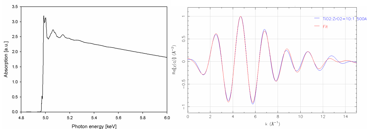
Fig. 5: a) The Ti K-EXAFS spectrum of the sample \text{TiO}_2\text{:ZrO}_2=10\text{:}1 annealed at 500^\circ\text{C} . b) A fit of the data in the q space.
