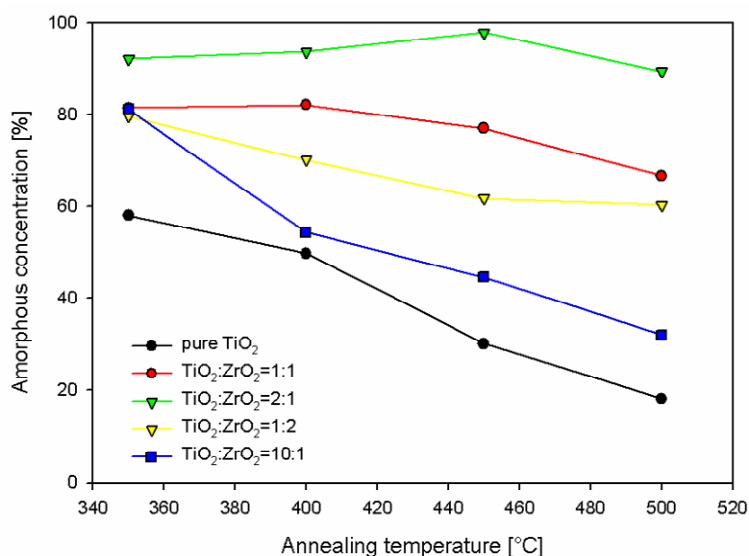
Fig. 2: Amorphous contents on the \text{TiO}_2 - \text{ZrO}_2 composite powders determined from linear combination XANES analysis. Only in the pure \text{TiO}_2 and the \text{TiO}_2:\text{ZrO}_2=10:1 samples significant crystallisation occurs.
