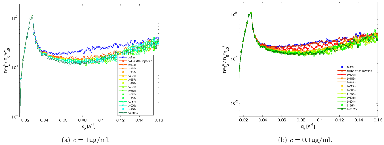
Figure 2: Intensity as a function of the wave vector transfer q_z = \frac{4\pi}{\lambda} \sin \theta for two different protein concentrations. \lambda is the wavelength of the incident radiation.
