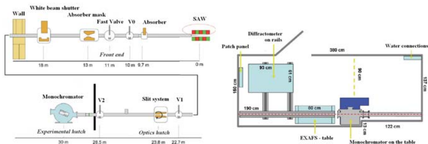
(a) BL10 Lay-out and main components (b) Experimental hut (top-view).
