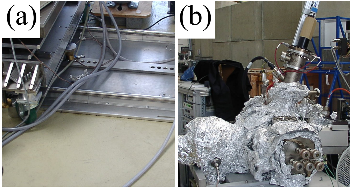
Figure 1: (a) The rail-system allowing a precise and reproducible mounting of the experiment. (b) CCD camera without cover box.
