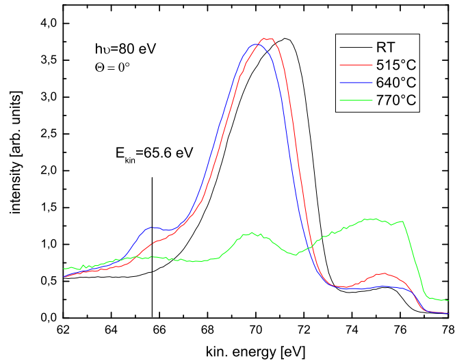
Figure 1: \text{TiO}_2 spectra after annealing at different temperatures. After annealing at 515^\circ\text{C} , a new spectral component arises in the spectra, which is displayed at E_{kin} \approx 65.6 eV kinetic energy. The new component vanishes after an annealing at 770^\circ\text{C} .
