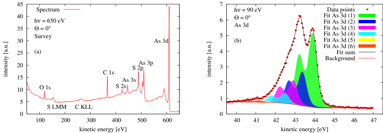
Figure 1: Spectra of the unmodified sample. Survey scan (a), high-resolution scan of the As 3d peak (b).
