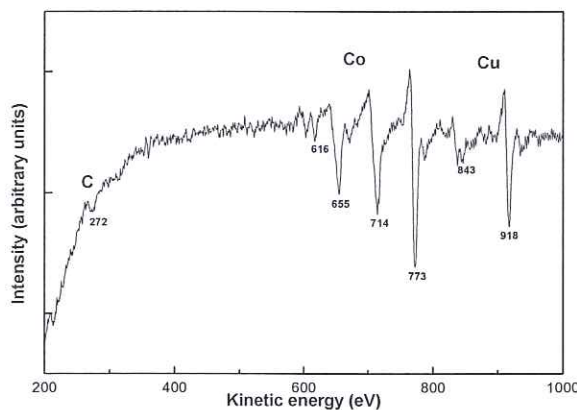
Figure 5: AES spectrum of Co on Cu (100)
