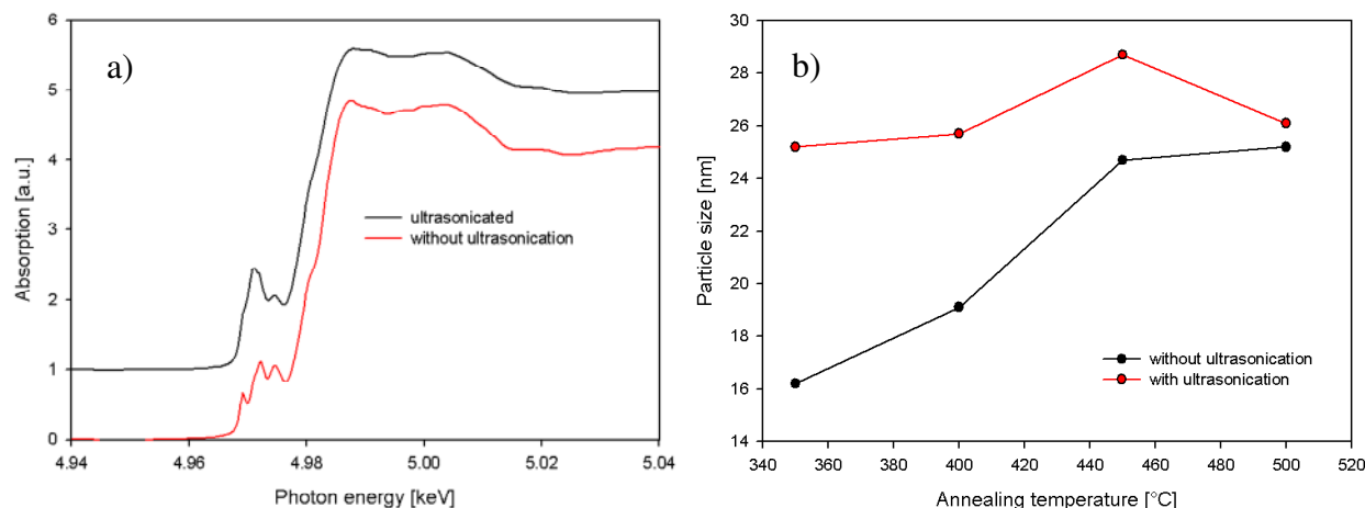
Fig. 1: a) Near edge absorption spectra of \text{TiO}_2 samples prepared with 1 M NaOH annealed at 400°C. Significant structural differences can be observed especially in the pre-edge region. b) The particle sizes of the powders synthesized in 1M KOH with and without ultrasonication after annealing. The sizes of the particles in the ultrasonicated powders are larger.
