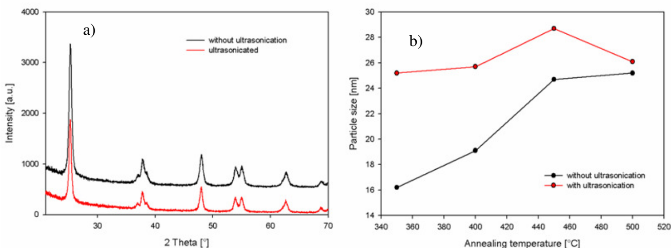
Fig. 1: a) Diffraction patterns of \text{TiO}_2 powders synthesized with 1 M NaOH and annealed at 450°C for four hours. b) Development of the particle size with increasing annealing temperature in samples synthesized with 1M KOH. The trend of higher particle sizes in the ultrasonicated samples is also visible in the case of samples prepared with 1M NaOH.
