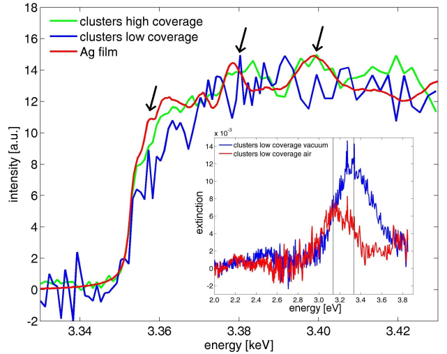
Figure 1: Large: XANES spectra of a Ag film and two different packing densities of Ag clusters. Small: Silver plasmons at low coverage in vacuum before and after exposure to air.
