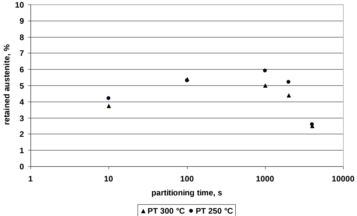
Figure 2: Effect of partitioning time on retained austenite
