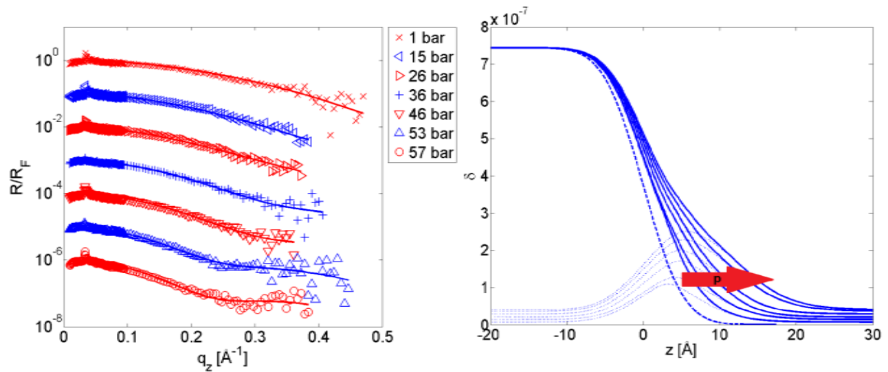
Fig. 3: Normalized and shifted reflectivities of carbon dioxide on a silicon wafer for different pressures at T = 36.7\text{ }^\circ\text{C} ( > T_c = 31\text{ }^\circ\text{C} ) and the corresponding dispersion profiles perpendicular to the surface.
