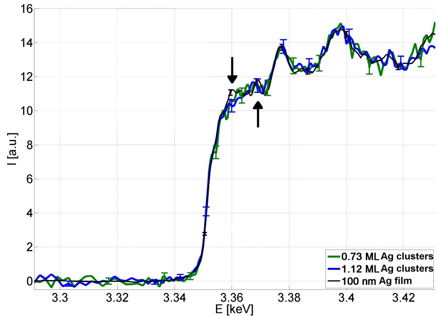
Figure 1: XANES spectra of the Ag L_3 edge of a Ag film and two different packing densities of Ag clusters in PDMS. Differences in the near edge structure indicated with arrows.
