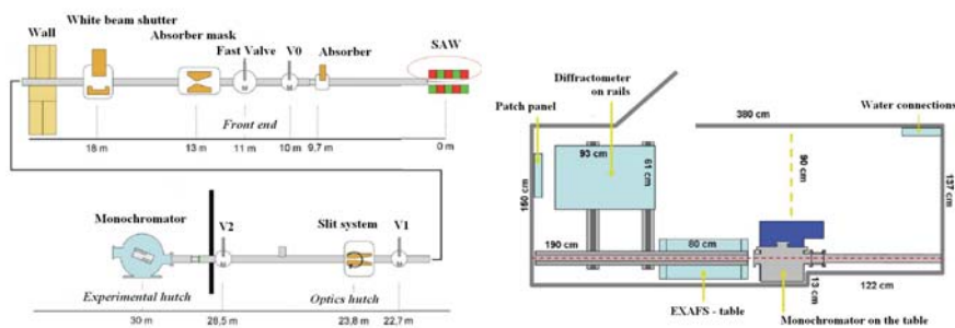
Fig.1 (a) BL10 Lay-out and main components (b) Experimental hutch (top-view).
