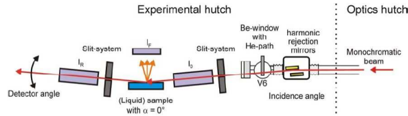
Fig. 1: Sketch of the experimental setup at Beamline BL8. The photon beam is bent down on the sample surface by the harmonic rejection mirror. The incident angle was adjusted to 0.1^\circ . [7]
