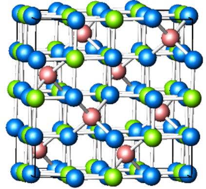
Figure 1: \text{NiFe}_2\text{O}_4 crystallizes in an inverse spinel structure.
