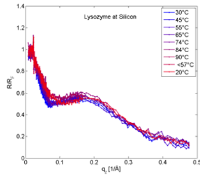
Fig. 3: Normalised reflectivities of lysozyme on a silicon wafer in pure buffer solution for different temperatures.
