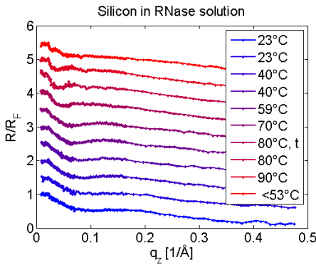
Fig. 4: Normalised and shifted reflectivities of RNase on a silicon wafer in protein solution for different temperatures.
