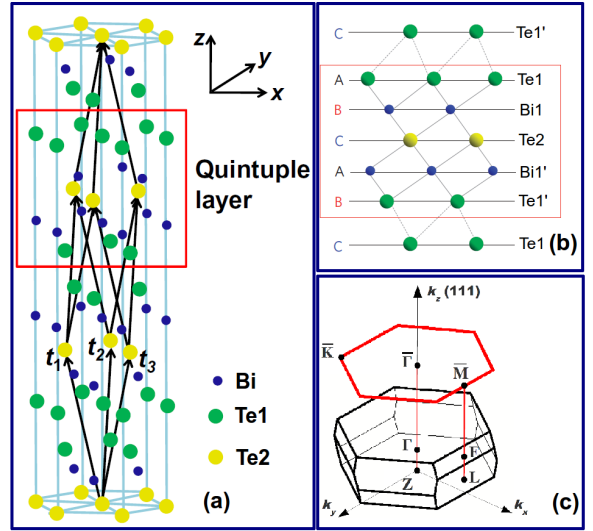
Figure 1: (a) Layered crystal structure of Bi 2 Te 3 . 1QL represents five atomic layers. (b) Schematic representation of 1QL sequence along the z-axis, taken from [2]. (c) Projection of the bulk zone onto the surface.
