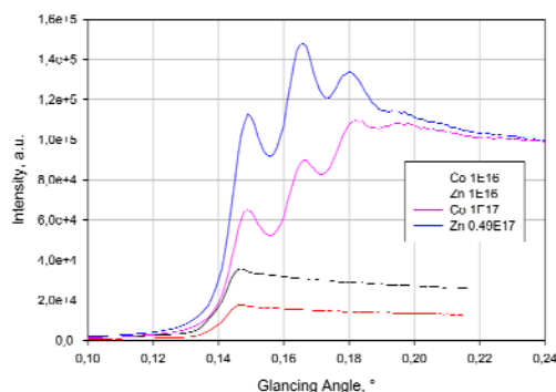
Figure 1. Co- and Zn-ions implanted in Si-wafer. Different slopes of the GIXRF can be observed in dependence of the dose.
