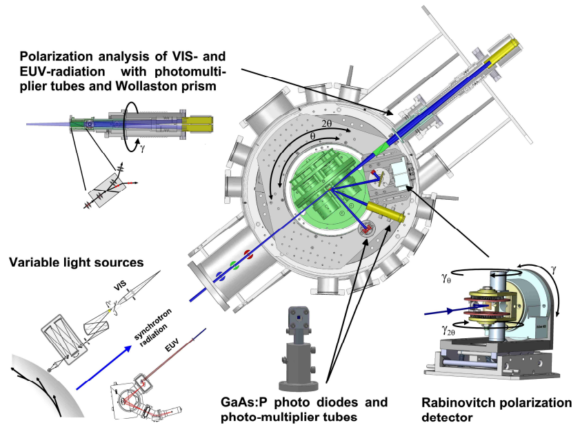
Fig. 1 Experimental setup with optical components and detectors.
