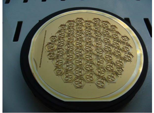
Figure 1: 4-inch Wafer with microgear structure after exposure, post exposure bake and development.
