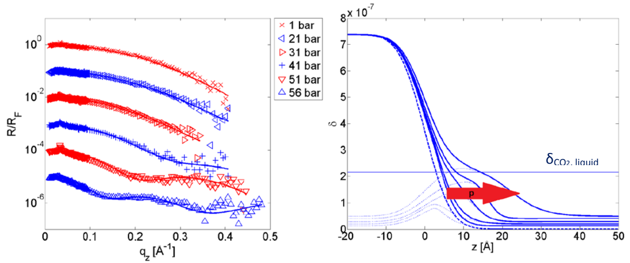
Fig. 2: Normalized and shifted reflectivities of carbon dioxide on a silicon wafer for different pressures at T = 21.5\text{ }^\circ\text{C} ( < T_c = 31\text{ }^\circ\text{C} ) and the corresponding dispersion profiles (dispersion \propto electron density) perpendicular to the surface.
