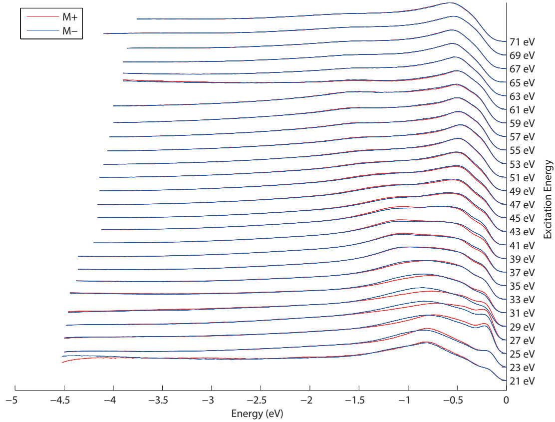
Figure 2: Valence band photoelectron spectra from a 8 ML thick hcp(0001) Co film on tungsten with linearly polarized light for opposite magnetization directions.
