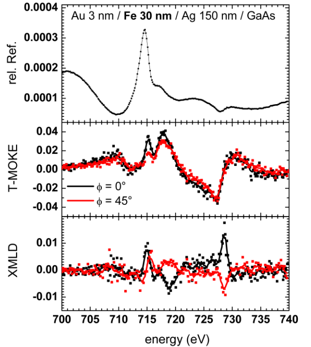
Fig 2: top: relative reflectivity, middle: T-MOKE asymmetry, and XMLD asymmetry of a 30nm crystalline Fe film at near normal incidence for the easy axis \langle 100 \rangle (black) and medium hard axis \langle 110 \rangle (red).
