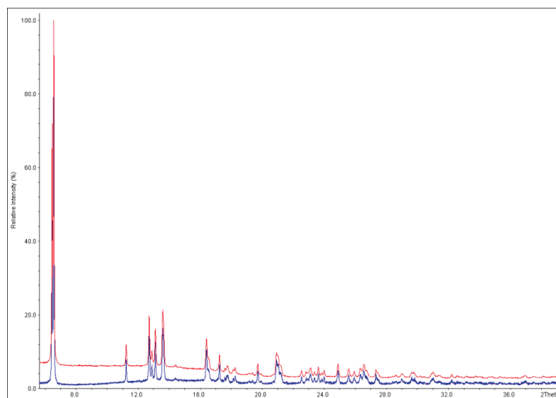
Figure 3: XRPD pattern of \text{Y}(\text{CH}_3\text{CO}_2)_3 (BL09, scintillation counter (blue) vs. Pilatus detector (red)).
