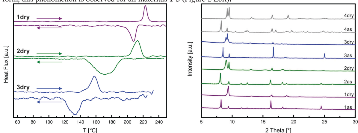
Figure 2: Left: Differential Scanning Calorimetry of the samples 1-3 . The peaks symbolize the phase transitions from np to lp and vice versa; Right: Powder X-ray Diffraction Patterns of the functionalized frameworks in the as-synthesized and in the dry form.
