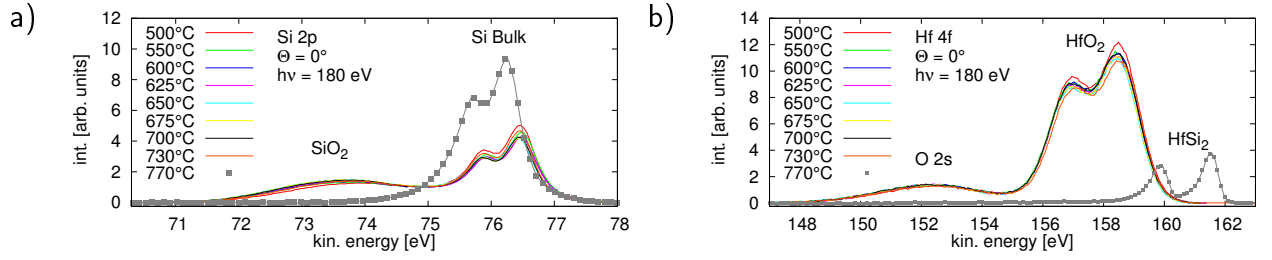
Figure 1: Si 2p a) and Hf 4f b) intensity as a function of temperature. For temperatures up to 730°C all spectra remain nearly constant. After annealing at 770°C spectra indicated by gray squares were recorded. Annealing at this temperature step removed any indication of oxygen from spectra, only Si and Hf signals were detected.
