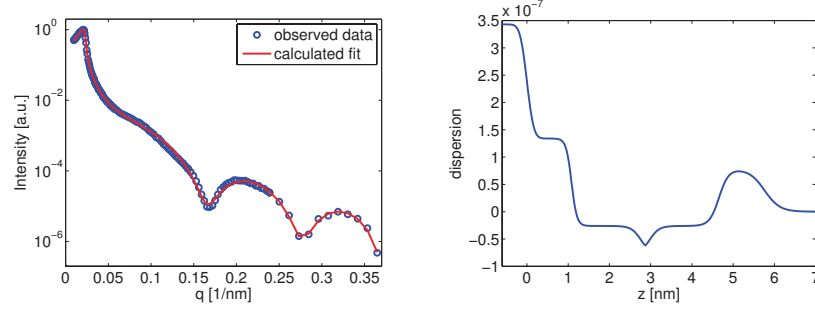
Figure 2: Left: Fit of the XRR-curve of pure DPPC at 39^\circ\text{C} and 30 bar with a bilayer model. Right: Corresponding calculated density profile.
