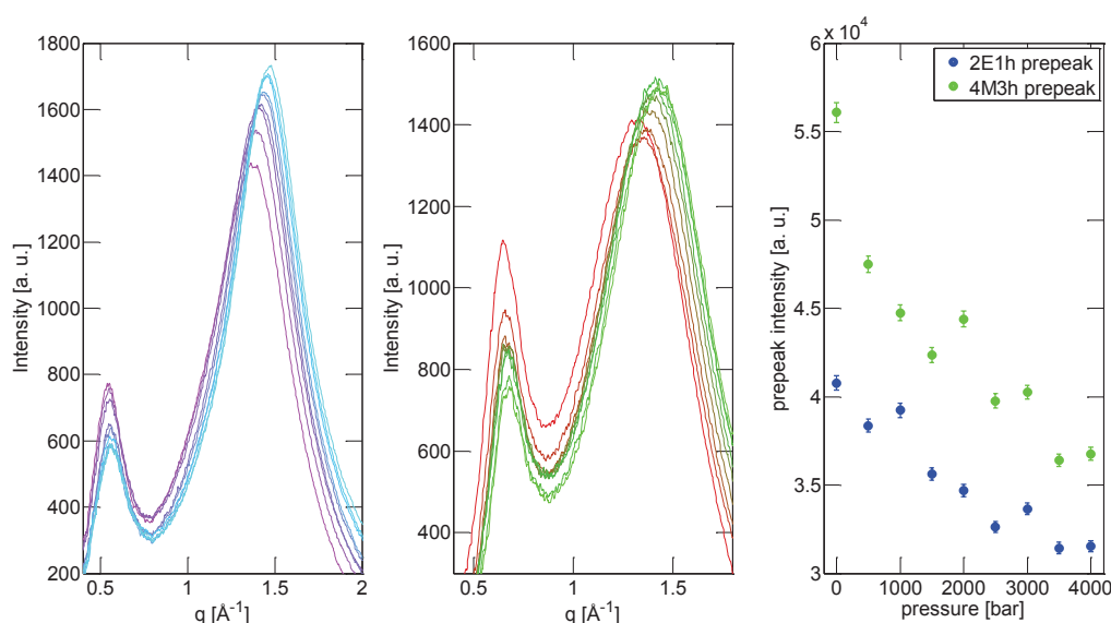
Fig. 2: Pressure dependent structure factor of 2E1h (left) and 4M3h (right). The pressure increases from 1 bar to 4000 bar in steps of 500 bar and the intensity of the prepeak plotted against pressure.
