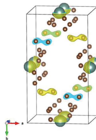
Figure 4: Electron density map of \text{Y}(\text{CH}_3\text{CO}_2)_3 ( Superflip ) [2] .
