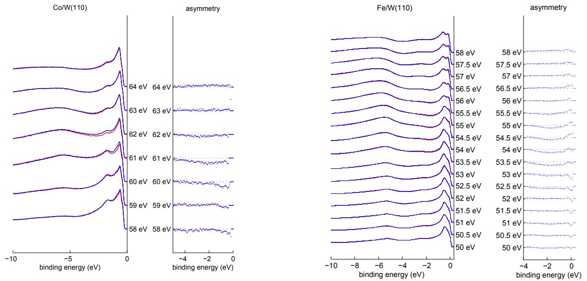
Figure 3: Valence band photoelectron spectra from a) 8 ML thick hcp(0001) Co film and b) 15 ML bcc(110) Fe film on tungsten with linearly polarized light at excitation energies around the 3p core-levels for opposite magnetization directions.
