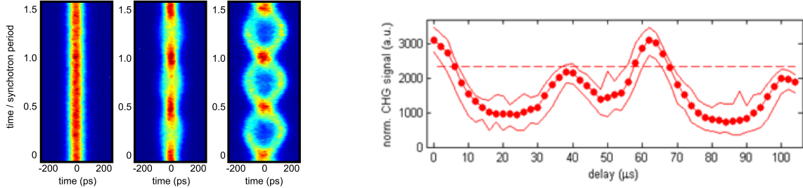
Fig. 3. (left) Evolution of the longitudinal bunch profile (abscissa) over 1.5 synchrotron oscillation periods (ordinate) observed with a streak camera with different parameter sets of RF-phase modulation. (right) CHG signal under the influence of RF-phase modulation after synchronization with varying delay. The dashed line indicates the signal level without RF-phase modulation
