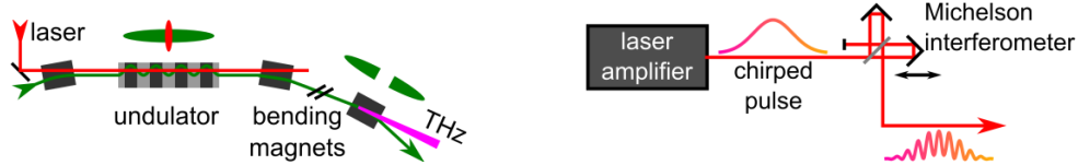
Figure 1: Setup of the short-pulse facility at DELTA (left) and chirped-pulse beating technique (right). See text for details.
