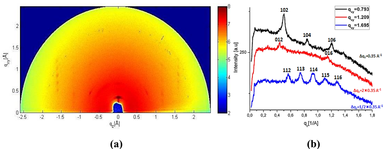
Fig.1 (a) Shows the first two-dimensional GIWAXS plots of the new polymer taken at BL9 of DELTA; (b) Vertical linecuts of the films, q_z is the perpendicular wave vector transfer with respect to substrate surface.
