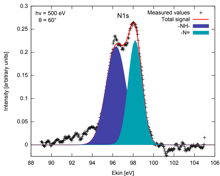
Figure 2: XPS spectrum of the N1s peak of the tetraphenylporphyrin molecule using a photon energy of 500 eV and with a polar angle of 60°. The left peak corresponds to the pyrrolic binding state at 96.3 eV and the right peak to the imminic binding state at 98.2 eV. The signal noise was reduced with 5 point adjacent averaging.
