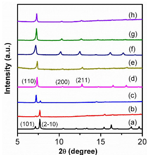
Figure 2 GIXRD patterns of ZIF thin films grown on \text{SiO}_2 surface with 10 deposition cycles in comparison with calculated ZIF-7 and ZIF-8, respectively: (a) calculated bulk ZIF-7 (hexagonal); (b) ZIF-7; (c) ZIF-9; (d) calculated bulk ZIF-8 (cubic); (e) ZIF-8; (f) ZIF-65-Zn; (g) ZIF-67; (h) ZIF-90.
