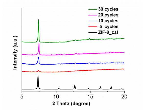
Figure 3 GIXRD patterns of ZIF-8 thin films deposited on \text{SiO}_2 coated QCM substrates with different number of growth cycles.
