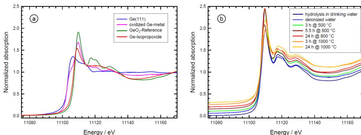
Fig. 1: (a) XANES spectra of Ge-reference samples, i.e. a Ge(111) single crystal, an oxidized polycrystalline Ge sample, \text{GeO}_2 and liquid Ge-isopropoxide \text{Ge}(\text{OCH}(\text{CH}_3)_2)_4 . (b) Comparison of the Ge K-edge XANES spectra of some selected Ge-nanoparticle samples derived by hydrolysis as indicated.
