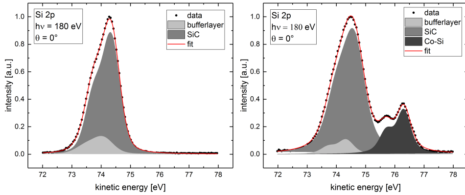
Figure 2: Left: Si 2p photoelectron spectrum recorded before intercalation of Co. Right: Si 2p photoelectron spectrum after in-situ intercalation of Co.
