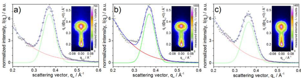
Figure 2. 1D normalized GIWAXS profiles and experimental 2D GIWAXS patterns (insets) of a) 8.1, b) 9.1 and c) 11.0 nm thick P3HT 94 films (thickness determined by AFM). Hollow circles show the averaged experimental intensity, lines represent double-Gaussian fit of the experimental points.
