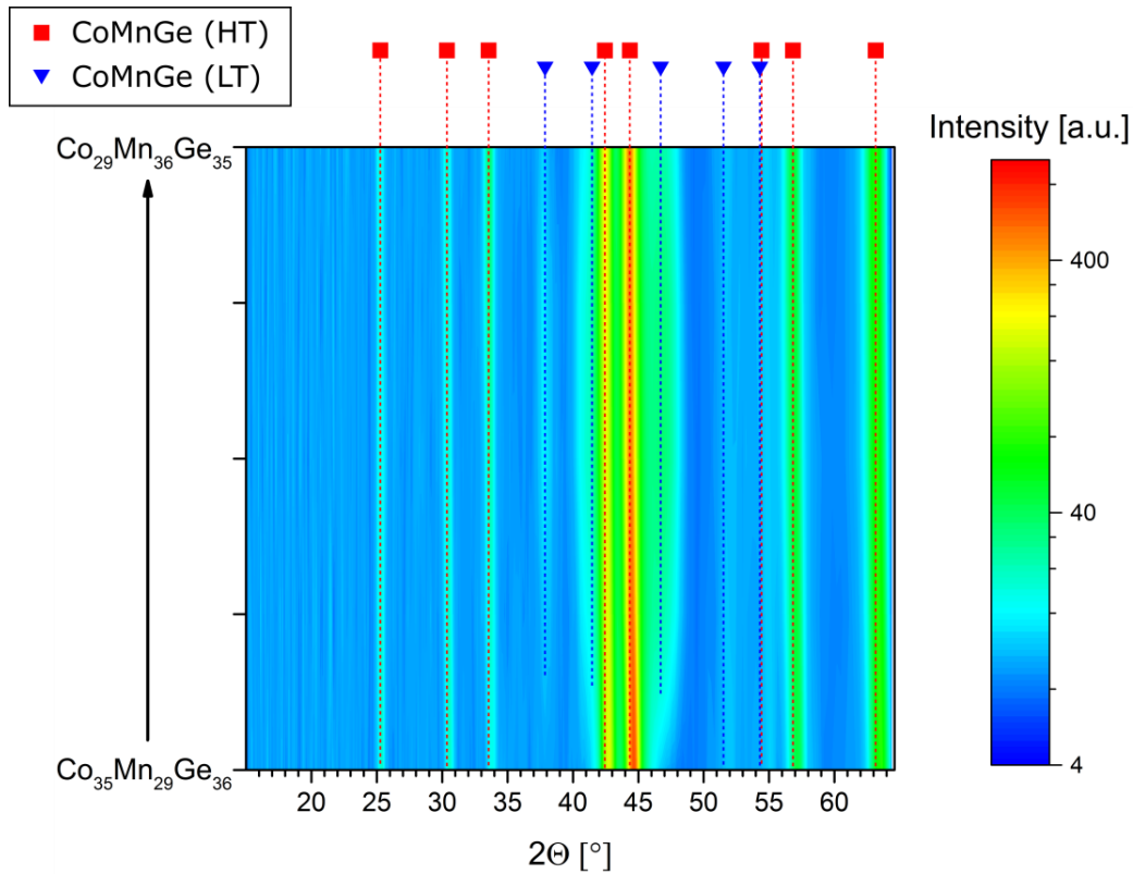
Figure 2: Diffraction patterns integrated along the azimuth and plotted over 2\theta (Cu- K_\alpha ) for increasing Co and decreasing Mn contents as indicated. The signal intensity is shown color-coded (logarithmic scale). The diffraction peaks were identified to correlate with CoMnGe (HT), red squares, and CoMnGe (LT), blue triangles.
