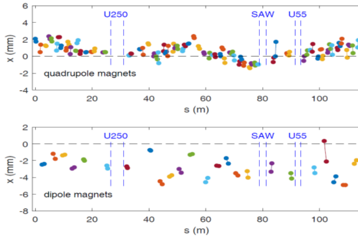
Figure 3: Radial displacement of quadrupole (top) and dipole magnets (bottom) as function of longitudinal position according to a survey in 2016. Each magnet is equipped with two alignment marks shown as two dots of the same color.
