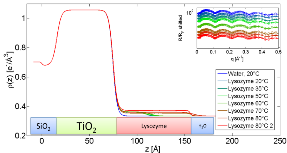
Figure 1: Electron density profiles of lysozyme on TiO 2 as a function of temperature. The XRR data is shown as inset in the figure.
