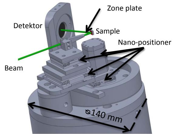
Fig. 1 Setup of SRXM
