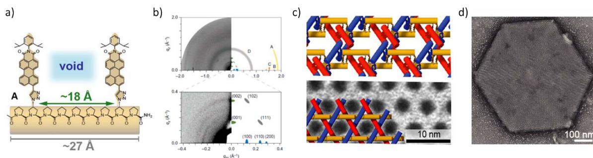
Figure 1. a) Structure of oligoproline-PMI conjugate A, b) GIWAXS pattern, c, d) TEM micrographs of the supramolecular assemblies deposited from THF/H 2 O (30:70) solutions. 3 Copyright 2017 Nature Publishing Group.
