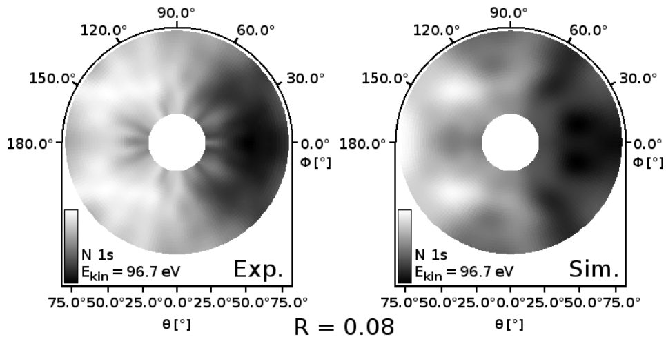
Figure 3: Left: Measured XPD pattern of the N 1s orbital of Caffeine on Ag(110). Right: Simulated XPD pattern of the best fitting structure model. The R-factor of 0.08 shows good accordance between the recorded and simulated pattern.
