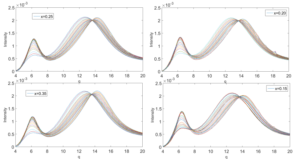
Figure 1: Diffraction patterns of (2\text{E1H})_x(4\text{M3H})_{1-x} mixtures with x=0.15, 0.20, 0.25, 0.35 measured at different temperatures in the range from 175 K to 405K
