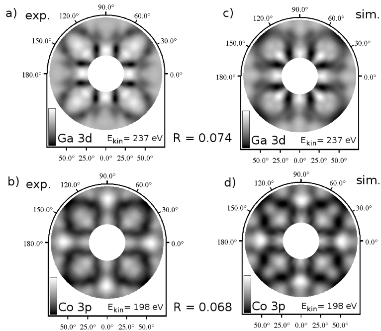
Figure 1: Measured Ga 3d (a) and Co 3p (b) XPD pattern for the Co/GaAs system at E_{\text{ph}}=260 eV and the corresponding simulations (c) and (d). R-factors of 0.074 and 0.068 indicate a perfect match between experiment and simulation, respectively.
