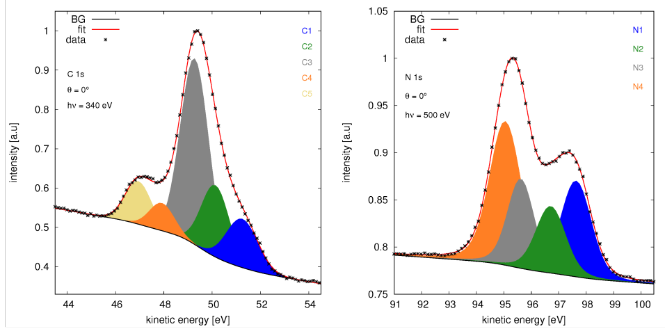
Figure 2: Left: C 1s XPS spectrum of caffeine using a photon energy of E_{\text{hv}} = 340 eV and a polar angle of \Theta = 0^\circ . Right: N 1s XPS spectrum of caffeine using a photon energy of E_{\text{hv}} = 500 eV and a polar angle of \Theta = 0^\circ . The signals are fitted with five and four Voigt-like components, respectively.
