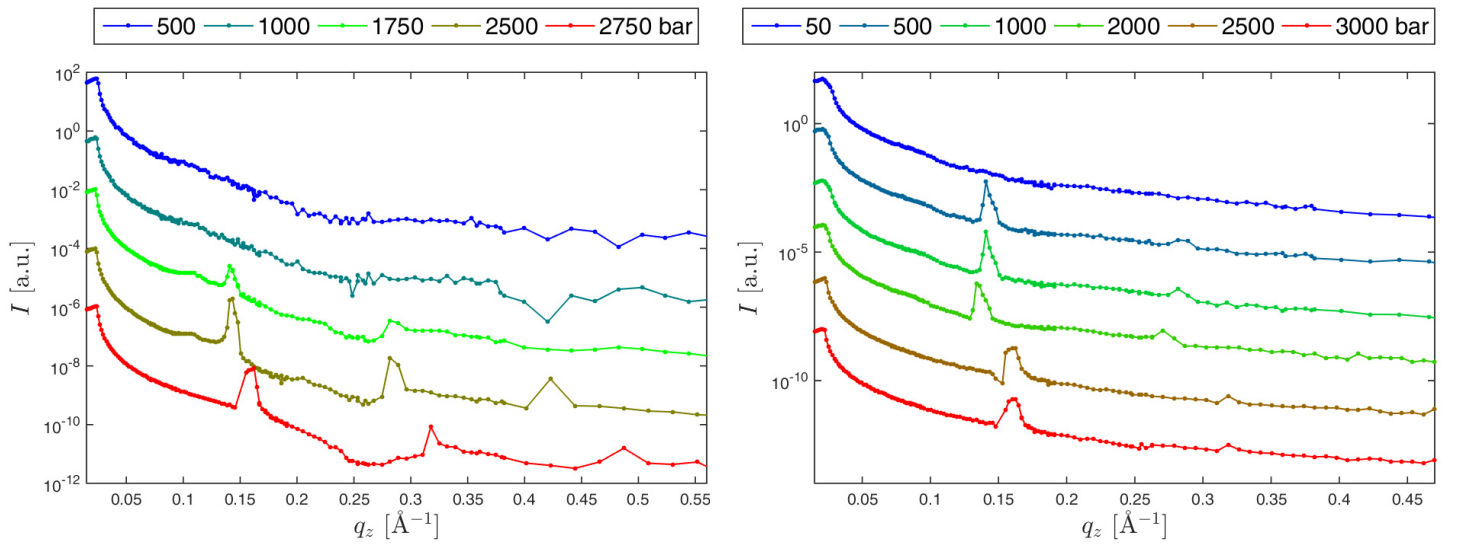
Fig. 2: Reflectivity data of a monoolein/water mixture in absence (left) and presence (right) of HA2-FP.
