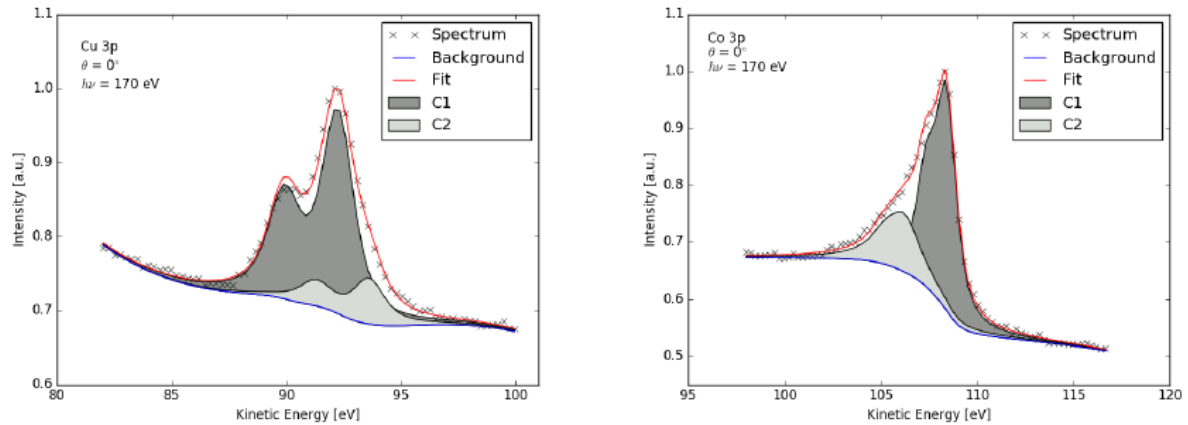
Figure 2: High resolution XPS spectrum of Co/Cu(100) for Cu 3p (left) and Co 3p (right).
