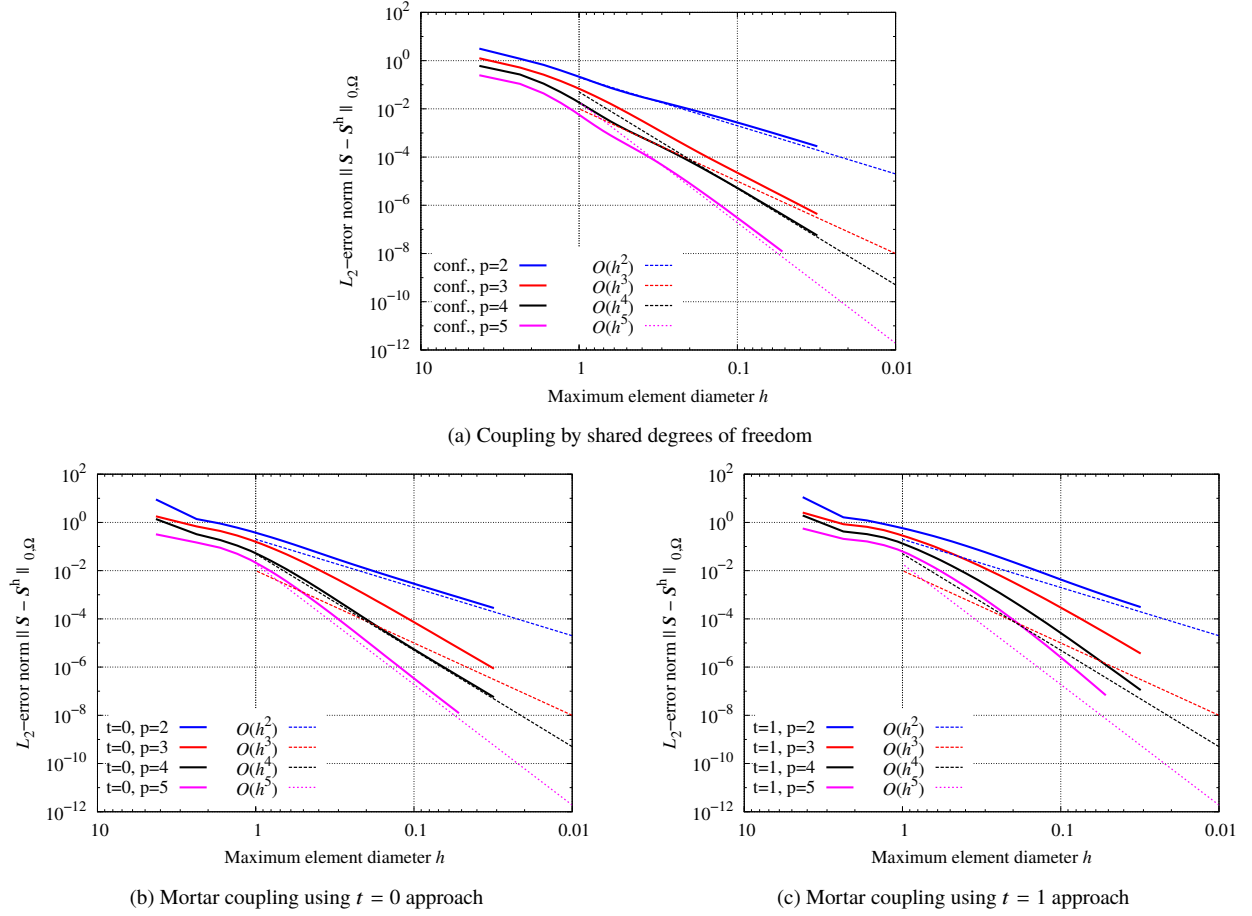
Figure 15: Elastic plate with hole: Comparison of error level and convergence rates for the discretization scheme with curved interface and conforming discretization.
