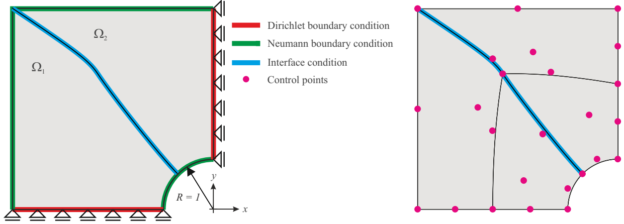
Figure 14: Elastic plate with hole: Discretization scheme with curved interface (left). Coarsest mesh with conforming discretization for this scheme (right)
