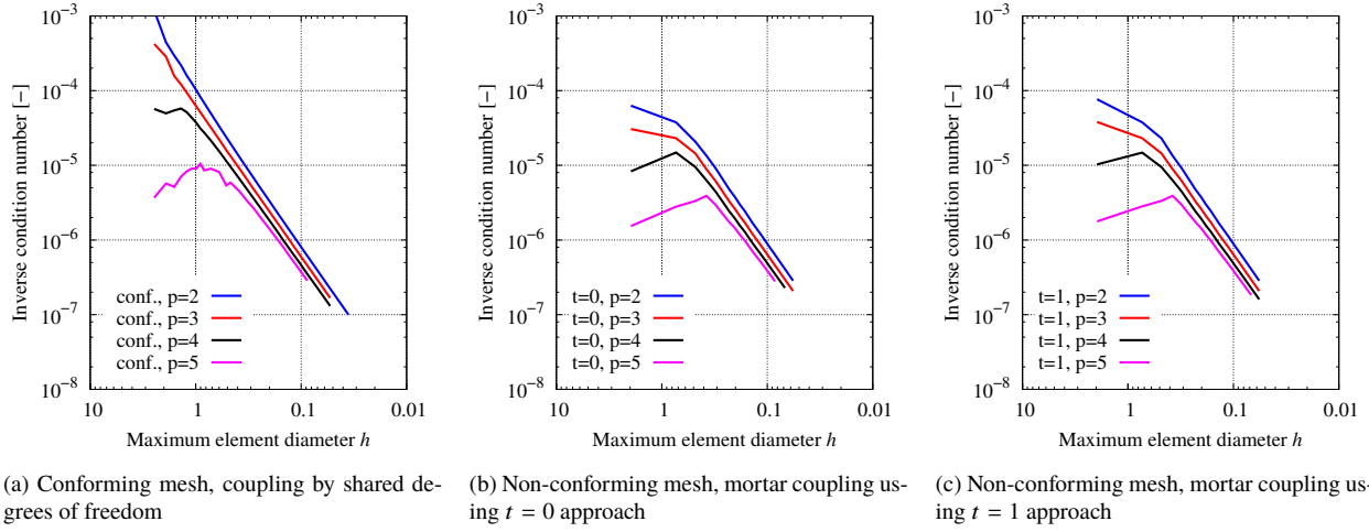
Figure 29: Elastic plate with hole: Inverse condition number of the global system of equations. Comparison between the conforming discretization of Sec. 9.2.1 and the discretization scheme with ten patches of this section.
