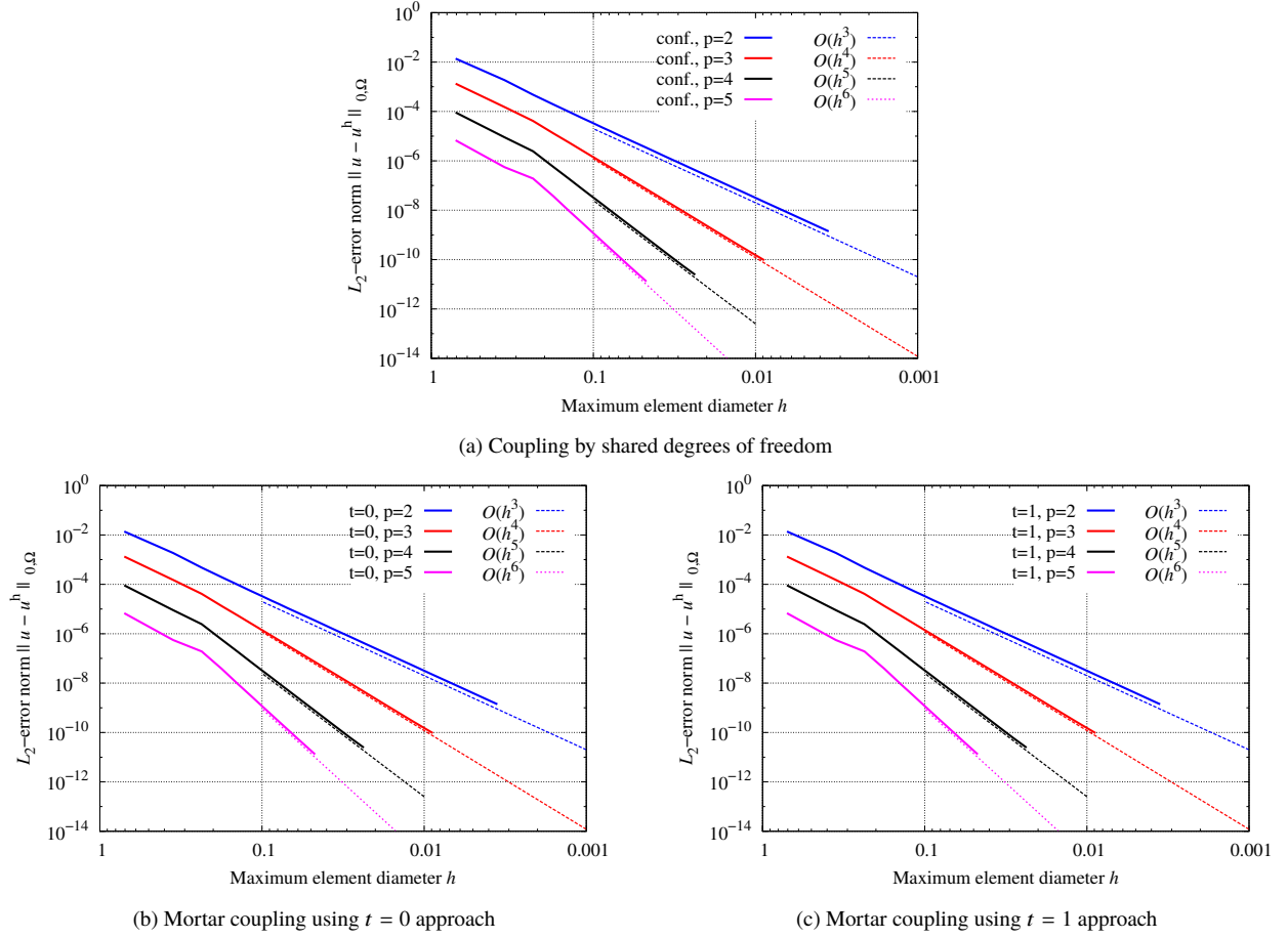
Figure 3: Poisson Equation: Comparison of error level and convergence rates for the discretization scheme with straight interface and conforming knot sequences.
