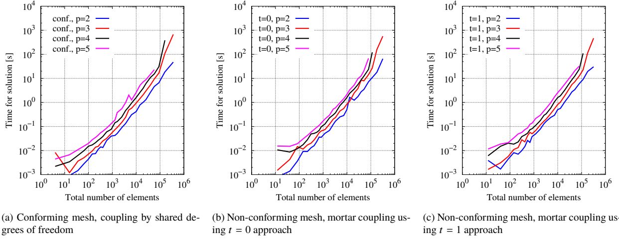
Figure 22: Elastic plate with hole discretized by two patches: Comparison of the CPU time in seconds for the solution of the global system of equations.
