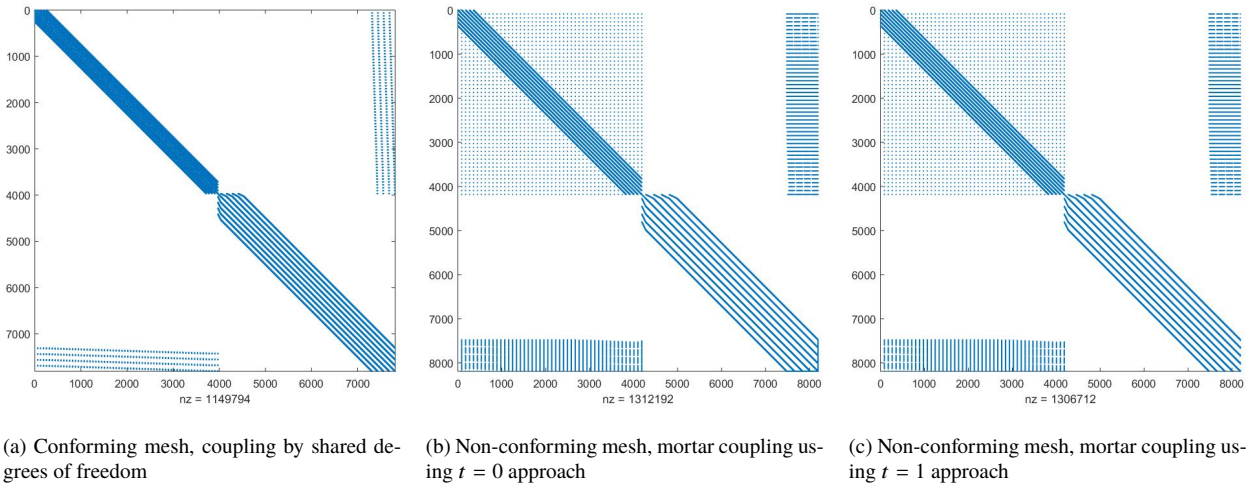
Figure 23: Elastic plate with hole discretized by two patches: Sparsity pattern of the global stiffness matrix. For the conforming mesh a subdivision factor of 28 and p = 4 is used (total number of elements is 3136). For the non-conforming meshes a subdivision factor of 20 and order p = 4 is used (total number of elements is 3280).
