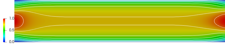
(a) x -velocity from 2D
